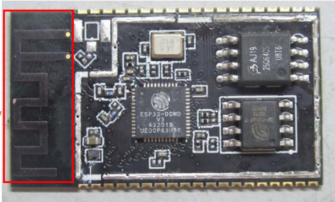
PCB Antenna
