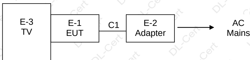
Radiated Spurious Emission Test
