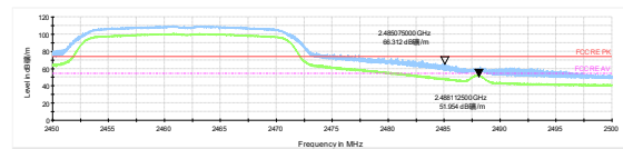
802.11n HT20-Channel 11 Peak+ Average
