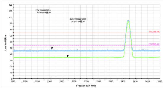
Bluetooth LE (2M) Channel 0 Peak+ Average
