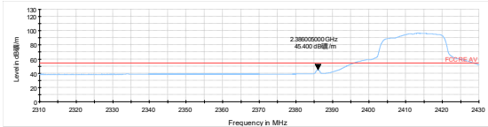
802.11b-Channel 1 Peak+ Average
