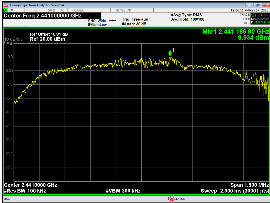
Tx. Spurious 3-DH5 2441MHz Emission
