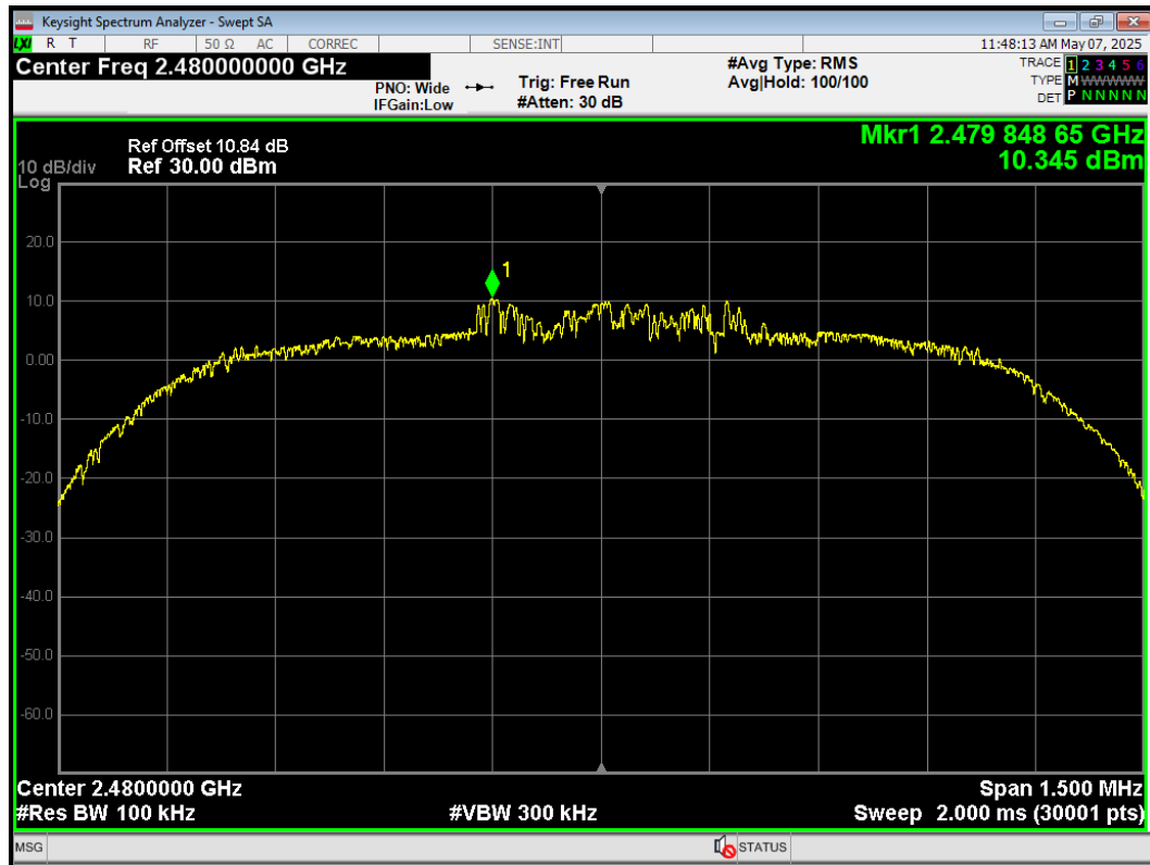
Tx. Spurious 2-DH5 2480MHz Emission
