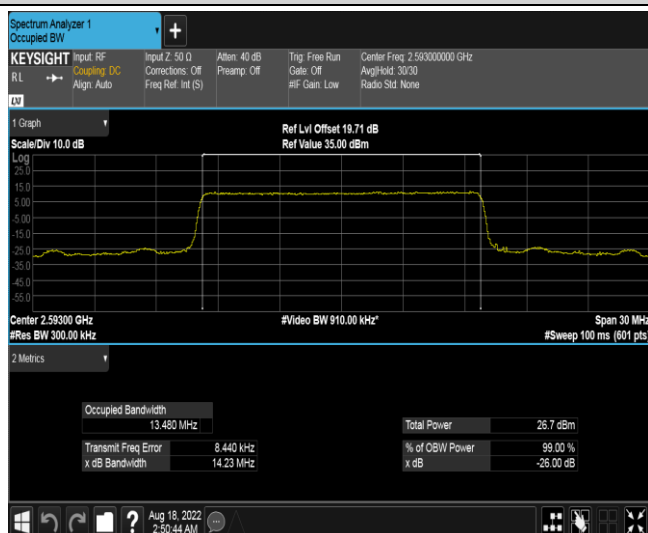
Band41-15MHz-QPSK-41515-75RB#0
