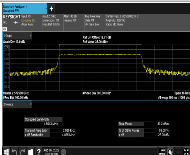
Band38-5MHz-QPSK-38000-25RB#0
