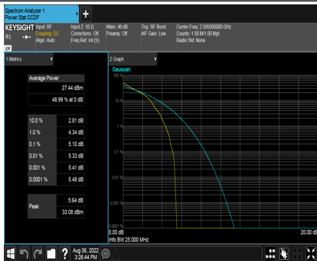
Band38-10MHz-QPSK-38000-1RB#0
