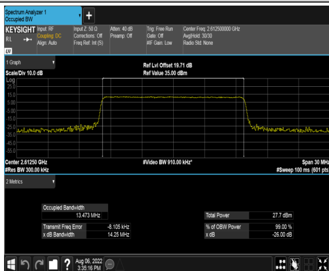
Band38-15MHz-QPSK-38175-75RB#0
