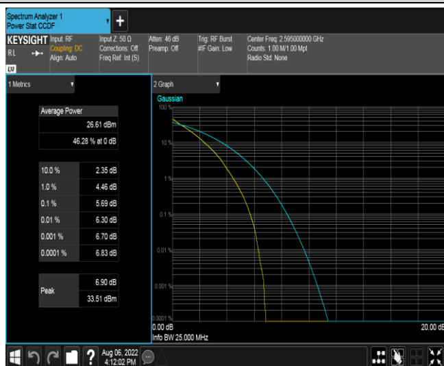
Band38-20MHz-QPSK-38000-100RB#0
