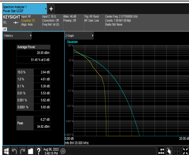
Band38-15MHz-QPSK-37825-1RB#0
