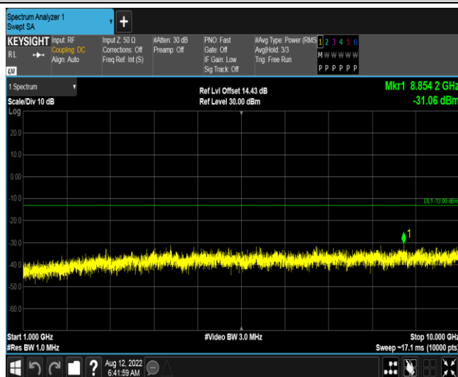
Band26-10MHz-QPSK-26915-1RB#0-Range2:1000~10000MHz
