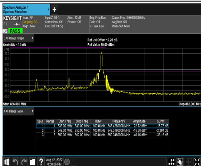
Band26-10MHz-QPSK-26990-1RB#49
