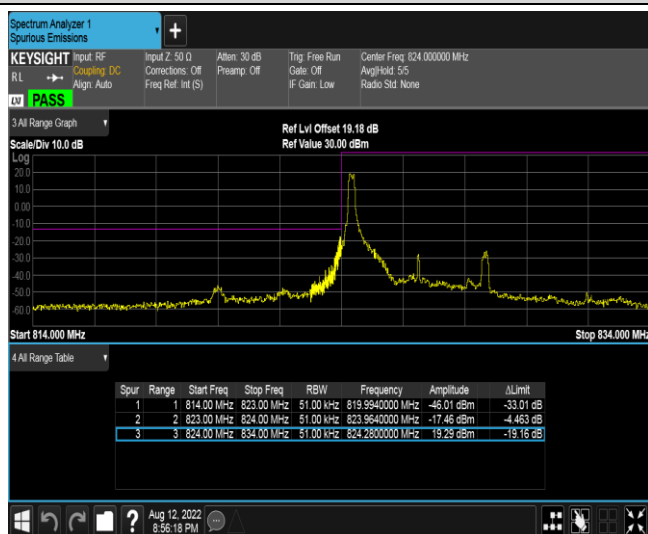
Band26-5MHz-QPSK-26815-1RB#0
