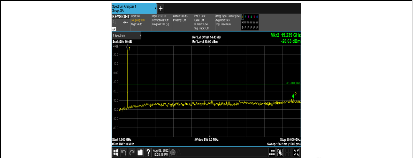
Band25-15MHz-16QAM-26615-1RB#0-Range2:1000~20000MHz
