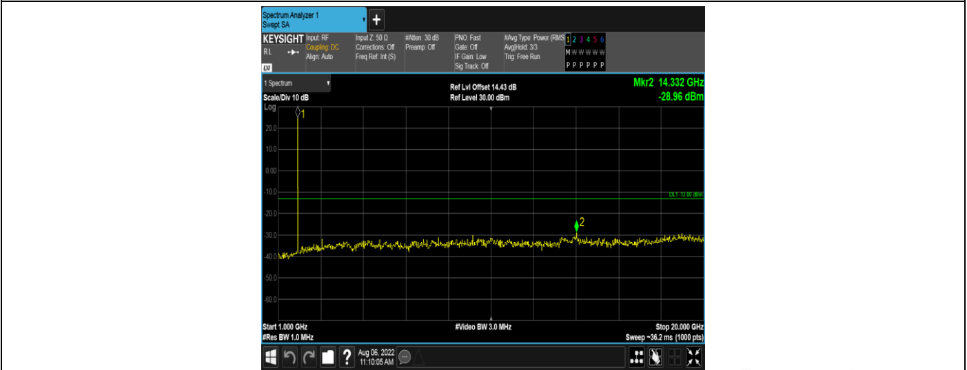
Band25-1.4MHz-16QAM-26365-1RB#0-Range2:1000~20000MHz
