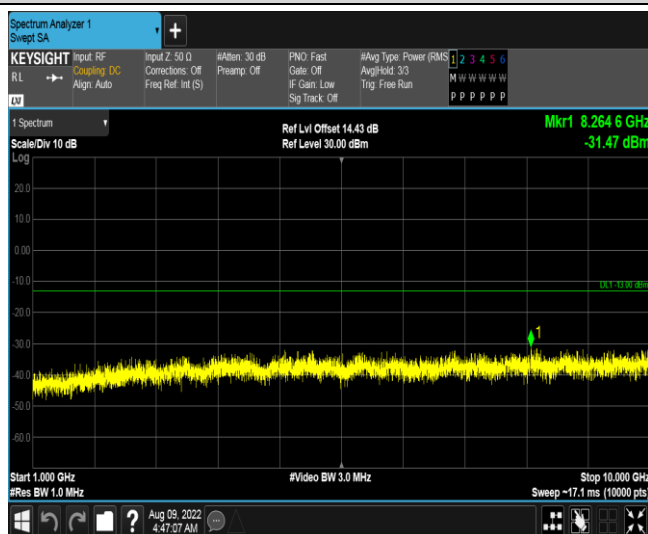
Band19-10MHz-16QAM-24050-1RB#0-Range2:1000~10000MHz
