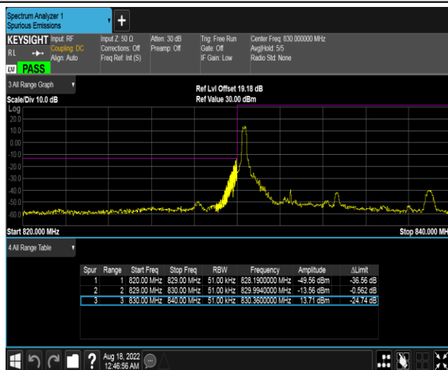
Band19-5MHz-QPSK-24025-1RB#24
