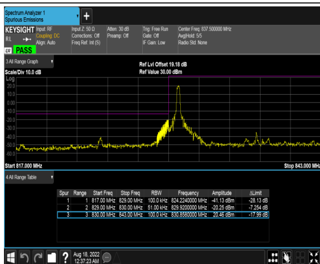
Band19-15MHz-QPSK-24075-1RB#74
