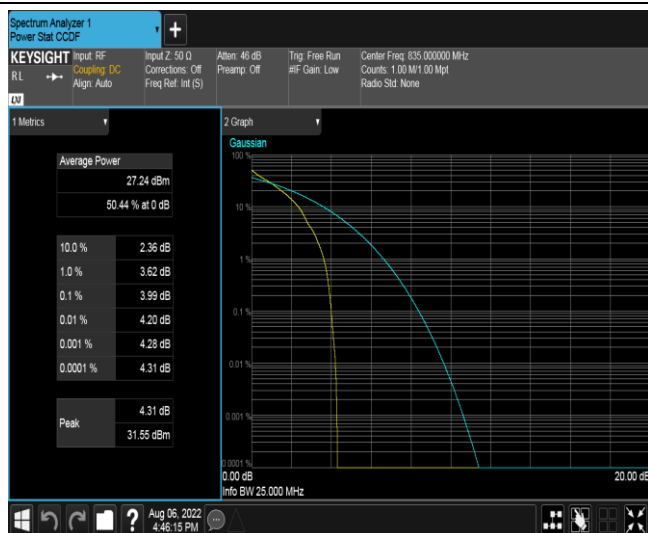
Band19-10MHz-QPSK-24050-50RB#0
