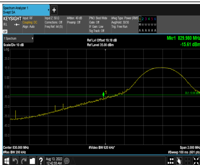
Band19-10MHz-QPSK-24050-1RB#49
