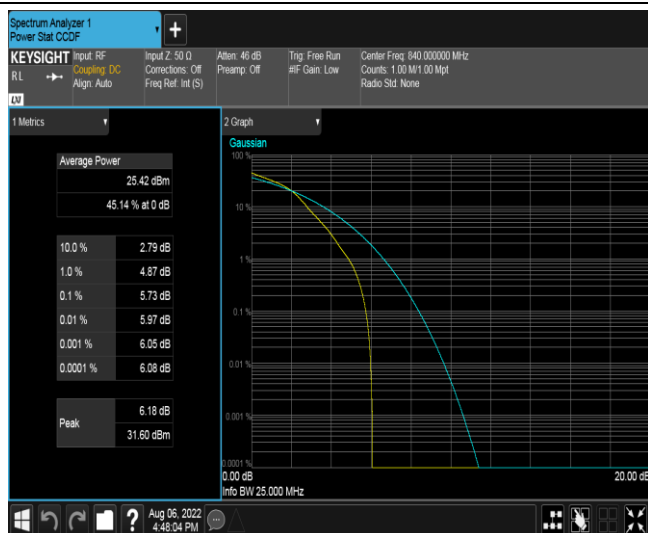
Band19-10MHz-16QAM-24100-50RB#0
