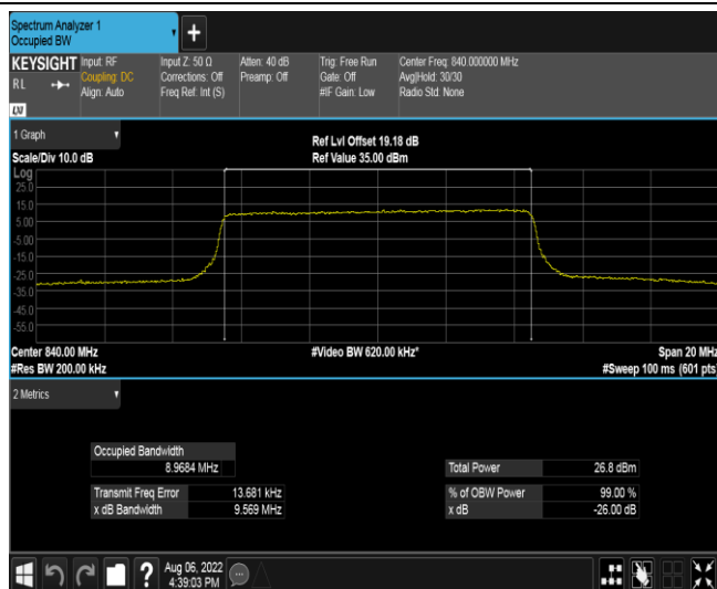
Band19-15MHz-QPSK-24075-75RB#0
