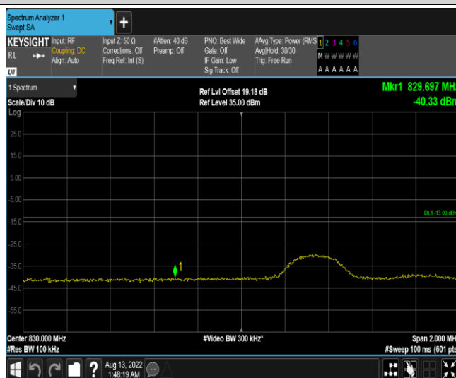
Band19-5MHz-QPSK-24025-25RB#0
