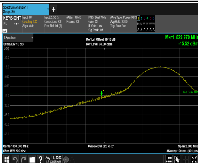
Band19-10MHz-16QAM-24050-1RB#49
