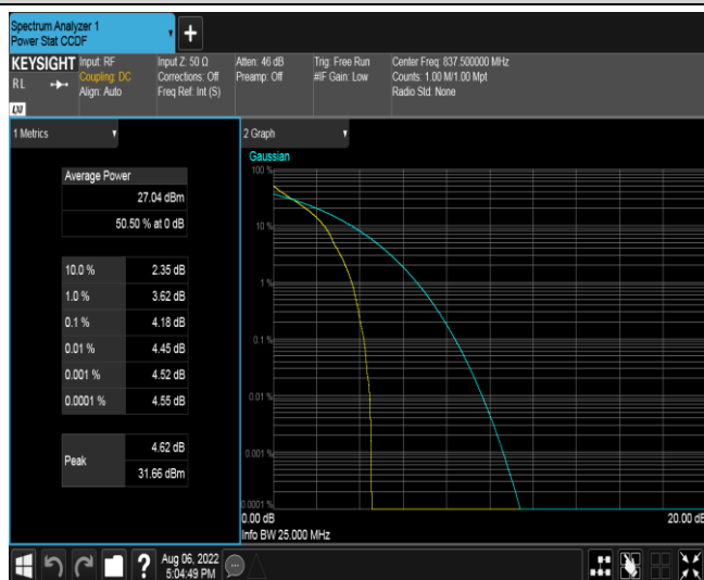
Band19-15MHz-QPSK-24075-1RB#0
