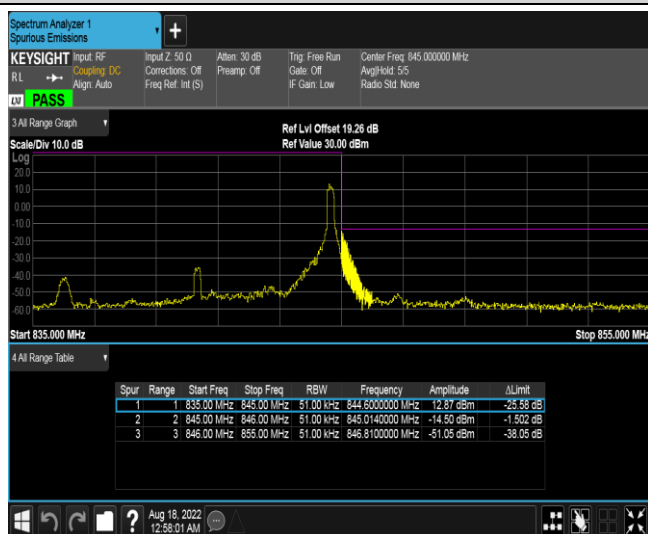
Band19-5MHz-QPSK-24125-1RB#24
