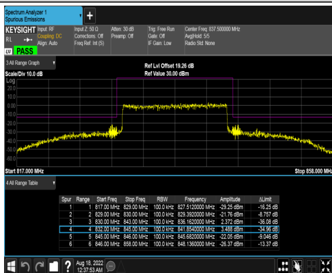
Band19-15MHz-QPSK-24075-75RB#0
