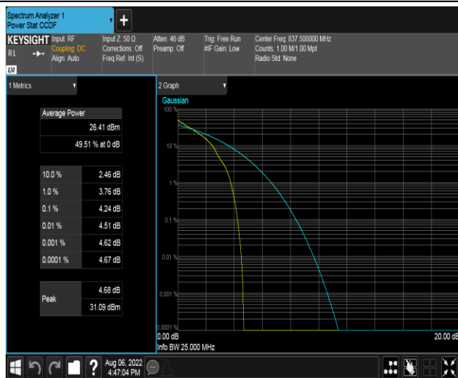
Band19-10MHz-QPSK-24075-1RB#0
