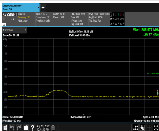
Band19-5MHz-16QAM-24125-1RB#0
