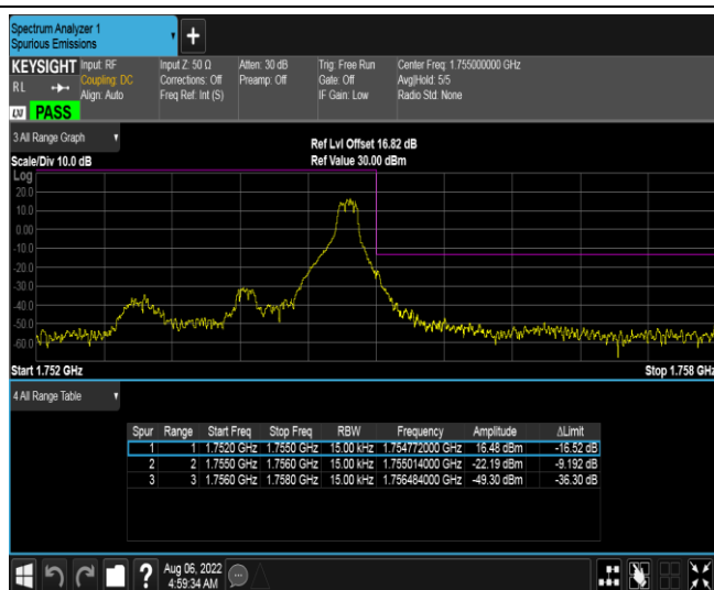
Band4-1.4MHz-16QAM-20393-6RB#0
