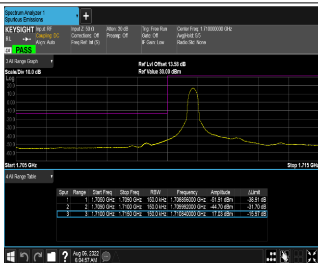
Band4-15MHz-16QAM-20025-75RB#0
