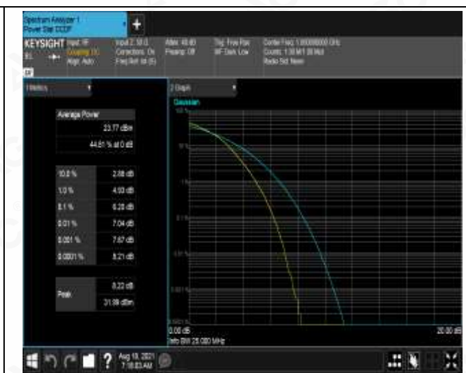
HCH_16QAM_100RB#0
