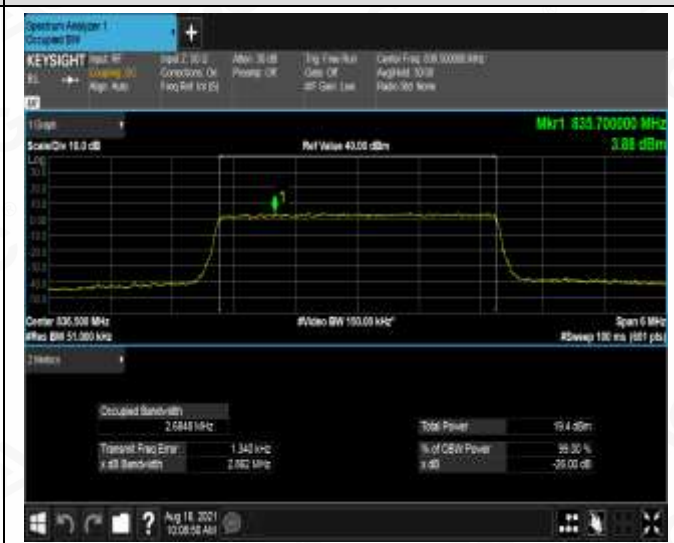
MCH_16QAM_15RB#0
