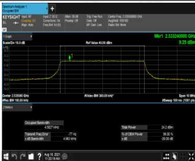
MCH_QPSK_25RB#0
