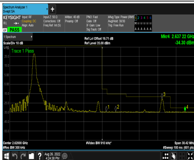
Band38-15MHz-16QAM-38175-1RB#0
