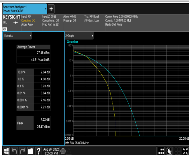
Band38-5MHz-16QAM-38000-25RB#0
