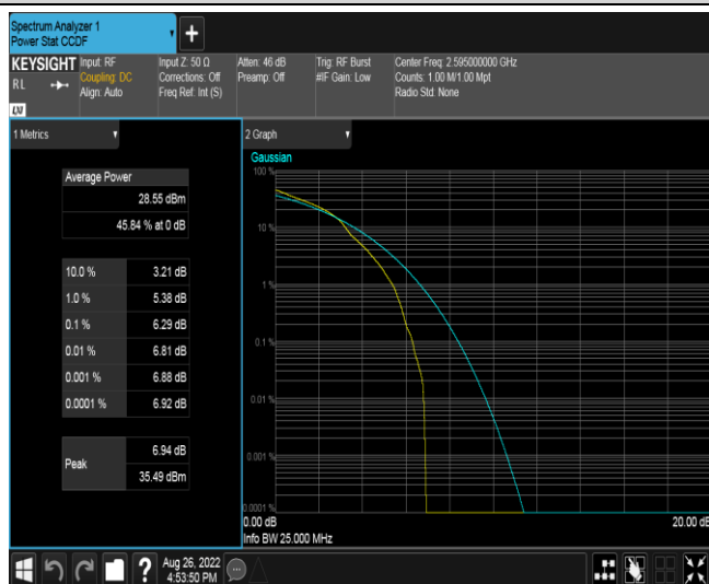
Band38-20MHz-16QAM-38000-1RB#0
