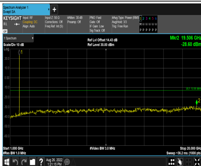
Band25-5MHz-QPSK-26665-1RB#0-Range2:1000~20000MHz
