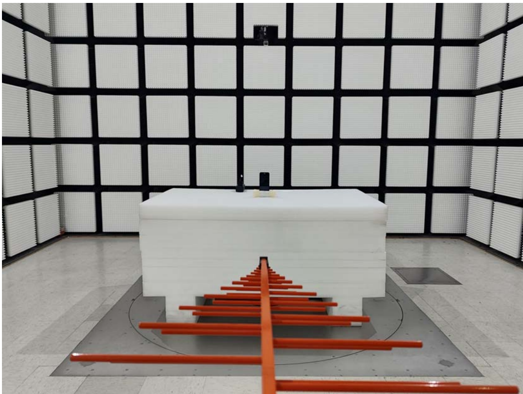
Radiated Emission Below 1GHz View-2B7S-3
