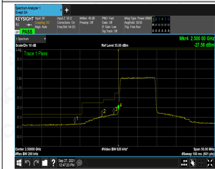
LCH_QPSK_50RB#0
