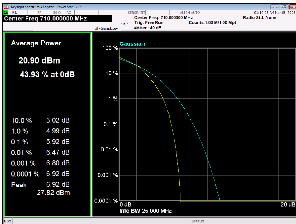
Band17 16QAM BW=10MHz Channel=23790 RB Size=50 Position=#0
