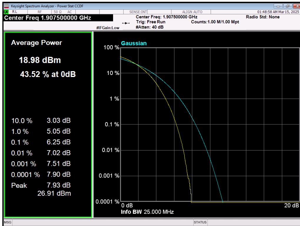
Band25 64QAM BW=15MHz Channel=26615 RB Size=75 Position=#0
