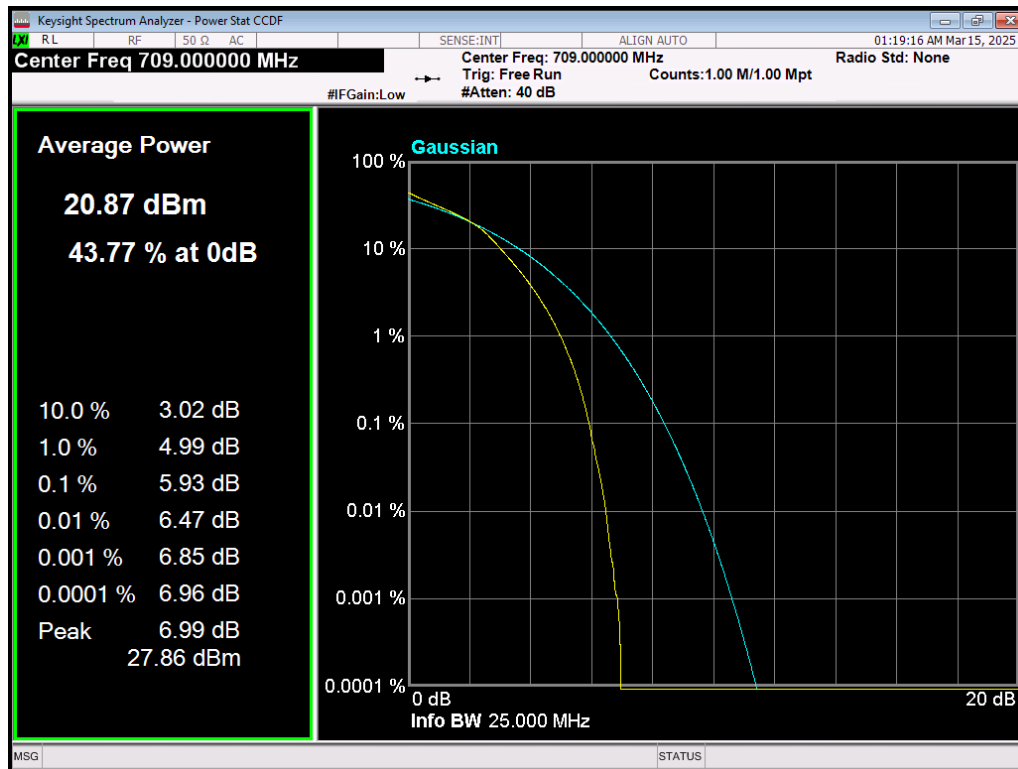
Band17 16QAM BW=10MHz Channel=23780 RB Size=50 Position=#0
