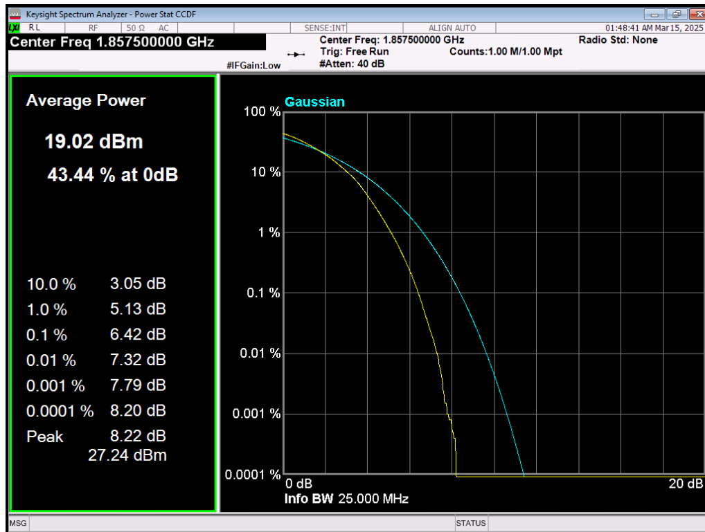
Band25 64QAM BW=15MHz Channel=26115 RB Size=75 Position=#0
