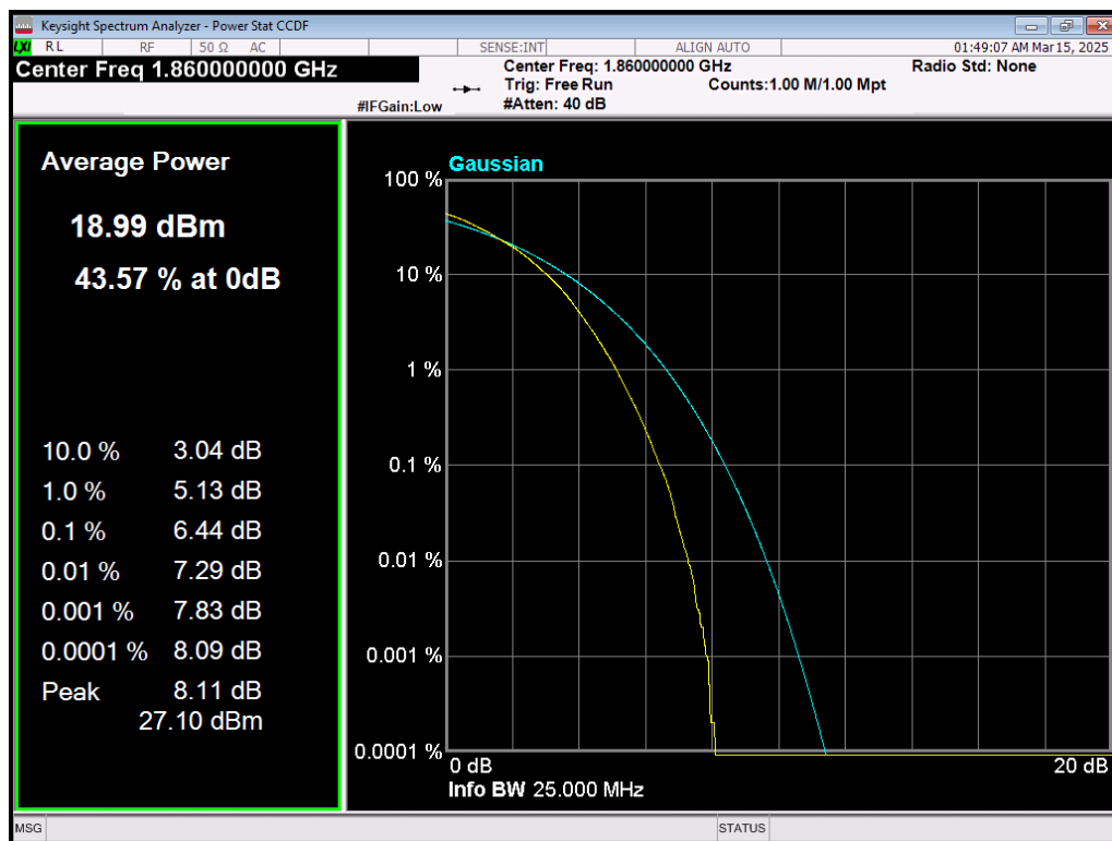
Band25 64QAM BW=20MHz Channel=26140 RB Size=100 Position=#0
