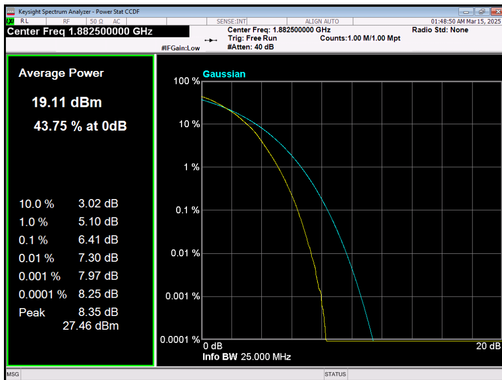
Band25 64QAM BW=15MHz Channel=26365 RB Size=75 Position=#0
