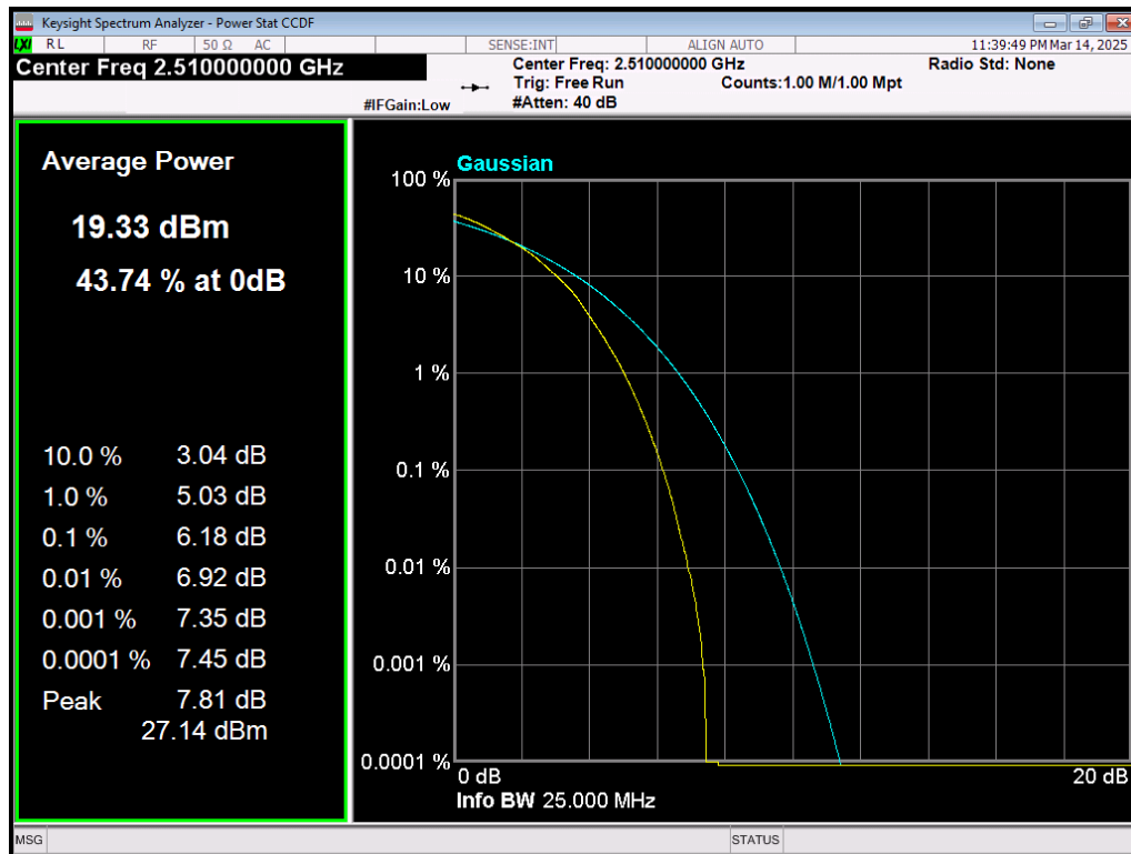
Band7 64QAM BW=20MHz Channel=20850 RB Size=100 Position=#0
