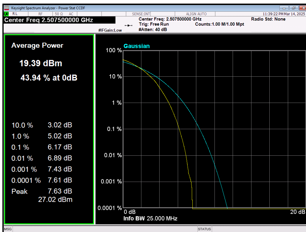
Band7 64QAM BW=15MHz Channel=20825 RB Size=75 Position=#0
