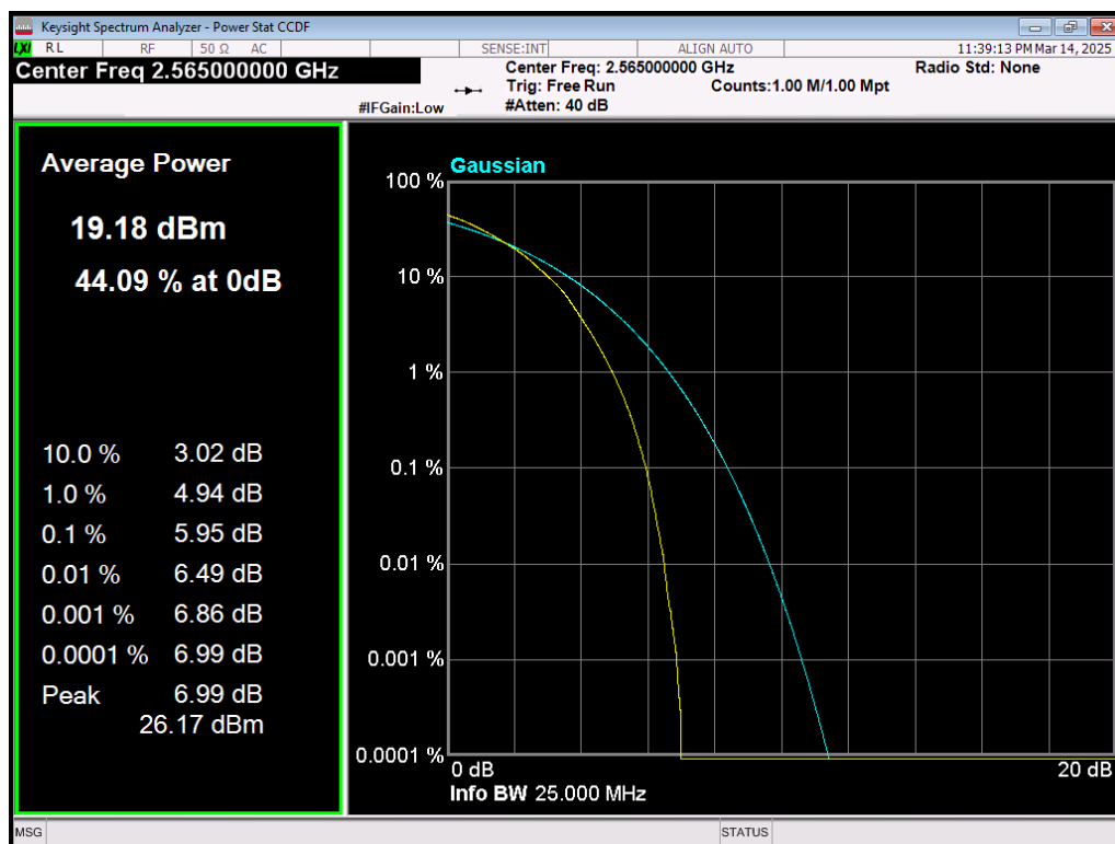
Band7 64QAM BW=10MHz Channel=21400 RB Size=50 Position=#0
