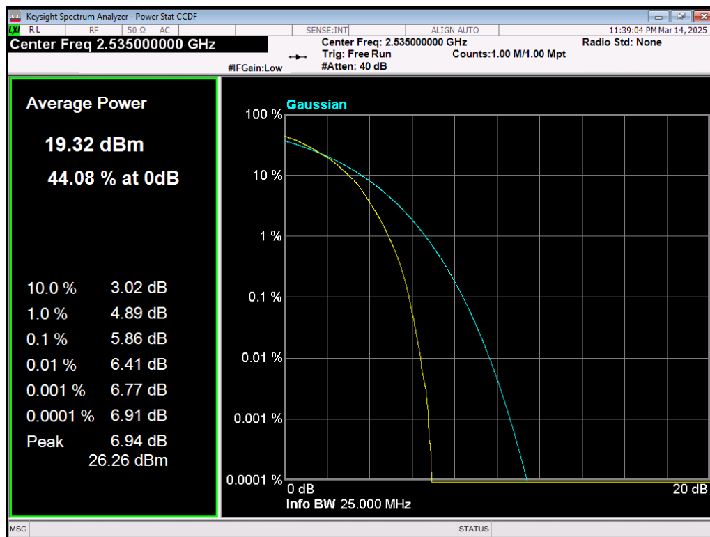
Band7 64QAM BW=10MHz Channel=21100 RB Size=50 Position=#0
