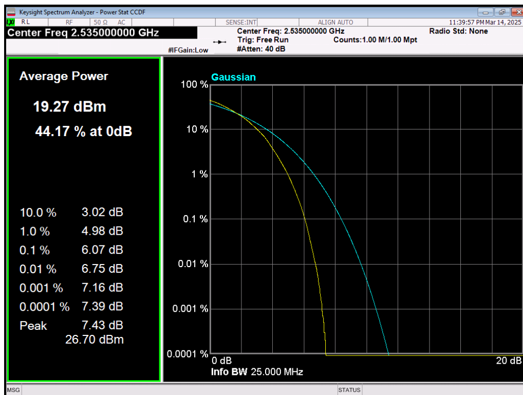
Band7 64QAM BW=20MHz Channel=21100 RB Size=100 Position=#0
