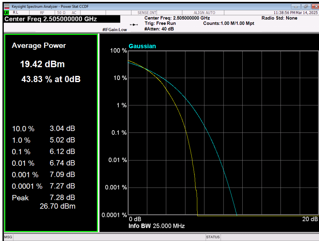
Band7 64QAM BW=10MHz Channel=20800 RB Size=50 Position=#0
