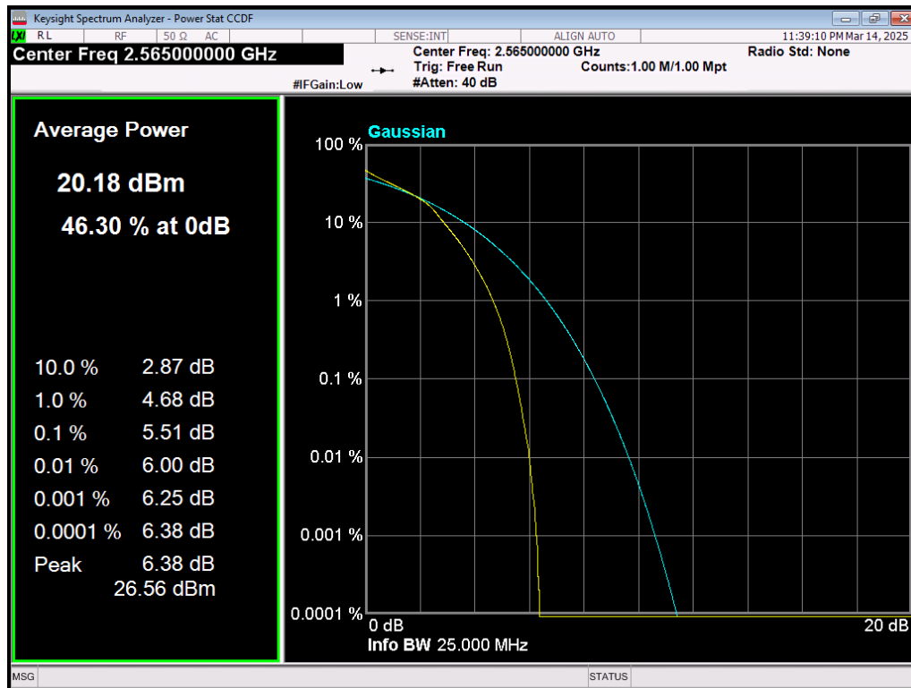
Band7 16QAM BW=10MHz Channel=21400 RB Size=50 Position=#0
