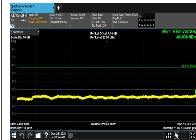
Band26(824-849)-15MHz-QPSK-26965-75RB#0-3000~10000-PASS
