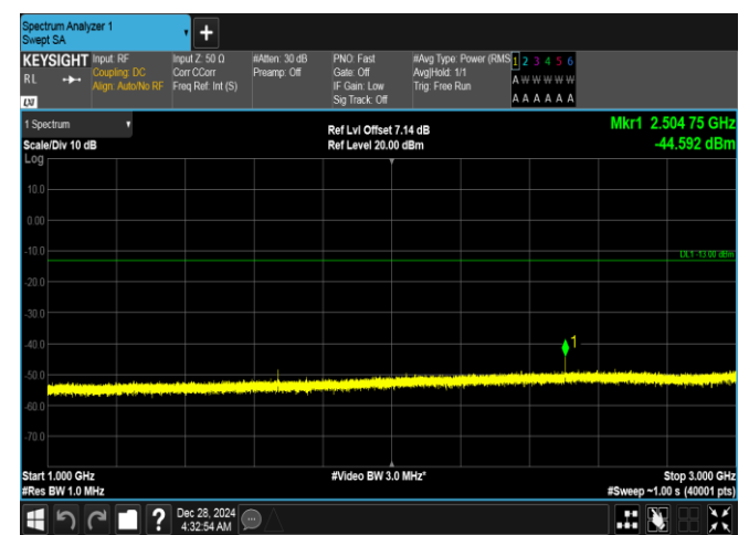
Band26(824-849)-15MHz-QPSK-26965-1RB#0-1000~3000-PASS
