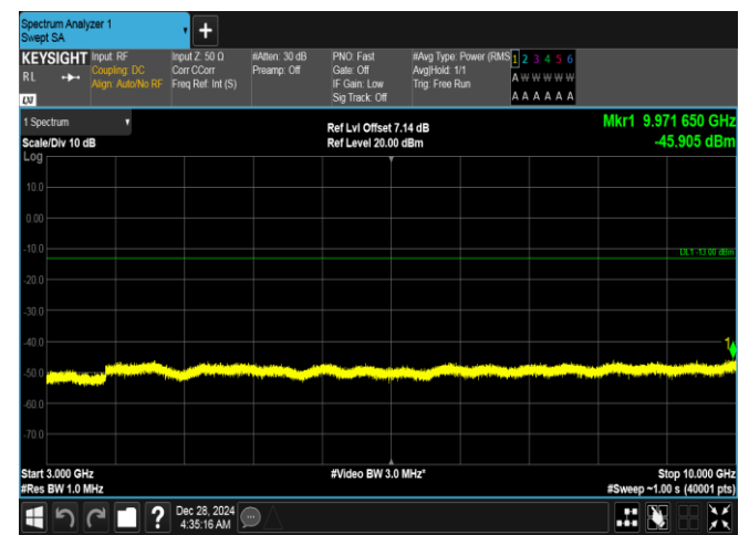
Band26(824-849)-15MHz-QPSK-26965-1RB#74-3000~10000-PASS
