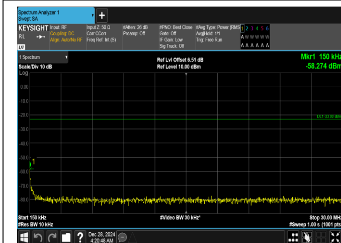
Band26(824-849)-15MHz-16QAM-26865-1RB#0-0.15~30-PASS
