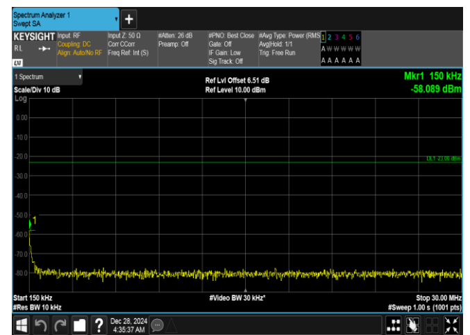
Band26(824-849)-15MHz-16QAM-26965-1RB#74-0.15~30-PASS
