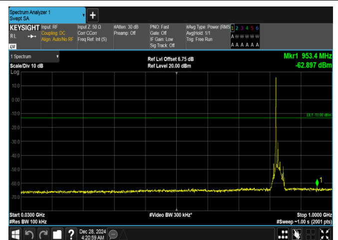
Band26(824-849)-15MHz-16QAM-26865-1RB#0-30~1000-PASS
