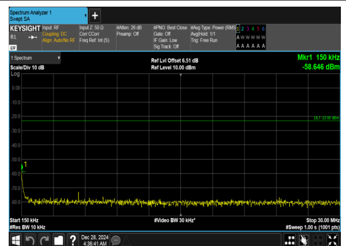
Band26(824-849)-15MHz-QPSK-26965-75RB#0-0.15~30-PASS
