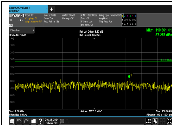
Band26(824-849)-15MHz-QPSK-26965-1RB#0-0.009~0.15-PASS
