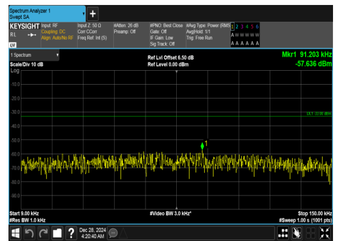
Band26(824-849)-15MHz-16QAM-26865-1RB#0-0.009~0.15-PASS
