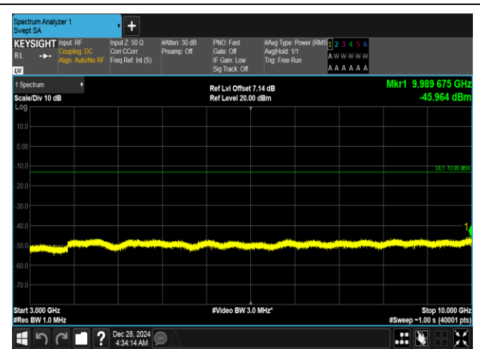
Band26(824-849)-15MHz-16QAM-26965-1RB#0-3000~10000-PASS
