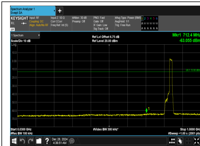
Band26(824-849)-15MHz-QPSK-26965-75RB#0-30~1000-PASS
