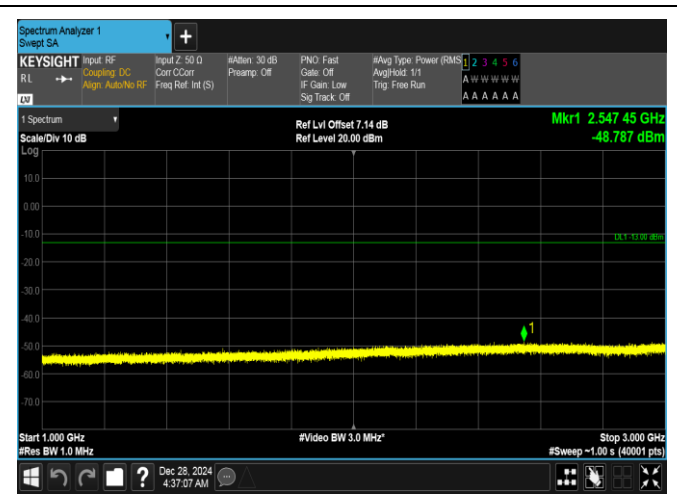
Band26(824-849)-15MHz-QPSK-26965-75RB#0-1000~3000-PASS
