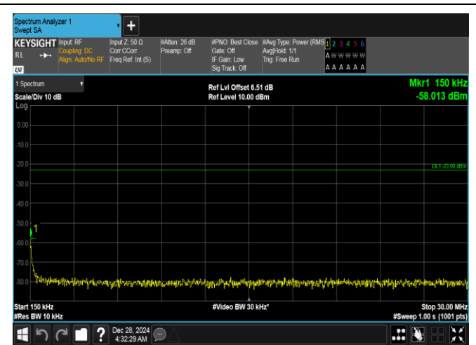
Band26(824-849)-15MHz-QPSK-26965-1RB#0-0.15~30-PASS
