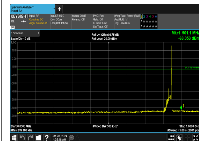
Band26(824-849)-15MHz-16QAM-26965-1RB#74-30~1000-PASS
