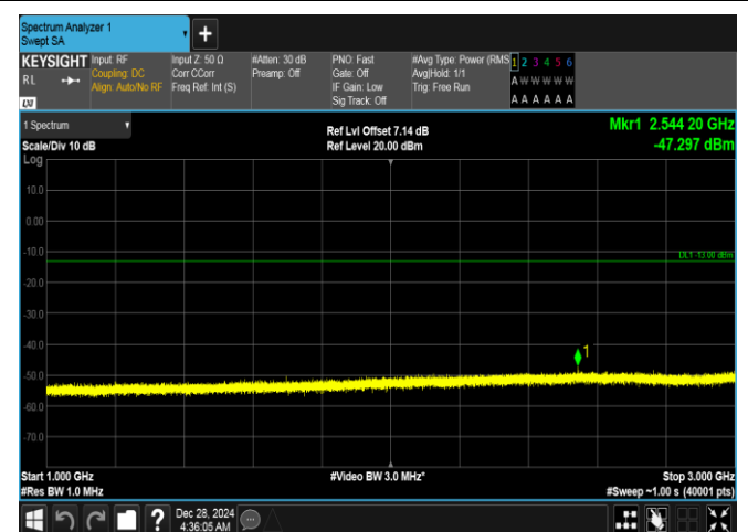
Band26(824-849)-15MHz-16QAM-26965-1RB#74-1000~3000-PASS
