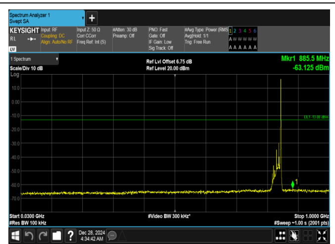
Band26(824-849)-15MHz-QPSK-26965-1RB#74-30~1000-PASS
