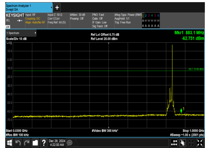
Band26(824-849)-15MHz-QPSK-26865-1RB#74-30~1000-PASS
