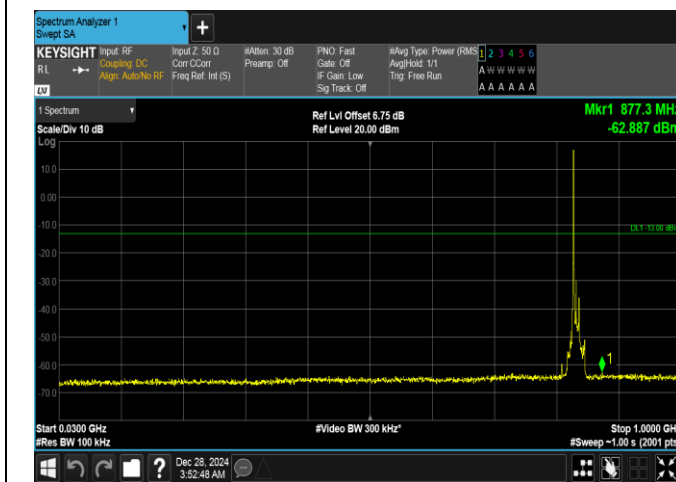
Band26(824-849)-10MHz-16QAM-26915-1RB#0-30~1000-PASS
