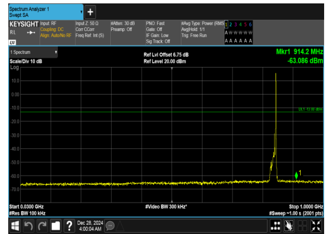
Band26(824-849)-10MHz-QPSK-26990-1RB#49-30~1000-PASS
