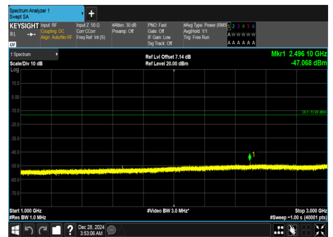
Band26(824-849)-10MHz-16QAM-26915-1RB#0-1000~3000-PASS
