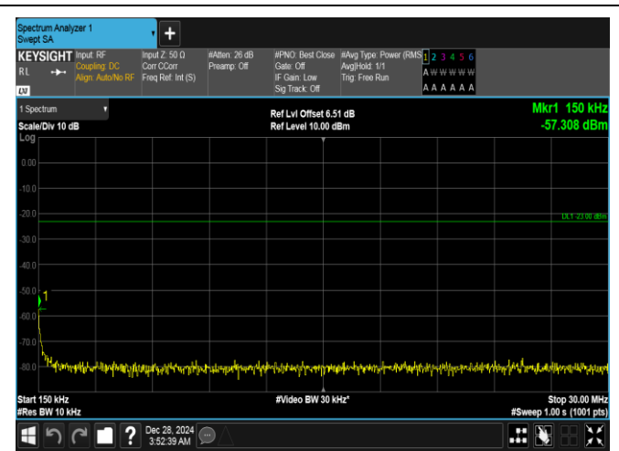
Band26(824-849)-10MHz-16QAM-26915-1RB#0-0.15~30-PASS
