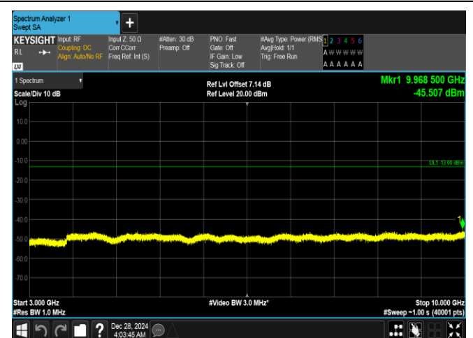
Band26(824-849)-10MHz-16QAM-26990-50RB#0-3000~10000-PASS
