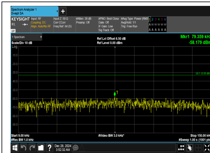
Band26(824-849)-10MHz-16QAM-26915-1RB#0-0.009~0.15-PASS
