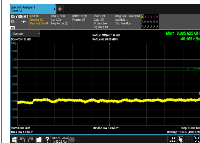
Band26(824-849)-10MHz-16QAM-26915-1RB#0-3000~10000-PASS
