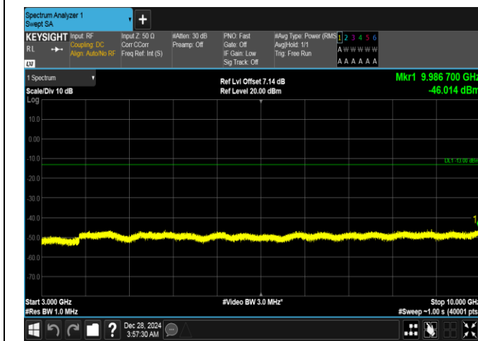
Band26(824-849)-10MHz-16QAM-26915-50RB#0-3000~10000-PASS
