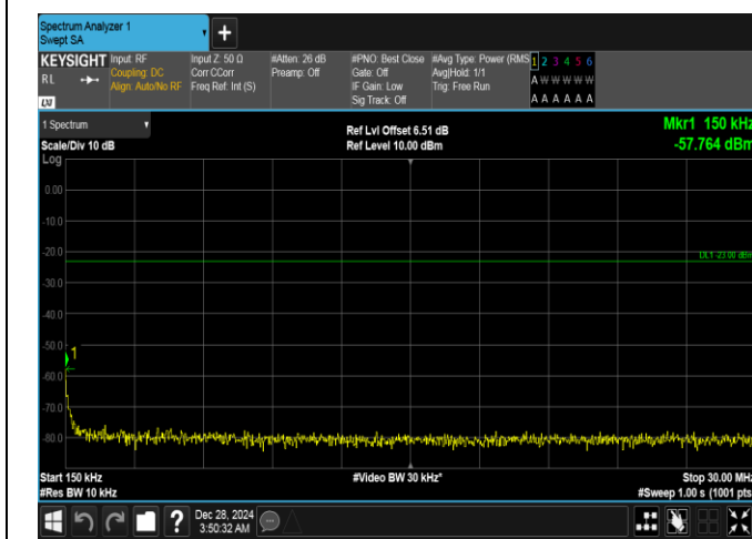
Band26(824-849)-10MHz-16QAM-26840-50RB#0-0.15~30-PASS
