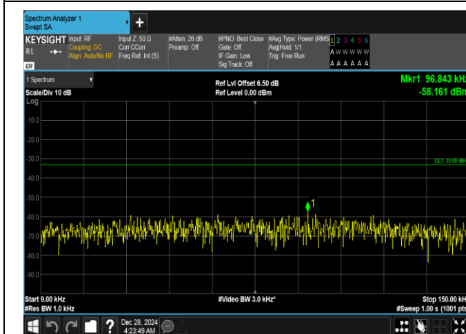
Band26(824-849)-15MHz-QPSK-26865-75RB#0-0.009~0.15-PASS
