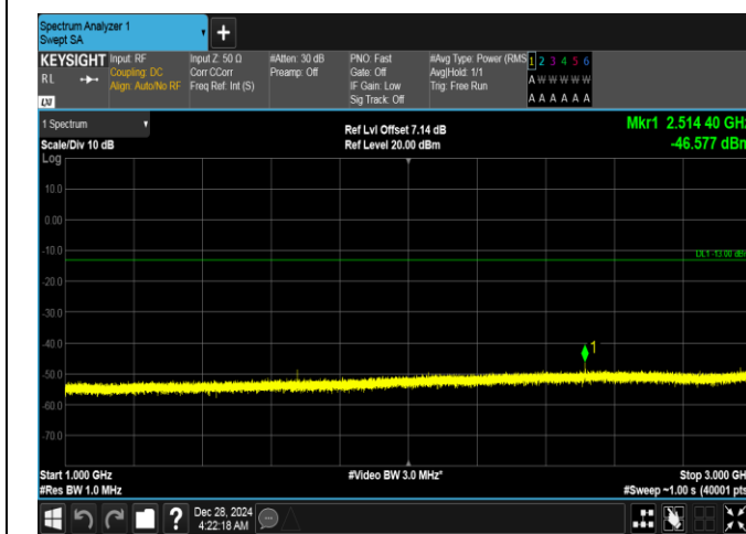
Band26(824-849)-15MHz-QPSK-26865-1RB#74-1000~3000-PASS
