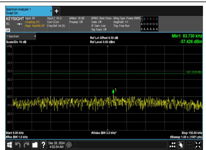
Band26(824-849)-10MHz-16QAM-26990-50RB#0-0.009~0.15-PASS
