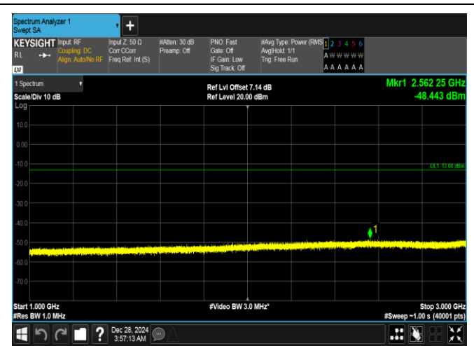
Band26(824-849)-10MHz-16QAM-26915-50RB#0-1000~3000-PASS
