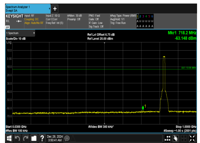
Band26(824-849)-10MHz-16QAM-26840-50RB#0-30~1000-PASS
