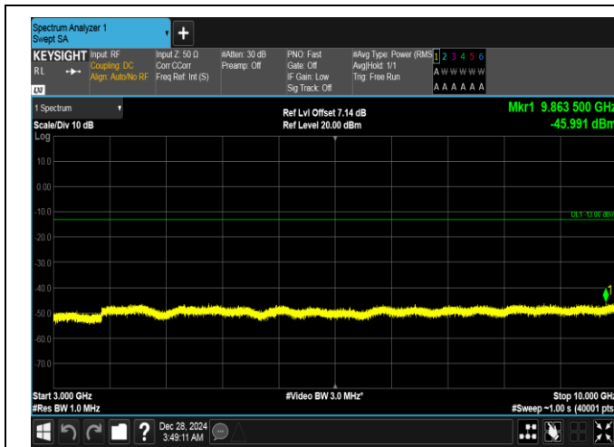
Band26(824-849)-10MHz-16QAM-26840-1RB#49-3000~10000-PASS
