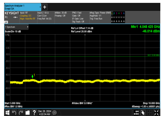
Band26(824-849)-15MHz-QPSK-26865-1RB#74-3000~10000-PASS
