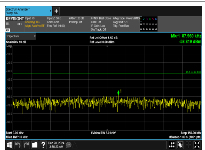
Band26(824-849)-10MHz-16QAM-26840-50RB#0-0.009~0.15-PASS
