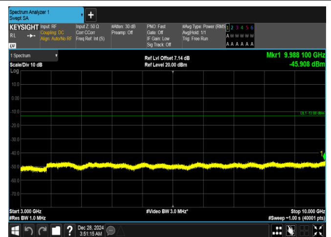
Band26(824-849)-10MHz-16QAM-26840-50RB#0-3000~10000-PASS
