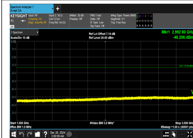
Band26(824-849)-10MHz-16QAM-26840-50RB#0-1000~3000-PASS
