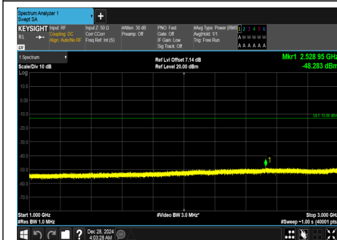
Band26(824-849)-10MHz-16QAM-26990-50RB#0-1000~3000-PASS
