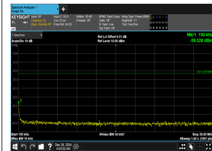
Band26(824-849)-10MHz-16QAM-26990-50RB#0-0.15~30-PASS
