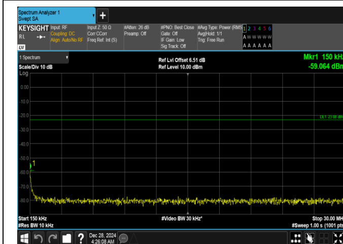
Band26(824-849)-15MHz-QPSK-26915-1RB#0-0.15~30-PASS
