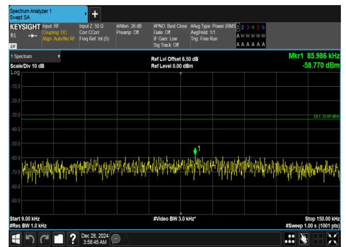
Band26(824-849)-10MHz-16QAM-26990-1RB#0-0.009~0.15-PASS
