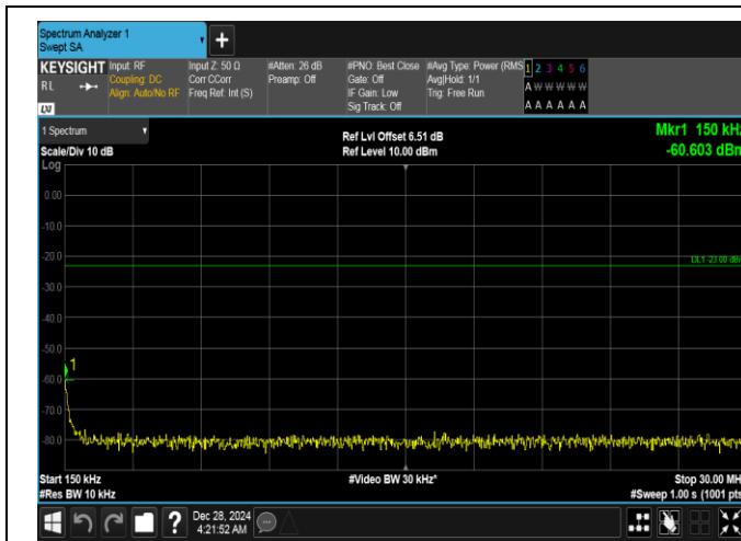
Band26(824-849)-15MHz-QPSK-26865-1RB#74-0.15~30-PASS
