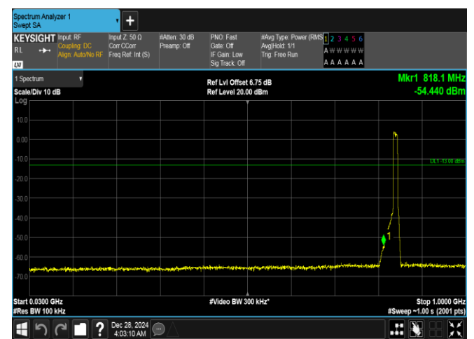
Band26(824-849)-10MHz-16QAM-26990-50RB#0-30~1000-PASS
