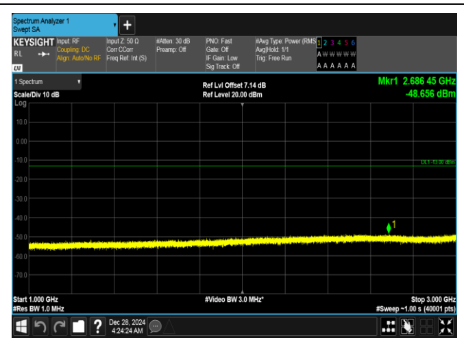
Band26(824-849)-15MHz-QPSK-26865-75RB#0-1000~3000-PASS
