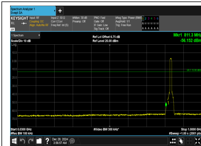
Band26(824-849)-10MHz-16QAM-26915-50RB#0-30~1000-PASS
