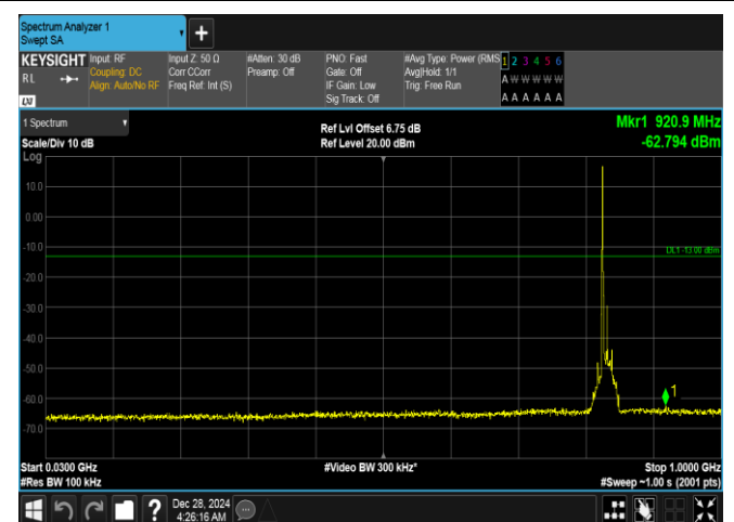
Band26(824-849)-15MHz-QPSK-26915-1RB#0-30~1000-PASS
