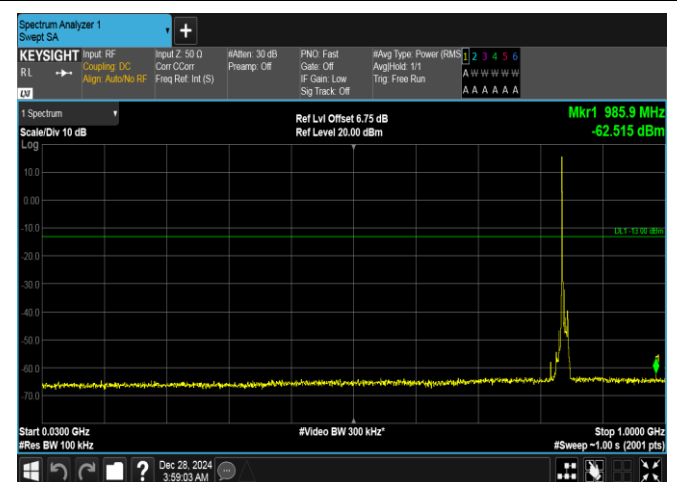
Band26(824-849)-10MHz-16QAM-26990-1RB#0-30~1000-PASS
