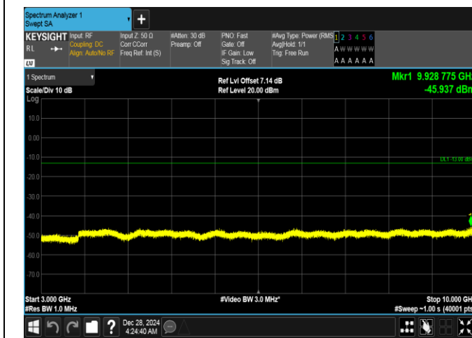
Band26(824-849)-15MHz-QPSK-26865-75RB#0-3000~10000-PASS
