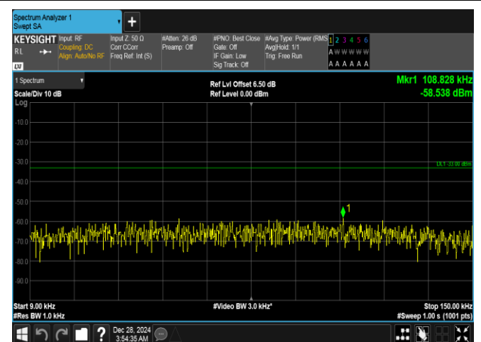
Band26(824-849)-10MHz-16QAM-26915-1RB#49-0.009~0.15-PASS
