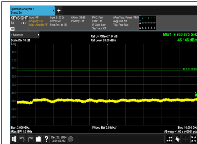
Band26(824-849)-10MHz-16QAM-26990-1RB#49-3000~10000-PASS
