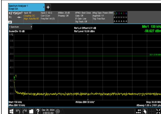
Band26(824-849)-10MHz-16QAM-26990-1RB#0-0.15~30-PASS
