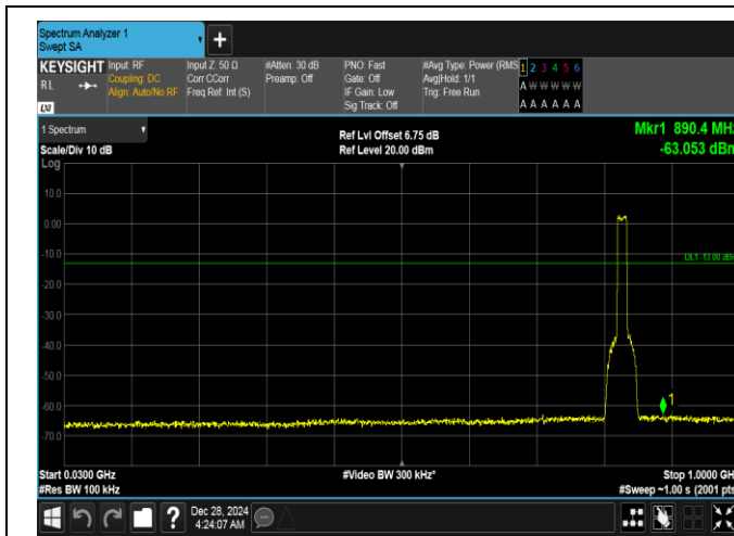
Band26(824-849)-15MHz-QPSK-26865-75RB#0-30~1000-PASS
