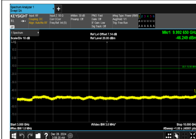
Band26(824-849)-10MHz-QPSK-26990-1RB#0-3000~10000-PASS
