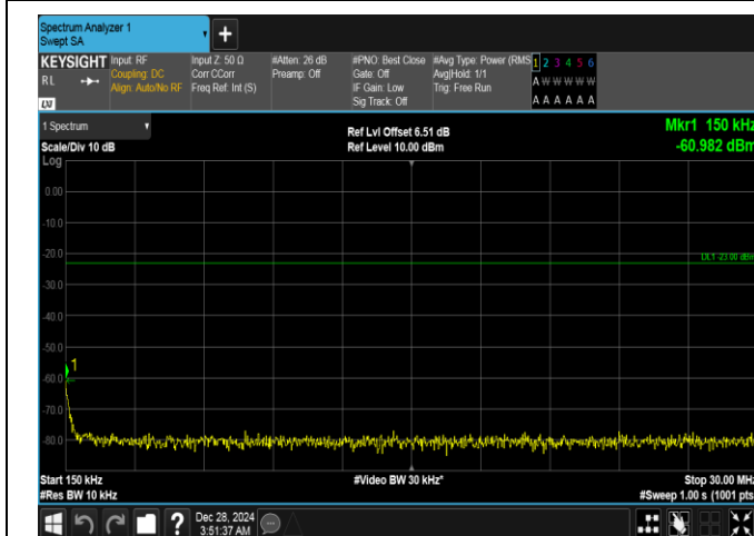
Band26(824-849)-10MHz-QPSK-26915-1RB#0-0.15~30-PASS
