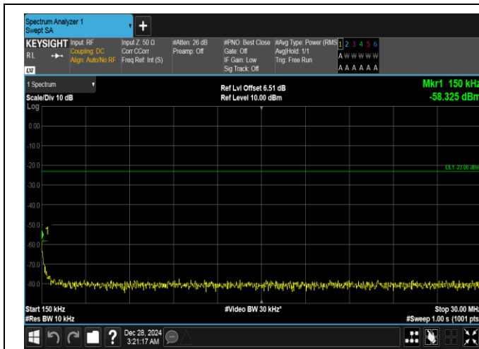
Band26(824-849)-5MHz-16QAM-26915-1RB#24-0.15~30-PASS
