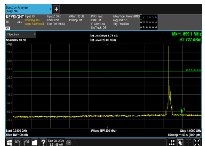
Band26(824-849)-10MHz-QPSK-26915-1RB#0-30~1000-PASS
