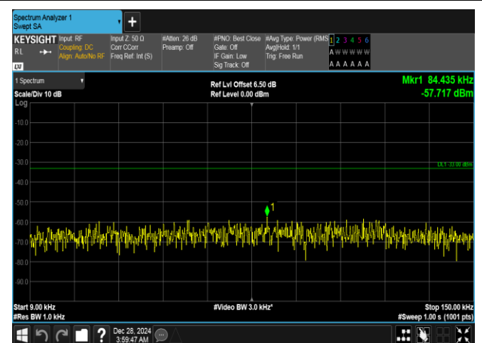
Band26(824-849)-10MHz-QPSK-26990-1RB#49-0.009~0.15-PASS
