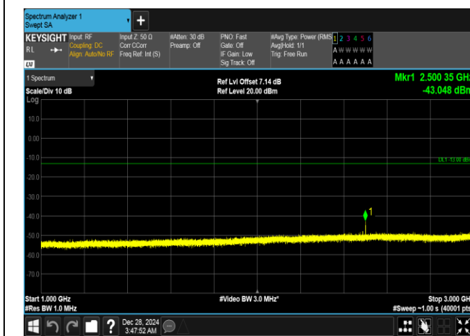
Band26(824-849)-10MHz-QPSK-26840-1RB#49-1000~3000-PASS
