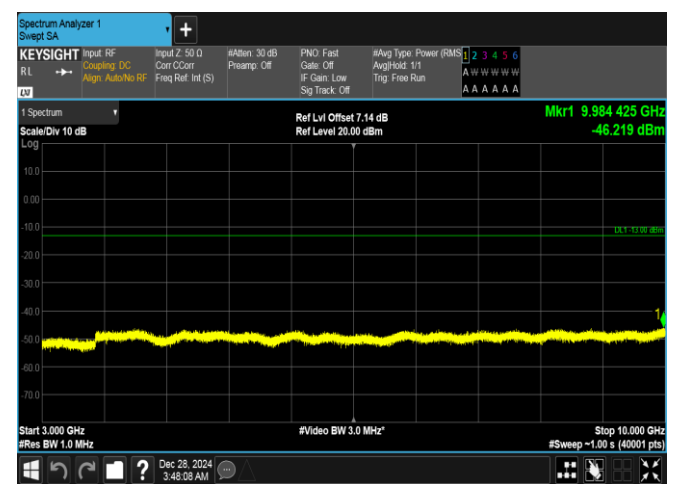
Band26(824-849)-10MHz-QPSK-26840-1RB#49-3000~10000-PASS
