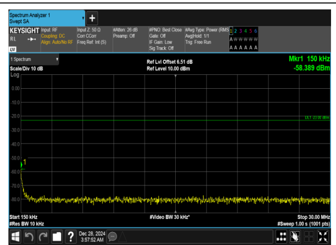
Band26(824-849)-10MHz-QPSK-26990-1RB#0-0.15~30-PASS
