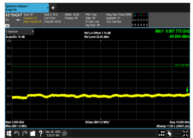
Band26(824-849)-5MHz-16QAM-26915-1RB#24-3000~10000-PASS
