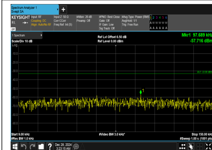
Band26(824-849)-5MHz-16QAM-26915-25RB#0-0.009~0.15-PASS
