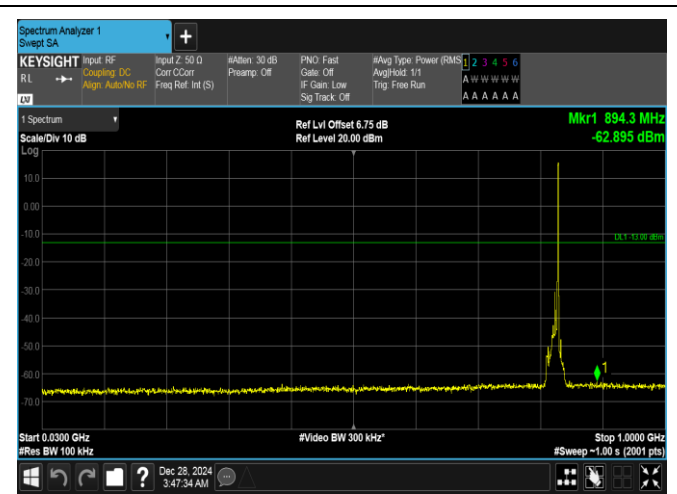
Band26(824-849)-10MHz-QPSK-26840-1RB#49-30~1000-PASS
