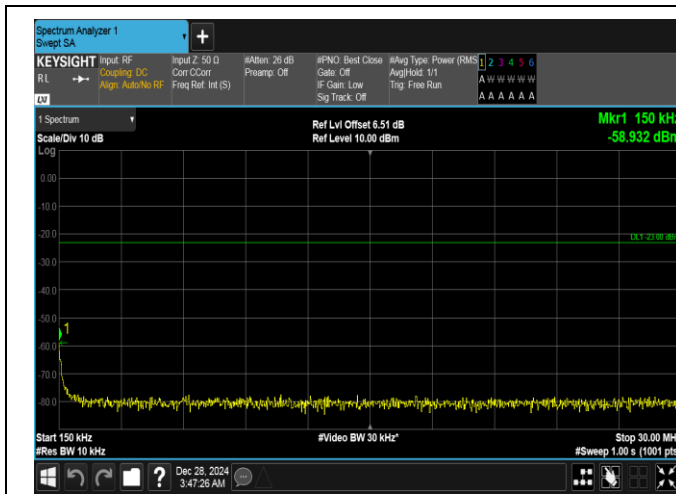
Band26(824-849)-10MHz-QPSK-26840-1RB#49-0.15~30-PASS
