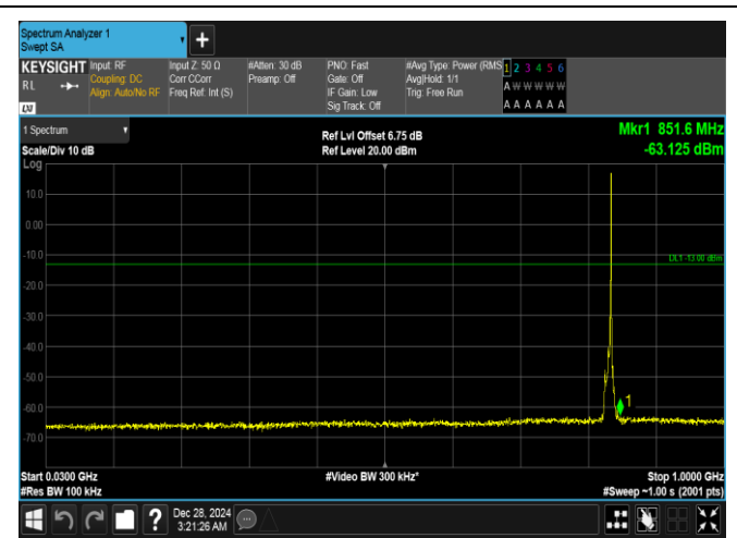
Band26(824-849)-5MHz-16QAM-26915-1RB#24-30~1000-PASS
