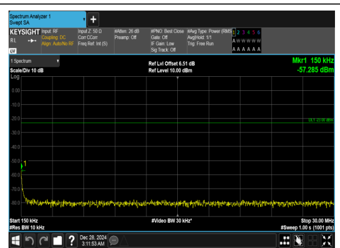
Band26(824-849)-5MHz-QPSK-26815-1RB#0-0.15~30-PASS
