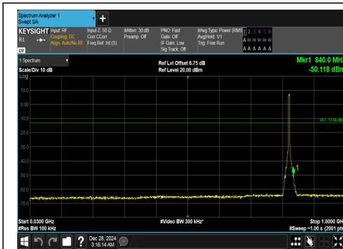
Band26(824-849)-5MHz-QPSK-26815-25RB#0-30~1000-PASS
