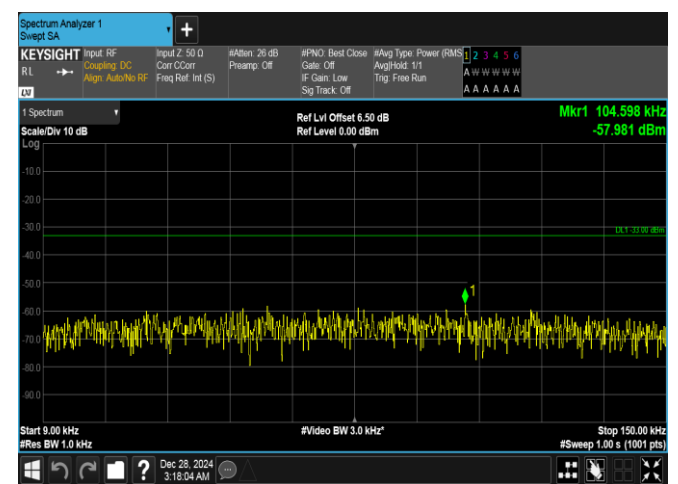
Band26(824-849)-5MHz-QPSK-26915-1RB#0-0.009~0.15-PASS
