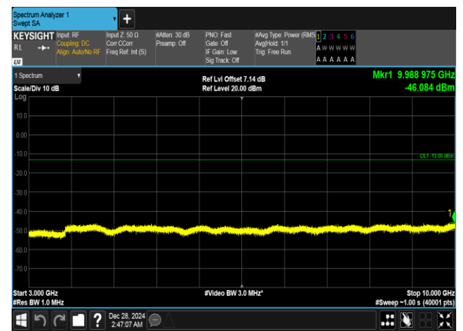
Band26(824-849)-3MHz-16QAM-26915-1RB#14-3000~10000-PASS
