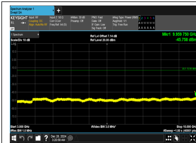
Band26(824-849)-5MHz-QPSK-26915-1RB#24-3000~10000-PASS
