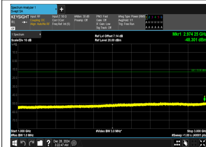
Band26(824-849)-5MHz-QPSK-26915-25RB#0-1000~3000-PASS
