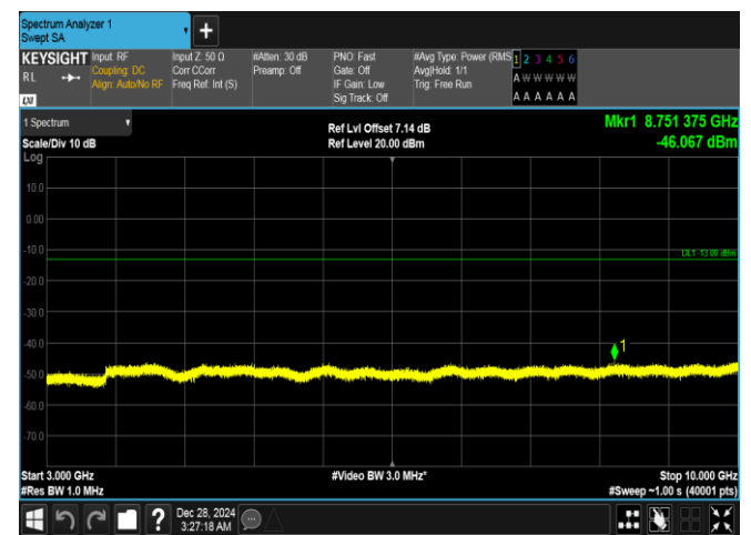
Band26(824-849)-5MHz-QPSK-27015-1RB#24-3000~10000-PASS
