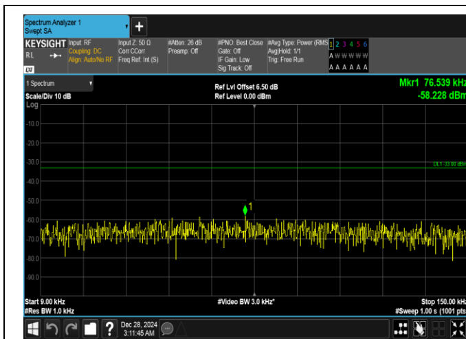
Band26(824-849)-5MHz-QPSK-26815-1RB#0-0.009~0.15-PASS
