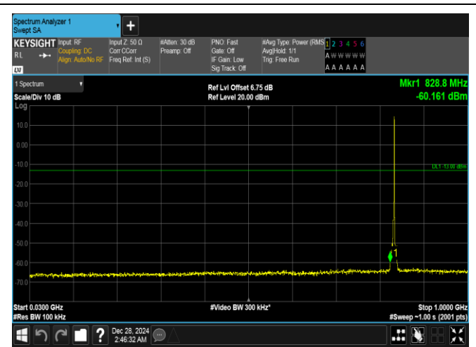
Band26(824-849)-3MHz-16QAM-26915-1RB#14-30~1000-PASS
