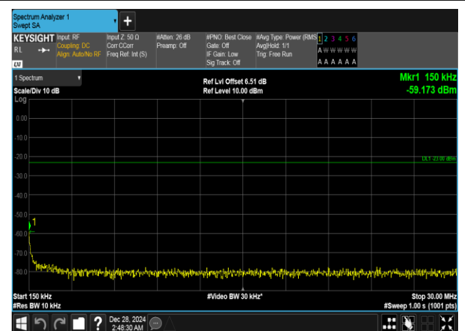
Band26(824-849)-3MHz-16QAM-26915-15RB#0-0.15~30-PASS
