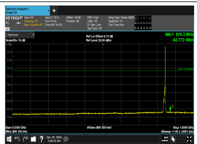
Band26(824-849)-5MHz-QPSK-27015-1RB#24-30~1000-PASS
