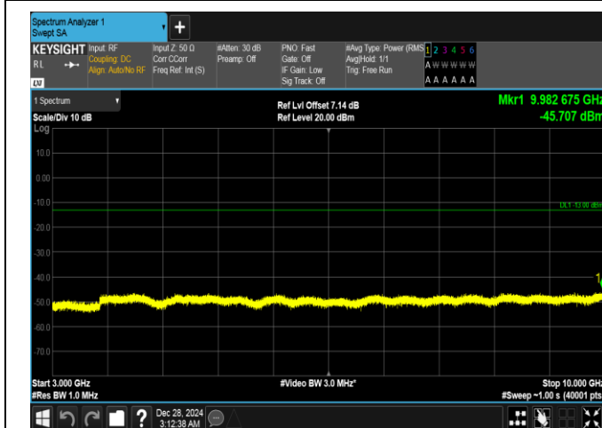
Band26(824-849)-5MHz-QPSK-26815-1RB#0-3000~10000-PASS
