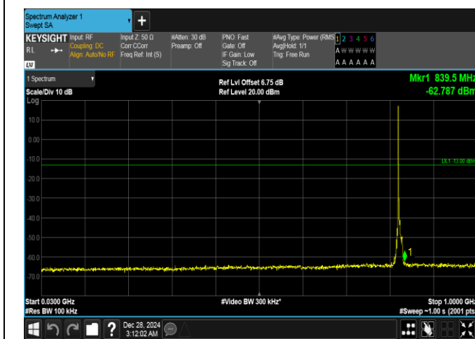
Band26(824-849)-5MHz-QPSK-26815-1RB#0-30~1000-PASS
