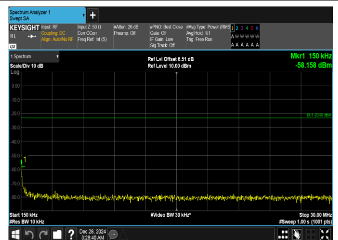
Band26(824-849)-5MHz-QPSK-27015-25RB#0-0.15~30-PASS
