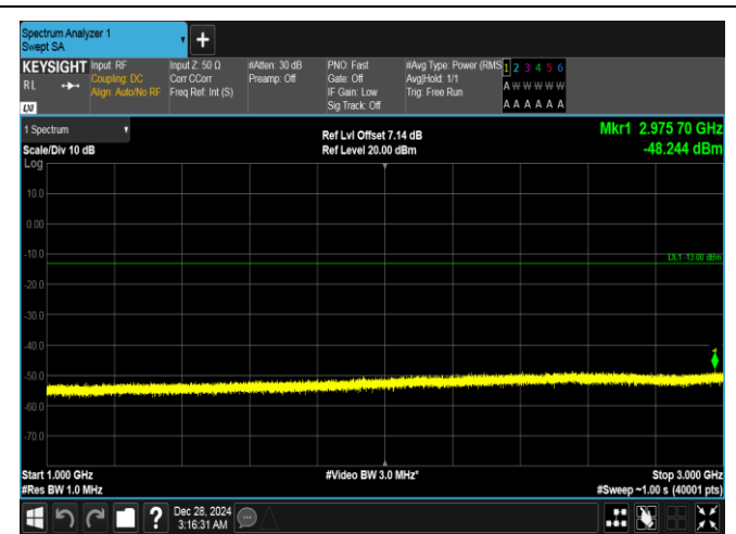
Band26(824-849)-5MHz-QPSK-26815-25RB#0-1000~3000-PASS
