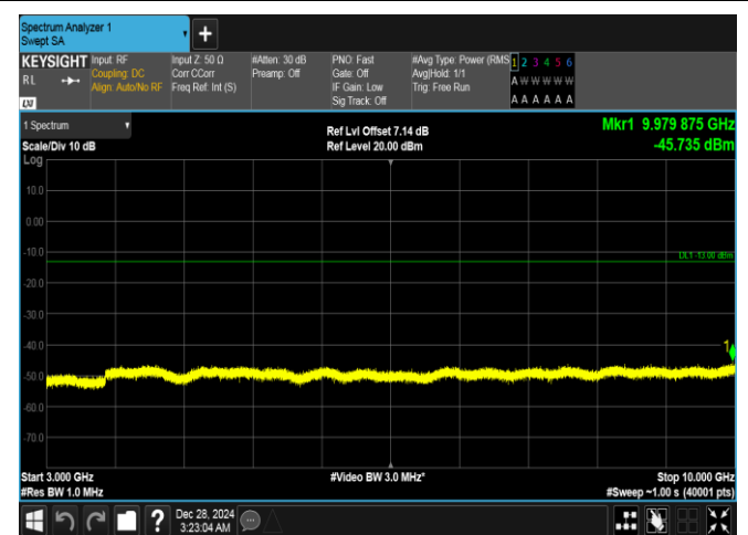
Band26(824-849)-5MHz-QPSK-26915-25RB#0-3000~10000-PASS
