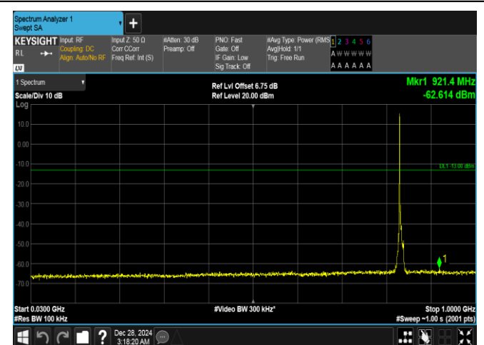
Band26(824-849)-5MHz-QPSK-26915-1RB#0-30~1000-PASS
