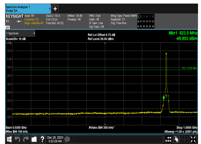
Band26(824-849)-5MHz-QPSK-26915-25RB#0-30~1000-PASS
