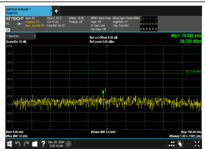
Band26(824-849)-5MHz-QPSK-26915-25RB#0-0.009~0.15-PASS
