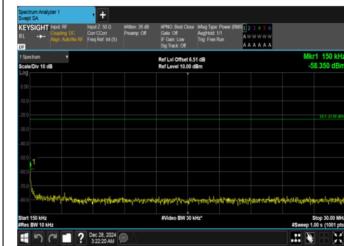
Band26(824-849)-5MHz-QPSK-26915-25RB#0-0.15~30-PASS
