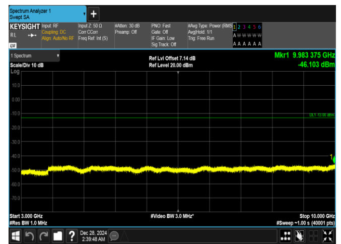
Band26(824-849)-3MHz-QPSK-26805-1RB#14-3000~10000-PASS
