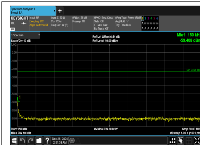
Band26(824-849)-3MHz-QPSK-27025-1RB#14-0.15~30-PASS
