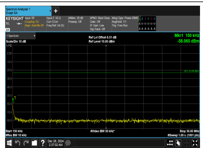
Band26(824-849)-3MHz-QPSK-26805-1RB#0-0.15~30-PASS
