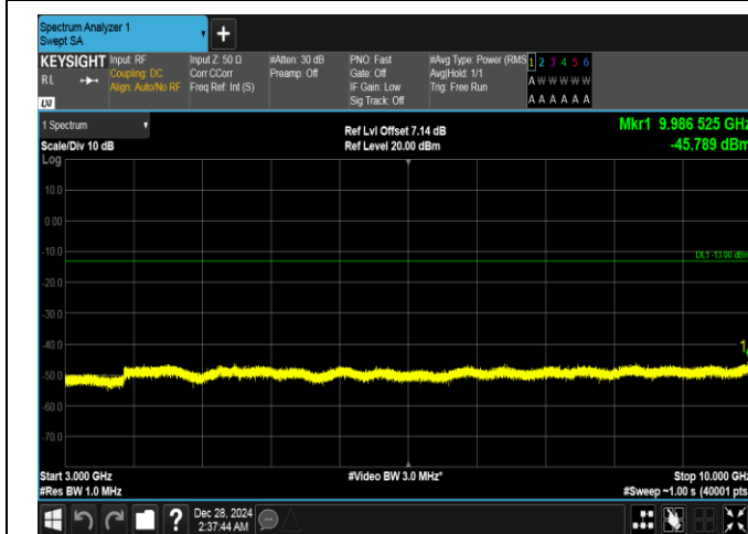
Band26(824-849)-3MHz-QPSK-26805-1RB#0-3000~10000-PASS
