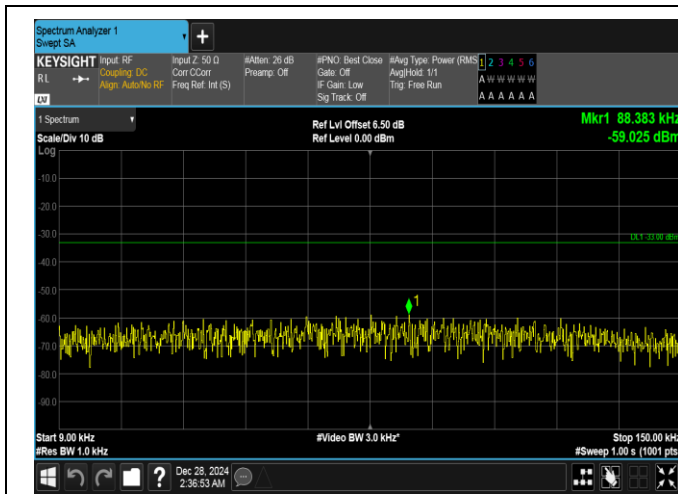
Band26(824-849)-3MHz-QPSK-26805-1RB#0-0.009~0.15-PASS
