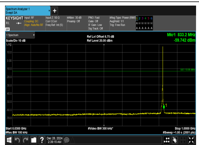
Band26(824-849)-3MHz-QPSK-26805-1RB#14-30~1000-PASS
