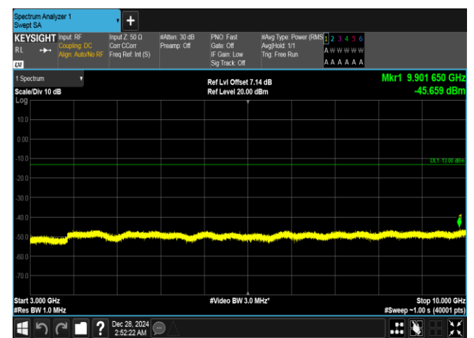
Band26(824-849)-3MHz-QPSK-27025-1RB#14-3000~10000-PASS
