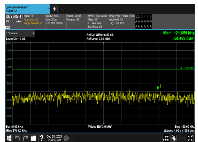
Band26(824-849)-3MHz-QPSK-26805-1RB#14-0.009~0.15-PASS
