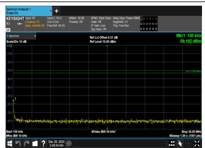
Band26(824-849)-3MHz-QPSK-27025-1RB#0-0.15~30-PASS
