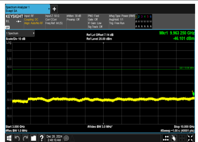
Band26(824-849)-3MHz-QPSK-26915-15RB#0-3000~10000-PASS
