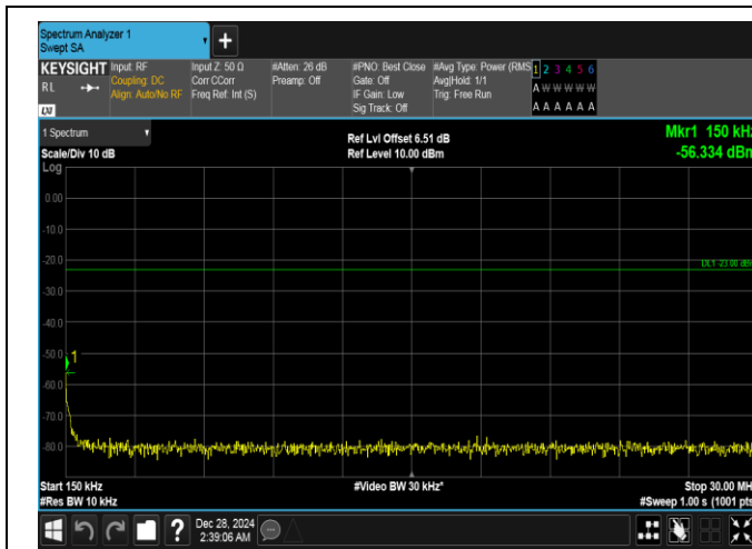
Band26(824-849)-3MHz-QPSK-26805-1RB#14-0.15~30-PASS
