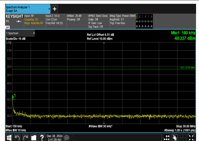
Band26(824-849)-3MHz-QPSK-26805-15RB#0-0.15~30-PASS
