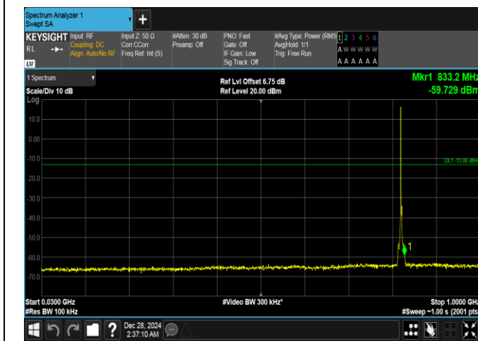
Band26(824-849)-3MHz-QPSK-26805-1RB#0-30~1000-PASS
