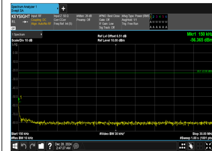
Band26(824-849)-3MHz-QPSK-26915-15RB#0-0.15~30-PASS
