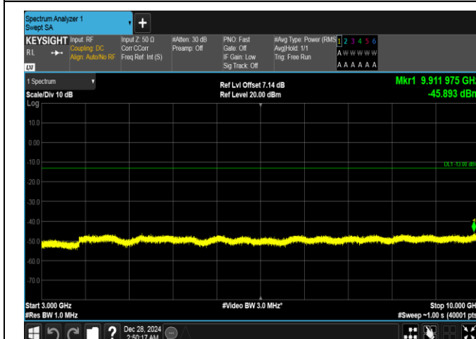
Band26(824-849)-3MHz-QPSK-27025-1RB#0-3000~10000-PASS
