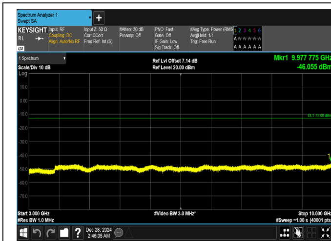
Band26(824-849)-3MHz-QPSK-26915-1RB#14-3000~10000-PASS
