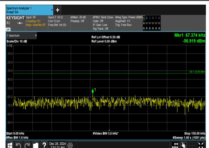
Band26(824-849)-3MHz-QPSK-27025-1RB#14-0.009~0.15-PASS
