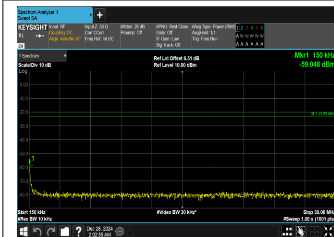
Band26(824-849)-1.4MHz-16QAM-26797-1RB#0-0.15~30-PASS
