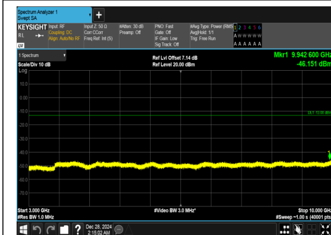
Band26(824-849)-1.4MHz-QPSK-27033-1RB#0-3000~10000-PASS
