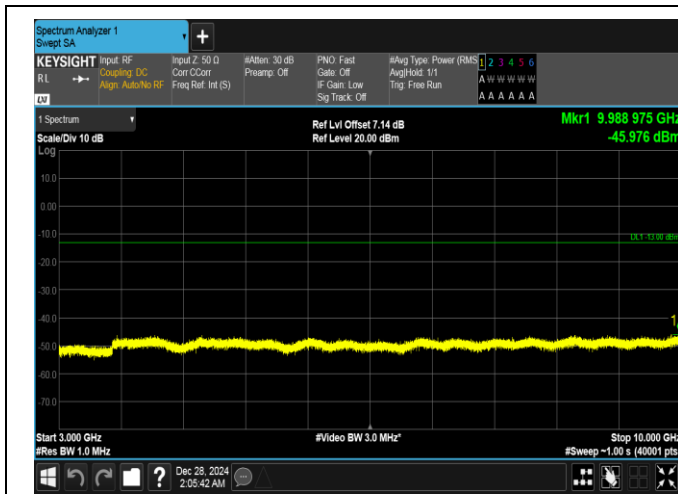
Band26(824-849)-1.4MHz-16QAM-26797-1RB#5-3000~10000-PASS
