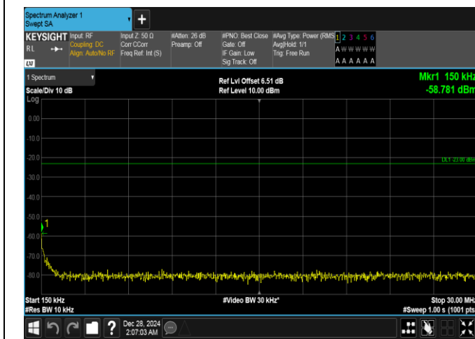
Band26(824-849)-1.4MHz-16QAM-26797-6RB#0-0.15~30-PASS
