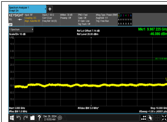
Band26(824-849)-1.4MHz-QPSK-26915-1RB#5-3000~10000-PASS
