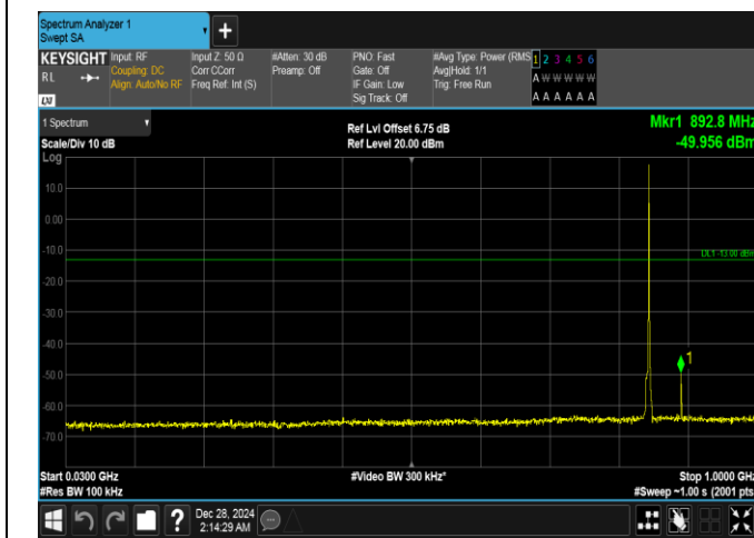
Band26(824-849)-1.4MHz-QPSK-27033-1RB#0-30~1000-PASS
