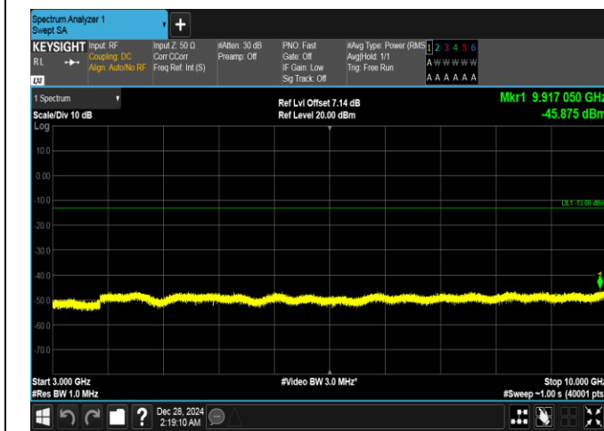
Band26(824-849)-1.4MHz-QPSK-27033-6RB#0-3000~10000-PASS
