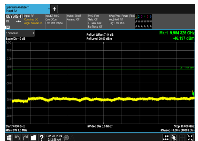
Band26(824-849)-1.4MHz-QPSK-26915-6RB#0-3000~10000-PASS
