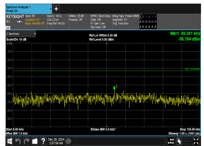
Band26(824-849)-1.4MHz-QPSK-26915-1RB#0-0.009~0.15-PASS
