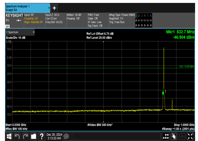
Band26(824-849)-1.4MHz-QPSK-26915-6RB#0-30~1000-PASS
