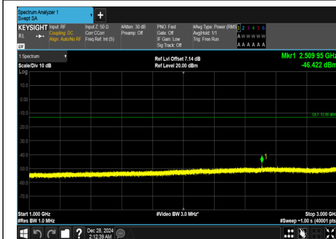
Band26(824-849)-1.4MHz-QPSK-26915-6RB#0-1000~3000-PASS
