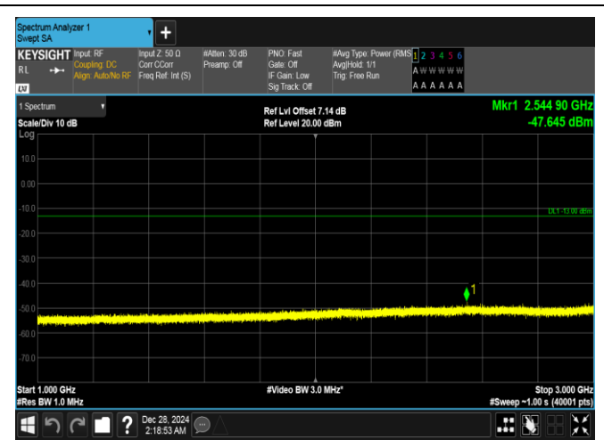
Band26(824-849)-1.4MHz-QPSK-27033-6RB#0-1000~3000-PASS
