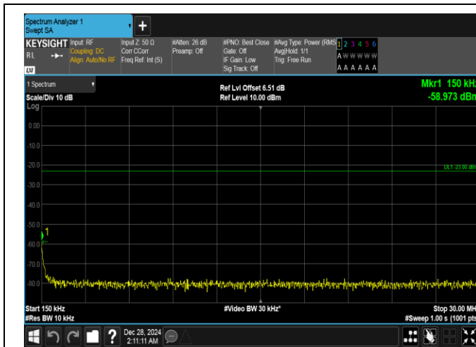
Band26(824-849)-1.4MHz-16QAM-26915-1RB#5-0.15~30-PASS
