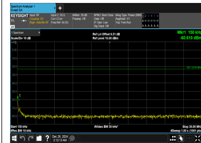
Band26(824-849)-1.4MHz-QPSK-26915-6RB#0-0.15~30-PASS
