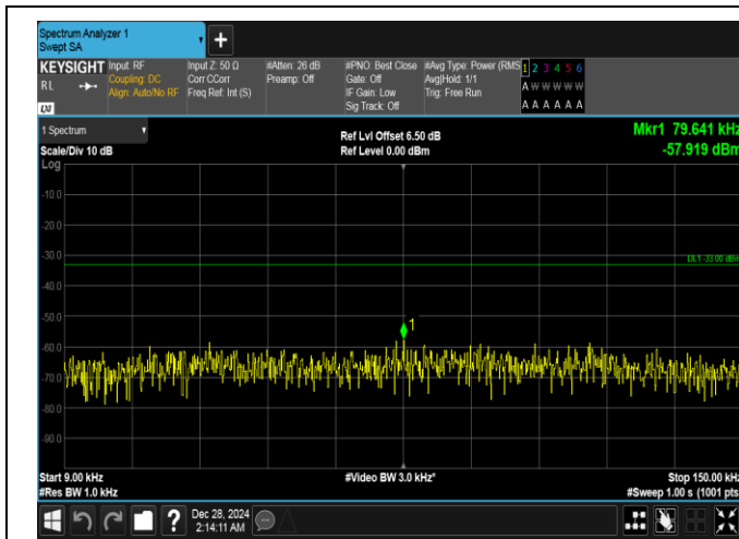
Band26(824-849)-1.4MHz-QPSK-27033-1RB#0-0.009~0.15-PASS
