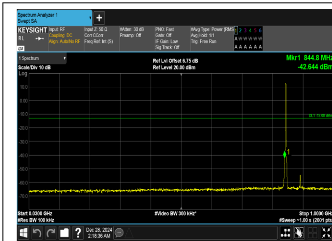
Band26(824-849)-1.4MHz-QPSK-27033-6RB#0-30~1000-PASS
