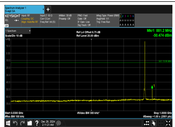
Band26(824-849)-1.4MHz-16QAM-26915-1RB#5-30~1000-PASS
