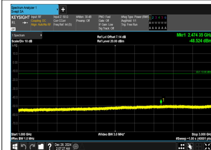
Band26(824-849)-1.4MHz-16QAM-26797-6RB#0-1000~3000-PASS
