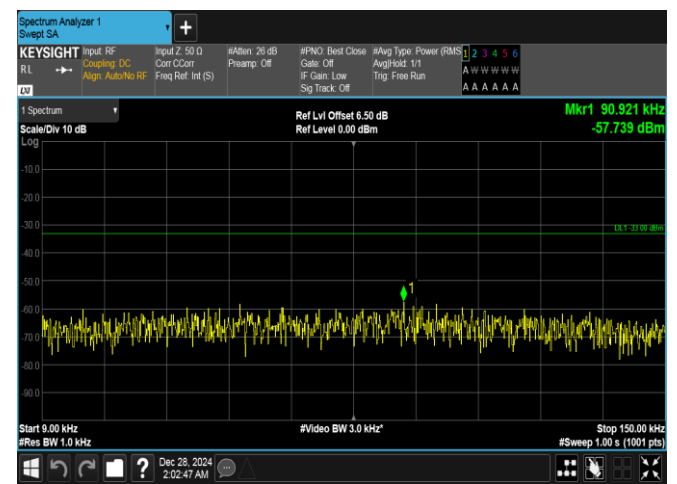
Band26(824-849)-1.4MHz-16QAM-26797-1RB#0-0.009~0.15-PASS
