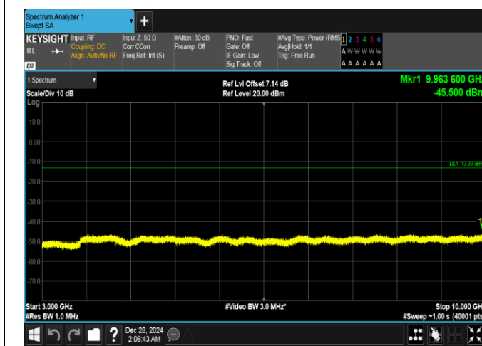
Band26(824-849)-1.4MHz-QPSK-26797-6RB#0-3000~10000-PASS
