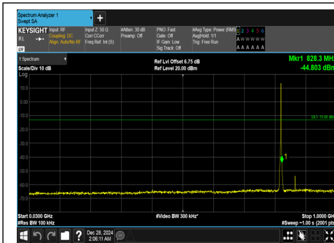
Band26(824-849)-1.4MHz-QPSK-26797-6RB#0-30~1000-PASS
