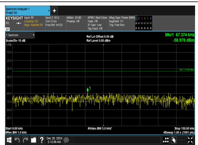
Band26(824-849)-1.4MHz-QPSK-26915-6RB#0-0.009~0.15-PASS
