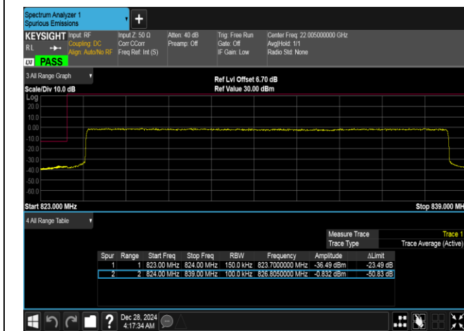
Band26(824-849)-15MHz-QPSK-26865-75RB#0-PASS
