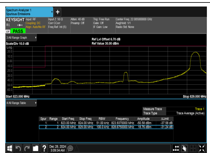
Band26(824-849)-5MHz-16QAM-26815-1RB#24-PASS
