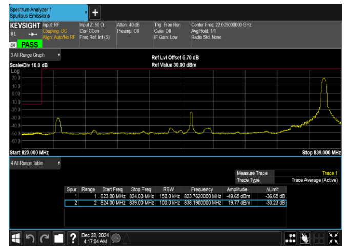
Band26(824-849)-15MHz-QPSK-26865-1RB#74-PASS
