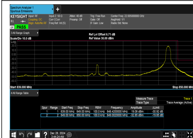
Band26(824-849)-10MHz-16QAM-26990-1RB#49-PASS
