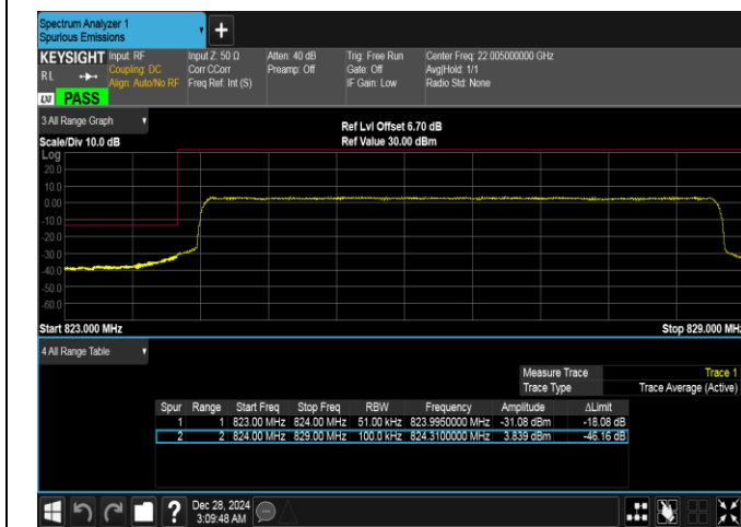
Band26(824-849)-5MHz-QPSK-26815-25RB#0-PASS
