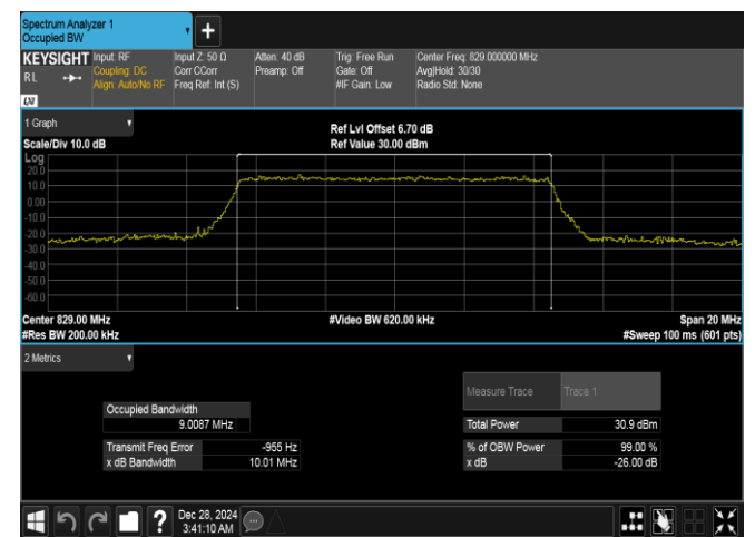
Band26(824-849)-10MHz-16QAM-26840-50RB#0-PASS
