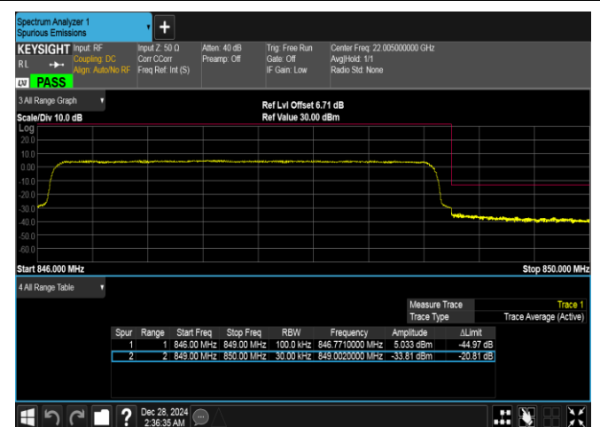
Band26(824-849)-3MHz-16QAM-27025-15RB#0-PASS
