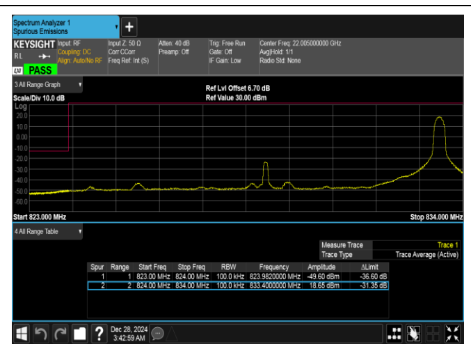
Band26(824-849)-10MHz-16QAM-26840-1RB#49-PASS
