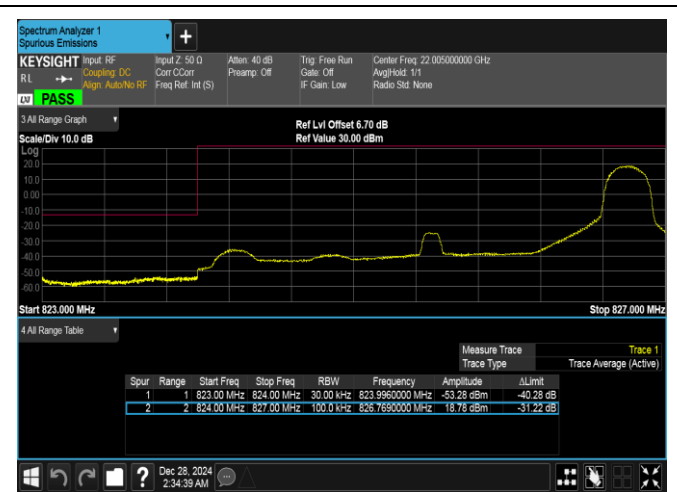
Band26(824-849)-3MHz-16QAM-26805-1RB#14-PASS
