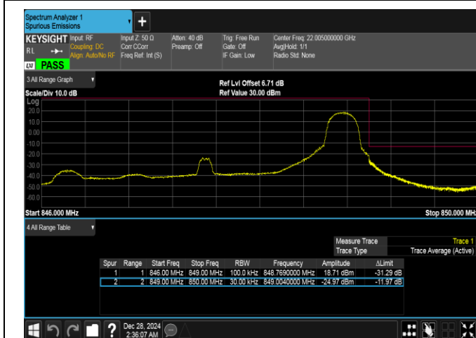
Band26(824-849)-3MHz-16QAM-27025-1RB#14-PASS
