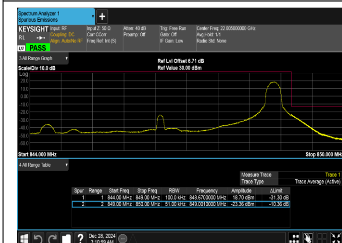
Band26(824-849)-5MHz-16QAM-27015-1RB#24-PASS
