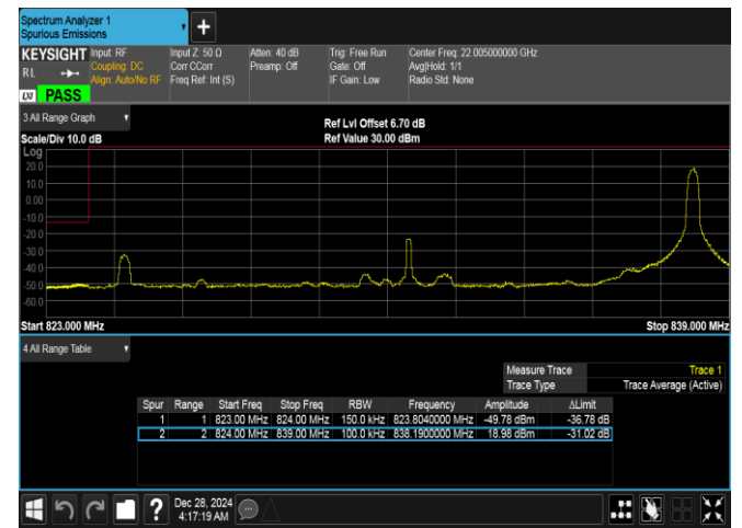
Band26(824-849)-15MHz-16QAM-26865-1RB#74-PASS
