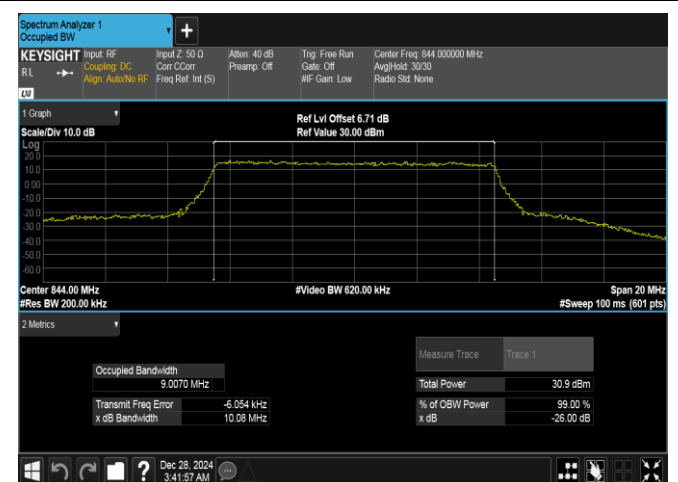
Band26(824-849)-10MHz-16QAM-26990-50RB#0-PASS
