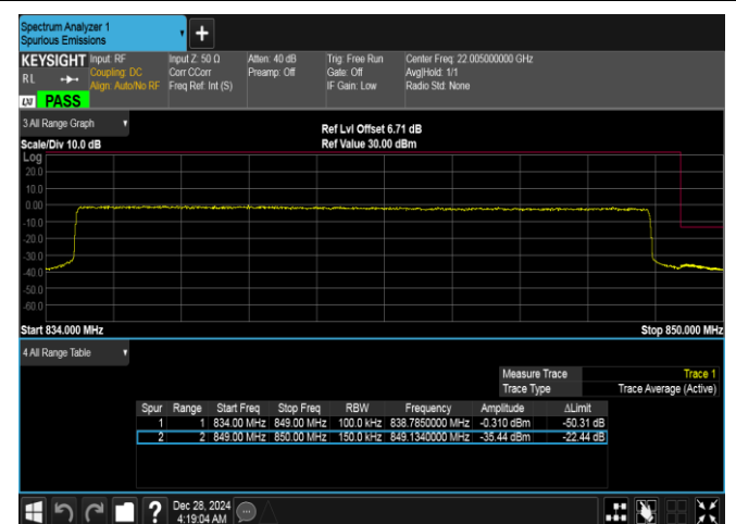
Band26(824-849)-15MHz-QPSK-26965-75RB#0-PASS
