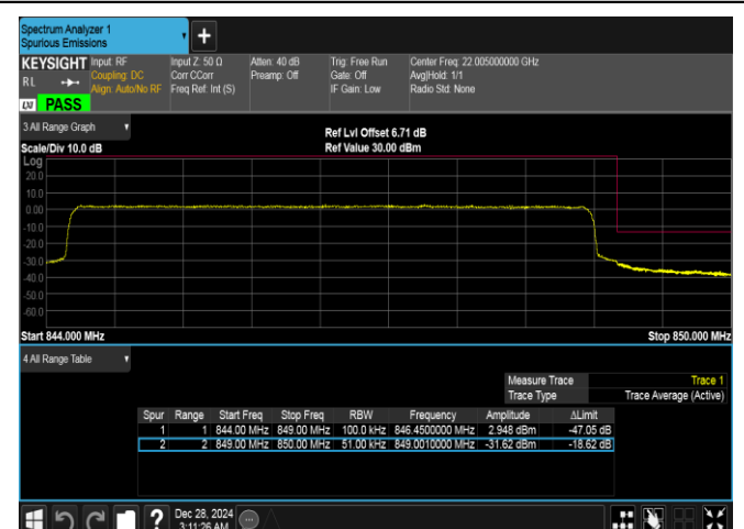
Band26(824-849)-5MHz-16QAM-27015-25RB#0-PASS
