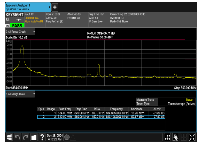
Band26(824-849)-15MHz-16QAM-26965-1RB#0-PASS
