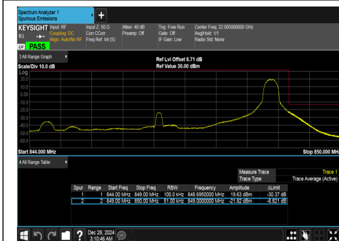
Band26(824-849)-5MHz-QPSK-27015-1RB#24-PASS
