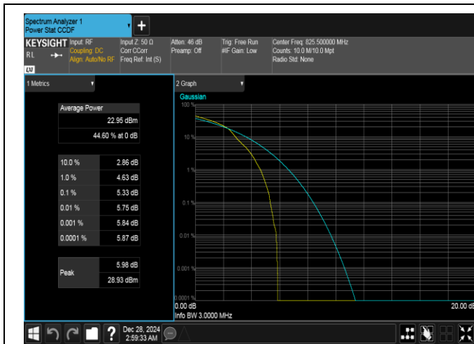
Band26(824-849)-3MHz-16QAM-26805-1RB#0-PASS
