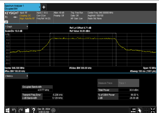
Band26(824-849)-5MHz-16QAM-27015-25RB#0-PASS
