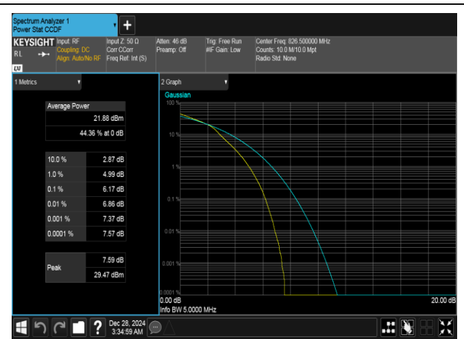
Band26(824-849)-5MHz-16QAM-26815-25RB#0-PASS
