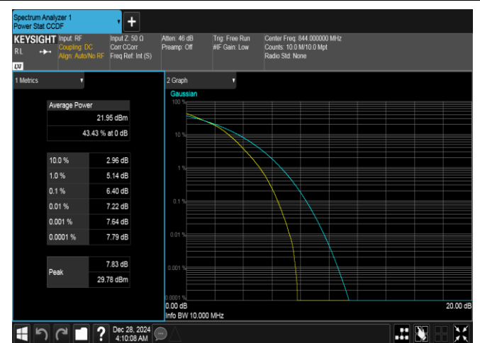
Band26(824-849)-10MHz-16QAM-26990-50RB#0-PASS
