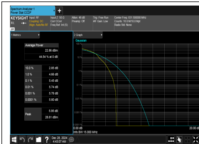
Band26(824-849)-15MHz-16QAM-26865-1RB#0-PASS
