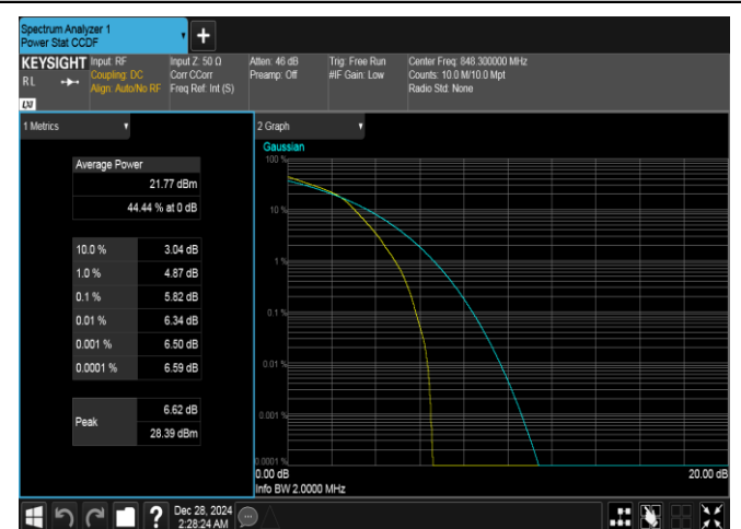
Band26(824-849)-1.4MHz-16QAM-27033-6RB#0-PASS
