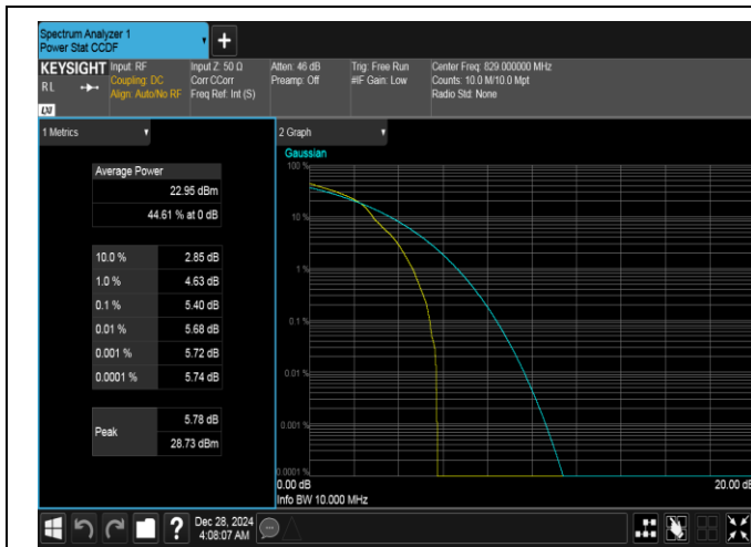
Band26(824-849)-10MHz-16QAM-26840-1RB#0-PASS
