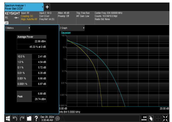
Band26(824-849)-5MHz-QPSK-26915-25RB#0-PASS
