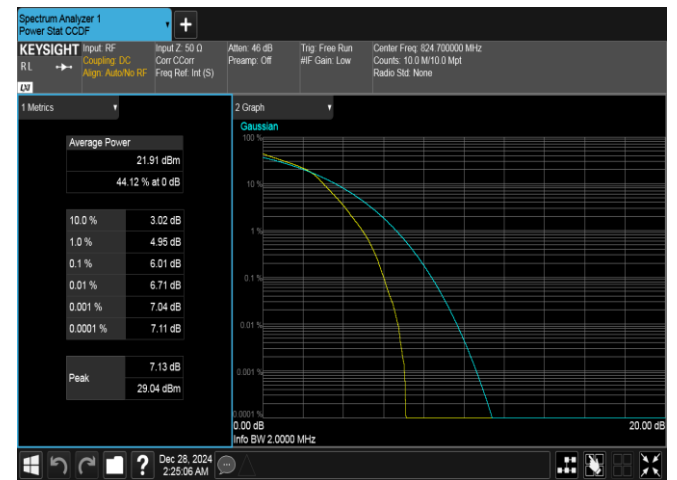
Band26(824-849)-1.4MHz-16QAM-26797-6RB#0-PASS
