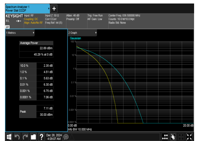
Band26(824-849)-10MHz-QPSK-26915-50RB#0-PASS
