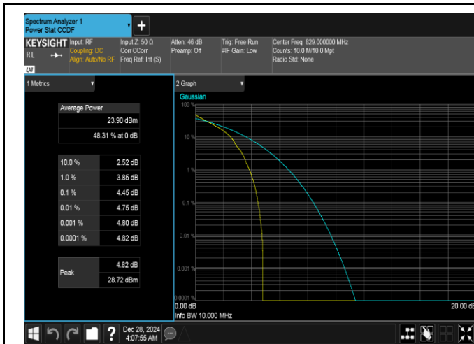
Band26(824-849)-10MHz-QPSK-26840-1RB#0-PASS
