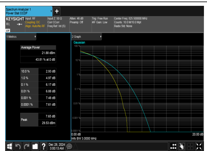
Band26(824-849)-3MHz-16QAM-26805-15RB#0-PASS
