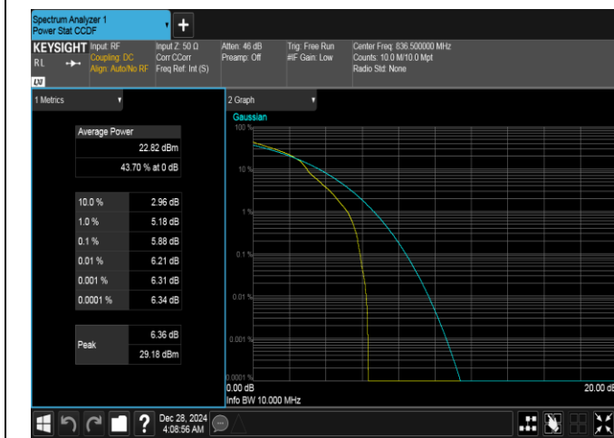
Band26(824-849)-10MHz-16QAM-26915-1RB#0-PASS
