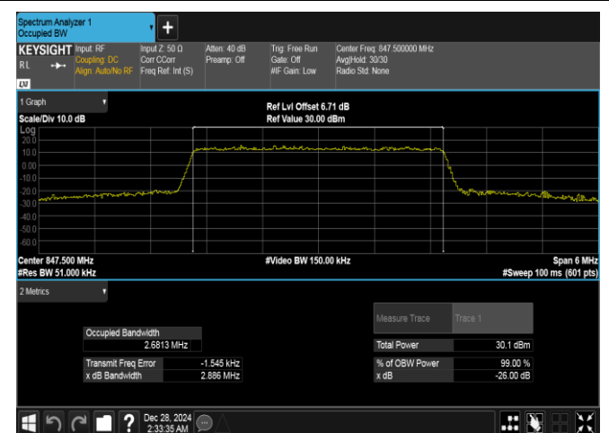
Band26(824-849)-3MHz-16QAM-27025-15RB#0-PASS
