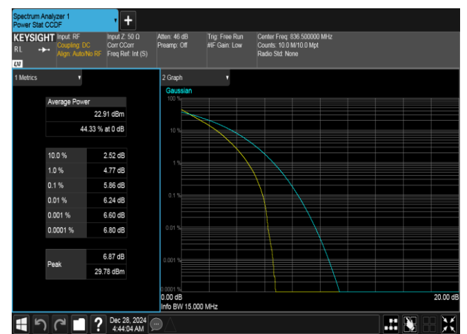
Band26(824-849)-15MHz-QPSK-26915-75RB#0-PASS
