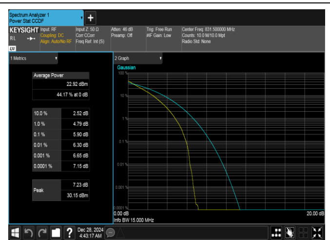
Band26(824-849)-15MHz-QPSK-26865-75RB#0-PASS
