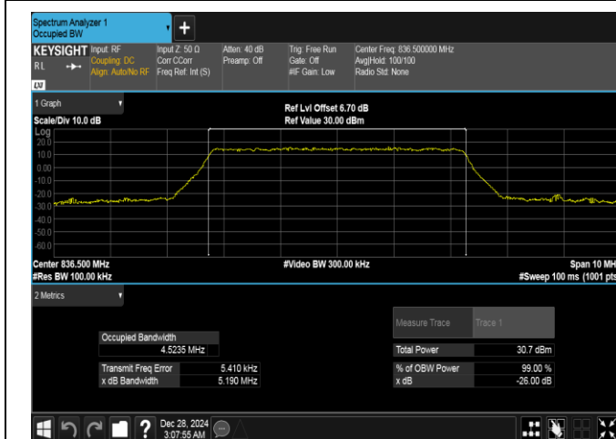
Band26(824-849)-5MHz-16QAM-26915-25RB#0-PASS
