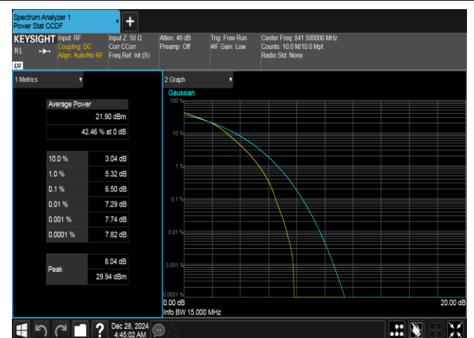
Band26(824-849)-15MHz-16QAM-26965-75RB#0-PASS
