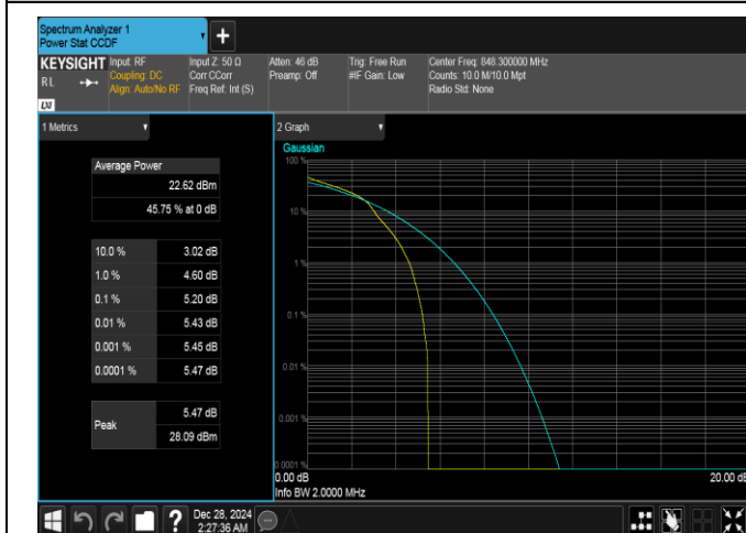
Band26(824-849)-1.4MHz-16QAM-27033-1RB#0-PASS
