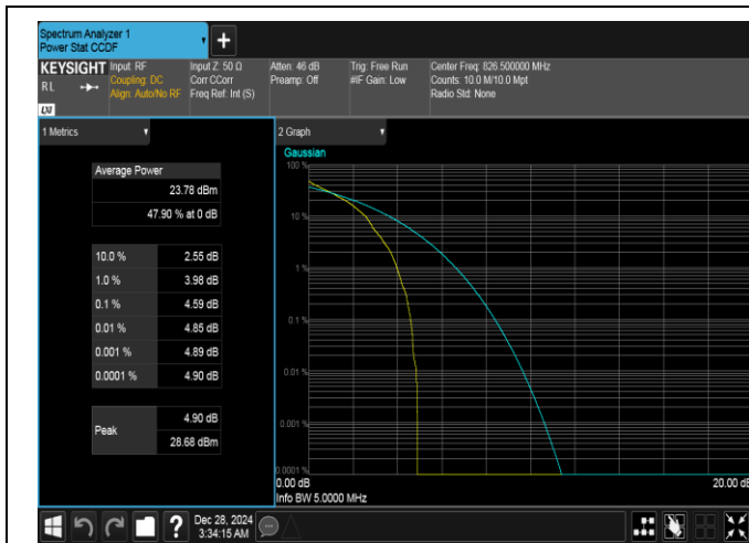
Band26(824-849)-5MHz-QPSK-26815-1RB#0-PASS
