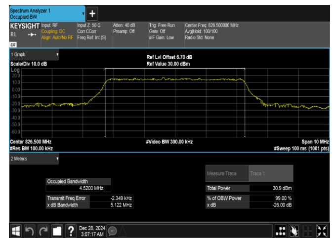
Band26(824-849)-5MHz-16QAM-26815-25RB#0-PASS
