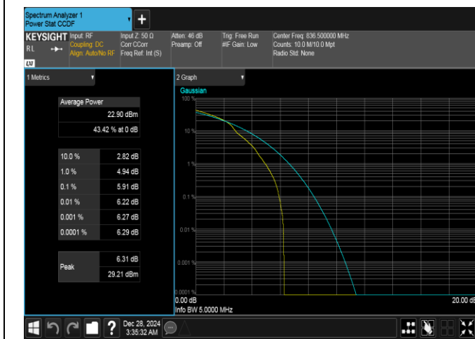
Band26(824-849)-5MHz-16QAM-26915-1RB#0-PASS
