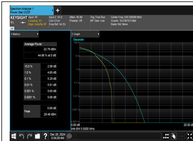
Band26(824-849)-5MHz-16QAM-26815-1RB#0-PASS
