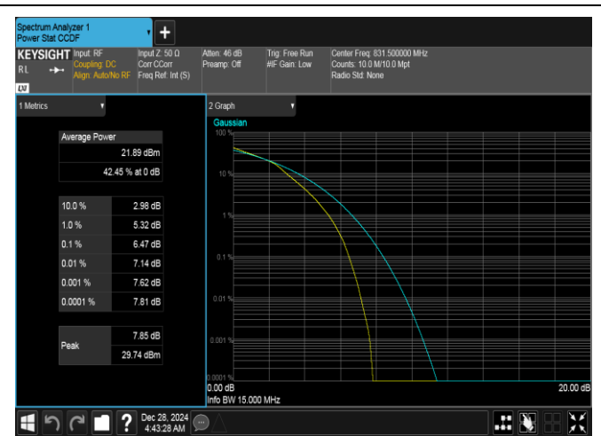
Band26(824-849)-15MHz-16QAM-26865-75RB#0-PASS
