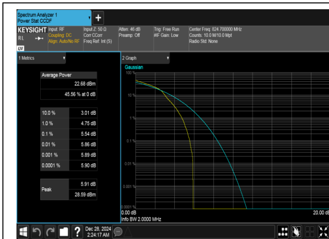
Band26(824-849)-1.4MHz-16QAM-26797-1RB#0-PASS
