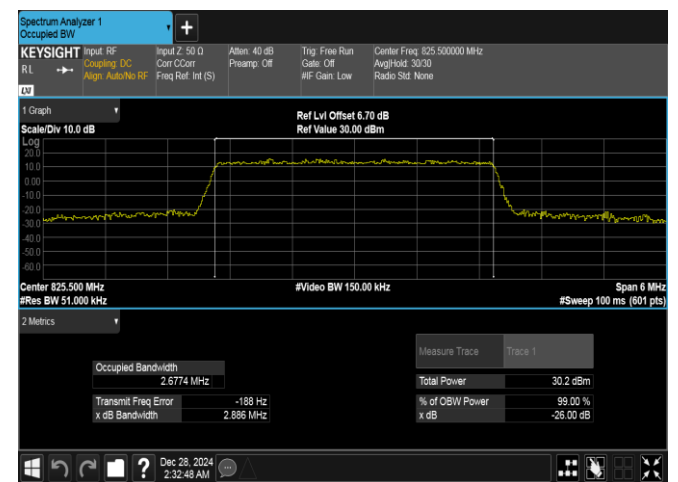
Band26(824-849)-3MHz-16QAM-26805-15RB#0-PASS
