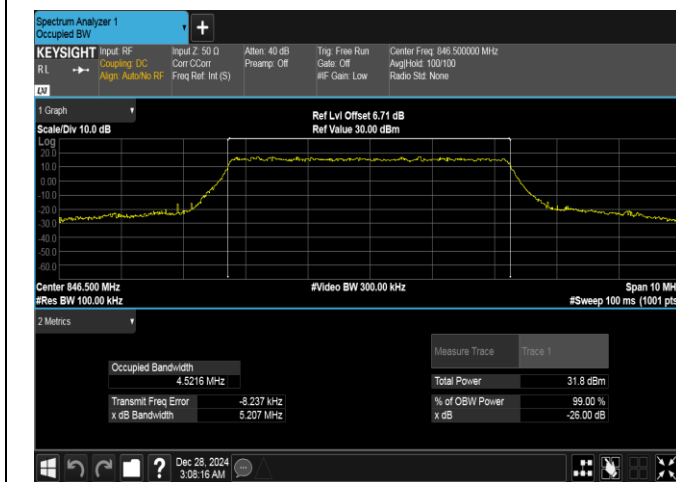
Band26(824-849)-5MHz-QPSK-27015-25RB#0-PASS
