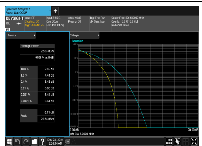
Band26(824-849)-5MHz-QPSK-26815-25RB#0-PASS
