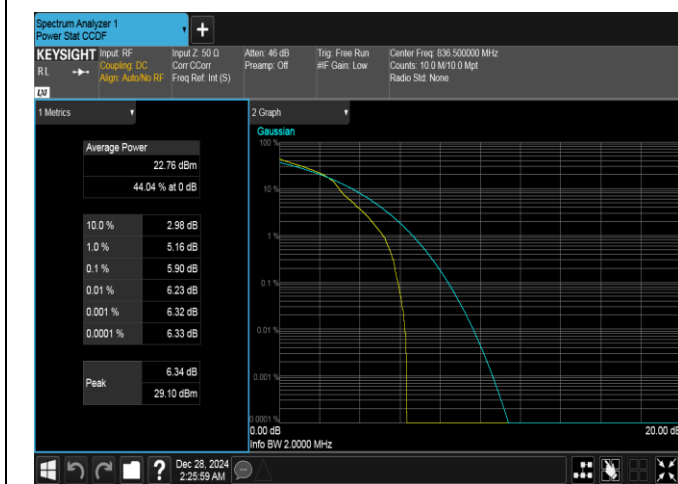
Band26(824-849)-1.4MHz-16QAM-26915-1RB#0-PASS
