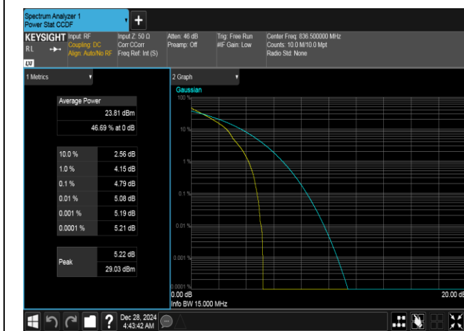
Band26(824-849)-15MHz-QPSK-26915-1RB#0-PASS
