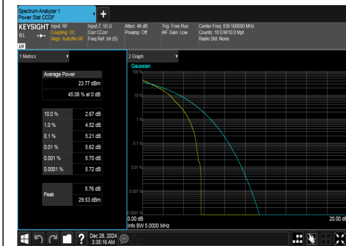
Band26(824-849)-5MHz-QPSK-26915-1RB#0-PASS
