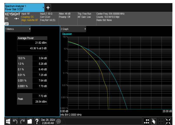
Band26(824-849)-1.4MHz-16QAM-26915-6RB#0-PASS
