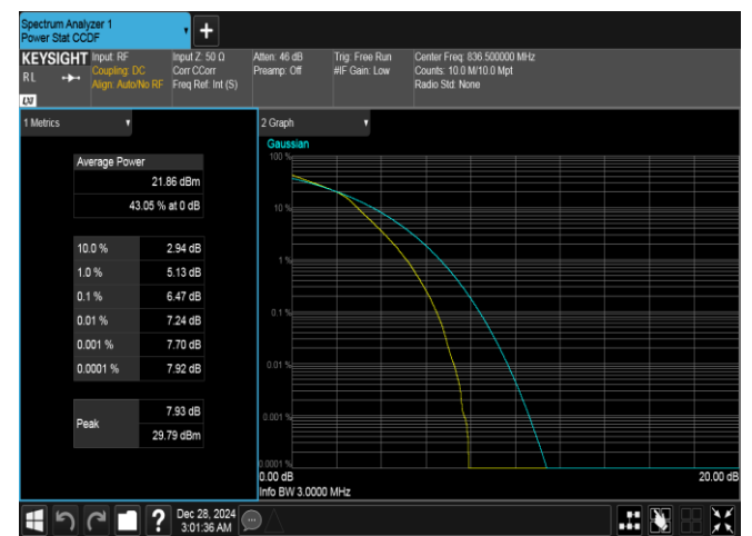
Band26(824-849)-3MHz-16QAM-26915-15RB#0-PASS
