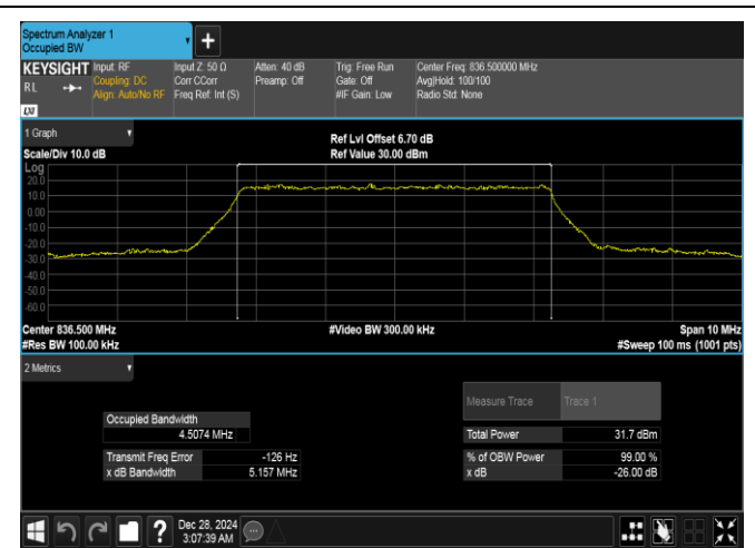
Band26(824-849)-5MHz-QPSK-26915-25RB#0-PASS
