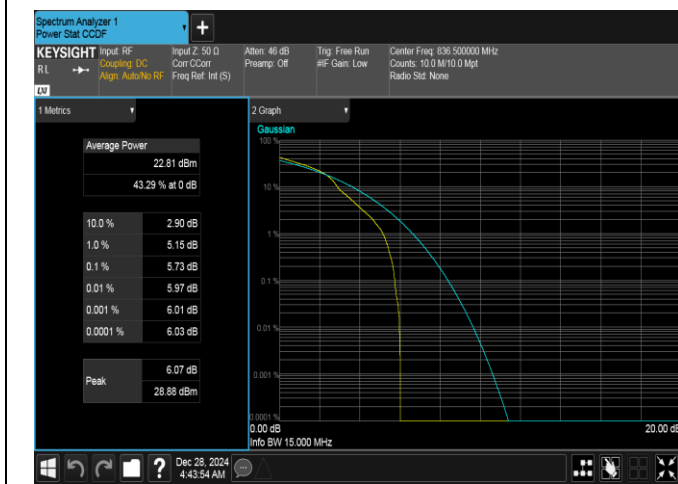
Band26(824-849)-15MHz-16QAM-26915-1RB#0-PASS
