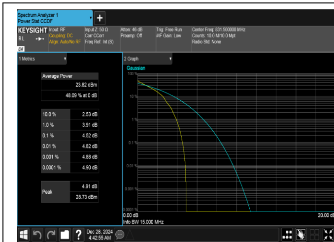
Band26(824-849)-15MHz-QPSK-26865-1RB#0-PASS
