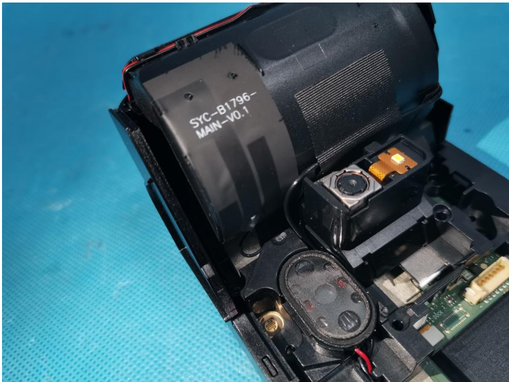
INTERNAL VIEW-3 OF EUT(GSM&WCDMA&LTE Antenna)
