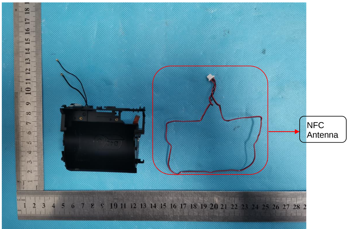
INTERNAL VIEW-19 OF EUT
