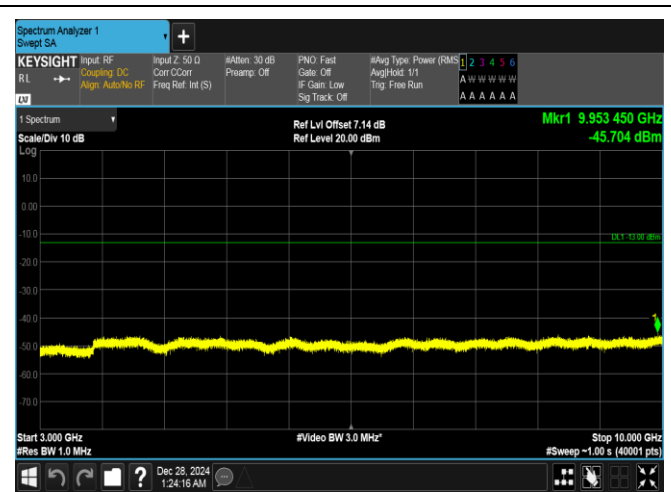
Band26(814-824)-5MHz-QPSK-26740-1RB#0-3000~10000-PASS
