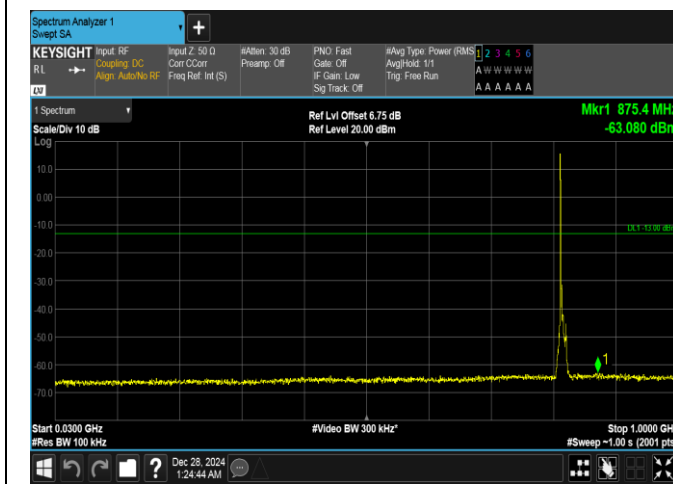
Band26(814-824)-5MHz-16QAM-26740-1RB#0-30~1000-PASS
