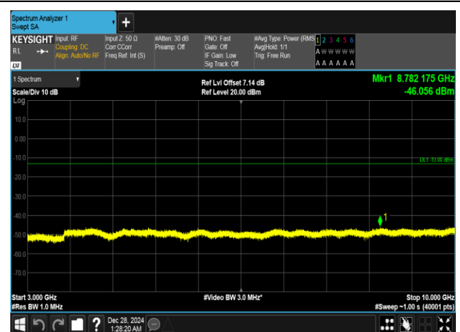
Band26(814-824)-5MHz-QPSK-26740-25RB#0-3000~10000-PASS
