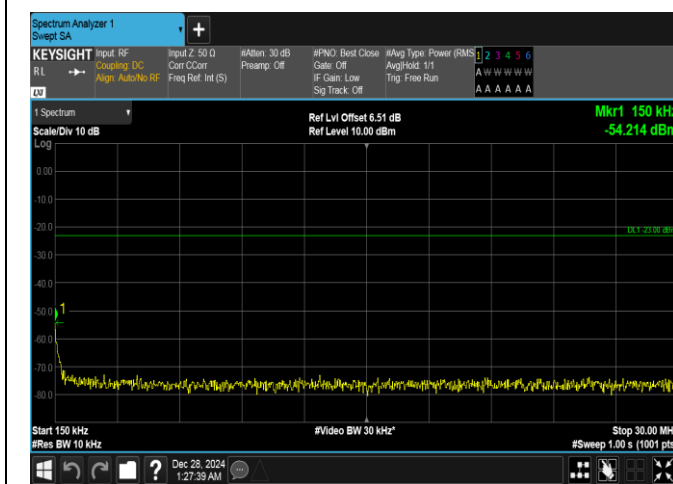
Band26(814-824)-5MHz-QPSK-26740-25RB#0-0.15~30-PASS
