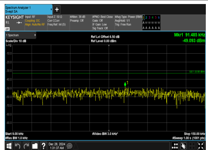
Band26(814-824)-5MHz-QPSK-26765-1RB#24-0.009~0.15-PASS
