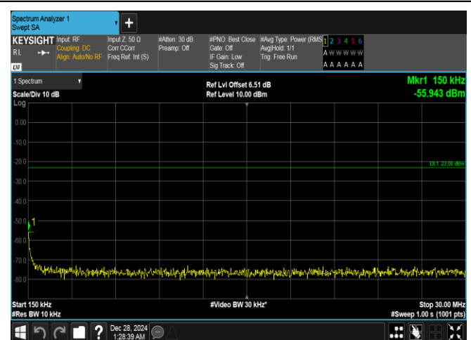
Band26(814-824)-5MHz-16QAM-26740-25RB#0-0.15~30-PASS
