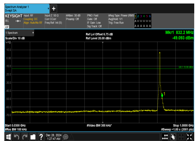
Band26(814-824)-5MHz-QPSK-26740-25RB#0-30~1000-PASS
