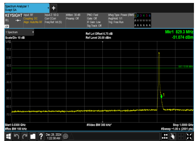
Band26(814-824)-5MHz-16QAM-26715-25RB#0-30~1000-PASS
