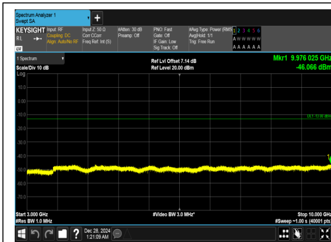
Band26(814-824)-5MHz-16QAM-26715-1RB#24-3000~10000-PASS
