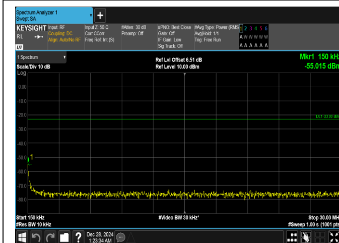
Band26(814-824)-5MHz-QPSK-26740-1RB#0-0.15~30-PASS
