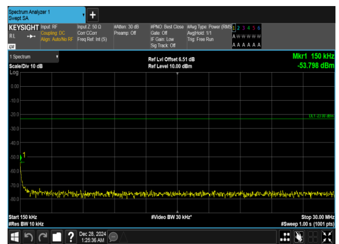
Band26(814-824)-5MHz-QPSK-26740-1RB#24-0.15~30-PASS
