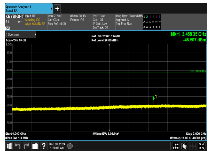
Band26(814-824)-5MHz-QPSK-26765-1RB#0-1000~3000-PASS
