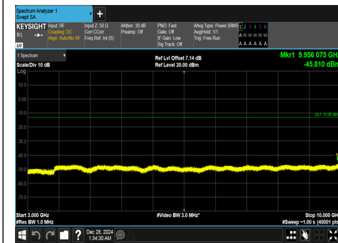
Band26(814-824)-5MHz-QPSK-26765-25RB#0-3000~10000-PASS
