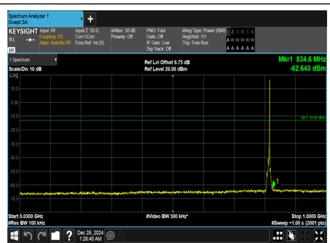
Band26(814-824)-5MHz-16QAM-26740-1RB#24-30~1000-PASS
