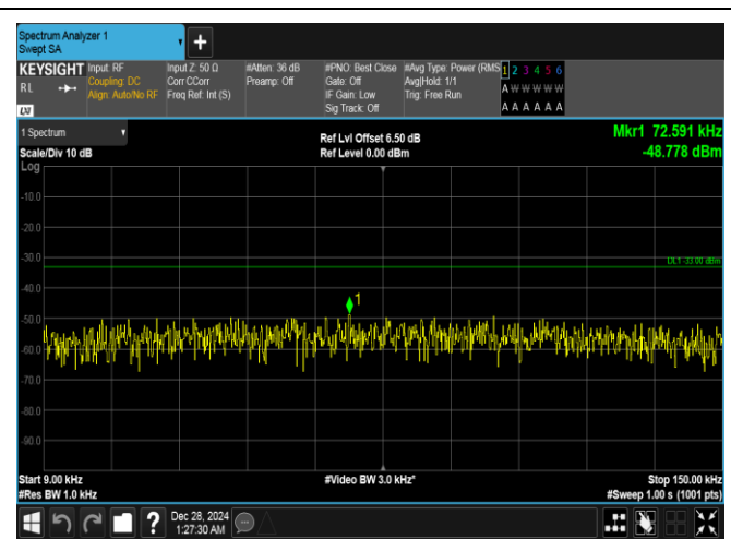
Band26(814-824)-5MHz-QPSK-26740-25RB#0-0.009~0.15-PASS
