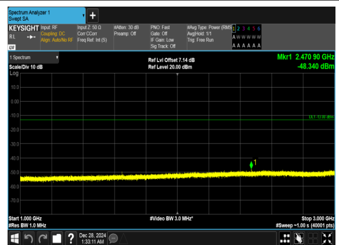
Band26(814-824)-5MHz-16QAM-26765-1RB#24-1000~3000-PASS
