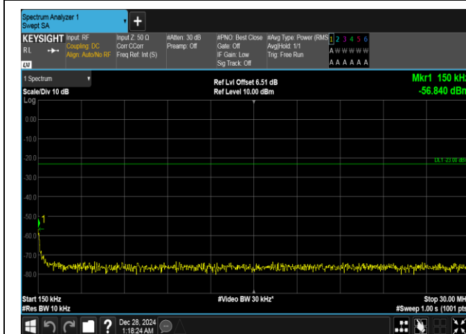
Band26(814-824)-5MHz-16QAM-26715-1RB#0-0.15~30-PASS
