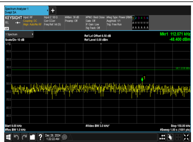
Band26(814-824)-5MHz-16QAM-26715-25RB#0-0.009~0.15-PASS
