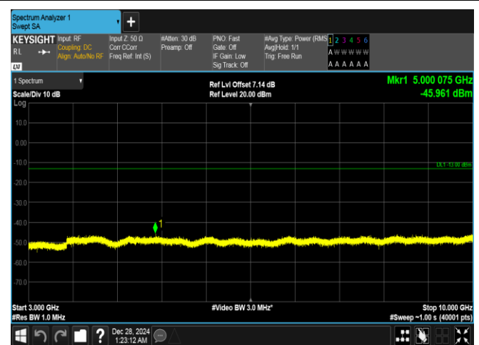
Band26(814-824)-5MHz-16QAM-26715-25RB#0-3000~10000-PASS
