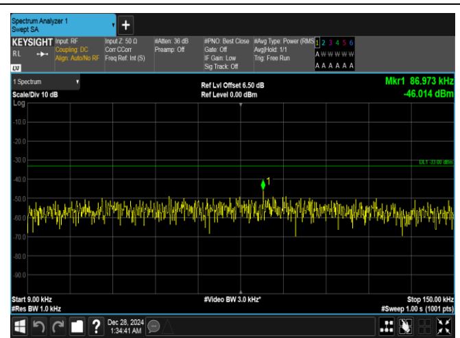
Band26(814-824)-5MHz-16QAM-26765-25RB#0-0.009~0.15-PASS
