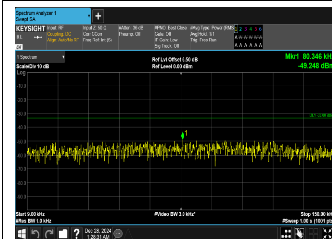
Band26(814-824)-5MHz-16QAM-26740-25RB#0-0.009~0.15-PASS
