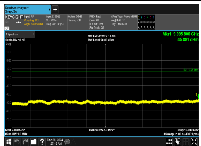
Band26(814-824)-5MHz-16QAM-26740-1RB#24-3000~10000-PASS
