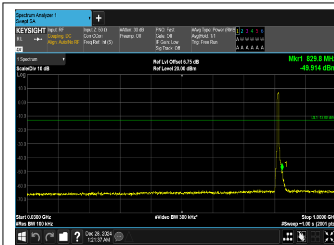
Band26(814-824)-5MHz-QPSK-26715-25RB#0-30~1000-PASS
