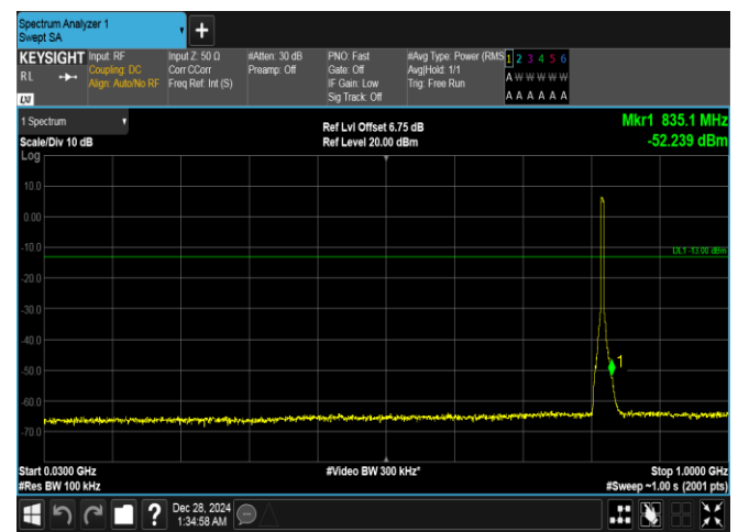
Band26(814-824)-5MHz-16QAM-26765-25RB#0-30~1000-PASS
