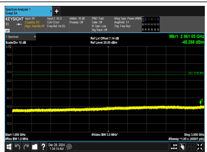
Band26(814-824)-5MHz-QPSK-26765-25RB#0-1000~3000-PASS
