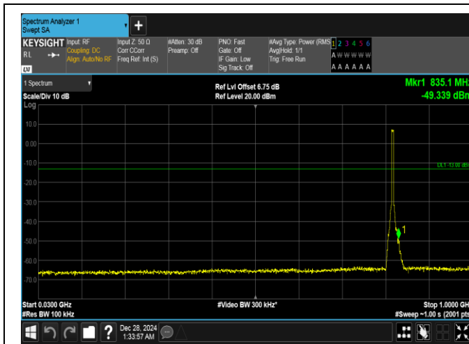
Band26(814-824)-5MHz-QPSK-26765-25RB#0-30~1000-PASS
