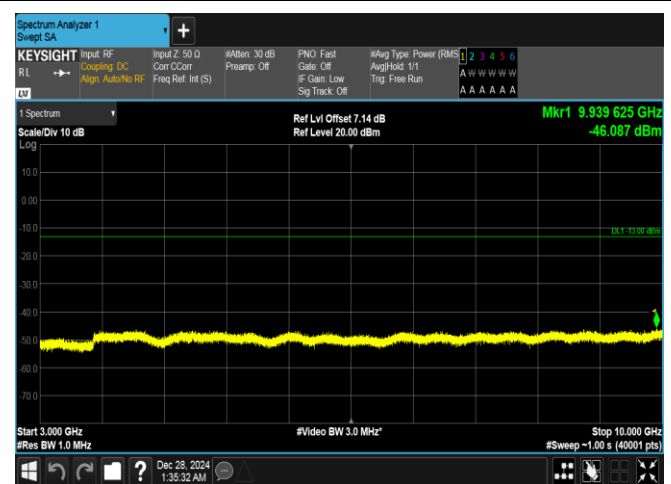
Band26(814-824)-5MHz-16QAM-26765-25RB#0-3000~10000-PASS
