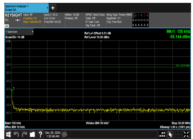
Band26(814-824)-5MHz-16QAM-26765-1RB#24-0.15~30-PASS
