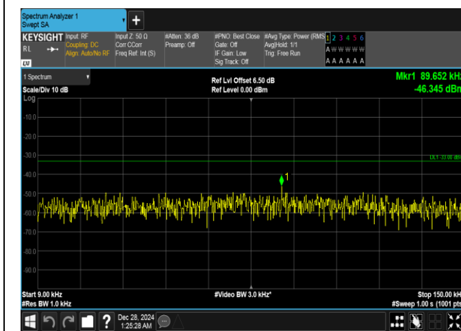
Band26(814-824)-5MHz-QPSK-26740-1RB#24-0.009~0.15-PASS
