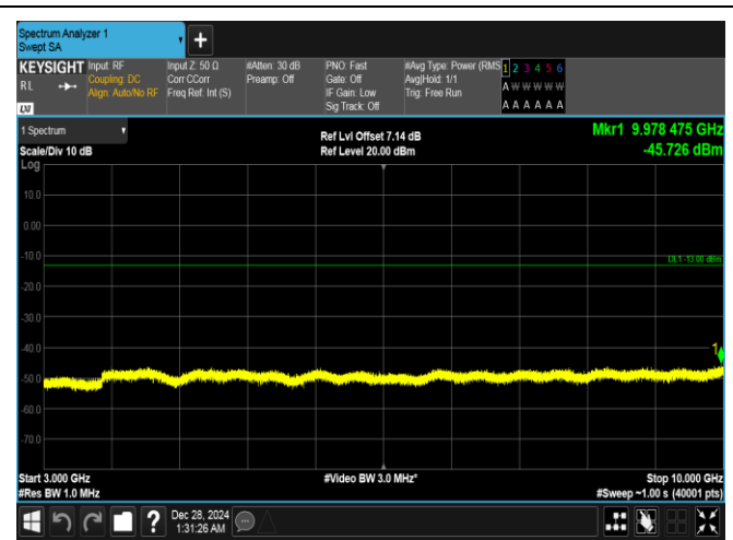
Band26(814-824)-5MHz-16QAM-26765-1RB#0-3000~10000-PASS
