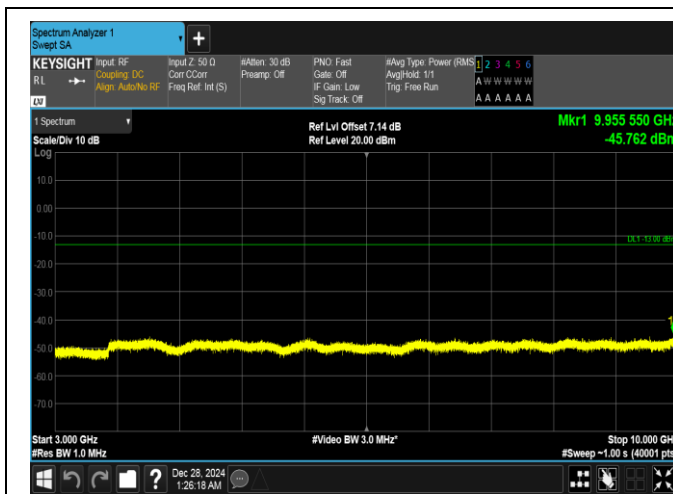
Band26(814-824)-5MHz-QPSK-26740-1RB#24-3000~10000-PASS
