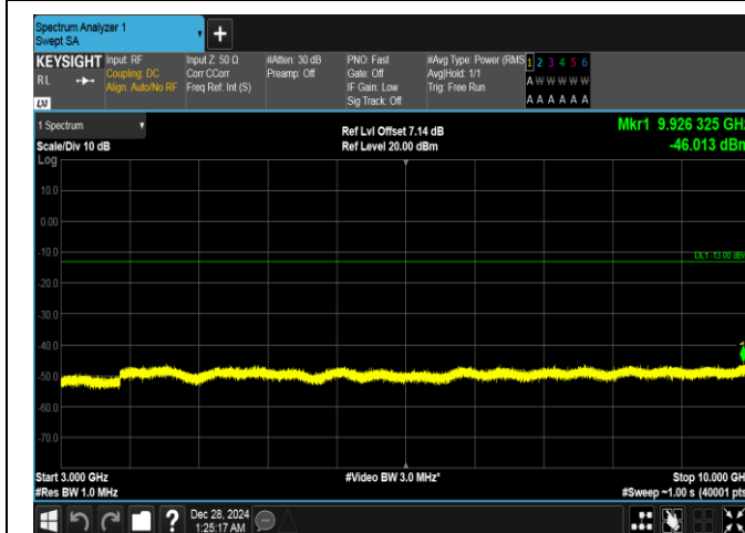
Band26(814-824)-5MHz-16QAM-26740-1RB#0-3000~10000-PASS
