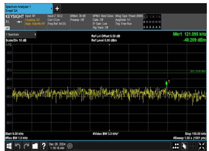
Band26(814-824)-5MHz-16QAM-26715-1RB#0-0.009~0.15-PASS
