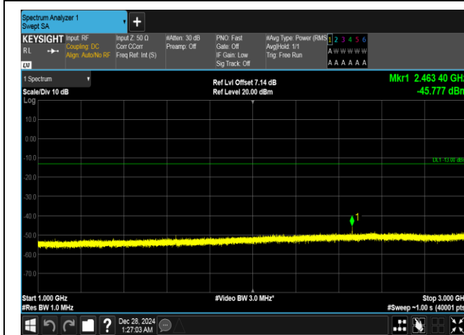
Band26(814-824)-5MHz-16QAM-26740-1RB#24-1000~3000-PASS
