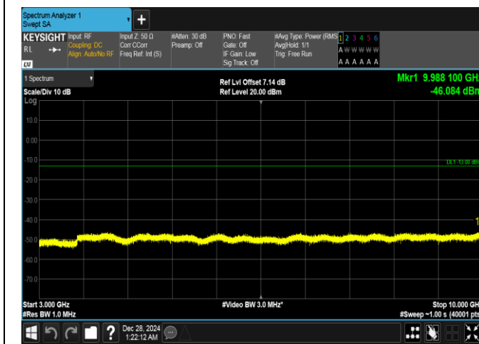
Band26(814-824)-5MHz-QPSK-26715-25RB#0-3000~10000-PASS
