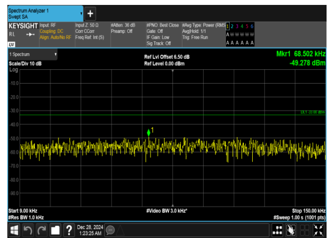
Band26(814-824)-5MHz-QPSK-26740-1RB#0-0.009~0.15-PASS
