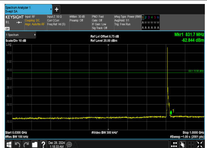
Band26(814-824)-5MHz-16QAM-26715-1RB#0-30~1000-PASS
