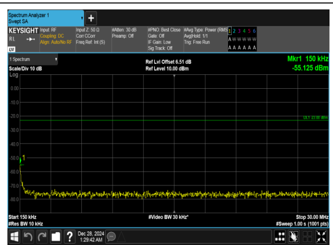
Band26(814-824)-5MHz-QPSK-26765-1RB#0-0.15~30-PASS
