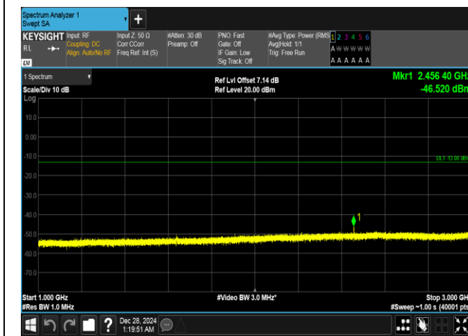
Band26(814-824)-5MHz-QPSK-26715-1RB#24-1000~3000-PASS
