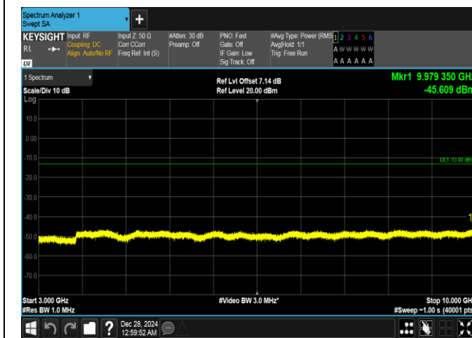
Band26(814-824)-3MHz-QPSK-26775-15RB#0-3000~10000-PASS
