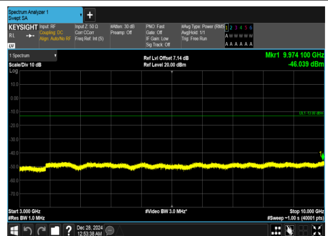
Band26(814-824)-3MHz-QPSK-26740-15RB#0-3000~10000-PASS
