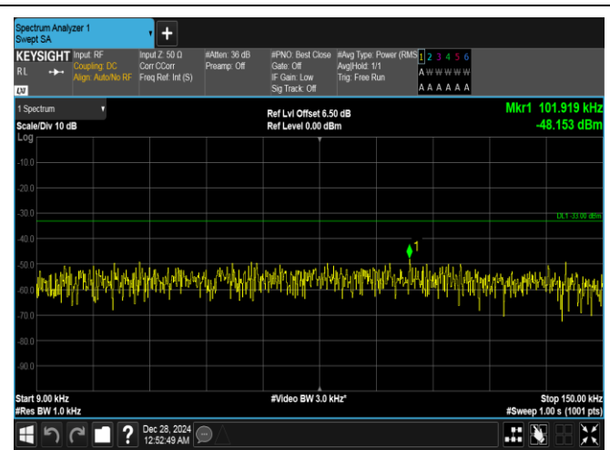
Band26(814-824)-3MHz-QPSK-26740-15RB#0-0.009~0.15-PASS
