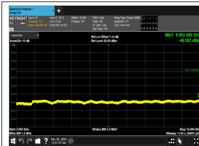
Band26(814-824)-3MHz-QPSK-26740-1RB#14-3000~10000-PASS
