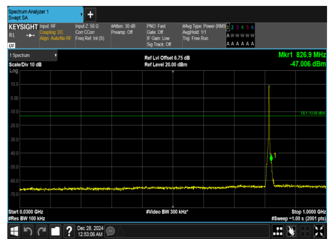
Band26(814-824)-3MHz-QPSK-26740-15RB#0-30~1000-PASS
