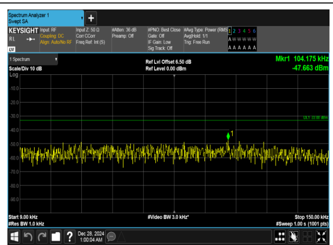
Band26(814-824)-3MHz-16QAM-26775-15RB#0-0.009~0.15-PASS
