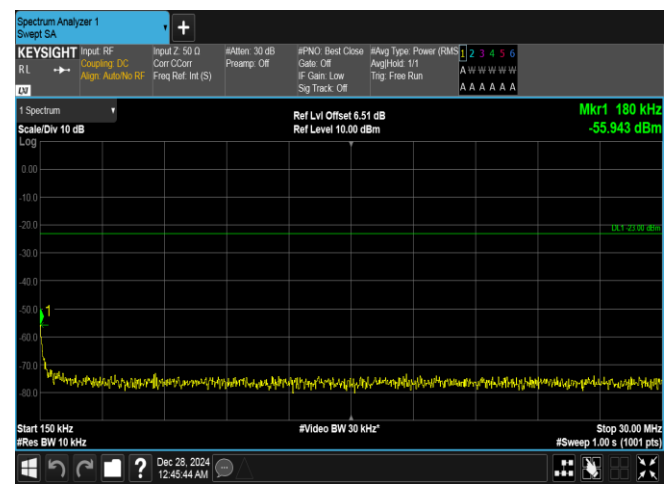
Band26(814-824)-3MHz-16QAM-26705-1RB#14-0.15~30-PASS
