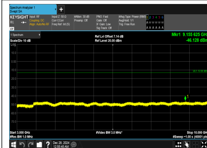
Band26(814-824)-3MHz-QPSK-26775-1RB#0-3000~10000-PASS
