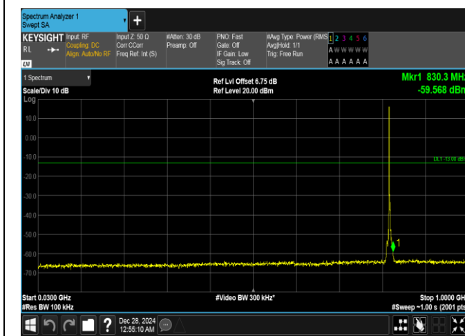
Band26(814-824)-3MHz-QPSK-26775-1RB#0-30~1000-PASS
