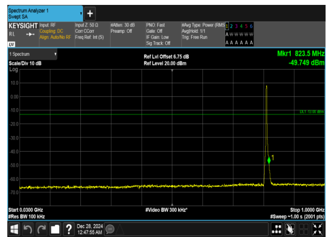
Band26(814-824)-3MHz-16QAM-26705-15RB#0-30~1000-PASS
