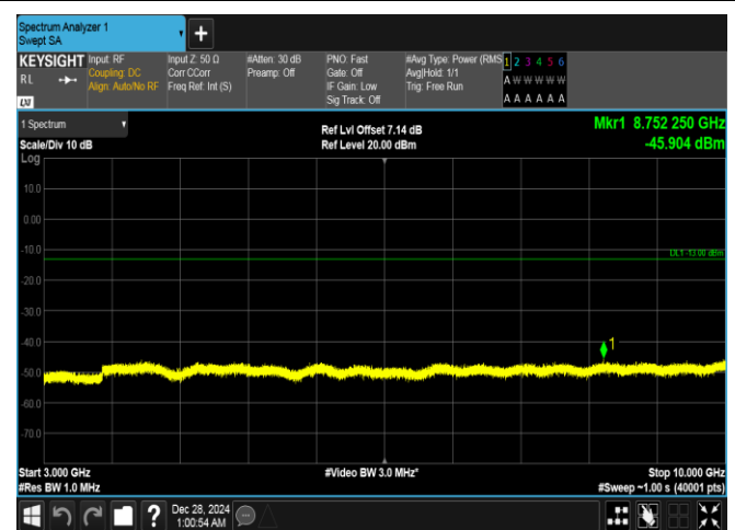
Band26(814-824)-3MHz-16QAM-26775-15RB#0-3000~10000-PASS
