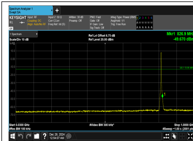
Band26(814-824)-3MHz-16QAM-26740-15RB#0-30~1000-PASS
