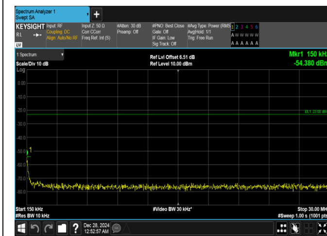
Band26(814-824)-3MHz-QPSK-26740-15RB#0-0.15~30-PASS
