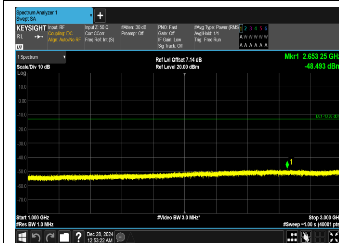
Band26(814-824)-3MHz-QPSK-26740-15RB#0-1000~3000-PASS
