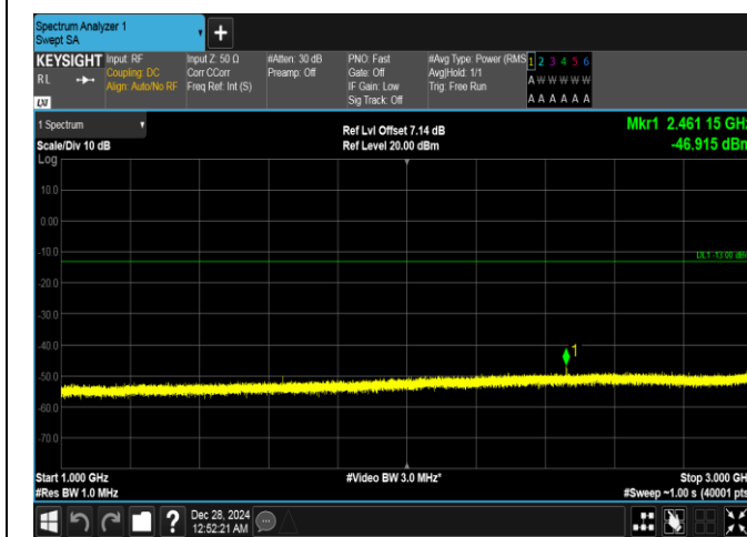
Band26(814-824)-3MHz-16QAM-26740-1RB#14-1000~3000-PASS
