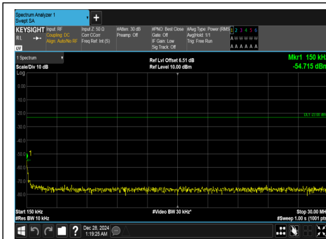
Band26(814-824)-5MHz-QPSK-26715-1RB#24-0.15~30-PASS
