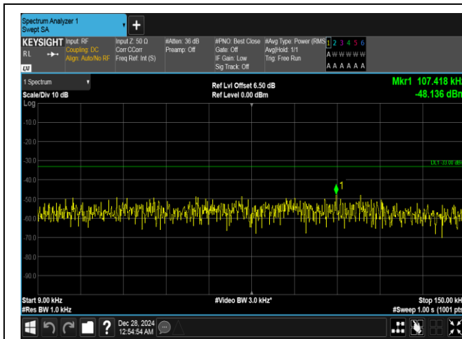
Band26(814-824)-3MHz-QPSK-26775-1RB#0-0.009~0.15-PASS
