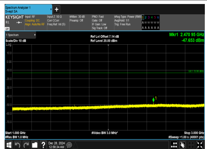
Band26(814-824)-3MHz-16QAM-26775-1RB#14-1000~3000-PASS
