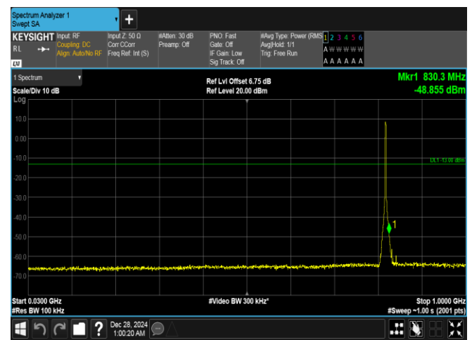
Band26(814-824)-3MHz-16QAM-26775-15RB#0-30~1000-PASS
