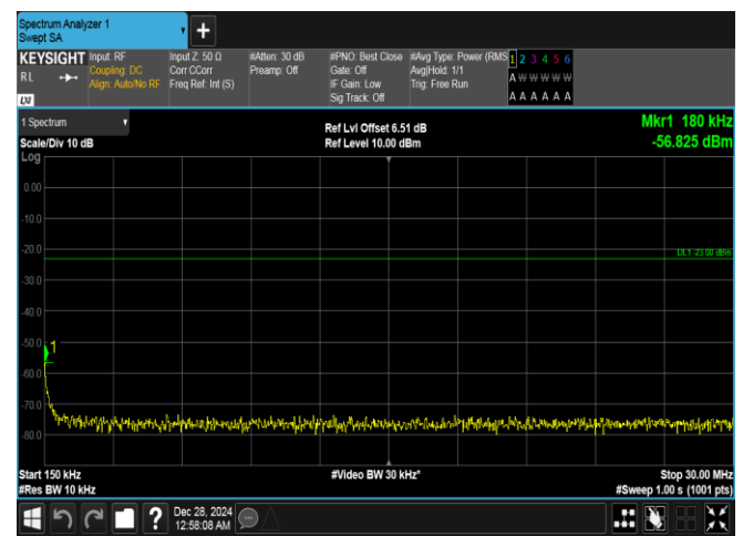
Band26(814-824)-3MHz-16QAM-26775-1RB#14-0.15~30-PASS
