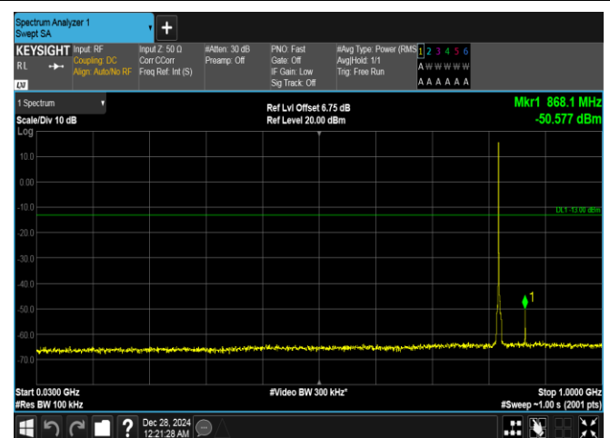
Band26(814-824)-1.4MHz-16QAM-26783-1RB#0-30~1000-PASS
