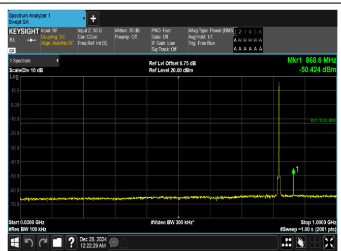
Band26(814-824)-1.4MHz-QPSK-26783-1RB#5-30~1000-PASS
