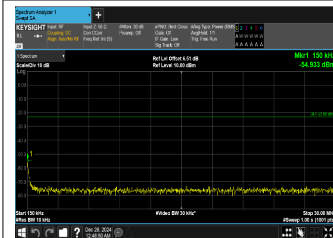
Band26(814-824)-3MHz-QPSK-26740-1RB#0-0.15~30-PASS
