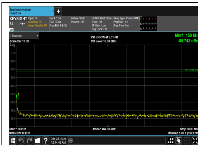
Band26(814-824)-3MHz-QPSK-26705-1RB#14-0.15~30-PASS
