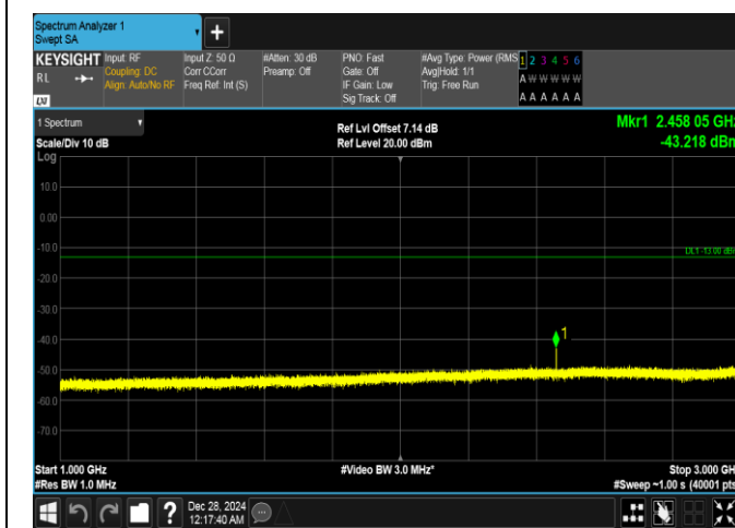
Band26(814-824)-1.4MHz-16QAM-26740-1RB#5-1000~3000-PASS
