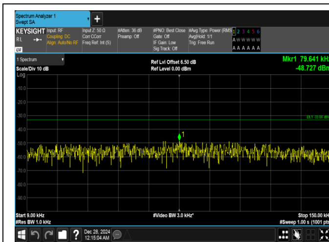
Band26(814-824)-1.4MHz-16QAM-26740-1RB#0-0.009~0.15-PASS
