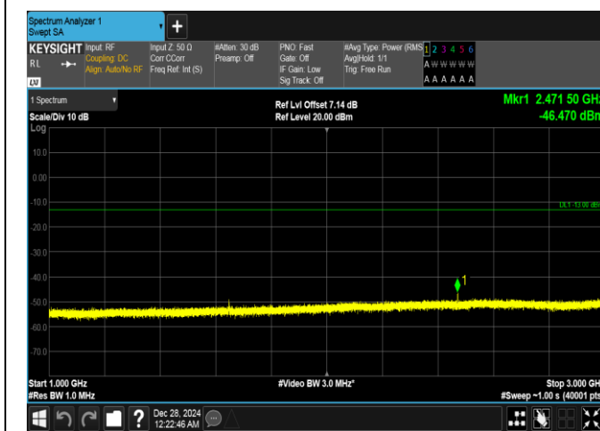
Band26(814-824)-1.4MHz-QPSK-26783-1RB#5-1000~3000-PASS
