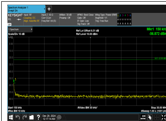
Band26(814-824)-1.4MHz-16QAM-26740-1RB#5-0.15~30-PASS
