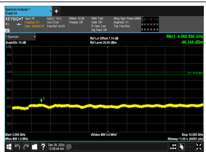
Band26(814-824)-1.4MHz-16QAM-26697-1RB#0-3000~10000-PASS
