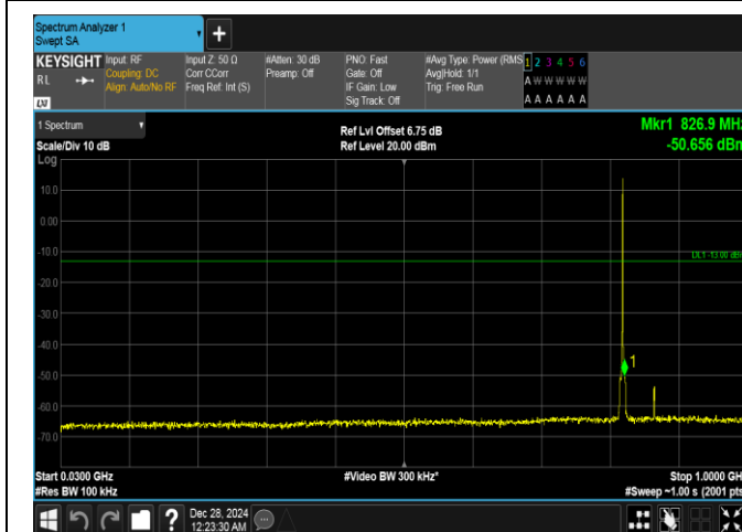
Band26(814-824)-1.4MHz-16QAM-26783-1RB#5-30~1000-PASS
