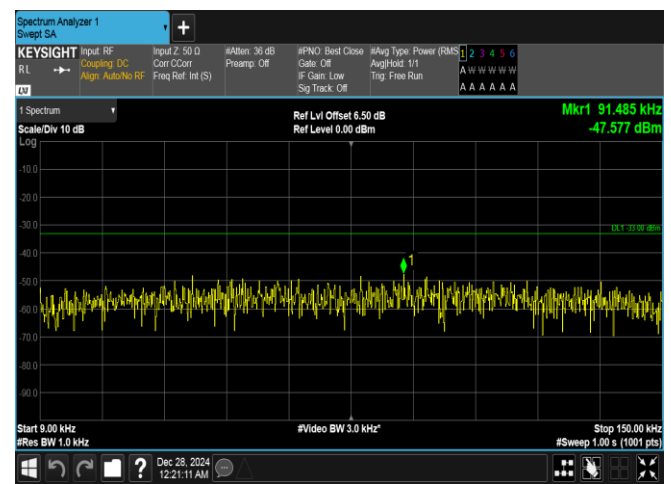
Band26(814-824)-1.4MHz-16QAM-26783-1RB#0-0.009~0.15-PASS
