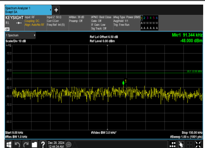
Band26(814-824)-3MHz-QPSK-26705-1RB#14-0.009~0.15-PASS
