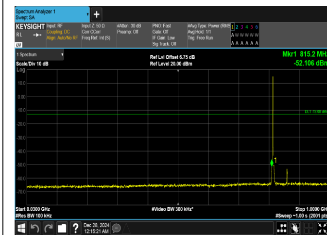
Band26(814-824)-1.4MHz-16QAM-26740-1RB#0-30~1000-PASS
