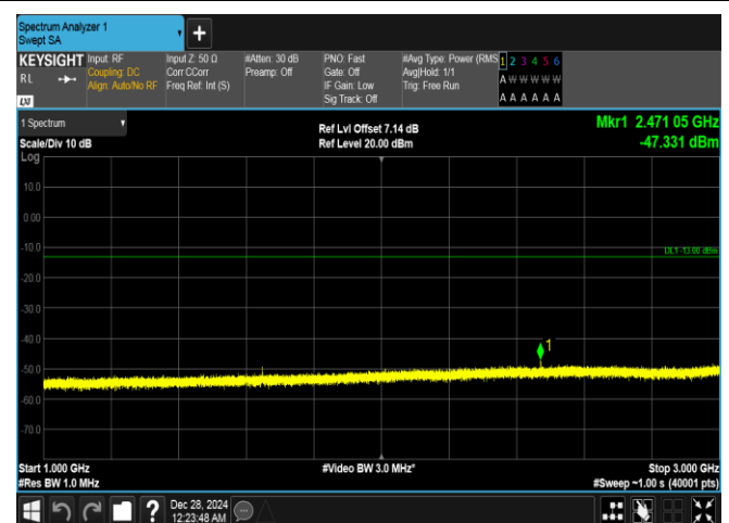
Band26(814-824)-1.4MHz-16QAM-26783-1RB#5-1000~3000-PASS
