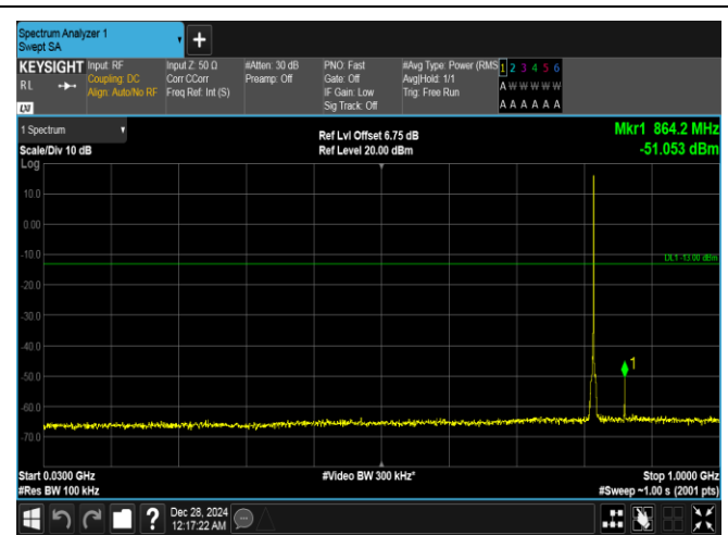
Band26(814-824)-1.4MHz-16QAM-26740-1RB#5-30~1000-PASS
