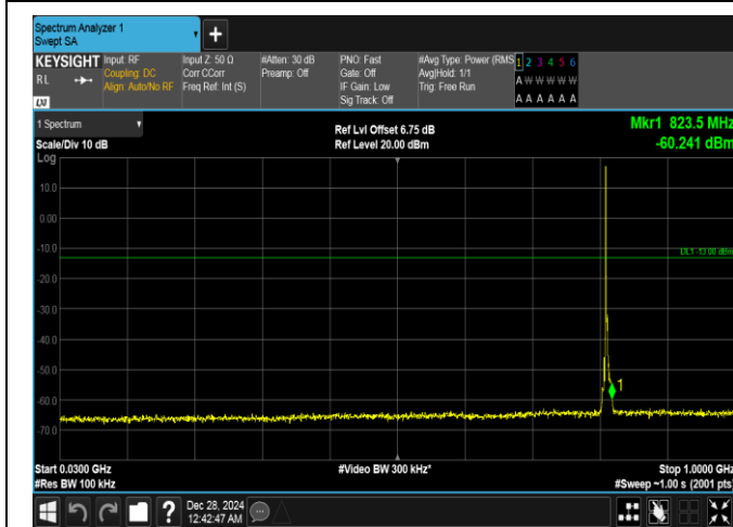
Band26(814-824)-3MHz-QPSK-26705-1RB#0-30~1000-PASS
