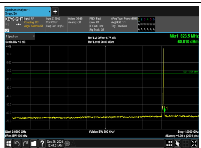
Band26(814-824)-3MHz-QPSK-26705-1RB#14-30~1000-PASS
