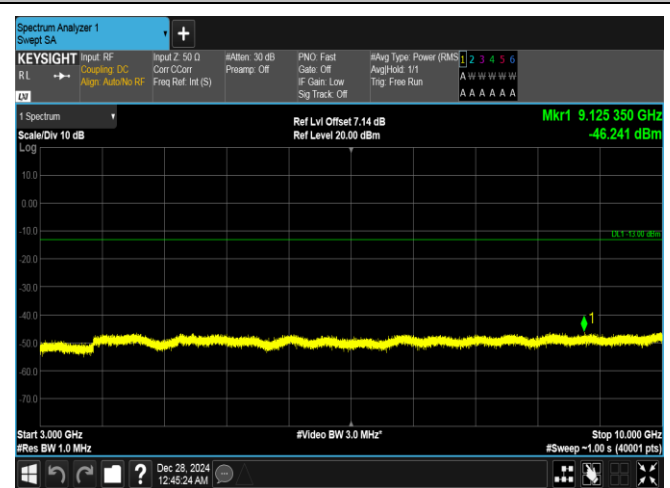
Band26(814-824)-3MHz-QPSK-26705-1RB#14-3000~10000-PASS
