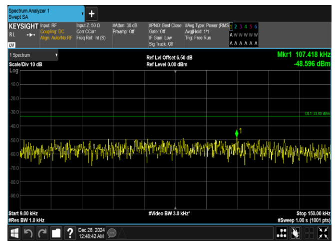
Band26(814-824)-3MHz-QPSK-26740-1RB#0-0.009~0.15-PASS
