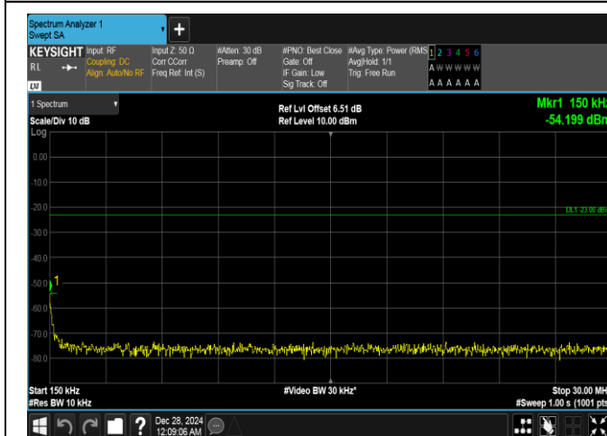
Band26(814-824)-1.4MHz-16QAM-26697-1RB#0-0.15~30-PASS
