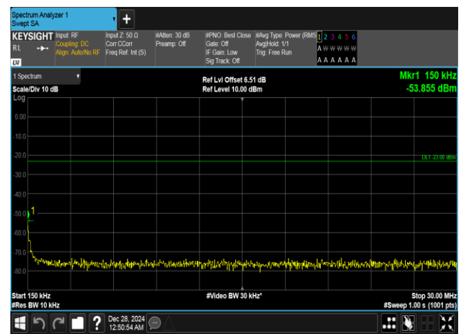
Band26(814-824)-3MHz-QPSK-26740-1RB#14-0.15~30-PASS
