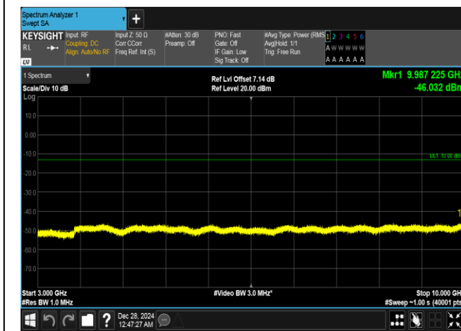
Band26(814-824)-3MHz-QPSK-26705-15RB#0-3000~10000-PASS
