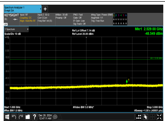
Band26(814-824)-3MHz-QPSK-26705-15RB#0-1000~3000-PASS
