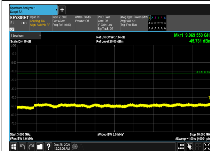
Band26(814-824)-1.4MHz-QPSK-26783-6RB#0-3000~10000-PASS
