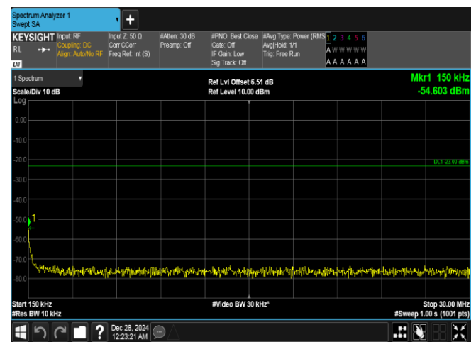
Band26(814-824)-1.4MHz-16QAM-26783-1RB#5-0.15~30-PASS
