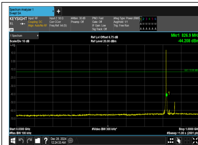
Band26(814-824)-1.4MHz-QPSK-26783-6RB#0-30~1000-PASS
