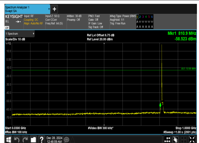
Band26(814-824)-3MHz-QPSK-26740-1RB#0-30~1000-PASS
