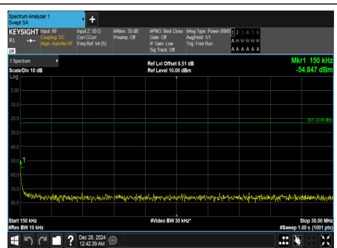
Band26(814-824)-3MHz-QPSK-26705-1RB#0-0.15~30-PASS
