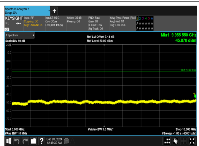
Band26(814-824)-3MHz-QPSK-26740-1RB#0-3000~10000-PASS
