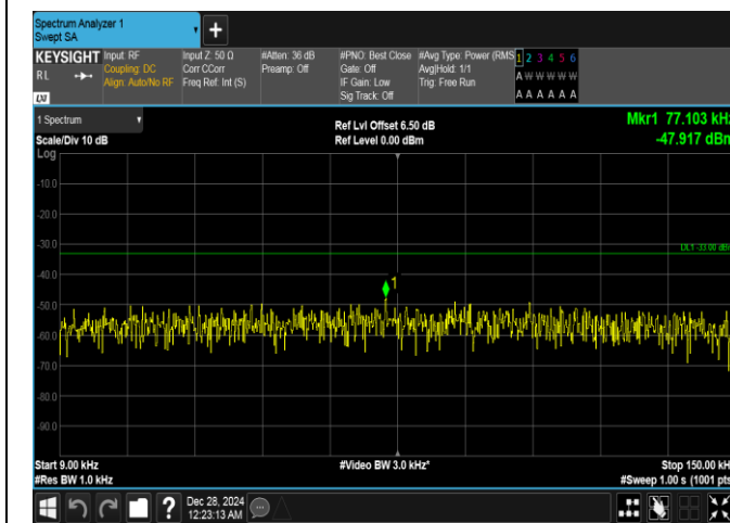
Band26(814-824)-1.4MHz-16QAM-26783-1RB#5-0.009~0.15-PASS
