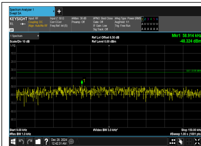
Band26(814-824)-3MHz-QPSK-26705-1RB#0-0.009~0.15-PASS
