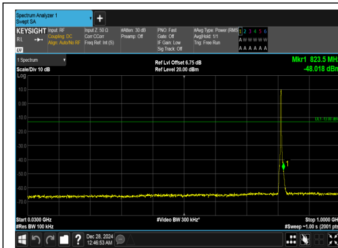
Band26(814-824)-3MHz-QPSK-26705-15RB#0-30~1000-PASS
