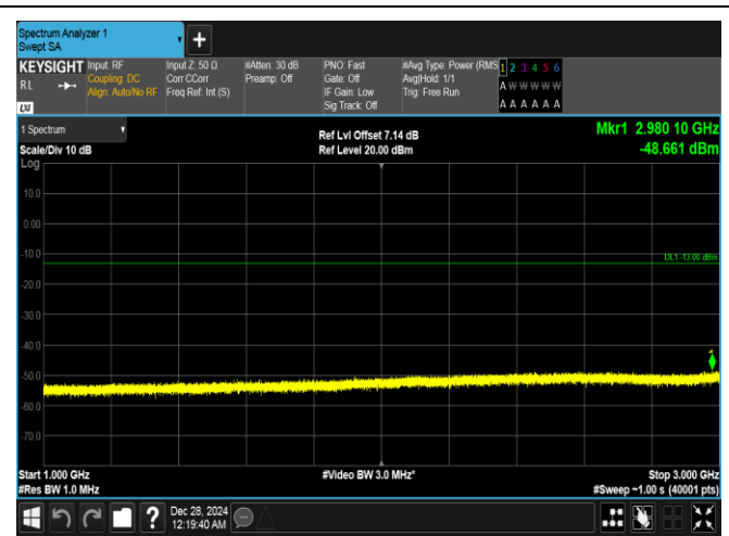
Band26(814-824)-1.4MHz-16QAM-26740-6RB#0-1000~3000-PASS
