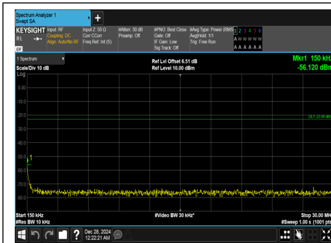
Band26(814-824)-1.4MHz-QPSK-26783-1RB#5-0.15~30-PASS
