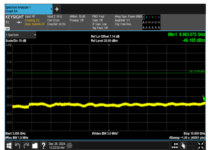
Band26(814-824)-1.4MHz-QPSK-26783-1RB#5-3000~10000-PASS
