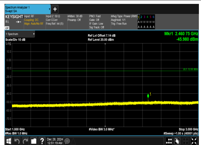
Band26(814-824)-3MHz-QPSK-26740-1RB#14-1000~3000-PASS
