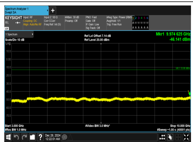
Band26(814-824)-1.4MHz-16QAM-26783-1RB#0-3000~10000-PASS
