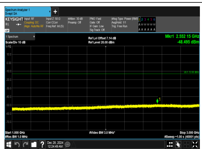
Band26(814-824)-1.4MHz-QPSK-26783-6RB#0-1000~3000-PASS
