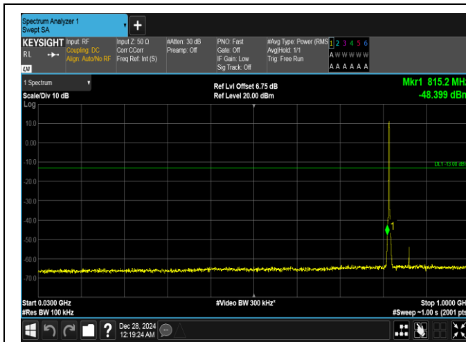
Band26(814-824)-1.4MHz-16QAM-26740-6RB#0-30~1000-PASS
