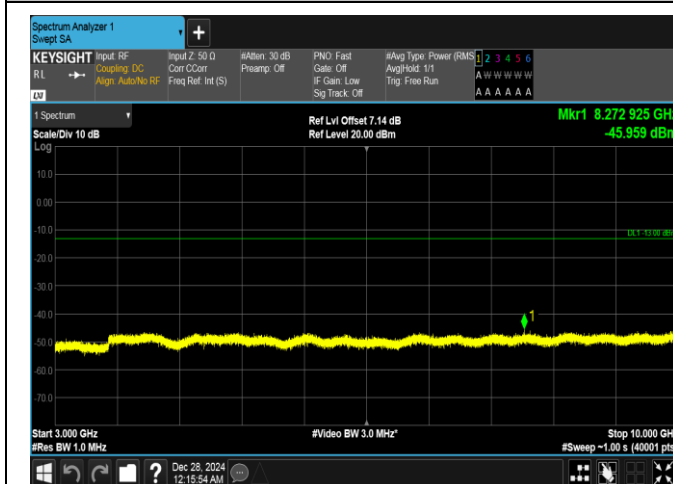
Band26(814-824)-1.4MHz-16QAM-26740-1RB#0-3000~10000-PASS
