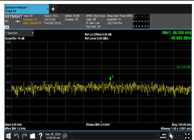
Band26(814-824)-1.4MHz-16QAM-26697-1RB#0-0.009~0.15-PASS
