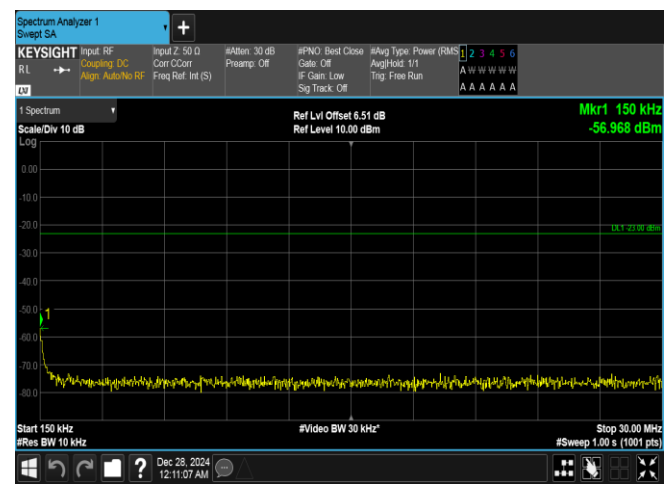
Band26(814-824)-1.4MHz-16QAM-26697-1RB#5-0.15~30-PASS
