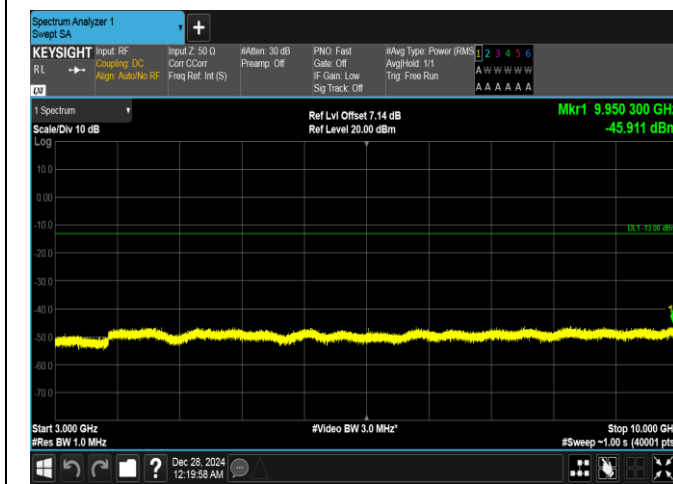
Band26(814-824)-1.4MHz-16QAM-26740-6RB#0-3000~10000-PASS
