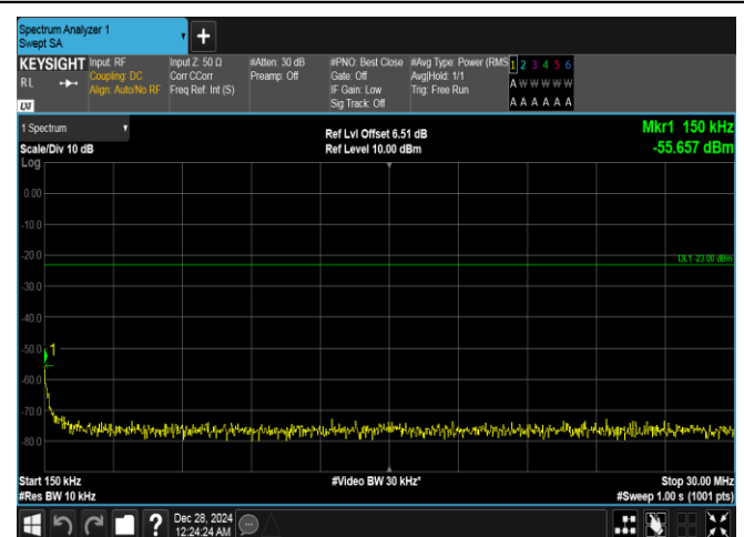
Band26(814-824)-1.4MHz-QPSK-26783-6RB#0-0.15~30-PASS
