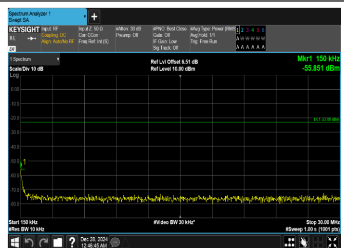
Band26(814-824)-3MHz-QPSK-26705-15RB#0-0.15~30-PASS
