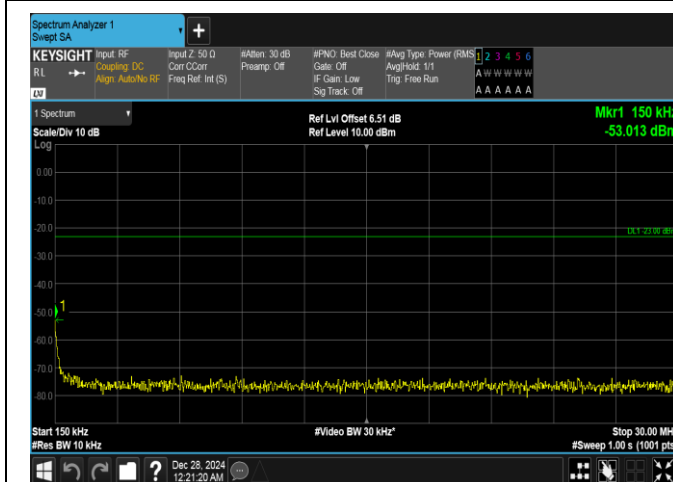
Band26(814-824)-1.4MHz-16QAM-26783-1RB#0-0.15~30-PASS
