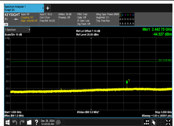
Band26(814-824)-3MHz-QPSK-26705-1RB#0-1000~3000-PASS
