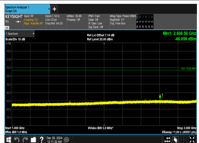
Band26(814-824)-1.4MHz-16QAM-26697-1RB#5-1000~3000-PASS
