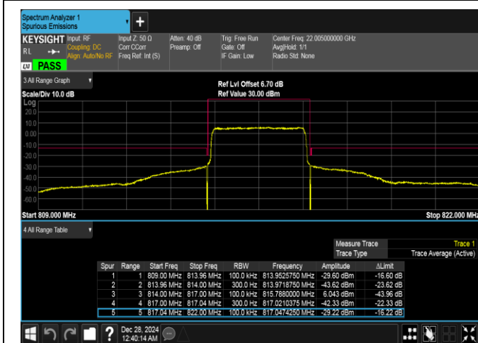
Band26(814-824)-3MHz-QPSK-26705-15RB#0-PASS
