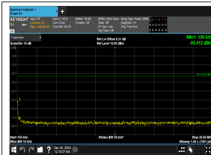
Band26(814-824)-1.4MHz-QPSK-26697-1RB#5-0.15~30-PASS
