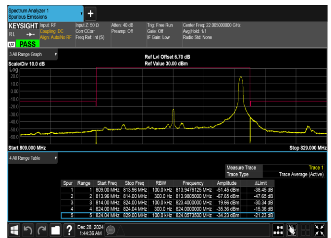
Band26(814-824)-10MHz-QPSK-26740-1RB#49-PASS
