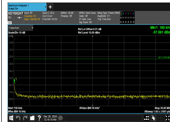
Band26(814-824)-1.4MHz-QPSK-26740-6RB#0-0.15~30-PASS
