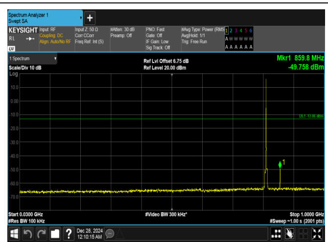
Band26(814-824)-1.4MHz-QPSK-26697-1RB#5-30~1000-PASS
