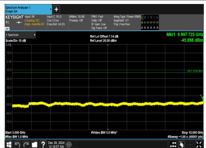
Band26(814-824)-1.4MHz-QPSK-26740-6RB#0-3000~10000-PASS
