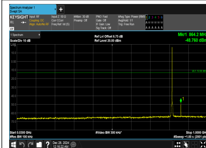
Band26(814-824)-1.4MHz-QPSK-26740-1RB#5-30~1000-PASS
