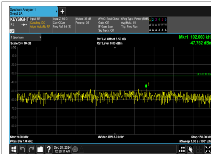
Band26(814-824)-1.4MHz-QPSK-26783-1RB#0-0.009~0.15-PASS
