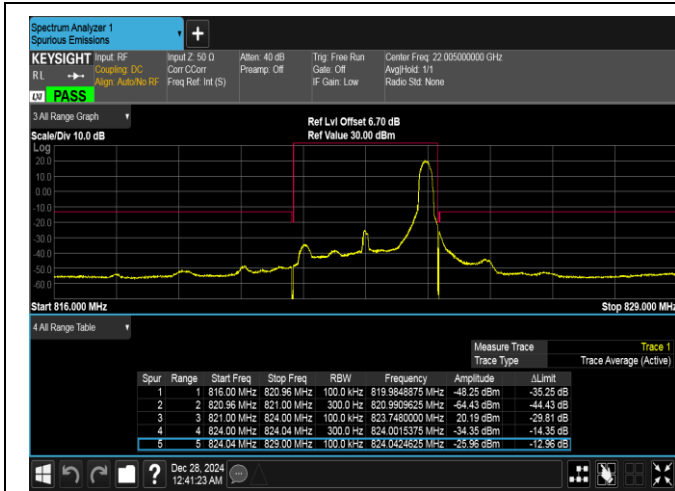
Band26(814-824)-3MHz-QPSK-26775-1RB#14-PASS
