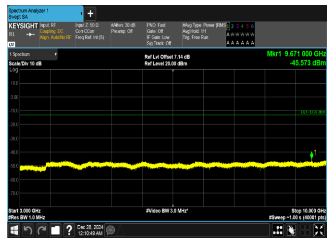
Band26(814-824)-1.4MHz-QPSK-26697-1RB#5-3000~10000-PASS
