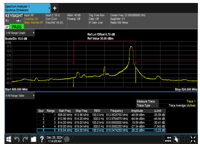
Band26(814-824)-5MHz-QPSK-26715-1RB#24-PASS
