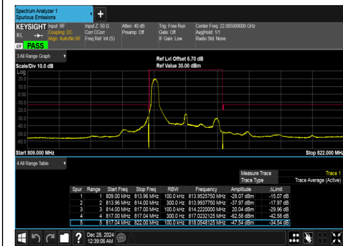
Band26(814-824)-3MHz-QPSK-26705-1RB#0-PASS
