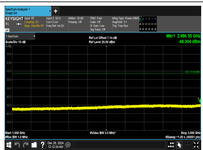
Band26(814-824)-1.4MHz-QPSK-26697-6RB#0-1000~3000-PASS
