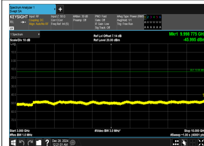
Band26(814-824)-1.4MHz-QPSK-26783-1RB#0-3000~10000-PASS
