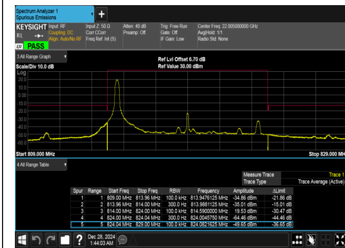
Band26(814-824)-10MHz-QPSK-26740-1RB#0-PASS
