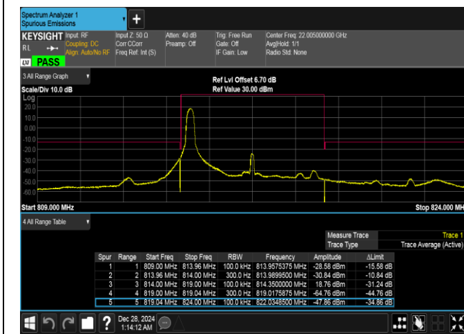
Band26(814-824)-5MHz-16QAM-26715-1RB#0-PASS
