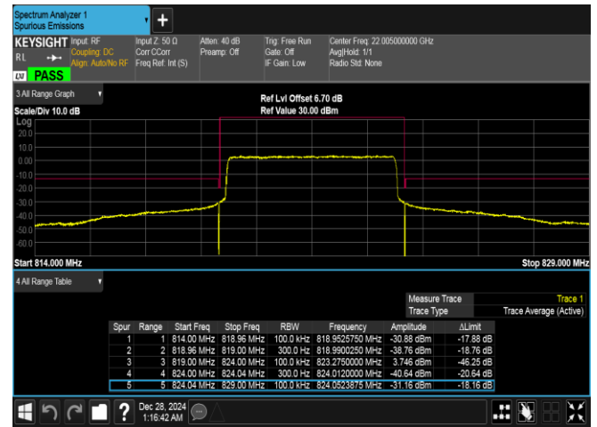
Band26(814-824)-5MHz-QPSK-26765-25RB#0-PASS
