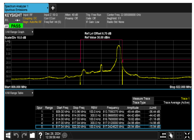
Band26(814-824)-3MHz-16QAM-26705-1RB#14-PASS
