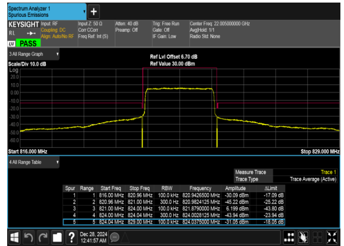
Band26(814-824)-3MHz-QPSK-26775-15RB#0-PASS
