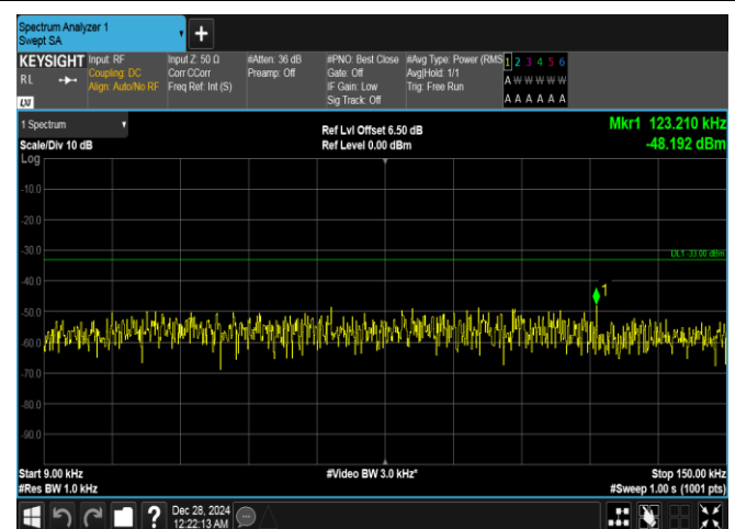
Band26(814-824)-1.4MHz-QPSK-26783-1RB#5-0.009~0.15-PASS
