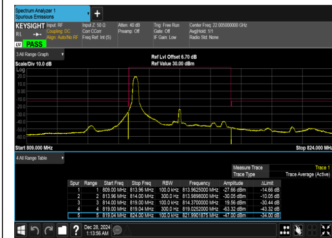
Band26(814-824)-5MHz-QPSK-26715-1RB#0-PASS
