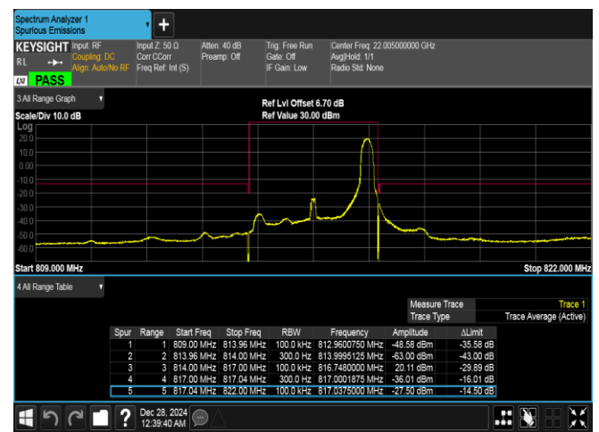
Band26(814-824)-3MHz-QPSK-26705-1RB#14-PASS
