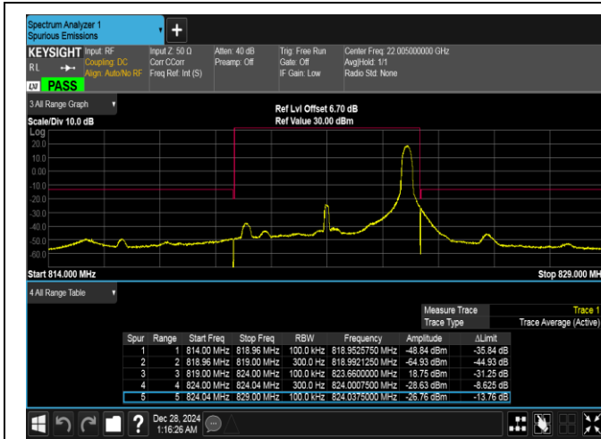
Band26(814-824)-5MHz-16QAM-26765-1RB#24-PASS
