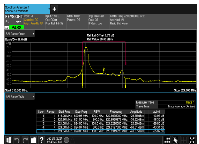
Band26(814-824)-3MHz-QPSK-26775-1RB#0-PASS
