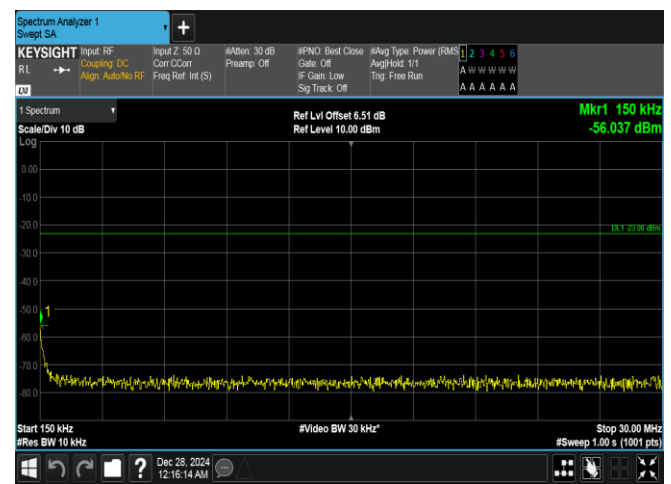
Band26(814-824)-1.4MHz-QPSK-26740-1RB#5-0.15~30-PASS
