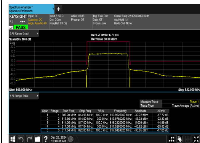
Band26(814-824)-3MHz-16QAM-26705-15RB#0-PASS
