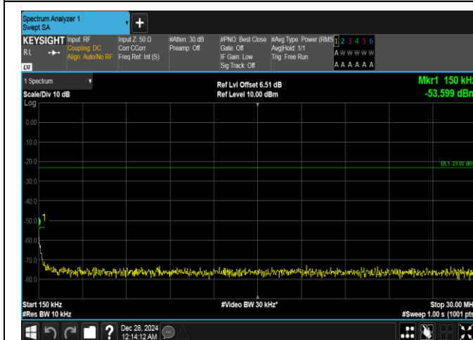
Band26(814-824)-1.4MHz-QPSK-26740-1RB#0-0.15~30-PASS
