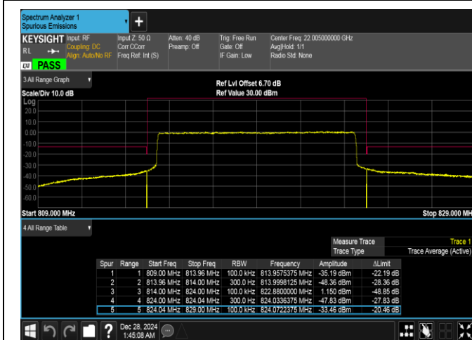
Band26(814-824)-10MHz-QPSK-26740-50RB#0-PASS
