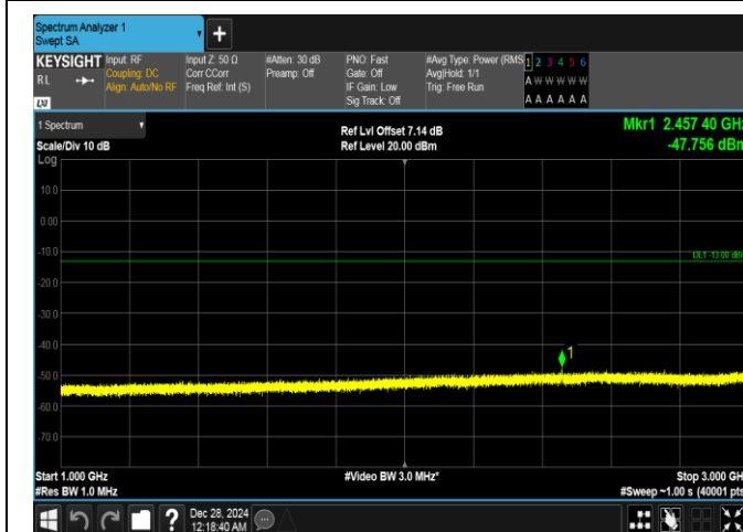
Band26(814-824)-1.4MHz-QPSK-26740-6RB#0-1000~3000-PASS
