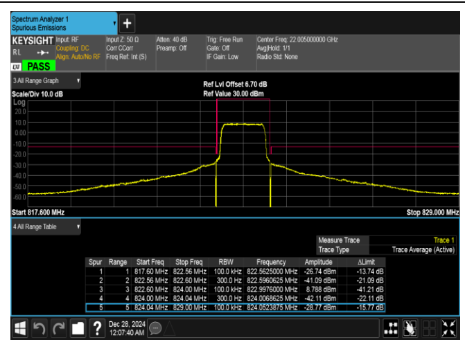
Band26(814-824)-1.4MHz-16QAM-26783-6RB#0-PASS
