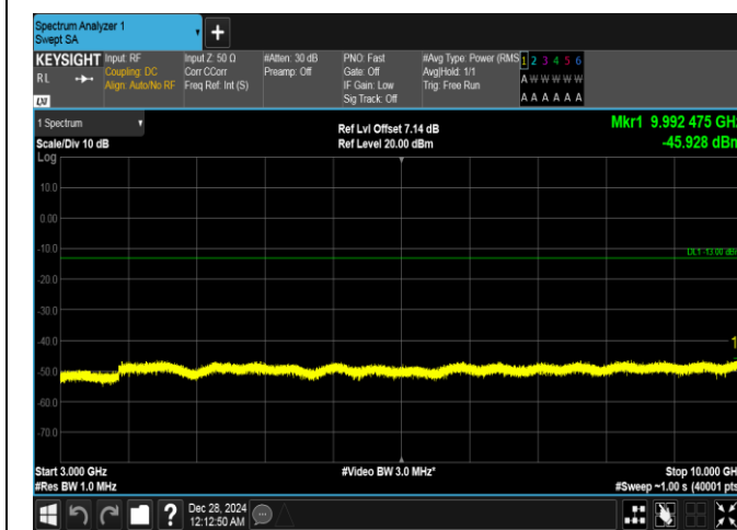
Band26(814-824)-1.4MHz-QPSK-26697-6RB#0-3000~10000-PASS
