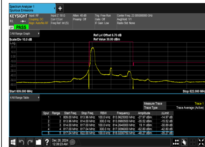
Band26(814-824)-3MHz-16QAM-26705-1RB#0-PASS
