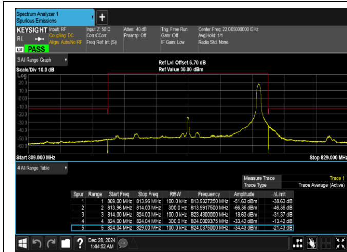
Band26(814-824)-10MHz-16QAM-26740-1RB#49-PASS
