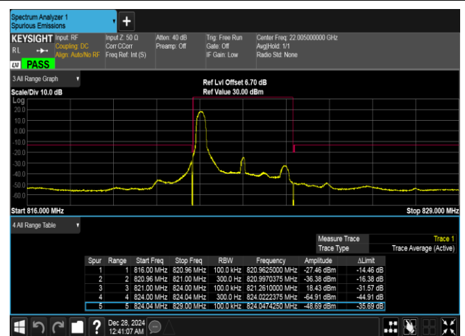
Band26(814-824)-3MHz-16QAM-26775-1RB#0-PASS
