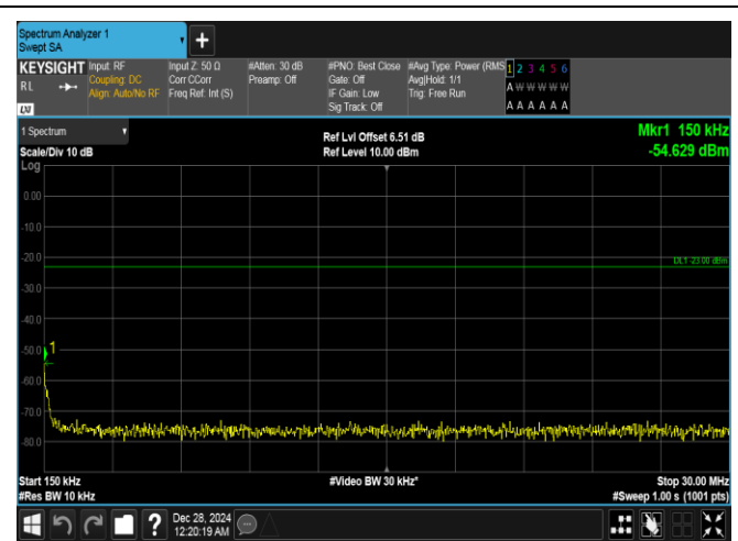
Band26(814-824)-1.4MHz-QPSK-26783-1RB#0-0.15~30-PASS
