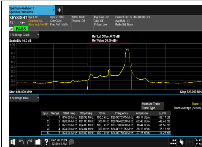
Band26(814-824)-3MHz-16QAM-26775-1RB#14-PASS
