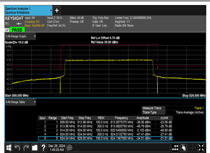
Band26(814-824)-10MHz-16QAM-26740-50RB#0-PASS
