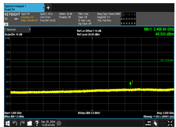
Band26(814-824)-1.4MHz-QPSK-26783-1RB#0-1000~3000-PASS
