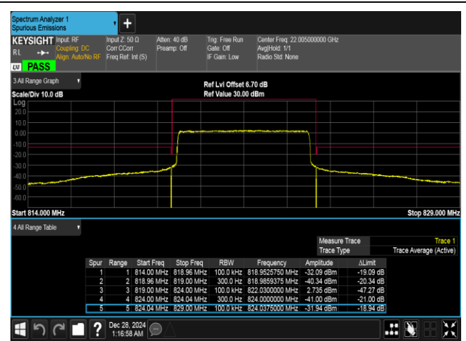
Band26(814-824)-5MHz-16QAM-26765-25RB#0-PASS
