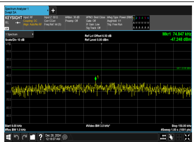
Band26(814-824)-1.4MHz-QPSK-26740-6RB#0-0.009~0.15-PASS
