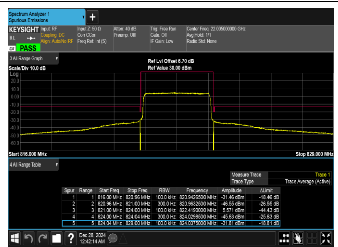
Band26(814-824)-3MHz-16QAM-26775-15RB#0-PASS
