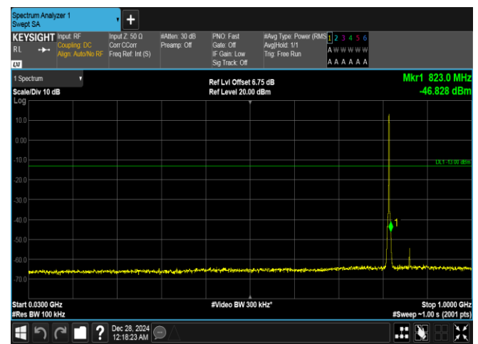
Band26(814-824)-1.4MHz-QPSK-26740-6RB#0-30~1000-PASS
