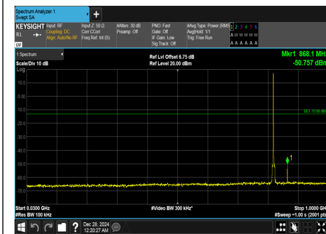
Band26(814-824)-1.4MHz-QPSK-26783-1RB#0-30~1000-PASS
