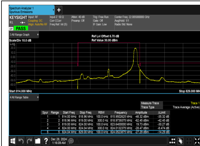
Band26(814-824)-5MHz-QPSK-26765-1RB#24-PASS
