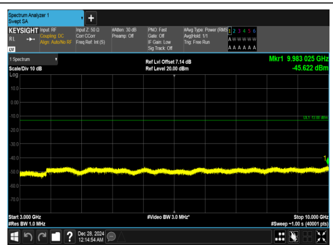
Band26(814-824)-1.4MHz-QPSK-26740-1RB#0-3000~10000-PASS
