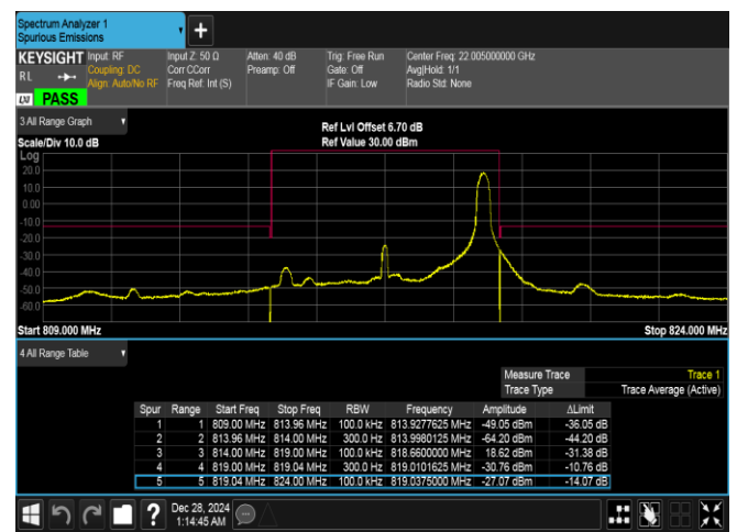
Band26(814-824)-5MHz-16QAM-26715-1RB#24-PASS
