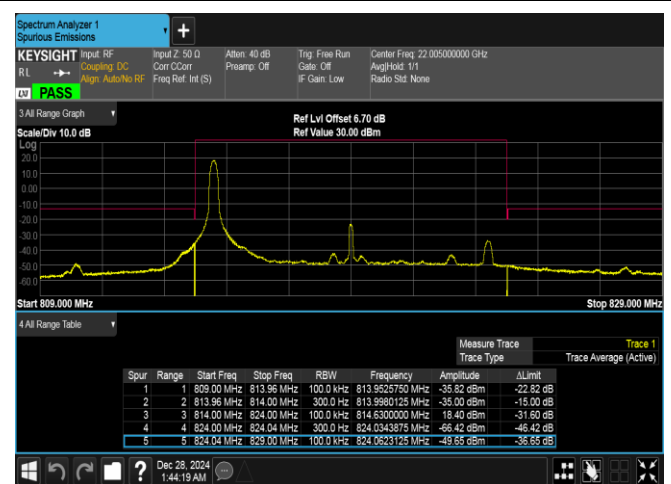
Band26(814-824)-10MHz-16QAM-26740-1RB#0-PASS
