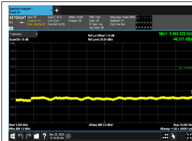
Band26(814-824)-1.4MHz-QPSK-26740-1RB#5-3000~10000-PASS
