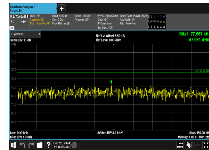
Band26(814-824)-1.4MHz-QPSK-26740-1RB#5-0.009~0.15-PASS
