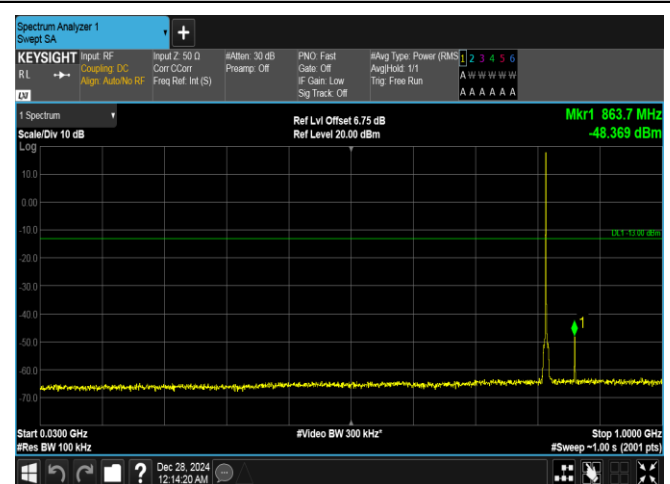
Band26(814-824)-1.4MHz-QPSK-26740-1RB#0-30~1000-PASS
