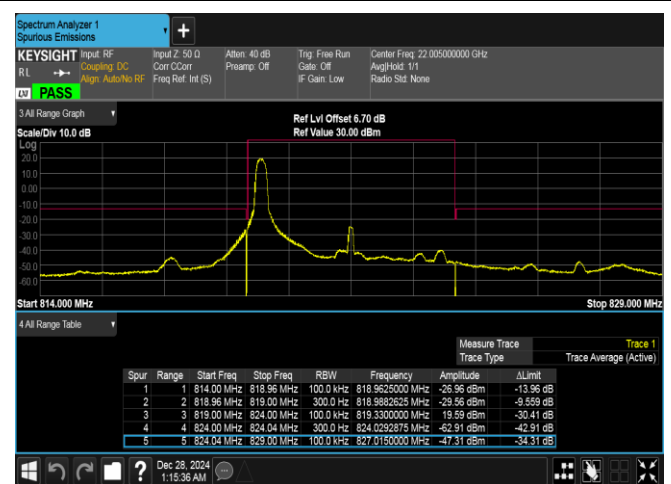
Band26(814-824)-5MHz-QPSK-26765-1RB#0-PASS
