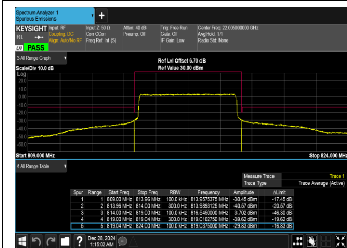
Band26(814-824)-5MHz-QPSK-26715-25RB#0-PASS
