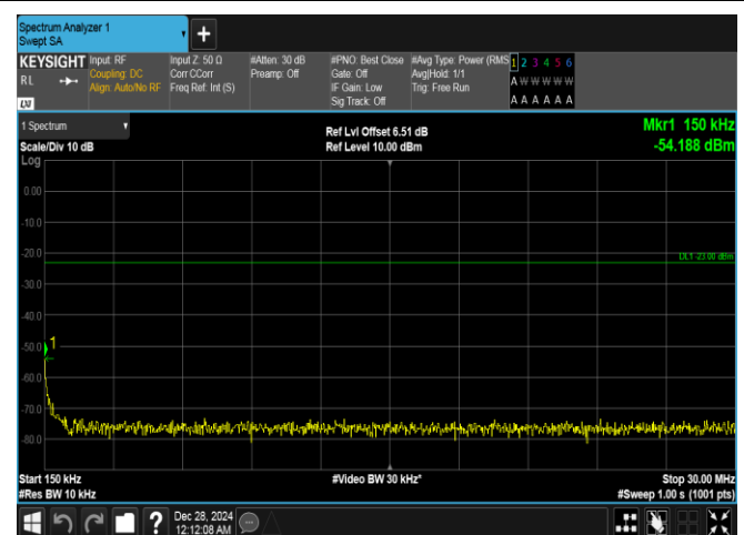
Band26(814-824)-1.4MHz-QPSK-26697-6RB#0-0.15~30-PASS
