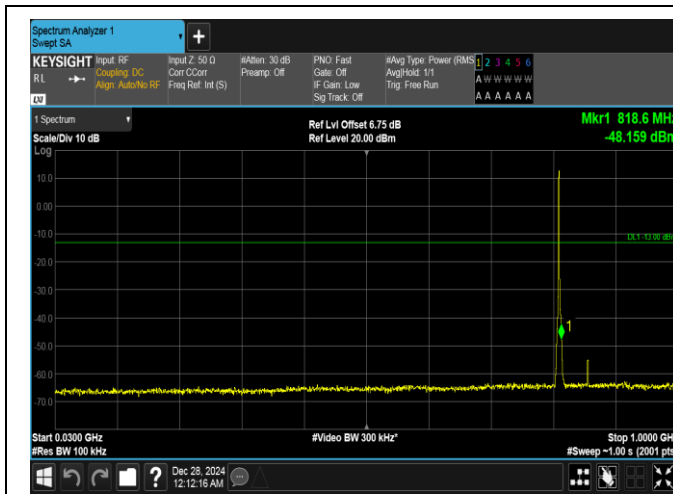
Band26(814-824)-1.4MHz-QPSK-26697-6RB#0-30~1000-PASS
