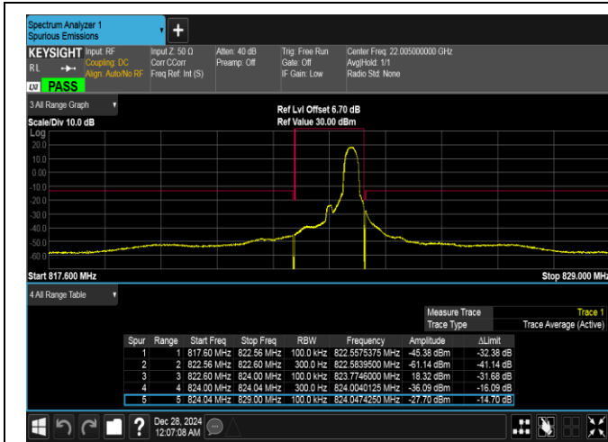
Band26(814-824)-1.4MHz-16QAM-26783-1RB#5-PASS
