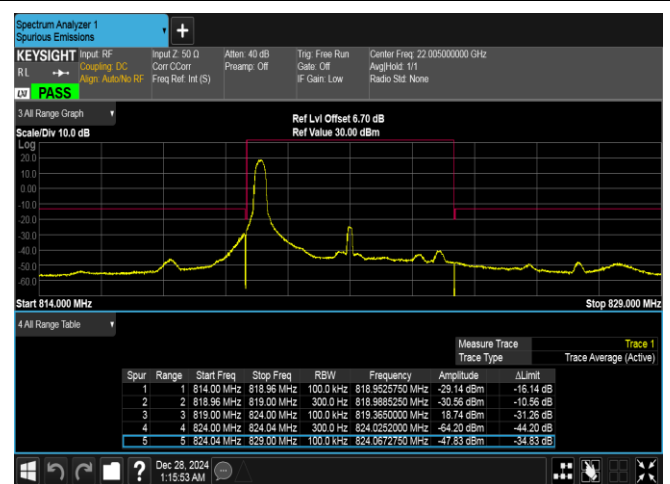
Band26(814-824)-5MHz-16QAM-26765-1RB#0-PASS
