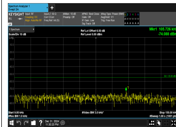
Band41(2535-2655)-20MHz-16QAM-40590-100RB#0-0.009~0.15-PASS
