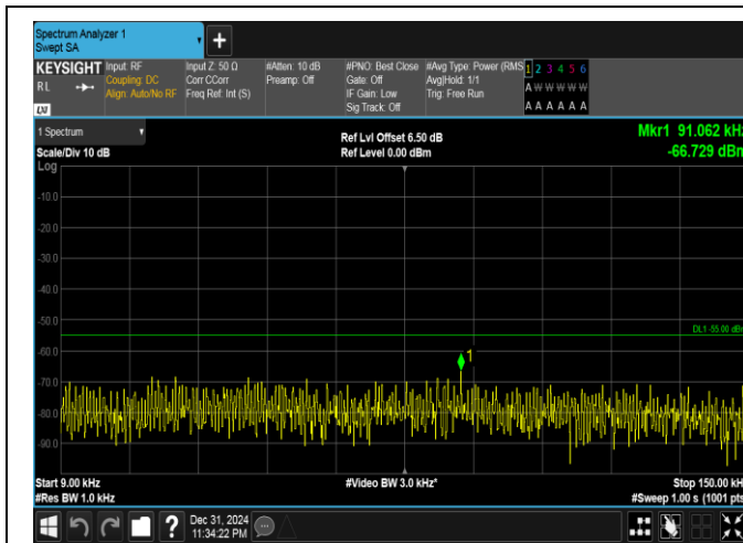
Band41(2535-2655)-20MHz-16QAM-41140-1RB#99-0.009~0.15-PASS
