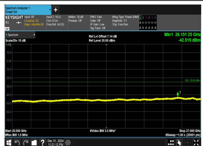
Band41(2535-2655)-20MHz-16QAM-40140-1RB#0-20000~27000-PASS
