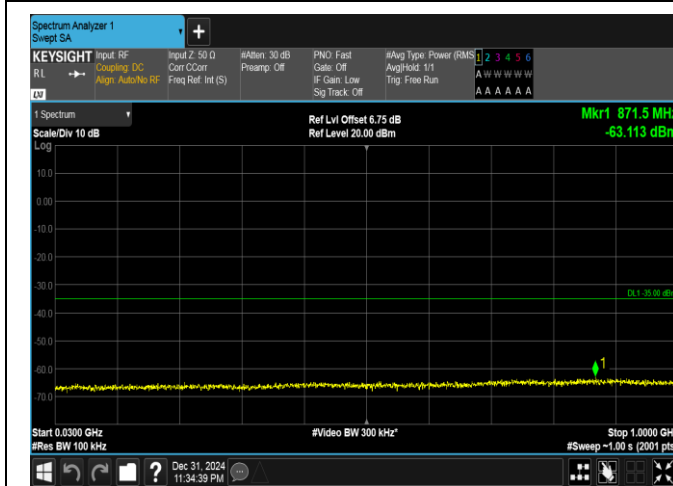
Band41(2535-2655)-20MHz-16QAM-41140-1RB#99-30~1000-PASS
