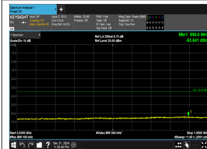
Band41(2535-2655)-20MHz-QPSK-41140-100RB#0-30~1000-PASS
