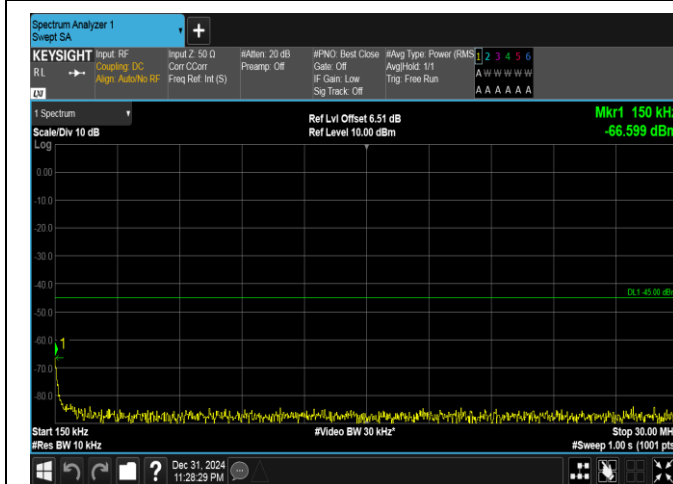
Band41(2535-2655)-20MHz-16QAM-40590-1RB#99-0.15~30-PASS
