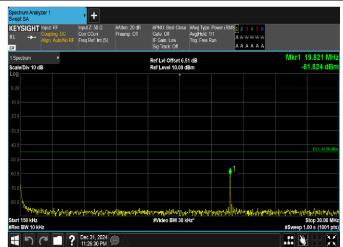
Band41(2535-2655)-20MHz-16QAM-40590-1RB#0-0.15~30-PASS
