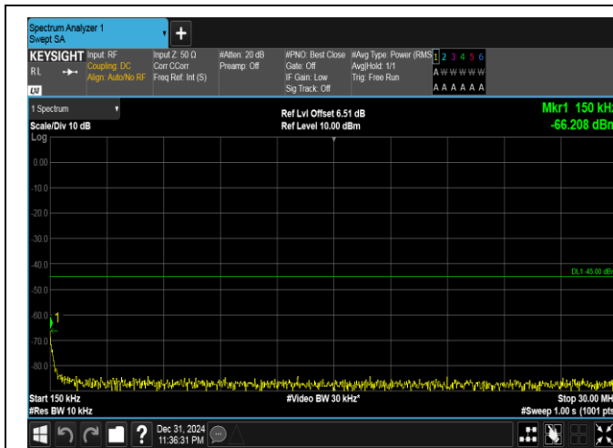
Band41(2535-2655)-20MHz-16QAM-41140-100RB#0-0.15~30-PASS
