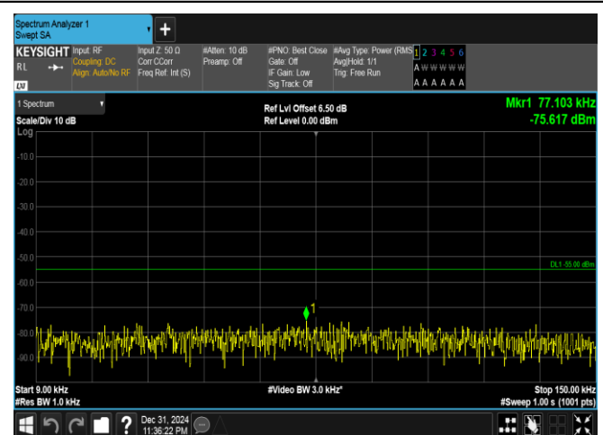
Band41(2535-2655)-20MHz-16QAM-41140-100RB#0-0.009~0.15-PASS
