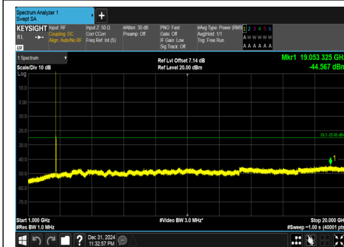
Band41(2535-2655)-20MHz-16QAM-41140-1RB#0-1000~20000-PASS
