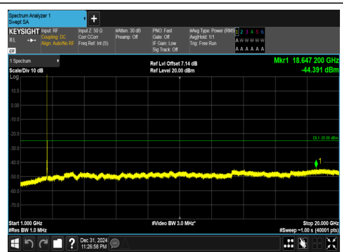
Band41(2535-2655)-20MHz-16QAM-40590-1RB#0-1000~20000-PASS
