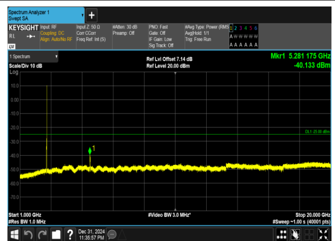
Band41(2535-2655)-20MHz-QPSK-41140-100RB#0-1000~20000-PASS
