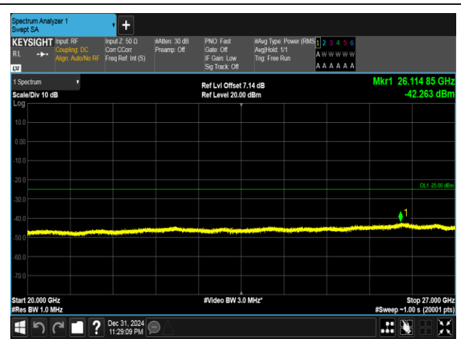
Band41(2535-2655)-20MHz-16QAM-40590-1RB#99-20000~27000-PASS
