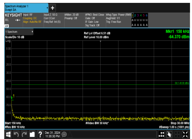
Band41(2535-2655)-20MHz-QPSK-41140-100RB#0-0.15~30-PASS
