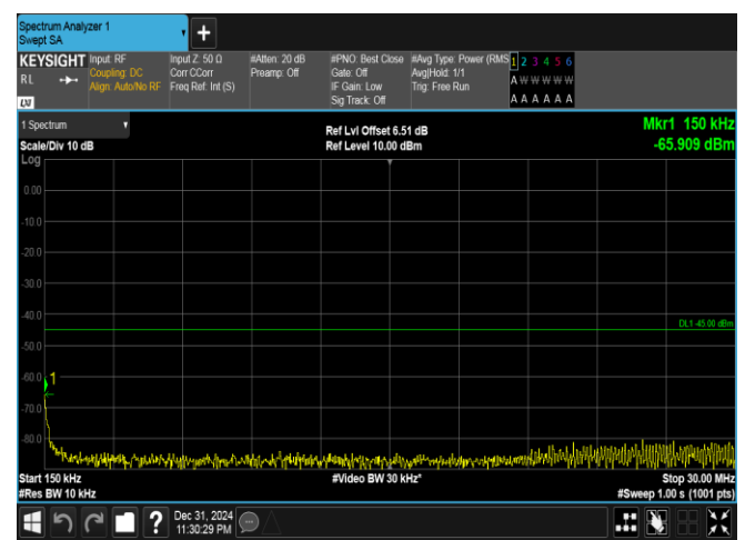
Band41(2535-2655)-20MHz-16QAM-40590-100RB#0-0.15~30-PASS
