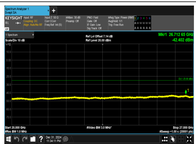
Band41(2535-2655)-20MHz-QPSK-41140-1RB#99-20000~27000-PASS
