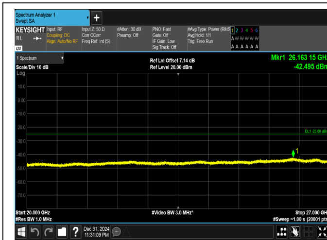
Band41(2535-2655)-20MHz-16QAM-40590-100RB#0-20000~27000-PASS
