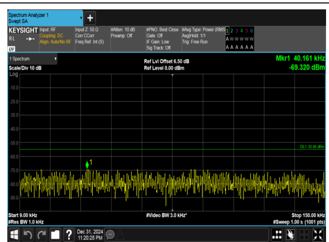
Band41(2535-2655)-20MHz-16QAM-40140-1RB#0-0.009~0.15-PASS
