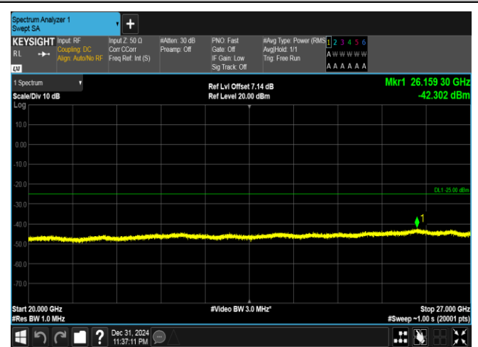
Band41(2535-2655)-20MHz-16QAM-41140-100RB#0-20000~27000-PASS
