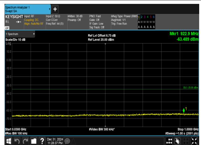
Band41(2535-2655)-20MHz-16QAM-40590-1RB#99-30~1000-PASS
