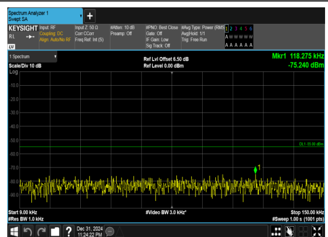
Band41(2535-2655)-20MHz-16QAM-40140-100RB#0-0.009~0.15-PASS
