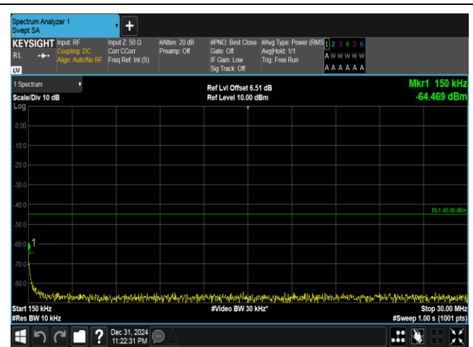
Band41(2535-2655)-20MHz-16QAM-40140-1RB#99-0.15~30-PASS
