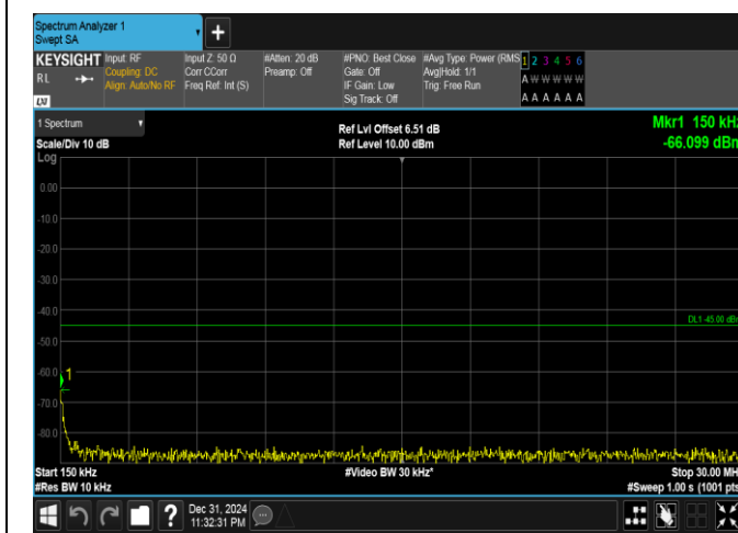
Band41(2535-2655)-20MHz-16QAM-41140-1RB#0-0.15~30-PASS
