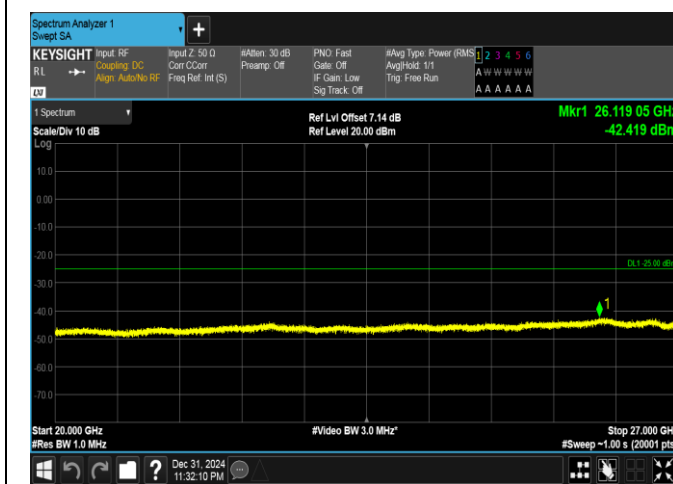
Band41(2535-2655)-20MHz-QPSK-41140-1RB#0-20000~27000-PASS
