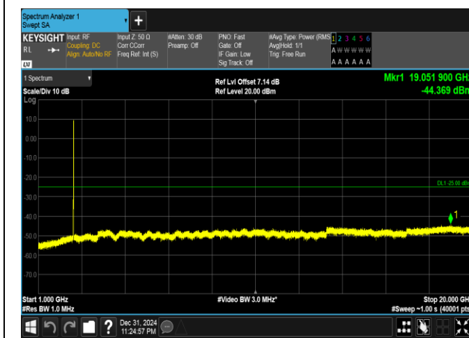
Band41(2535-2655)-20MHz-16QAM-40140-100RB#0-1000~20000-PASS
