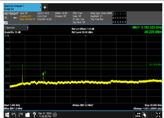
Band41(2535-2655)-20MHz-16QAM-40590-100RB#0-1000~20000-PASS
