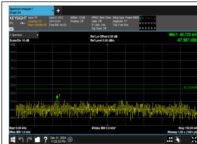
Band41(2535-2655)-20MHz-16QAM-40140-1RB#99-0.009~0.15-PASS
