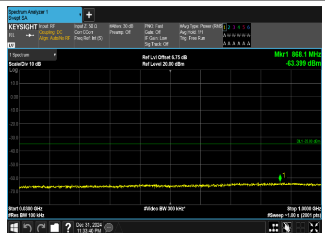
Band41(2535-2655)-20MHz-QPSK-41140-1RB#99-30~1000-PASS
