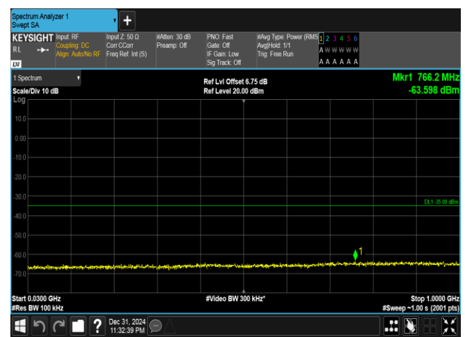
Band41(2535-2655)-20MHz-16QAM-41140-1RB#0-30~1000-PASS
