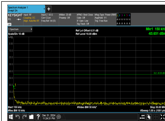
Band41(2535-2655)-20MHz-16QAM-40140-100RB#0-0.15~30-PASS
