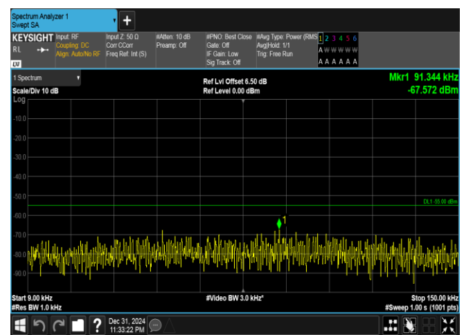
Band41(2535-2655)-20MHz-QPSK-41140-1RB#99-0.009~0.15-PASS
