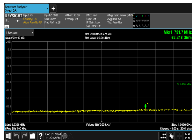
Band41(2535-2655)-20MHz-16QAM-40140-1RB#0-30~1000-PASS
