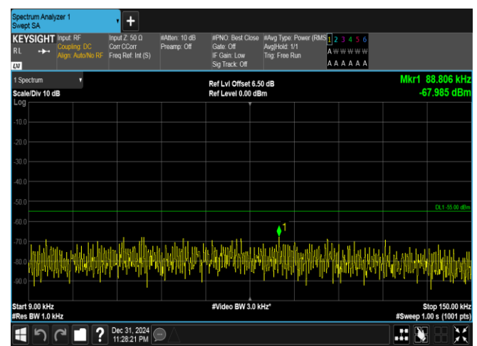
Band41(2535-2655)-20MHz-16QAM-40590-1RB#99-0.009~0.15-PASS
