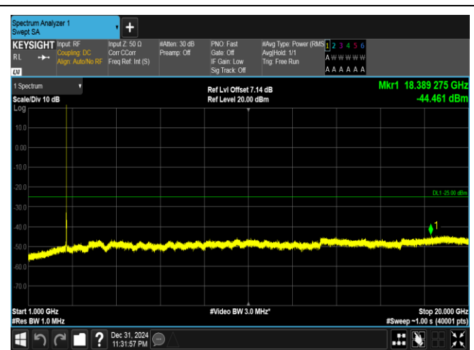
Band41(2535-2655)-20MHz-QPSK-41140-1RB#0-1000~20000-PASS
