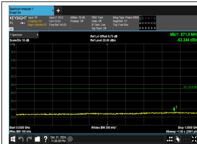
Band41(2535-2655)-20MHz-16QAM-40590-1RB#0-30~1000-PASS
