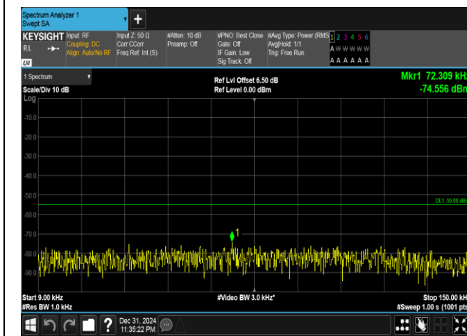
Band41(2535-2655)-20MHz-QPSK-41140-100RB#0-0.009~0.15-PASS
