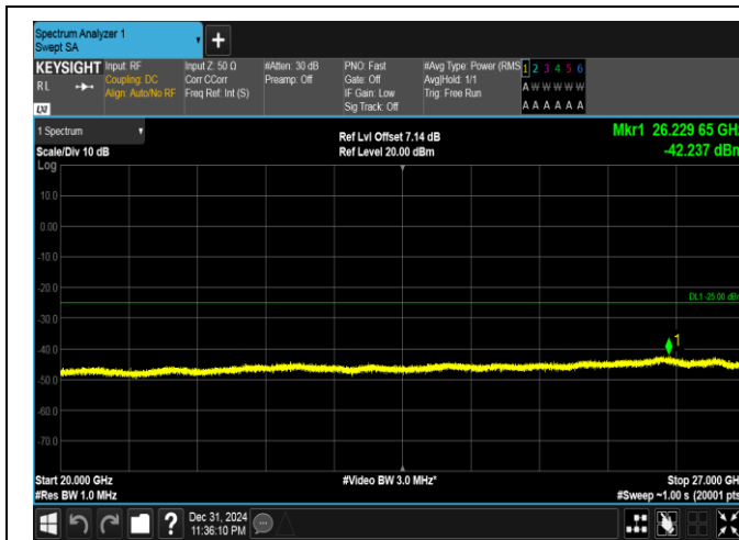
Band41(2535-2655)-20MHz-QPSK-41140-100RB#0-20000~27000-PASS
