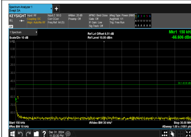
Band41(2535-2655)-20MHz-QPSK-41140-1RB#99-0.15~30-PASS
