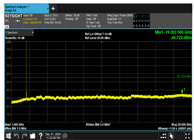
Band41(2535-2655)-20MHz-16QAM-40140-1RB#99-1000~20000-PASS
