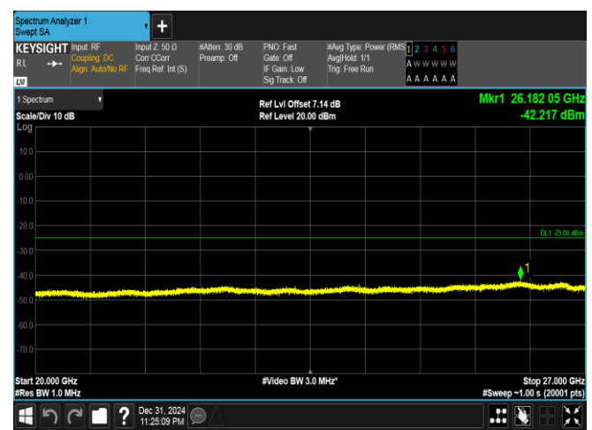
Band41(2535-2655)-20MHz-16QAM-40140-100RB#0-20000~27000-PASS
