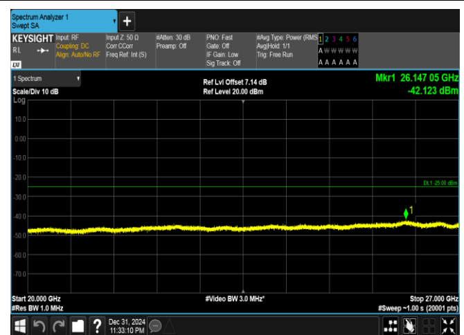
Band41(2535-2655)-20MHz-16QAM-41140-1RB#0-20000~27000-PASS
