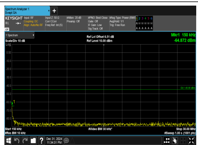
Band41(2535-2655)-20MHz-16QAM-41140-1RB#99-0.15~30-PASS
