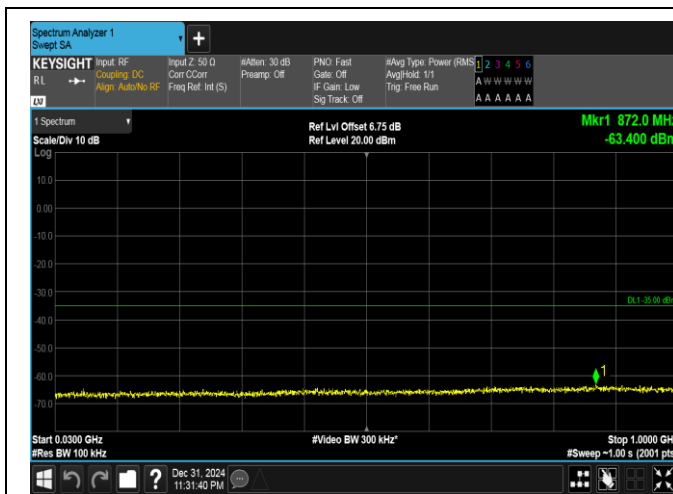
Band41(2535-2655)-20MHz-QPSK-41140-1RB#0-30~1000-PASS
