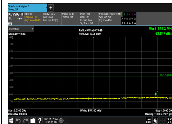
Band41(2535-2655)-20MHz-16QAM-40590-100RB#0-30~1000-PASS
