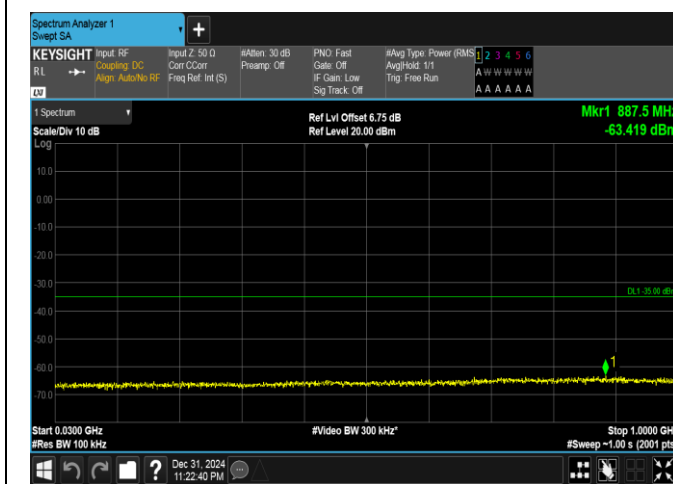
Band41(2535-2655)-20MHz-16QAM-40140-1RB#99-30~1000-PASS
