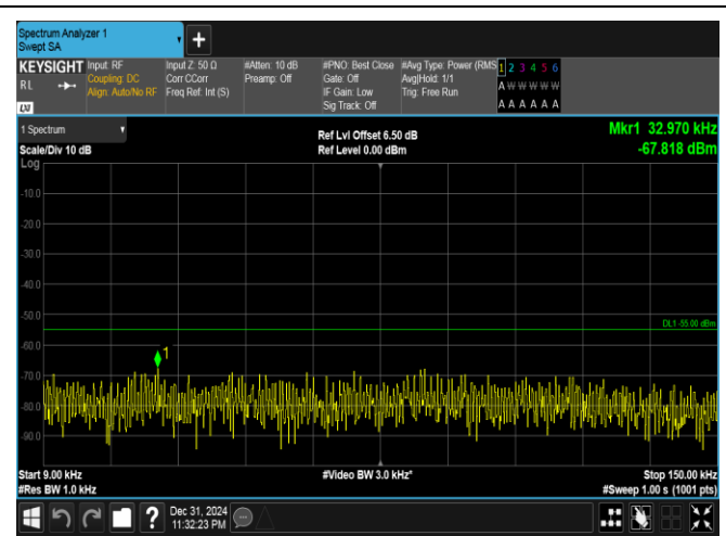
Band41(2535-2655)-20MHz-16QAM-41140-1RB#0-0.009~0.15-PASS
