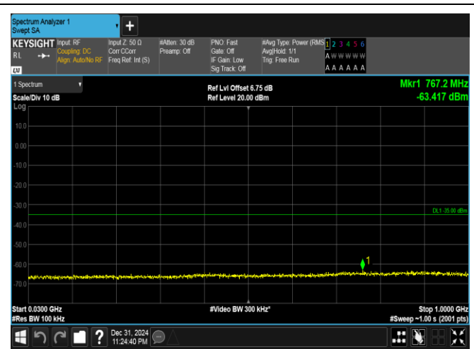
Band41(2535-2655)-20MHz-16QAM-40140-100RB#0-30~1000-PASS
