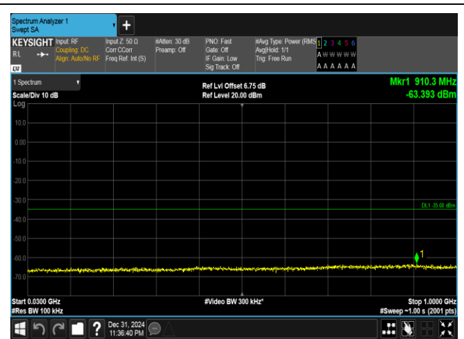
Band41(2535-2655)-20MHz-16QAM-41140-100RB#0-30~1000-PASS
