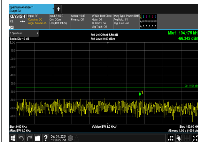
Band41(2535-2655)-20MHz-16QAM-40590-1RB#0-0.009~0.15-PASS
