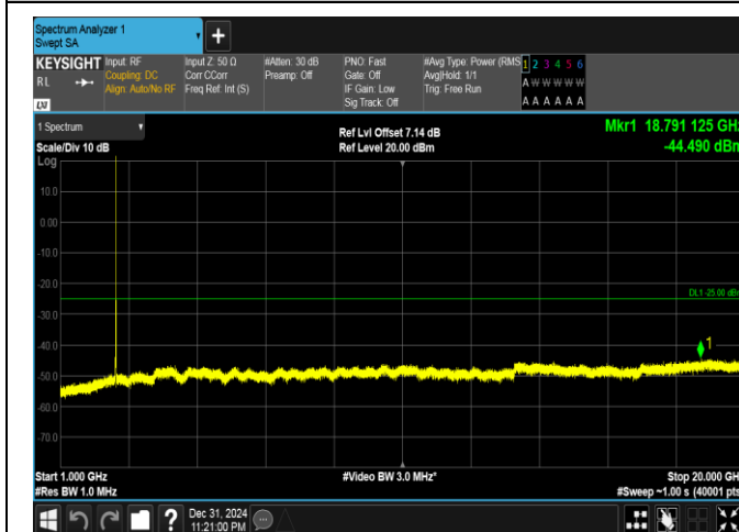
Band41(2535-2655)-20MHz-16QAM-40140-1RB#0-1000~20000-PASS
