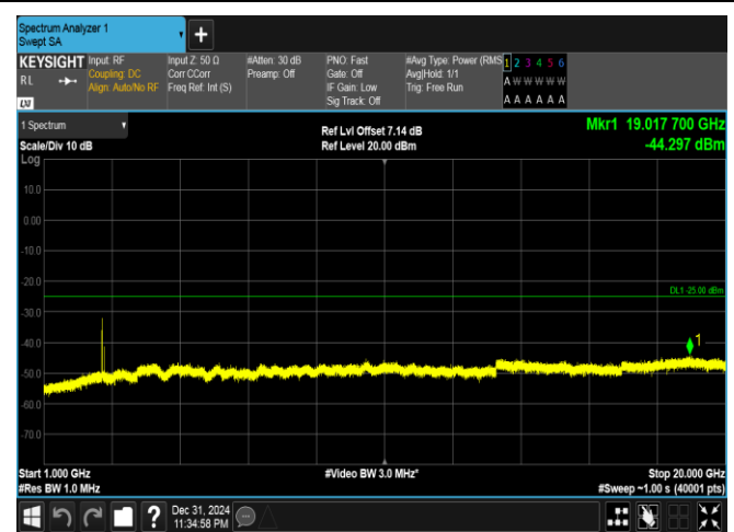
Band41(2535-2655)-20MHz-16QAM-41140-1RB#99-1000~20000-PASS
