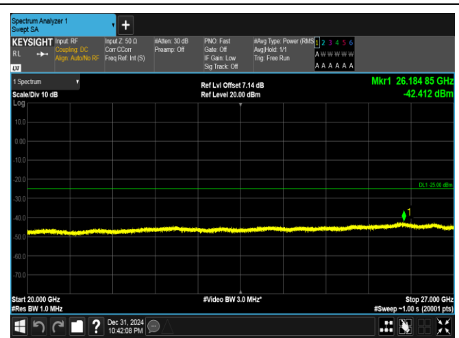
Band41(2535-2655)-15MHz-QPSK-41165-1RB#74-20000~27000-PASS
