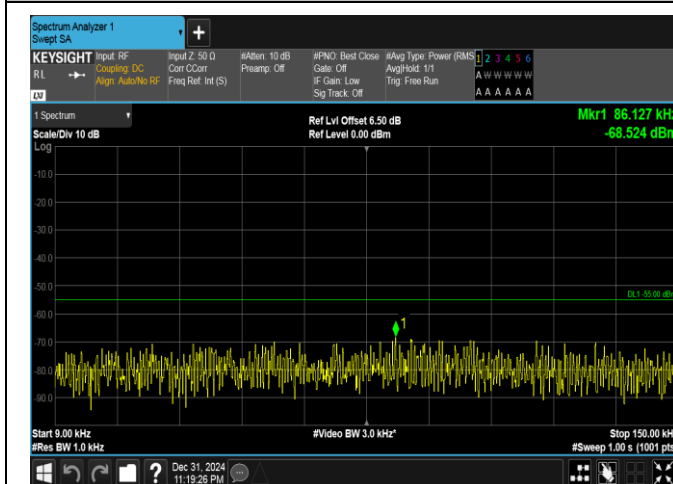
Band41(2535-2655)-20MHz-QPSK-40140-1RB#0-0.009~0.15-PASS
