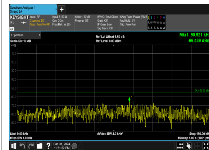
Band41(2535-2655)-20MHz-QPSK-41140-1RB#0-0.009~0.15-PASS
