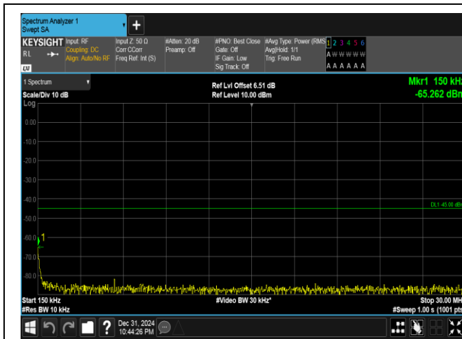
Band41(2535-2655)-15MHz-16QAM-41165-75RB#0-0.15~30-PASS
