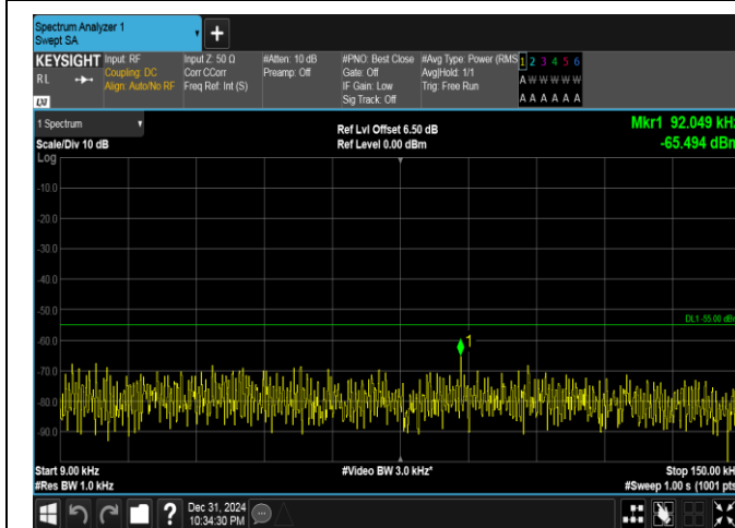
Band41(2535-2655)-15MHz-16QAM-40590-1RB#0-0.009~0.15-PASS
