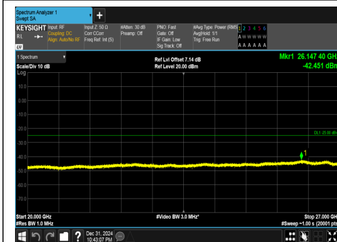
Band41(2535-2655)-15MHz-16QAM-41165-1RB#74-20000~27000-PASS
