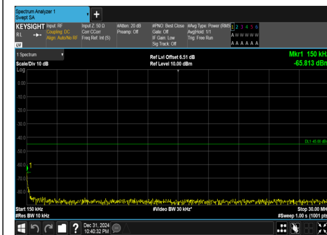
Band41(2535-2655)-15MHz-16QAM-41165-1RB#0-0.15~30-PASS
