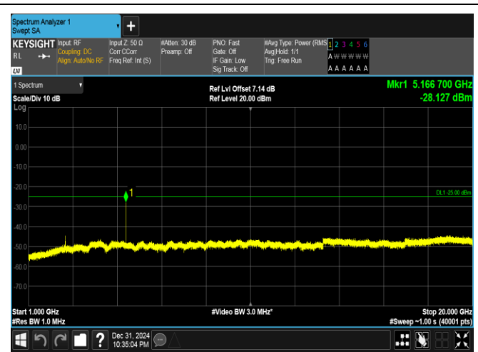
Band41(2535-2655)-15MHz-16QAM-40590-1RB#0-1000~20000-PASS
