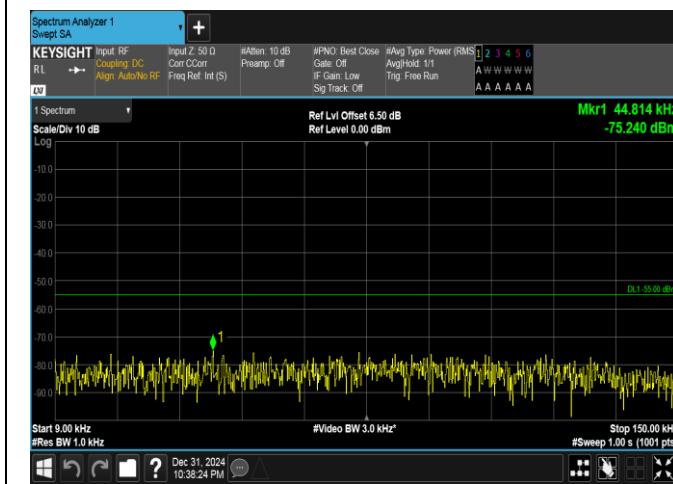
Band41(2535-2655)-15MHz-16QAM-40590-75RB#0-0.009~0.15-PASS
