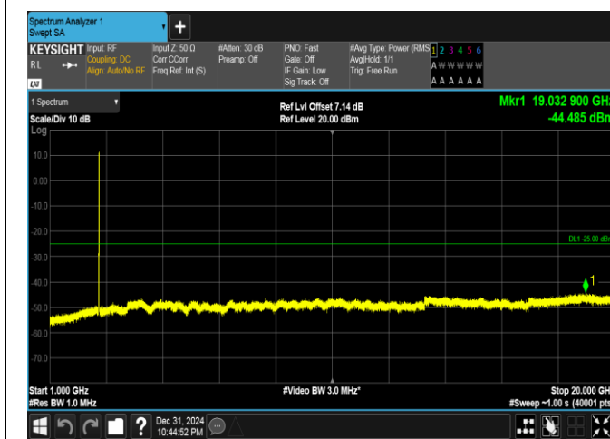
Band41(2535-2655)-15MHz-16QAM-41165-75RB#0-1000~20000-PASS
