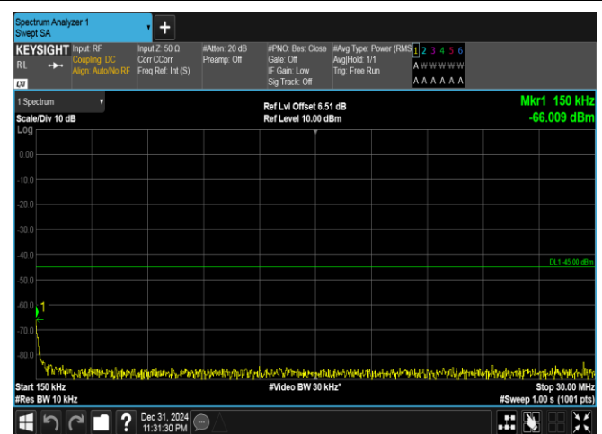
Band41(2535-2655)-20MHz-QPSK-41140-1RB#0-0.15~30-PASS
