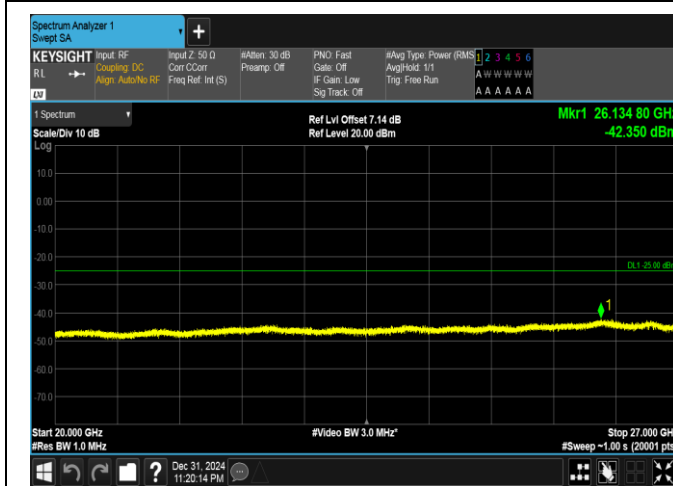
Band41(2535-2655)-20MHz-QPSK-40140-1RB#0-20000~27000-PASS
