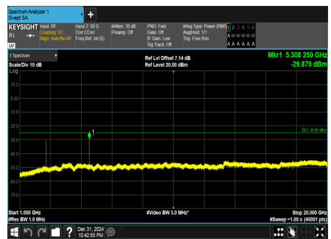
Band41(2535-2655)-15MHz-16QAM-41165-1RB#74-1000~20000-PASS
