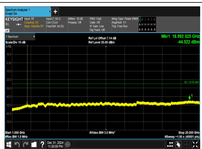
Band41(2535-2655)-20MHz-QPSK-40140-1RB#0-1000~20000-PASS
