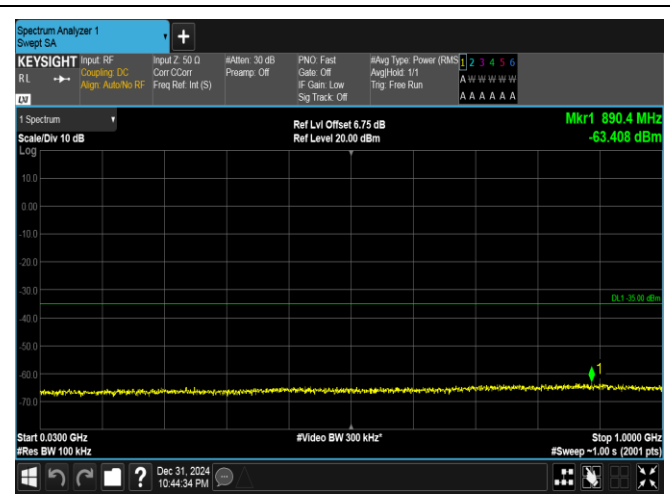
Band41(2535-2655)-15MHz-16QAM-41165-75RB#0-30~1000-PASS
