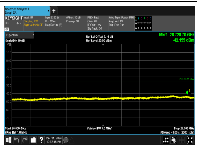
Band41(2535-2655)-15MHz-16QAM-40590-1RB#74-20000~27000-PASS
