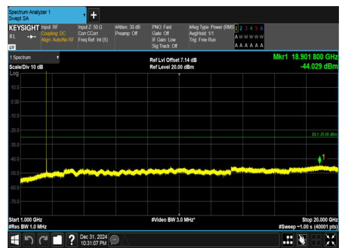
Band41(2535-2655)-15MHz-16QAM-40115-1RB#74-1000~20000-PASS
