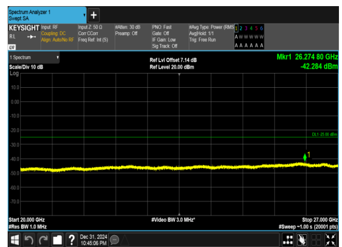
Band41(2535-2655)-15MHz-16QAM-41165-75RB#0-20000~27000-PASS
