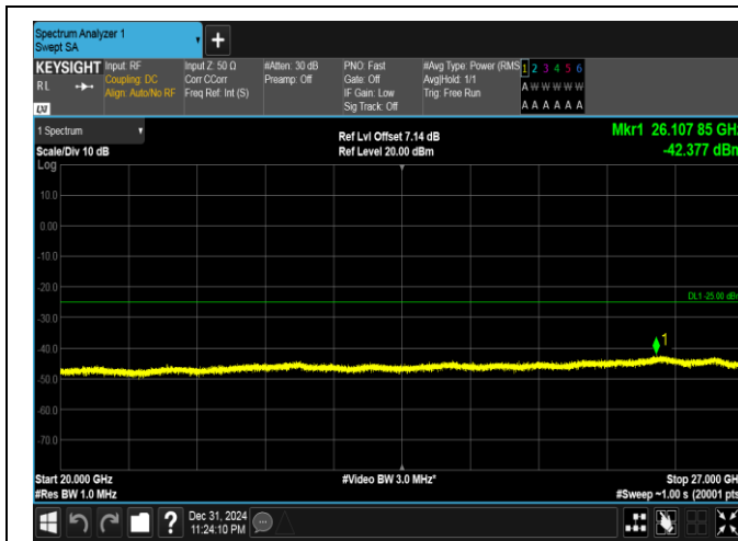
Band41(2535-2655)-20MHz-QPSK-40140-100RB#0-20000~27000-PASS
