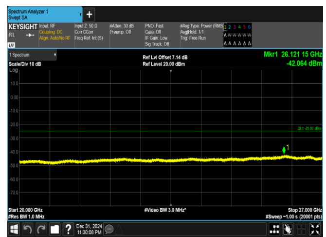
Band41(2535-2655)-20MHz-QPSK-40590-100RB#0-20000~27000-PASS
