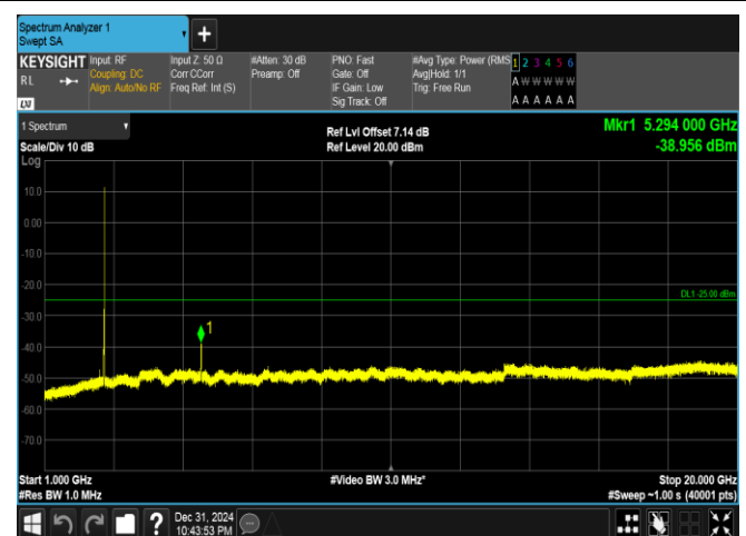
Band41(2535-2655)-15MHz-QPSK-41165-75RB#0-1000~20000-PASS
