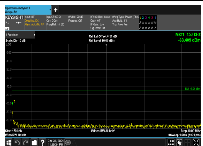
Band41(2535-2655)-20MHz-QPSK-40140-1RB#0-0.15~30-PASS
