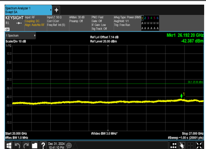
Band41(2535-2655)-15MHz-16QAM-41165-1RB#0-20000~27000-PASS
