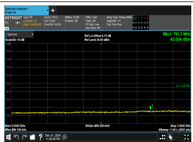
Band41(2535-2655)-20MHz-QPSK-40590-100RB#0-30~1000-PASS
