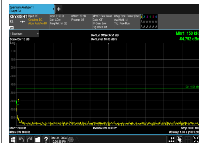
Band41(2535-2655)-15MHz-16QAM-40590-1RB#74-0.15~30-PASS
