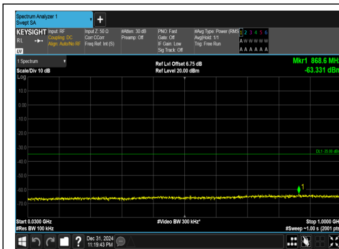
Band41(2535-2655)-20MHz-QPSK-40140-1RB#0-30~1000-PASS
