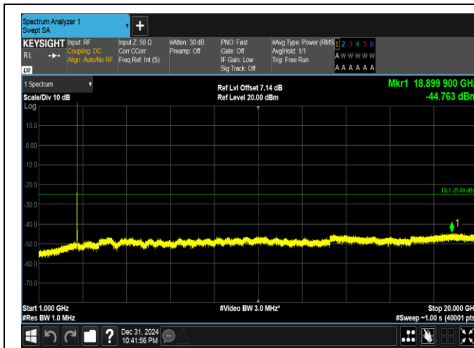
Band41(2535-2655)-15MHz-QPSK-41165-1RB#74-1000~20000-PASS
