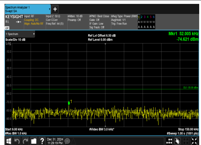
Band41(2535-2655)-20MHz-QPSK-40590-100RB#0-0.009~0.15-PASS
