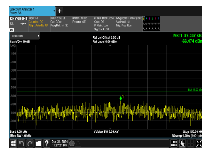
Band41(2535-2655)-20MHz-QPSK-40590-1RB#99-0.009~0.15-PASS
