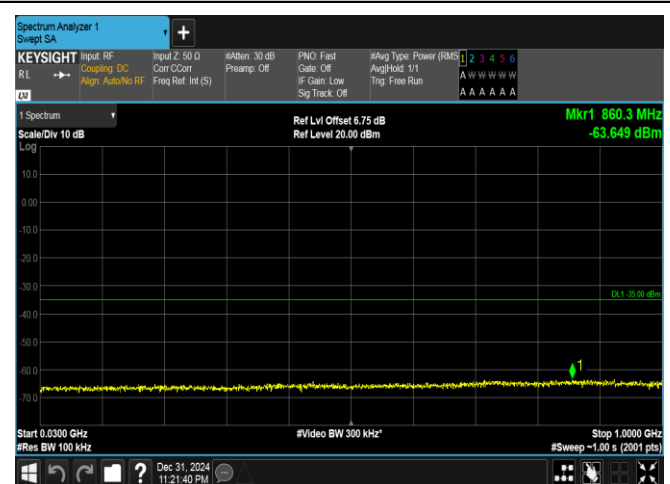
Band41(2535-2655)-20MHz-QPSK-40140-1RB#99-30~1000-PASS
