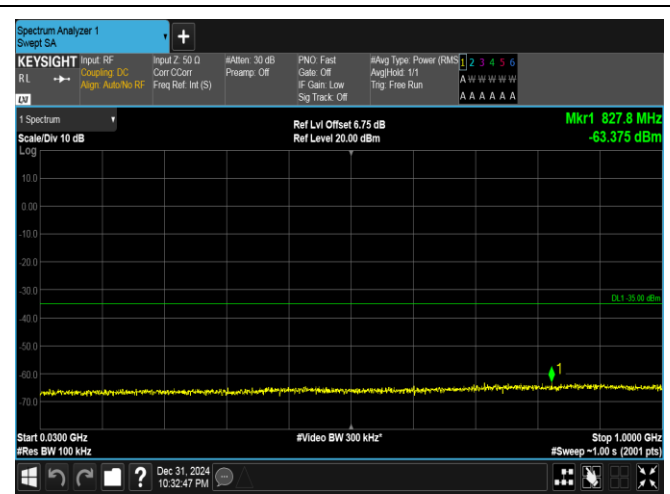
Band41(2535-2655)-15MHz-16QAM-40115-75RB#0-30~1000-PASS
