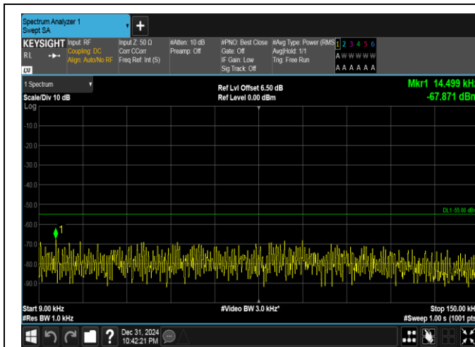
Band41(2535-2655)-15MHz-16QAM-41165-1RB#74-0.009~0.15-PASS
