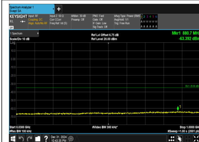
Band41(2535-2655)-15MHz-QPSK-41165-75RB#0-30~1000-PASS
