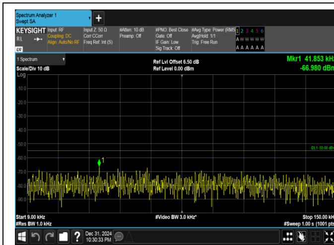
Band41(2535-2655)-15MHz-16QAM-40115-1RB#74-0.009~0.15-PASS
