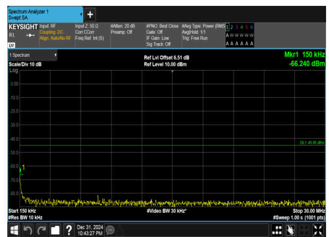
Band41(2535-2655)-15MHz-QPSK-41165-75RB#0-0.15~30-PASS
