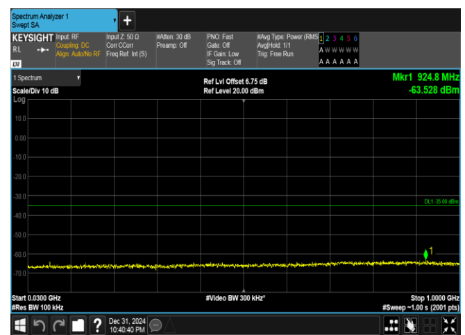
Band41(2535-2655)-15MHz-16QAM-41165-1RB#0-30~1000-PASS
