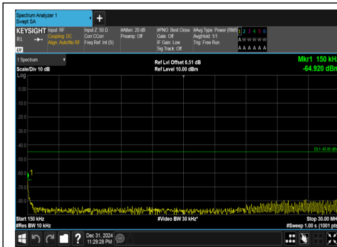
Band41(2535-2655)-20MHz-QPSK-40590-100RB#0-0.15~30-PASS
