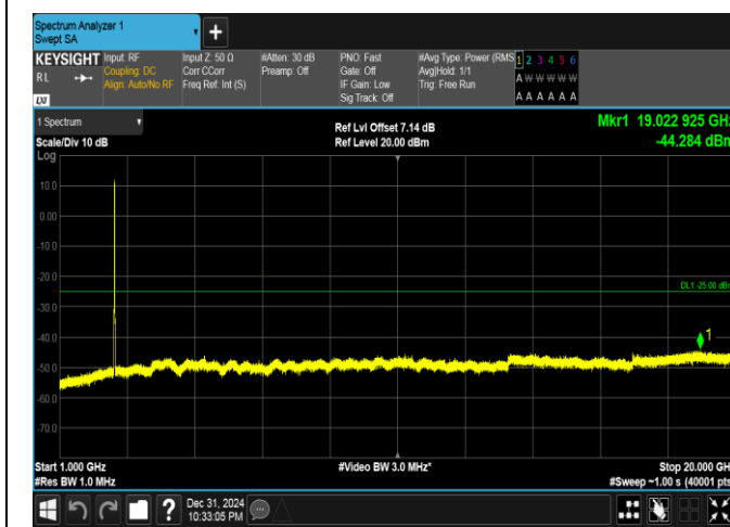
Band41(2535-2655)-15MHz-16QAM-40115-75RB#0-1000~20000-PASS
