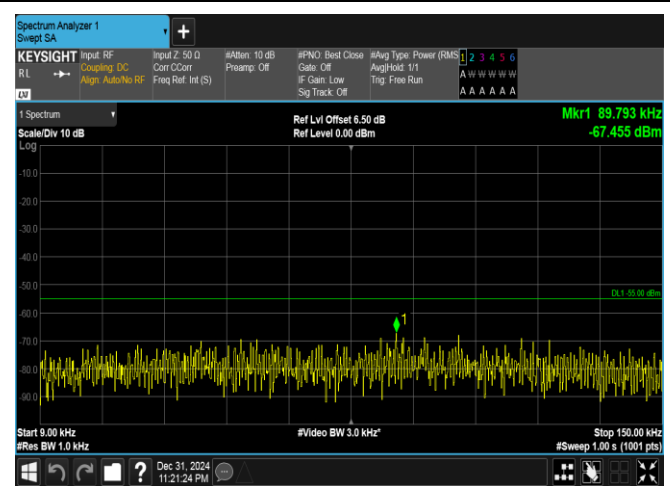
Band41(2535-2655)-20MHz-QPSK-40140-1RB#99-0.009~0.15-PASS
