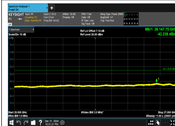
Band41(2535-2655)-15MHz-16QAM-40115-1RB#74-20000~27000-PASS
