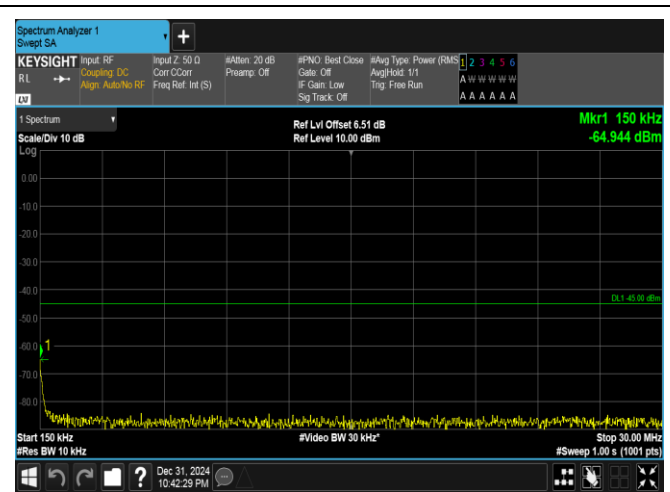
Band41(2535-2655)-15MHz-16QAM-41165-1RB#74-0.15~30-PASS
