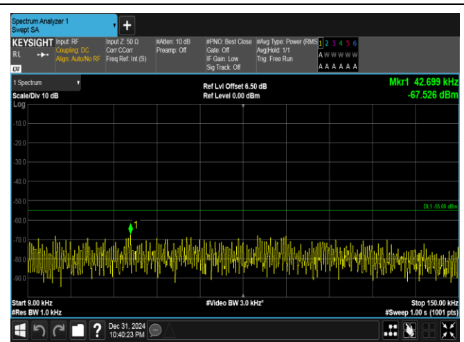
Band41(2535-2655)-15MHz-16QAM-41165-1RB#0-0.009~0.15-PASS
