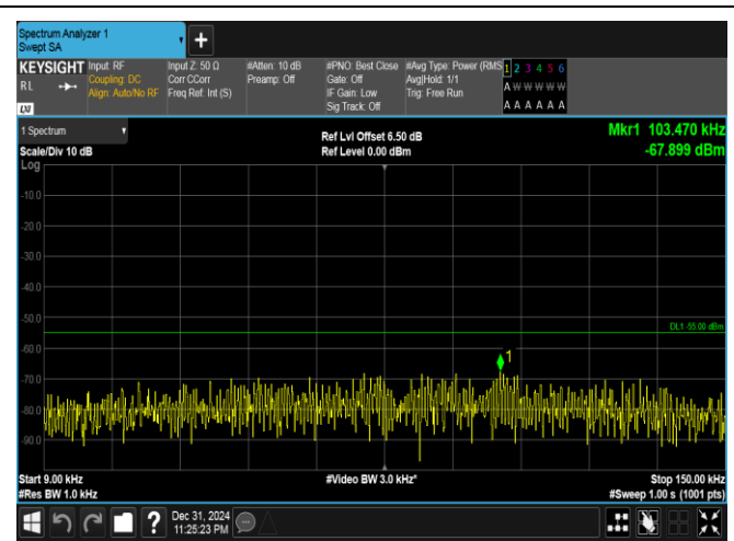
Band41(2535-2655)-20MHz-QPSK-40590-1RB#0-0.009~0.15-PASS
