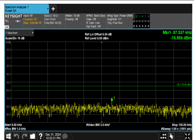
Band41(2535-2655)-15MHz-16QAM-40115-75RB#0-0.009~0.15-PASS
