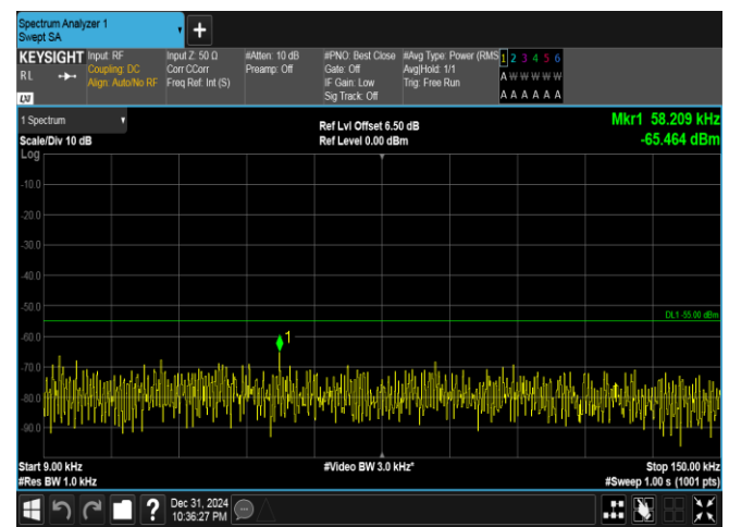
Band41(2535-2655)-15MHz-16QAM-40590-1RB#74-0.009~0.15-PASS
