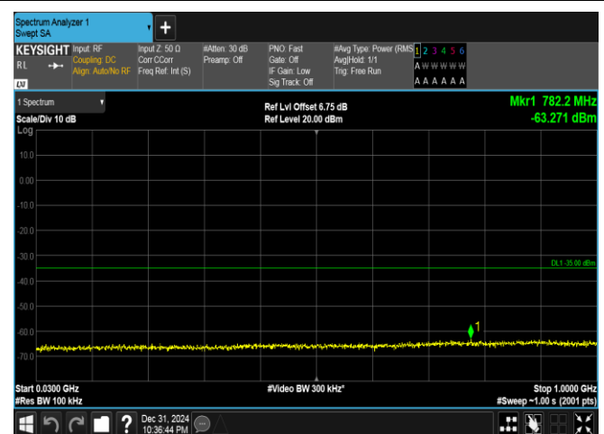
Band41(2535-2655)-15MHz-16QAM-40590-1RB#74-30~1000-PASS
