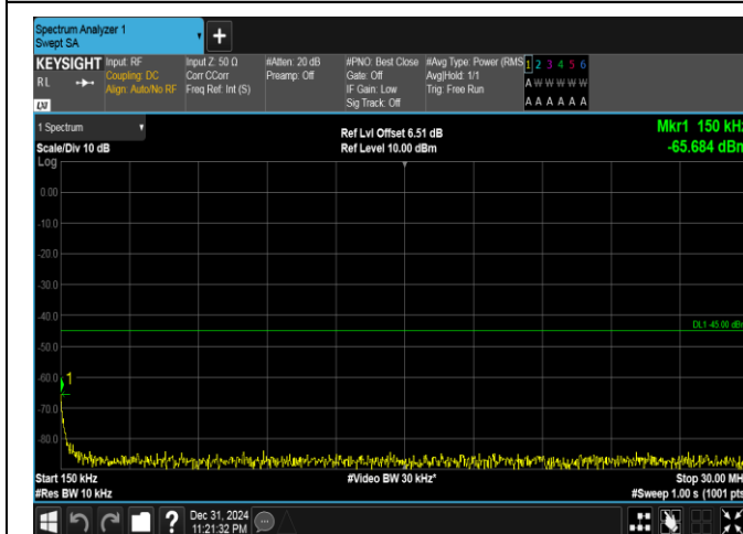
Band41(2535-2655)-20MHz-QPSK-40140-1RB#99-0.15~30-PASS
