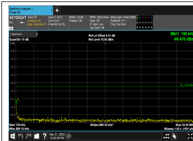
Band41(2535-2655)-15MHz-16QAM-40115-75RB#0-0.15~30-PASS
