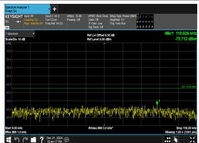
Band41(2535-2655)-15MHz-16QAM-41165-75RB#0-0.009~0.15-PASS
