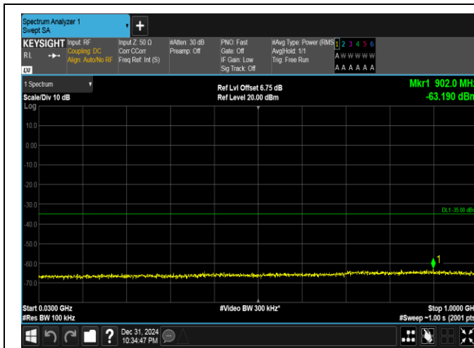
Band41(2535-2655)-15MHz-16QAM-40590-1RB#0-30~1000-PASS
