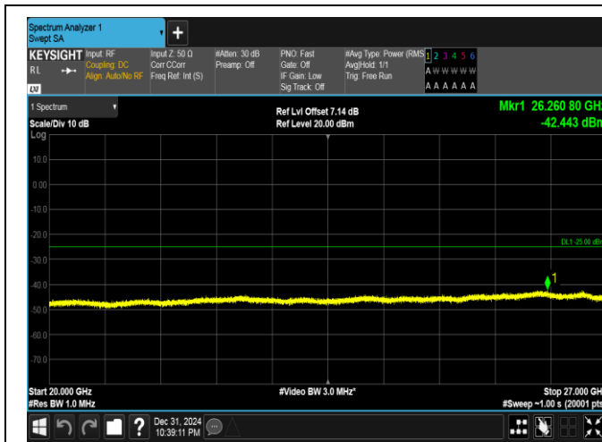
Band41(2535-2655)-15MHz-16QAM-40590-75RB#0-20000~27000-PASS
