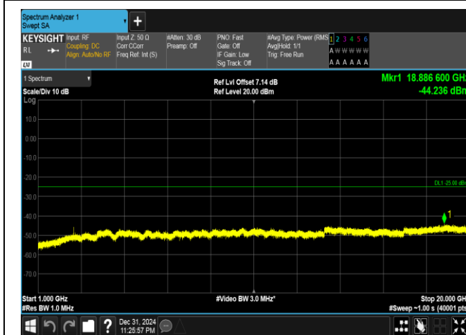
Band41(2535-2655)-20MHz-QPSK-40590-1RB#0-1000~20000-PASS
