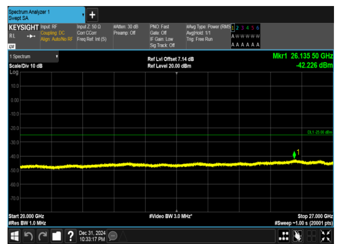
Band41(2535-2655)-15MHz-16QAM-40115-75RB#0-20000~27000-PASS
