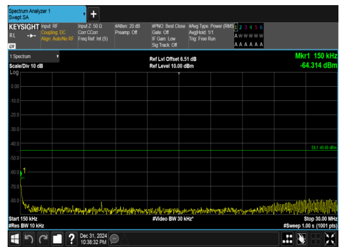
Band41(2535-2655)-15MHz-16QAM-40590-75RB#0-0.15~30-PASS
