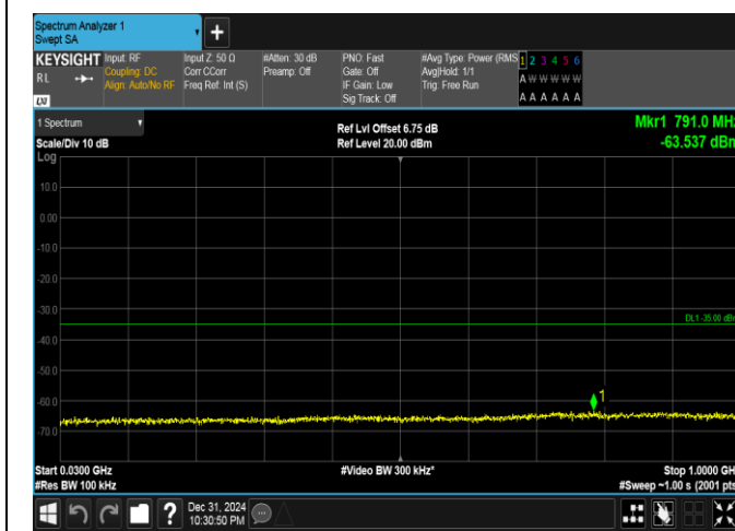
Band41(2535-2655)-15MHz-16QAM-40115-1RB#74-30~1000-PASS
