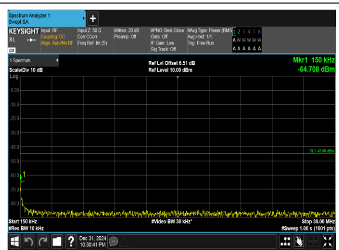
Band41(2535-2655)-15MHz-16QAM-40115-1RB#74-0.15~30-PASS
