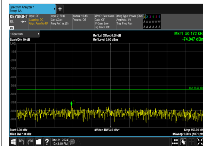
Band41(2535-2655)-15MHz-QPSK-41165-75RB#0-0.009~0.15-PASS
