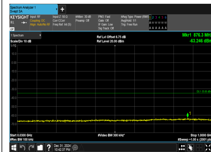
Band41(2535-2655)-15MHz-16QAM-41165-1RB#74-30~1000-PASS
