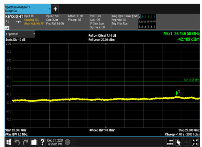
Band38-10MHz-16QAM-38200-50RB#0-20000~27000-PASS
