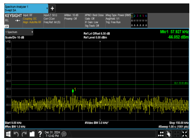
Band38-15MHz-QPSK-38175-1RB#74-0.009~0.15-PASS
