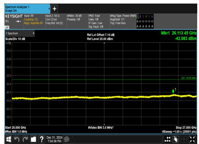
Band38-15MHz-16QAM-37825-75RB#0-20000~27000-PASS
