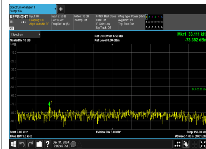
Band38-15MHz-16QAM-38000-75RB#0-0.009~0.15-PASS
