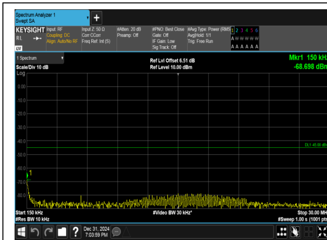
Band38-15MHz-16QAM-37825-75RB#0-0.15~30-PASS
