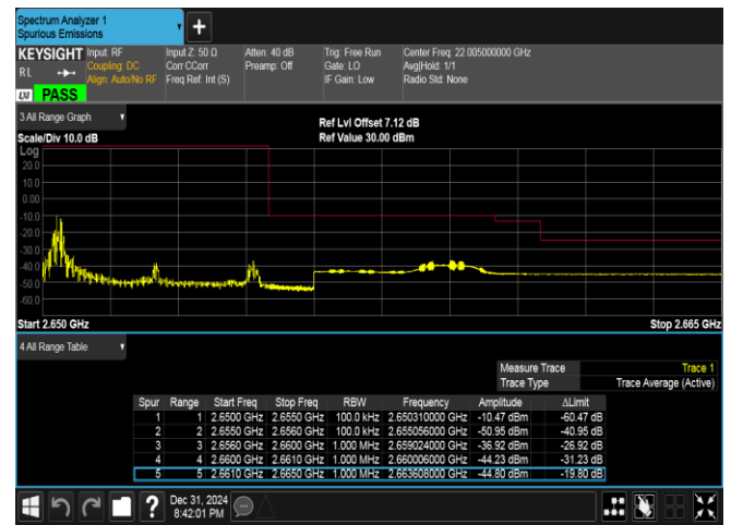
Band41(2535-2655)-5MHz-16QAM-41215-1RB#0-PASS
