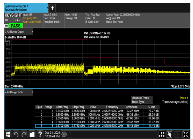
Band41(2535-2655)-15MHz-QPSK-41165-75RB#0-PASS
