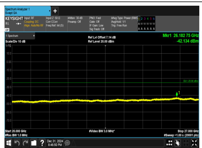
Band41(2535-2655)-5MHz-QPSK-40065-1RB#24-20000~27000-PASS
