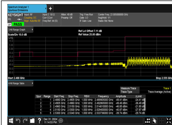
Band41(2535-2655)-20MHz-QPSK-40140-100RB#0-PASS
