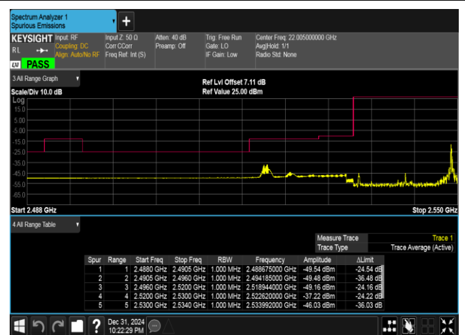
Band41(2535-2655)-15MHz-16QAM-40115-1RB#74-PASS
