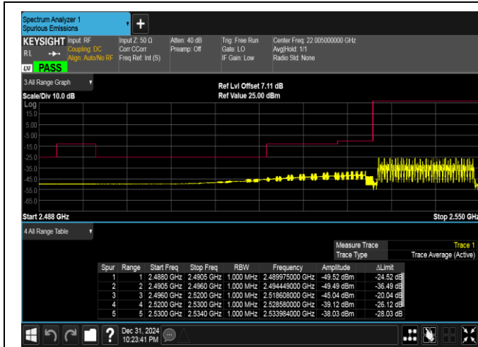
Band41(2535-2655)-15MHz-16QAM-40115-75RB#0-PASS
