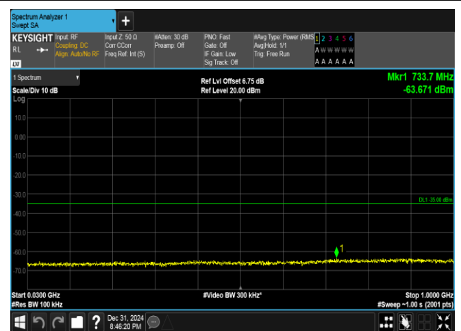
Band41(2535-2655)-5MHz-QPSK-40065-1RB#24-30~1000-PASS
