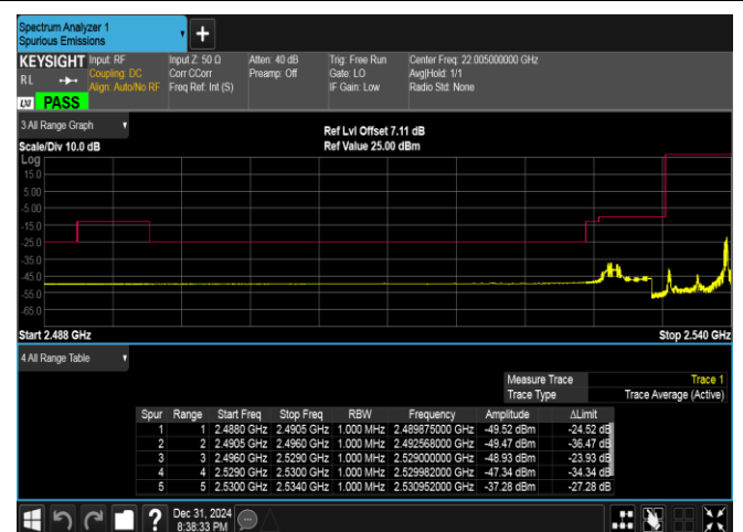
Band41(2535-2655)-5MHz-16QAM-40065-1RB#24-PASS
