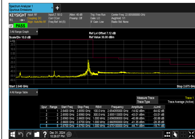
Band41(2535-2655)-15MHz-16QAM-41165-1RB#74-PASS
