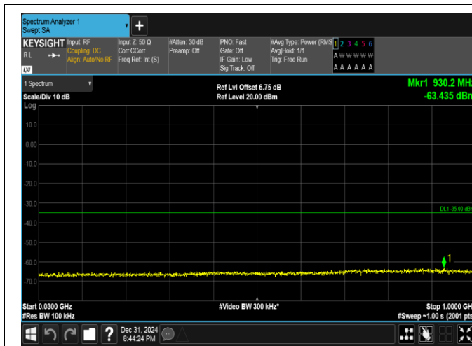
Band41(2535-2655)-5MHz-QPSK-40065-1RB#0-30~1000-PASS
