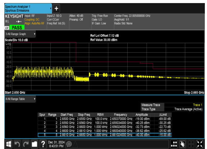
Band41(2535-2655)-5MHz-16QAM-41215-25RB#0-PASS
