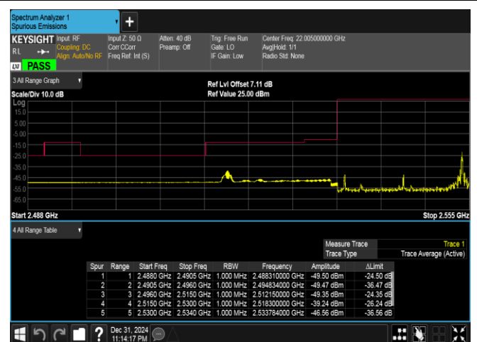
Band41(2535-2655)-20MHz-16QAM-40140-1RB#99-PASS
