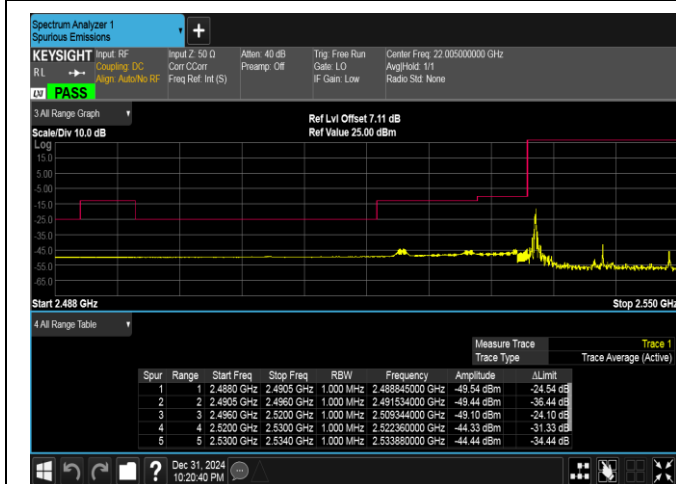
Band41(2535-2655)-15MHz-QPSK-40115-1RB#0-PASS
