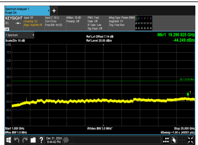
Band41(2535-2655)-5MHz-QPSK-40065-1RB#0-1000~20000-PASS
