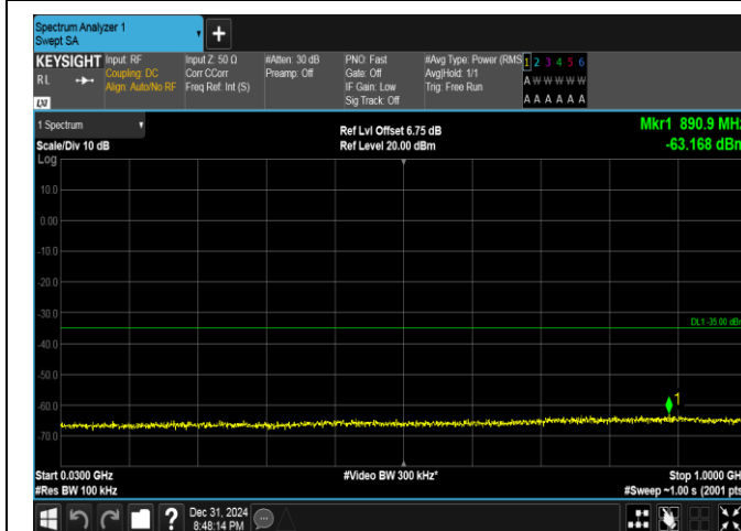
Band41(2535-2655)-5MHz-QPSK-40065-25RB#0-30~1000-PASS
