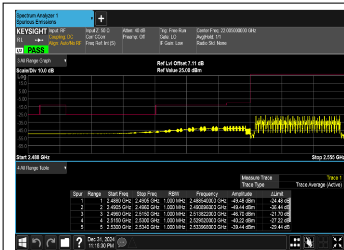
Band41(2535-2655)-20MHz-16QAM-40140-100RB#0-PASS
