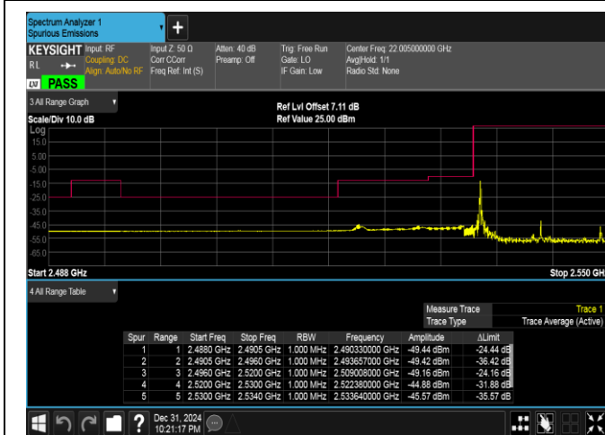
Band41(2535-2655)-15MHz-16QAM-40115-1RB#0-PASS
