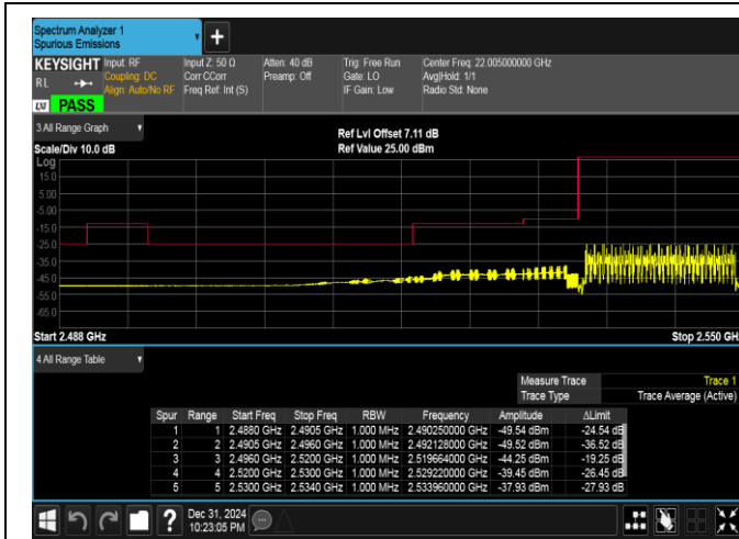
Band41(2535-2655)-15MHz-QPSK-40115-75RB#0-PASS
