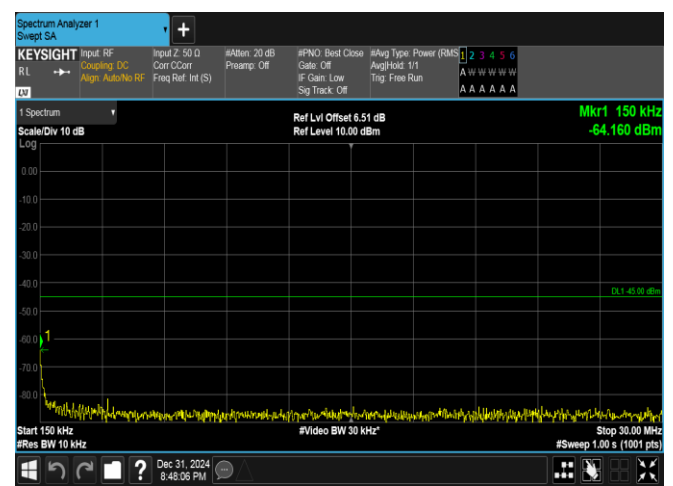
Band41(2535-2655)-5MHz-QPSK-40065-25RB#0-0.15~30-PASS
