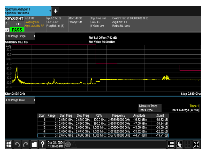
Band41(2535-2655)-20MHz-16QAM-41140-1RB#0-PASS
