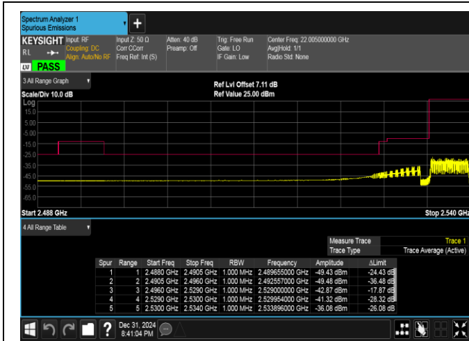
Band41(2535-2655)-5MHz-16QAM-40065-25RB#0-PASS
