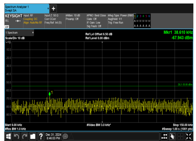
Band41(2535-2655)-5MHz-QPSK-40065-1RB#24-0.009~0.15-PASS
