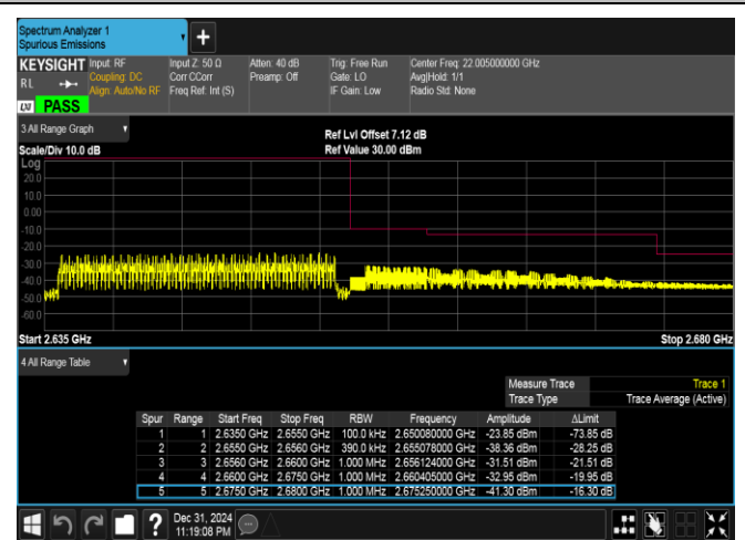
Band41(2535-2655)-20MHz-16QAM-41140-100RB#0-PASS
