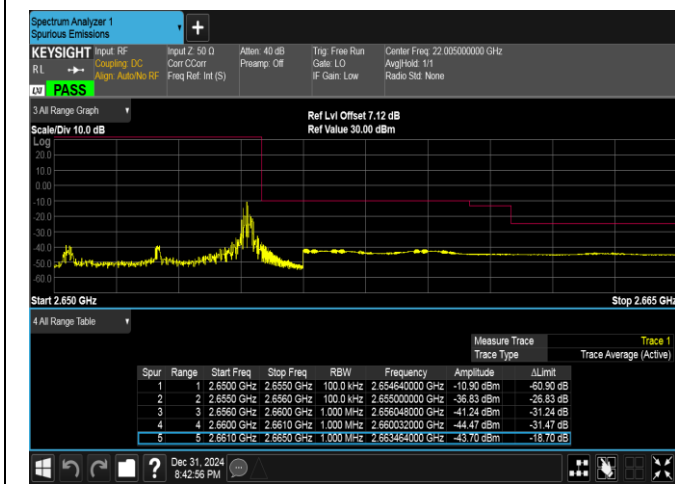
Band41(2535-2655)-5MHz-16QAM-41215-1RB#24-PASS
