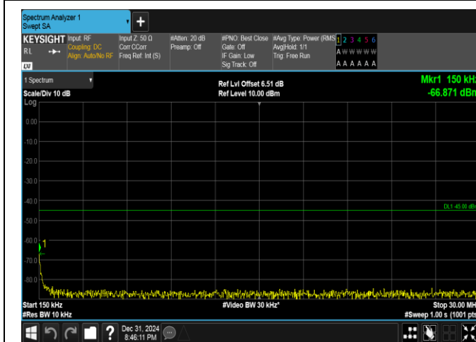
Band41(2535-2655)-5MHz-QPSK-40065-1RB#24-0.15~30-PASS
