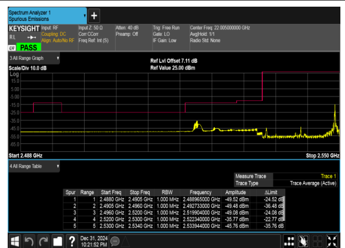
Band41(2535-2655)-15MHz-QPSK-40115-1RB#74-PASS
