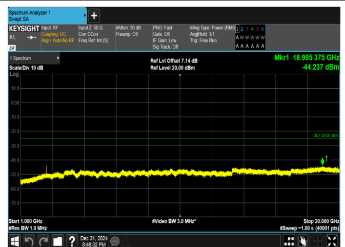
Band41(2535-2655)-5MHz-QPSK-40065-25RB#0-1000~20000-PASS
