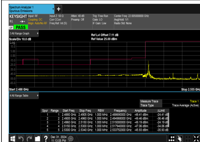
Band41(2535-2655)-20MHz-16QAM-40140-1RB#0-PASS
