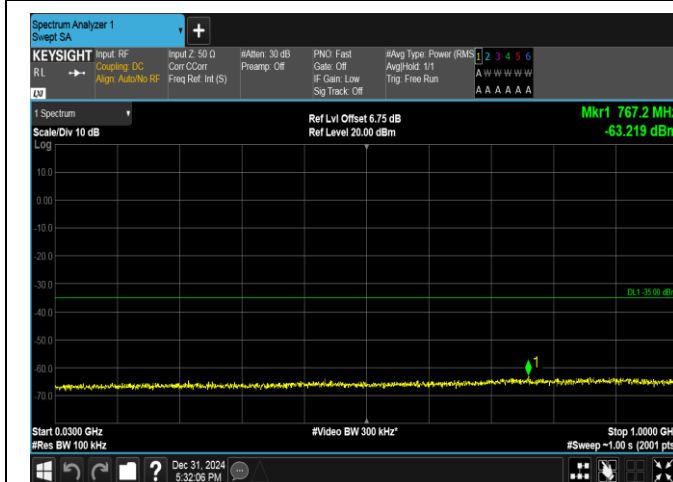
Band38-5MHz-QPSK-38225-25RB#0-30~1000-PASS
