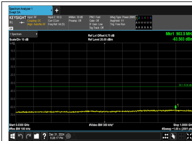
Band38-5MHz-QPSK-38225-1RB#0-30~1000-PASS
