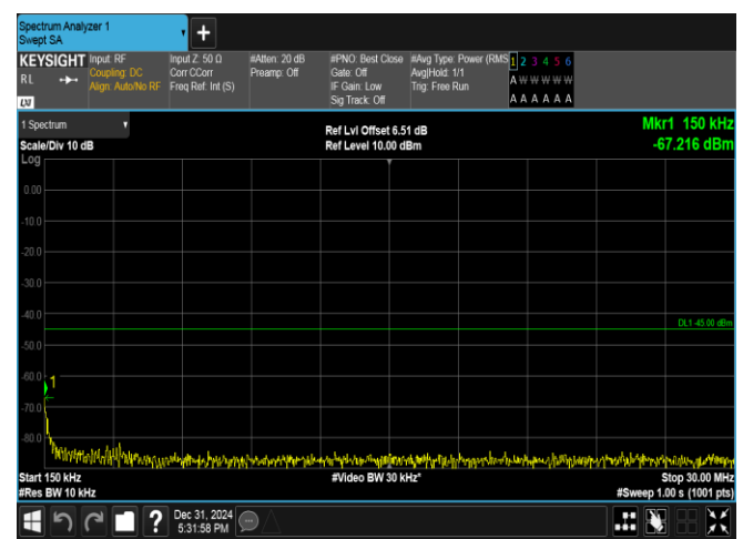
Band38-5MHz-QPSK-38225-25RB#0-0.15~30-PASS
