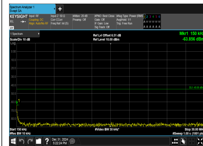
Band38-5MHz-QPSK-38000-1RB#0-0.15~30-PASS
