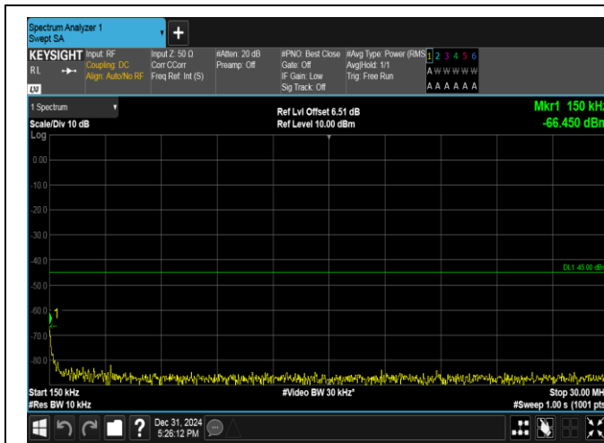
Band38-5MHz-QPSK-38000-25RB#0-0.15~30-PASS
