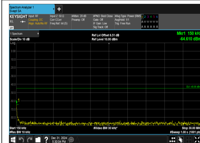
Band38-5MHz-QPSK-38225-1RB#24-0.15~30-PASS
