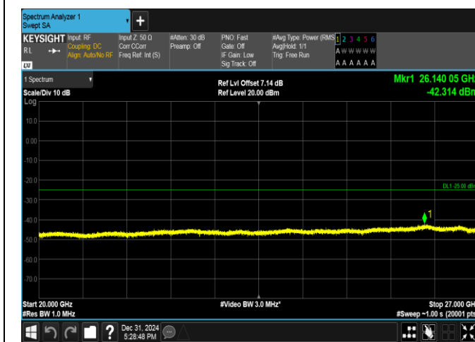
Band38-5MHz-QPSK-38225-1RB#0-20000~27000-PASS
