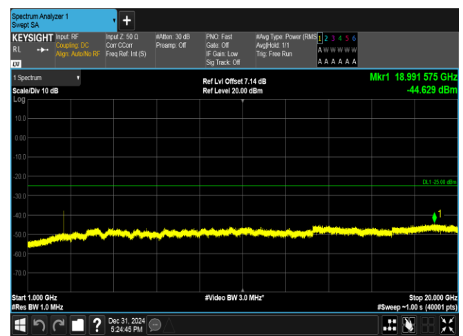
Band38-5MHz-QPSK-38000-1RB#24-1000~20000-PASS
