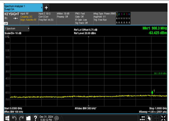
Band38-5MHz-QPSK-38225-1RB#24-30~1000-PASS
