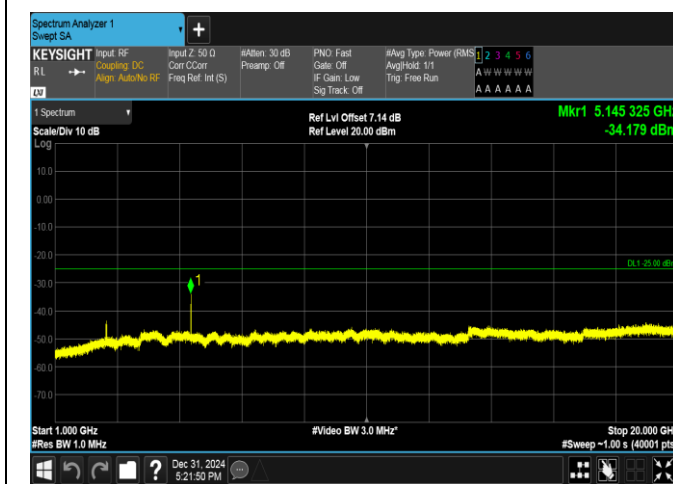
Band38-5MHz-16QAM-37775-25RB#0-1000~20000-PASS
