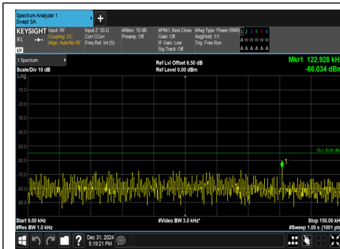
Band38-5MHz-16QAM-37775-1RB#24-0.009~0.15-PASS
