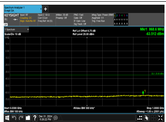
Band38-5MHz-QPSK-38000-25RB#0-30~1000-PASS
