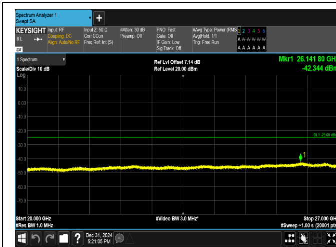
Band38-5MHz-QPSK-37775-25RB#0-20000~27000-PASS
