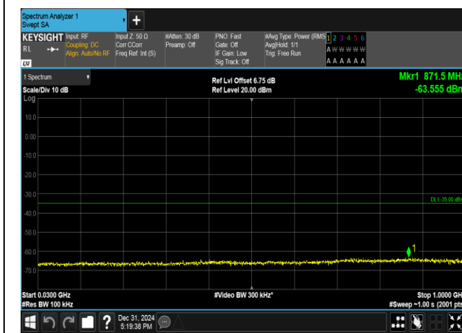
Band38-5MHz-16QAM-37775-1RB#24-30~1000-PASS
