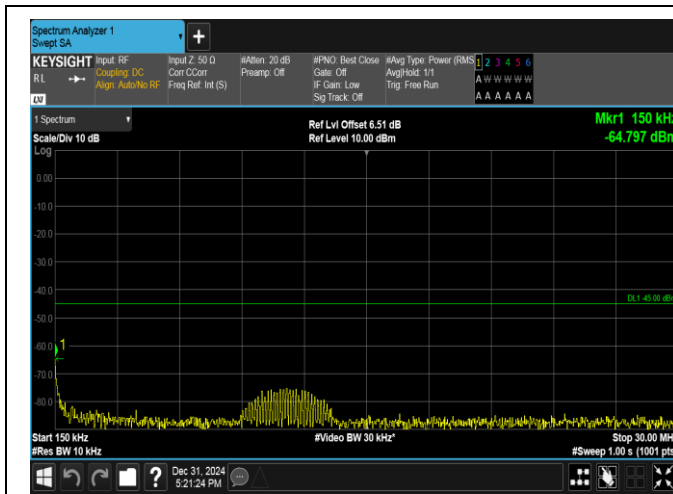
Band38-5MHz-16QAM-37775-25RB#0-0.15~30-PASS
