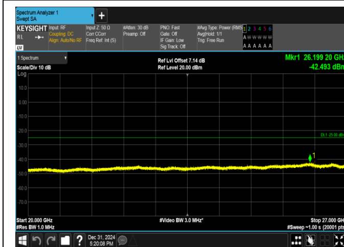
Band38-5MHz-16QAM-37775-1RB#24-20000~27000-PASS
