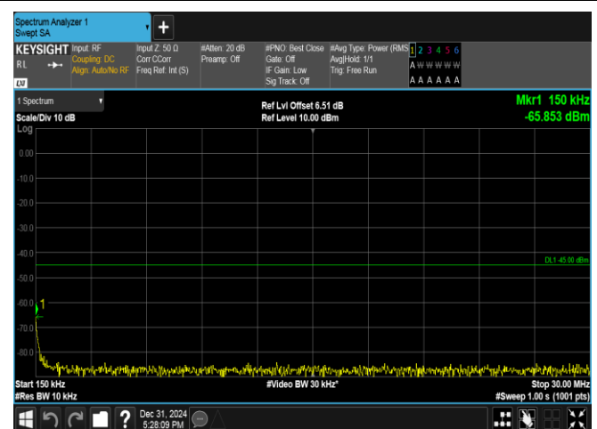
Band38-5MHz-QPSK-38225-1RB#0-0.15~30-PASS
