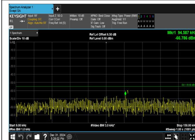
Band38-5MHz-QPSK-38225-1RB#0-0.009~0.15-PASS
