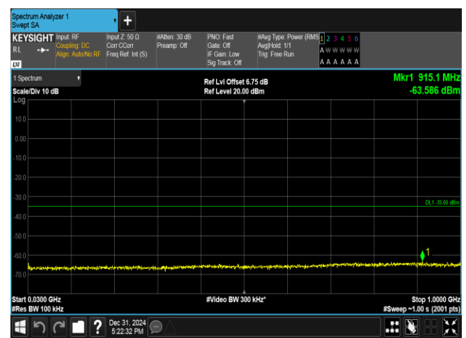
Band38-5MHz-QPSK-38000-1RB#0-30~1000-PASS
