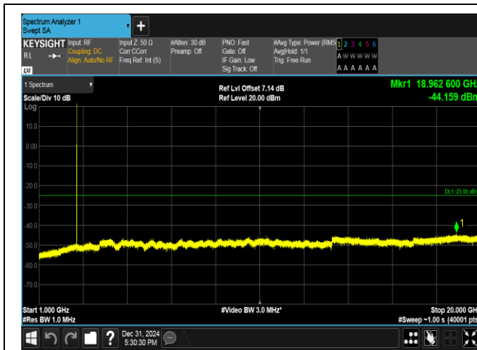
Band38-5MHz-QPSK-38225-1RB#24-1000~20000-PASS
