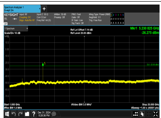
Band38-5MHz-QPSK-38225-1RB#0-1000~20000-PASS
