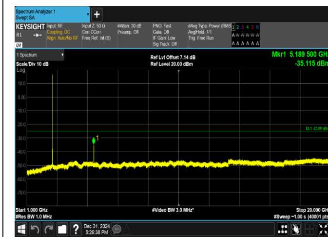
Band38-5MHz-QPSK-38000-25RB#0-1000~20000-PASS
