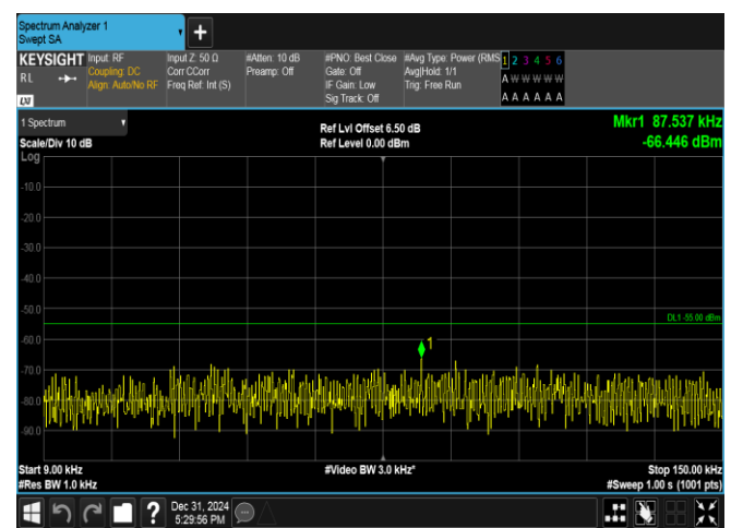
Band38-5MHz-QPSK-38225-1RB#24-0.009~0.15-PASS
