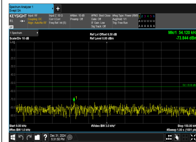
Band38-5MHz-QPSK-38225-25RB#0-0.009~0.15-PASS
