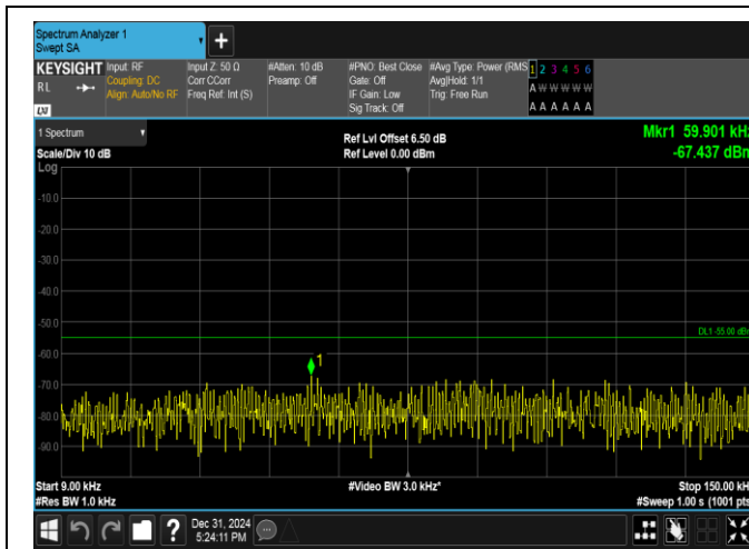
Band38-5MHz-QPSK-38000-1RB#24-0.009~0.15-PASS
