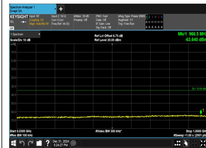
Band38-5MHz-QPSK-38000-1RB#24-30~1000-PASS
