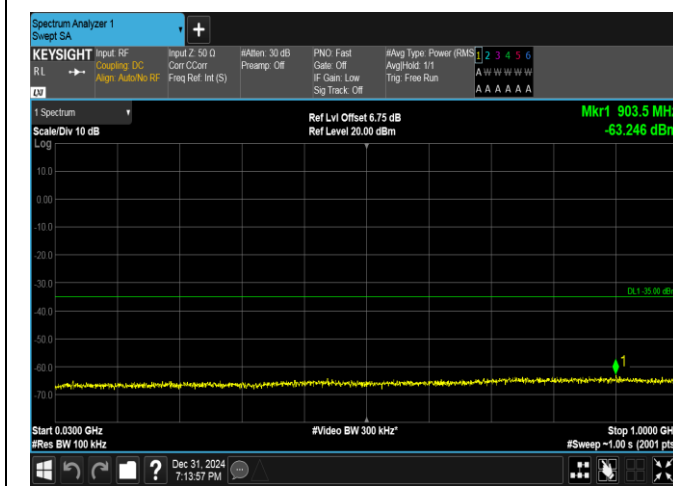
Band38-15MHz-16QAM-38175-1RB#74-30~1000-PASS
