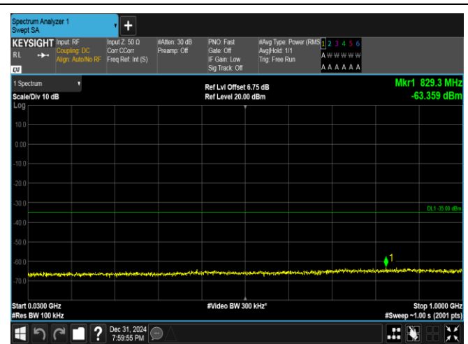
Band38-20MHz-QPSK-38000-100RB#0-30~1000-PASS
