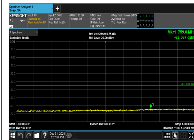
Band38-20MHz-QPSK-38000-1RB#99-30~1000-PASS
