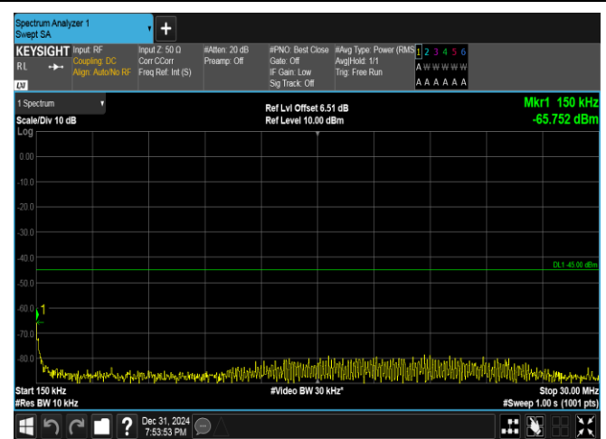
Band38-20MHz-QPSK-37850-100RB#0-0.15~30-PASS
