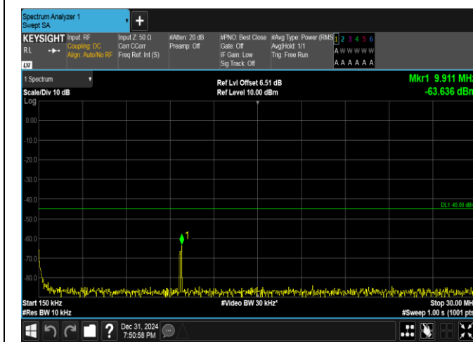
Band38-20MHz-16QAM-37850-1RB#0-0.15~30-PASS
