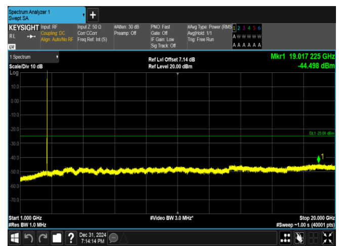
Band38-15MHz-16QAM-38175-1RB#74-1000~20000-PASS
