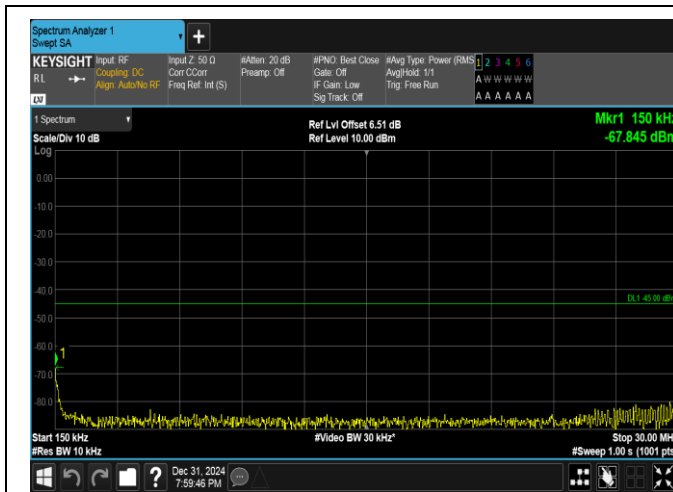
Band38-20MHz-QPSK-38000-100RB#0-0.15~30-PASS
