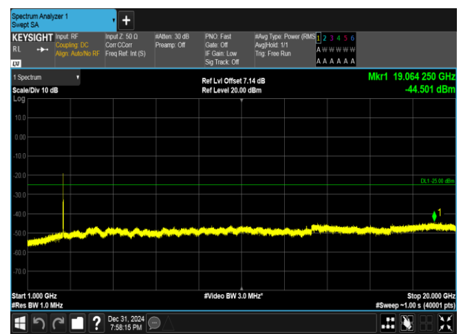
Band38-20MHz-QPSK-38000-1RB#99-1000~20000-PASS
