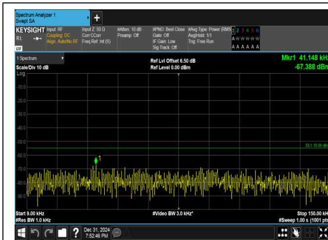
Band38-20MHz-16QAM-37850-1RB#99-0.009~0.15-PASS
