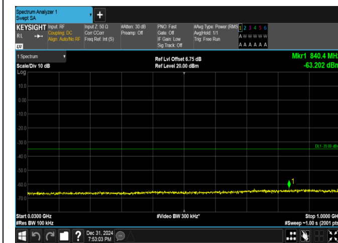
Band38-20MHz-16QAM-37850-1RB#99-30~1000-PASS
