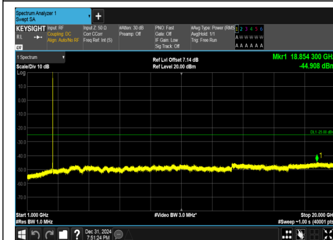
Band38-20MHz-16QAM-37850-1RB#0-1000~20000-PASS
