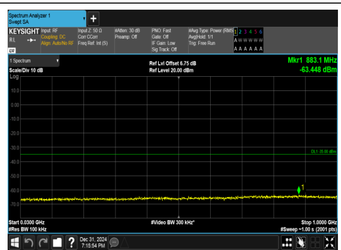
Band38-15MHz-16QAM-38175-75RB#0-30~1000-PASS
