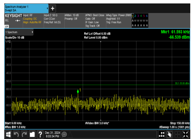
Band38-20MHz-QPSK-38150-1RB#99-0.009~0.15-PASS
