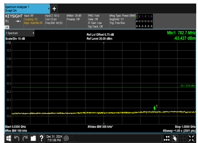
Band38-20MHz-16QAM-37850-1RB#0-30~1000-PASS
