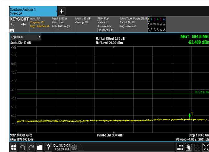
Band38-20MHz-16QAM-38000-1RB#0-30~1000-PASS
