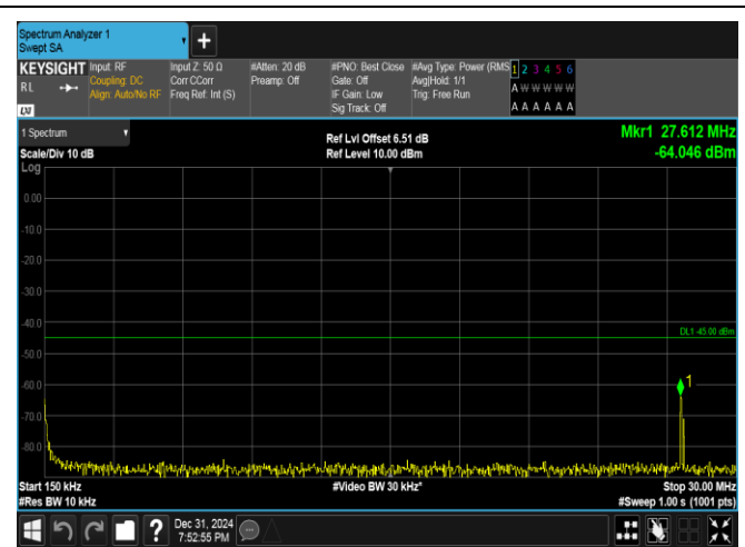
Band38-20MHz-16QAM-37850-1RB#99-0.15~30-PASS
