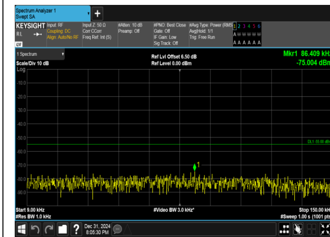
Band38-20MHz-QPSK-38150-100RB#0-0.009~0.15-PASS
