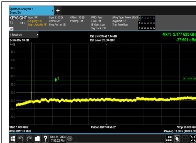
Band38-20MHz-QPSK-37850-1RB#99-1000~20000-PASS
