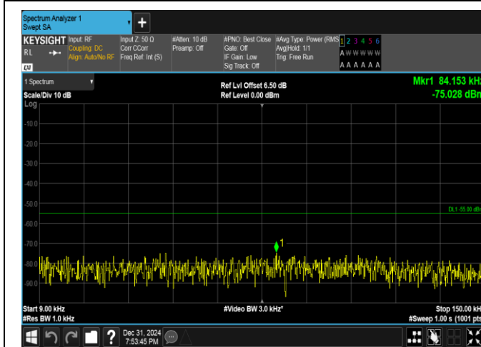
Band38-20MHz-QPSK-37850-100RB#0-0.009~0.15-PASS
