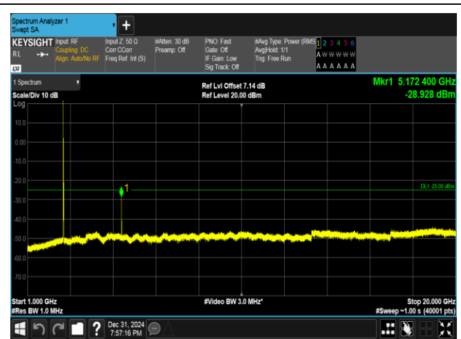
Band38-20MHz-16QAM-38000-1RB#0-1000~20000-PASS
