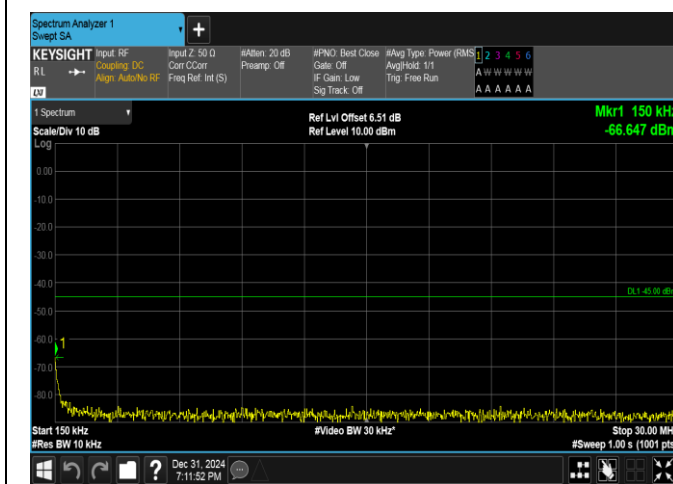
Band38-15MHz-16QAM-38175-1RB#0-0.15~30-PASS
