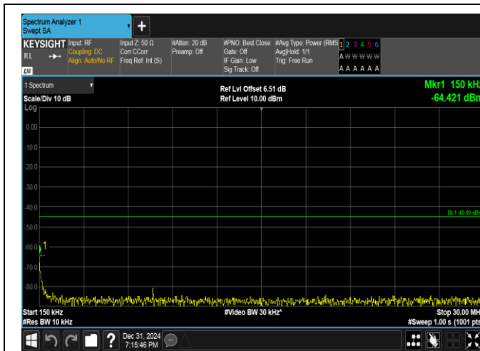
Band38-15MHz-16QAM-38175-75RB#0-0.15~30-PASS
