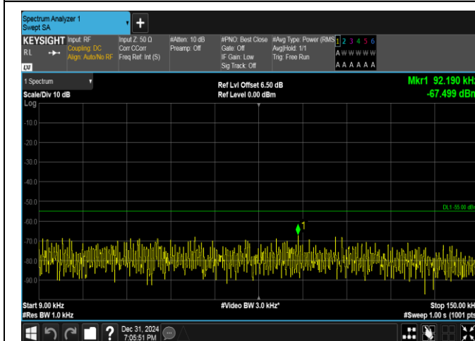
Band38-15MHz-16QAM-38000-1RB#0-0.009~0.15-PASS
