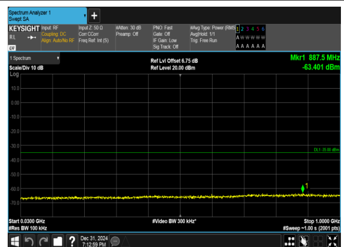
Band38-15MHz-QPSK-38175-1RB#74-30~1000-PASS
