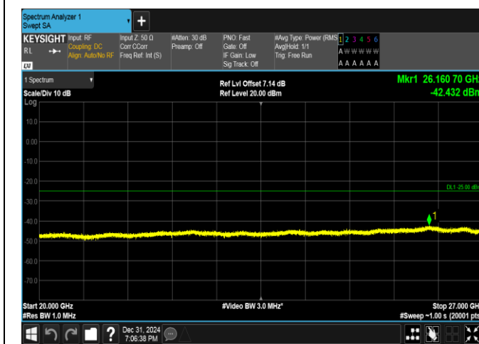
Band38-15MHz-16QAM-38000-1RB#0-20000~27000-PASS
