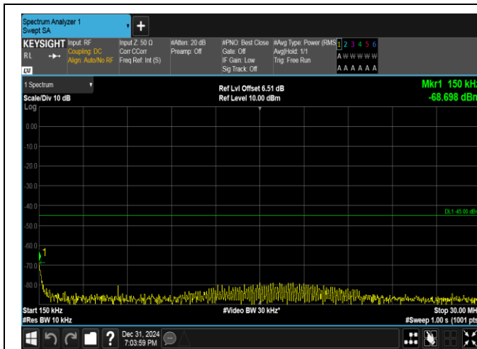
Band38-15MHz-16QAM-37825-75RB#0-0.15~30-PASS
