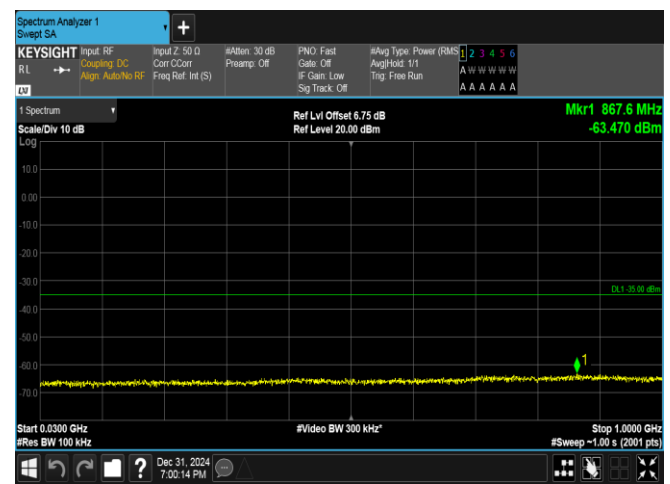
Band38-15MHz-16QAM-37825-1RB#0-30~1000-PASS
