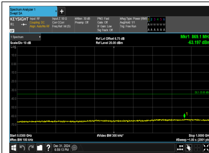
Band38-15MHz-QPSK-37825-1RB#0-30~1000-PASS
