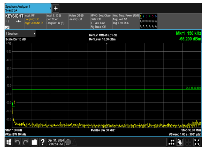
Band38-15MHz-16QAM-38000-75RB#0-0.15~30-PASS
