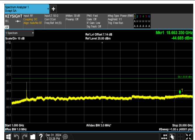
Band38-15MHz-QPSK-37825-75RB#0-1000~20000-PASS
