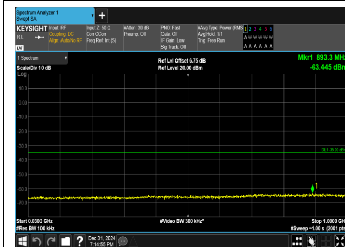
Band38-15MHz-QPSK-38175-75RB#0-30~1000-PASS
