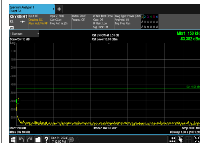
Band38-15MHz-QPSK-38175-1RB#74-0.15~30-PASS
