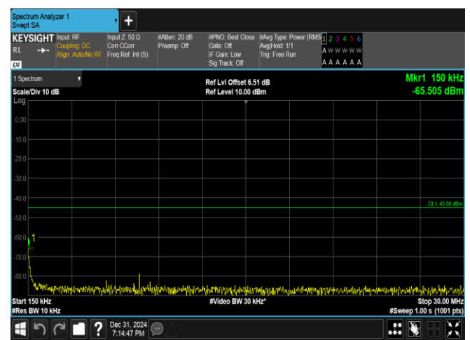
Band38-15MHz-QPSK-38175-75RB#0-0.15~30-PASS
