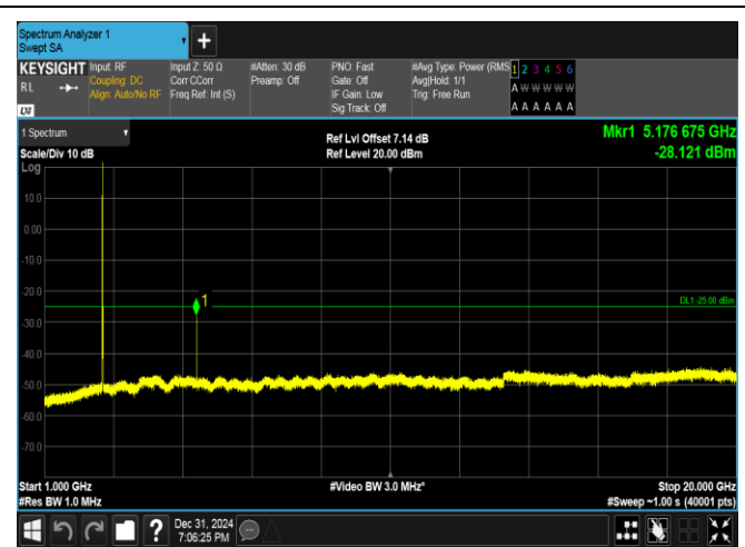
Band38-15MHz-16QAM-38000-1RB#0-1000~20000-PASS
