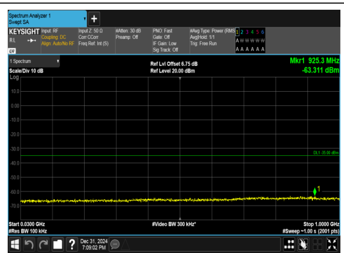
Band38-15MHz-QPSK-38000-75RB#0-30~1000-PASS
