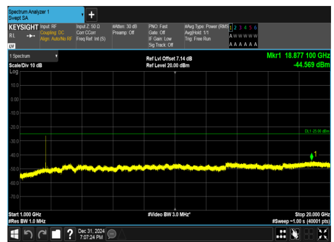
Band38-15MHz-QPSK-38000-1RB#74-1000~20000-PASS
