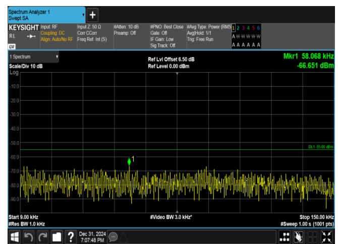
Band38-15MHz-16QAM-38000-1RB#74-0.009~0.15-PASS
