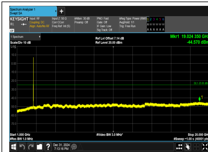
Band38-15MHz-QPSK-38175-1RB#74-1000~20000-PASS
