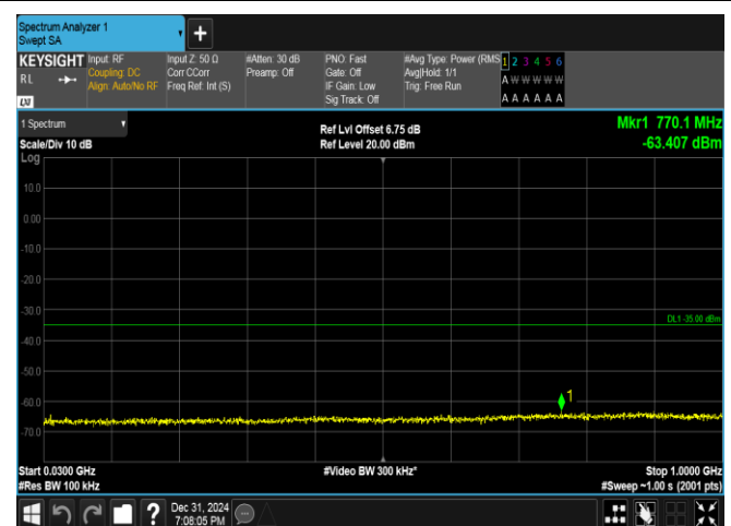
Band38-15MHz-16QAM-38000-1RB#74-30~1000-PASS
