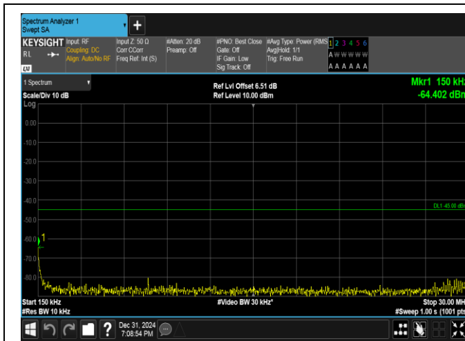
Band38-15MHz-QPSK-38000-75RB#0-0.15~30-PASS
