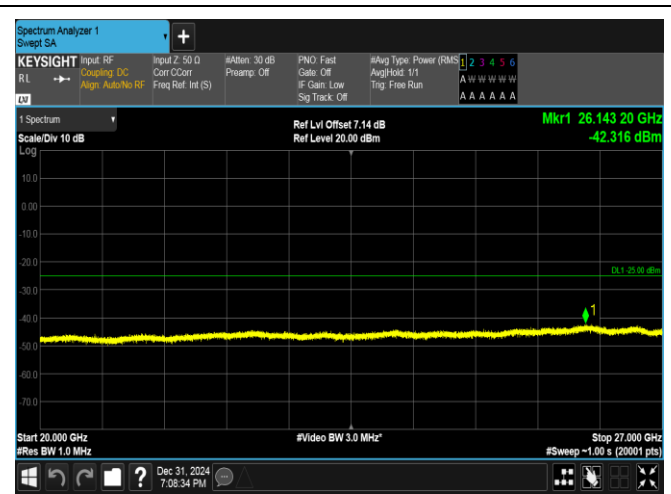
Band38-15MHz-16QAM-38000-1RB#74-20000~27000-PASS
