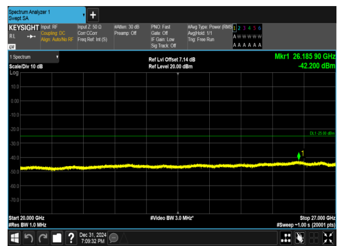
Band38-15MHz-QPSK-38000-75RB#0-20000~27000-PASS
