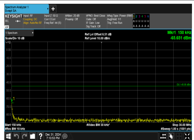
Band38-15MHz-QPSK-38175-1RB#0-0.15~30-PASS
