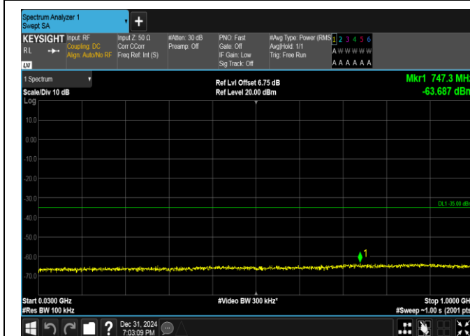
Band38-15MHz-QPSK-37825-75RB#0-30~1000-PASS
