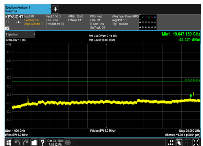
Band38-15MHz-QPSK-38175-75RB#0-1000~20000-PASS
