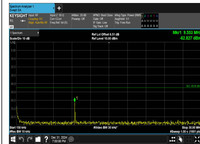
Band38-15MHz-16QAM-37825-1RB#0-0.15~30-PASS
