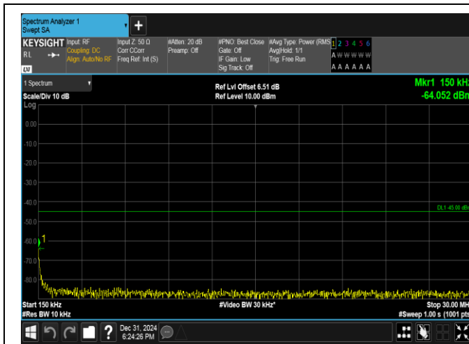
Band38-10MHz-16QAM-38200-50RB#0-0.15~30-PASS
