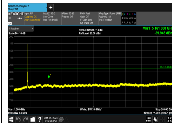
Band38-15MHz-16QAM-37825-75RB#0-1000~20000-PASS
