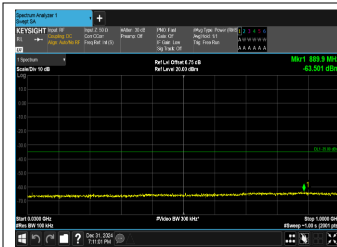
Band38-15MHz-QPSK-38175-1RB#0-30~1000-PASS
