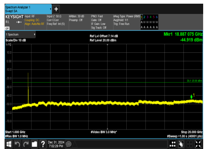
Band38-15MHz-16QAM-37825-1RB#74-1000~20000-PASS
