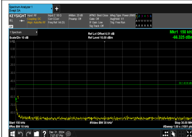
Band38-15MHz-16QAM-38000-1RB#74-0.15~30-PASS
