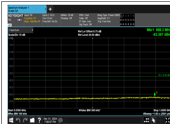
Band38-15MHz-16QAM-38000-1RB#0-30~1000-PASS
