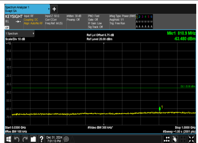
Band38-15MHz-QPSK-37825-1RB#74-30~1000-PASS
