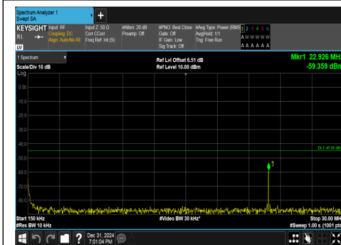
Band38-15MHz-QPSK-37825-1RB#74-0.15~30-PASS
