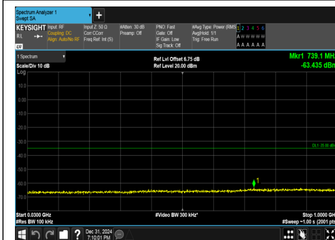
Band38-15MHz-16QAM-38000-75RB#0-30~1000-PASS
