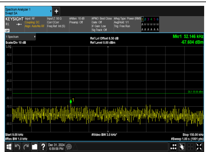
Band38-15MHz-16QAM-37825-1RB#0-0.009~0.15-PASS
