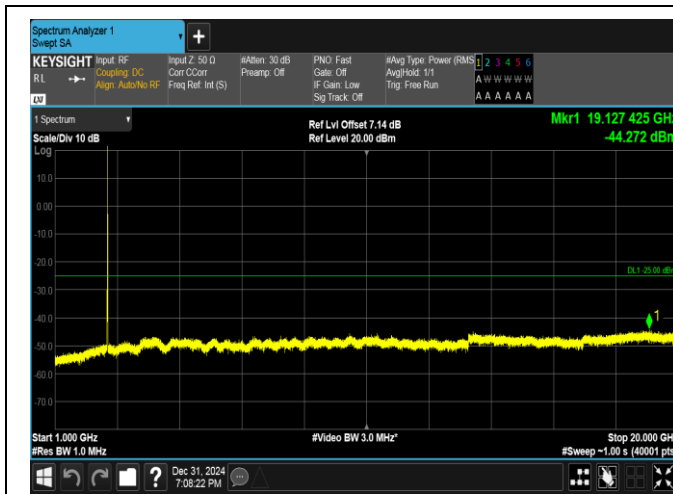
Band38-15MHz-16QAM-38000-1RB#74-1000~20000-PASS
