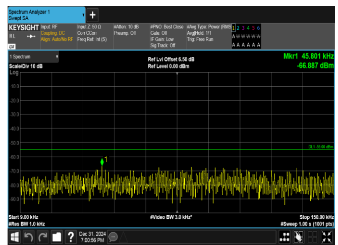
Band38-15MHz-QPSK-37825-1RB#74-0.009~0.15-PASS
