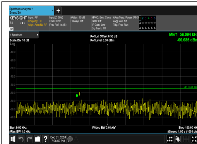
Band38-15MHz-QPSK-38000-1RB#74-0.009~0.15-PASS
