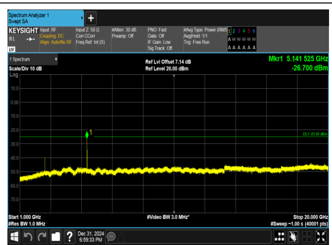
Band38-15MHz-QPSK-37825-1RB#0-1000~20000-PASS
