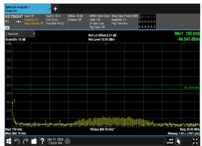
Band38-15MHz-QPSK-37825-75RB#0-0.15~30-PASS
