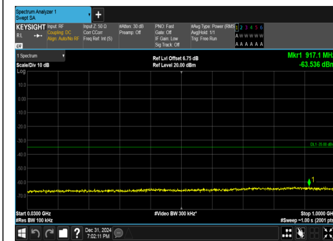
Band38-15MHz-16QAM-37825-1RB#74-30~1000-PASS
