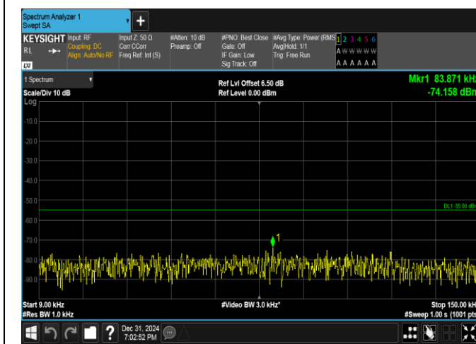
Band38-15MHz-QPSK-37825-75RB#0-0.009~0.15-PASS
