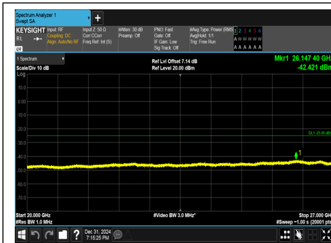
Band38-15MHz-QPSK-38175-75RB#0-20000~27000-PASS
