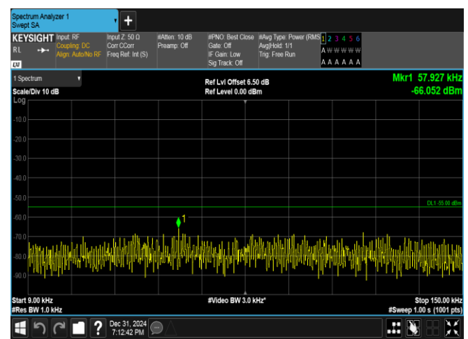
Band38-15MHz-QPSK-38175-1RB#74-0.009~0.15-PASS
