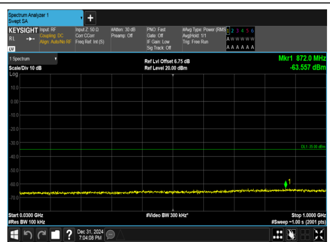
Band38-15MHz-16QAM-37825-75RB#0-30~1000-PASS
