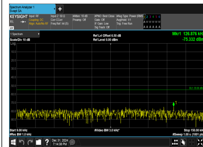
Band38-15MHz-QPSK-38175-75RB#0-0.009~0.15-PASS
