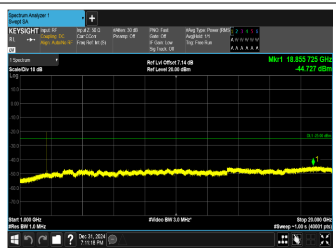
Band38-15MHz-QPSK-38175-1RB#0-1000~20000-PASS
