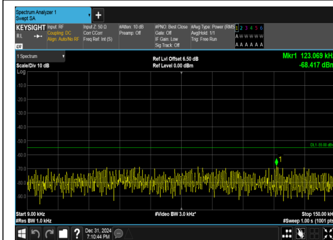
Band38-15MHz-QPSK-38175-1RB#0-0.009~0.15-PASS
