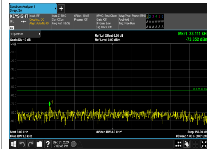
Band38-15MHz-16QAM-38000-75RB#0-0.009~0.15-PASS
