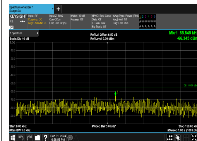
Band38-15MHz-QPSK-37825-1RB#0-0.009~0.15-PASS
