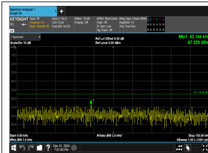
Band38-15MHz-16QAM-37825-1RB#74-0.009~0.15-PASS
