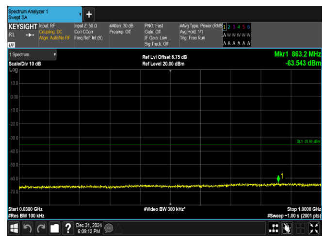
Band38-10MHz-16QAM-37800-1RB#0-30~1000-PASS
