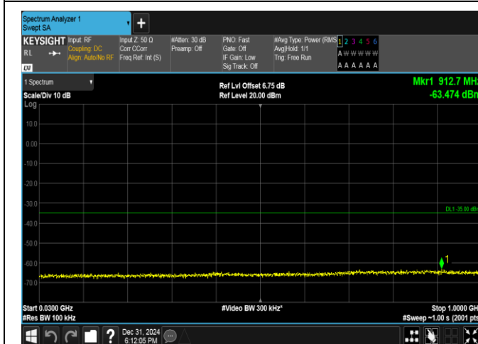
Band38-10MHz-QPSK-37800-50RB#0-30~1000-PASS
