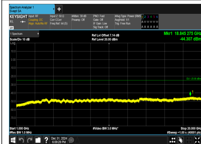
Band38-10MHz-16QAM-37800-1RB#0-1000~20000-PASS
