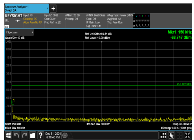
Band38-10MHz-16QAM-38000-50RB#0-0.15~30-PASS
