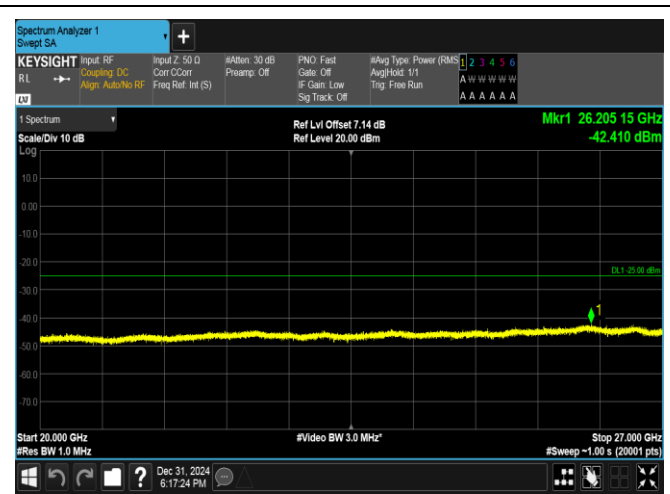
Band38-10MHz-16QAM-38000-1RB#49-20000~27000-PASS
