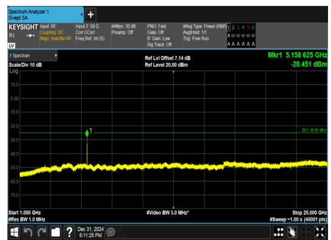
Band38-10MHz-16QAM-37800-1RB#49-1000~20000-PASS
