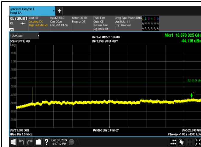
Band38-10MHz-16QAM-38000-1RB#49-1000~20000-PASS
