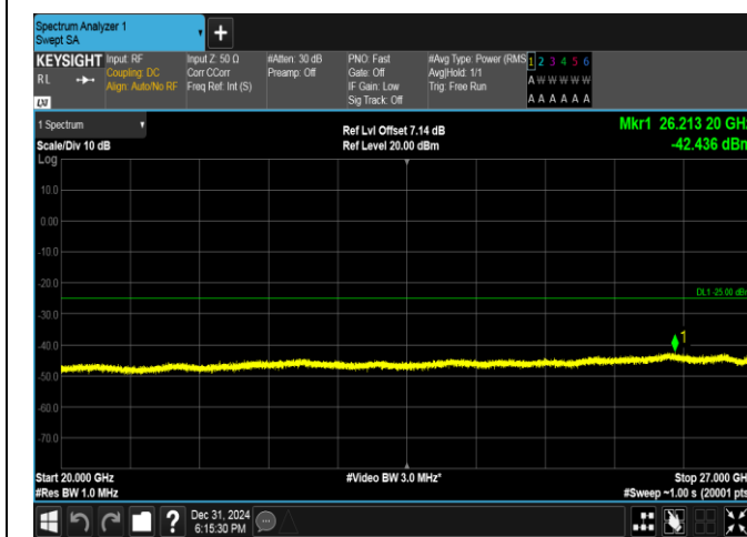
Band38-10MHz-16QAM-38000-1RB#0-20000~27000-PASS
