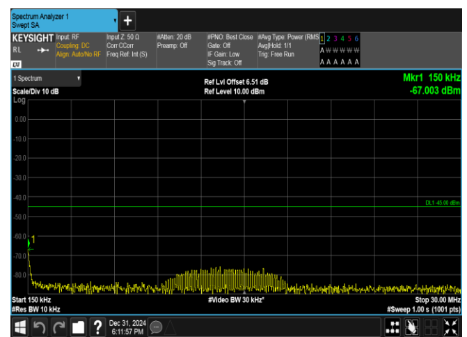
Band38-10MHz-QPSK-37800-50RB#0-0.15~30-PASS
