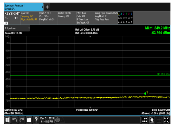
Band38-10MHz-QPSK-38000-1RB#0-30~1000-PASS
