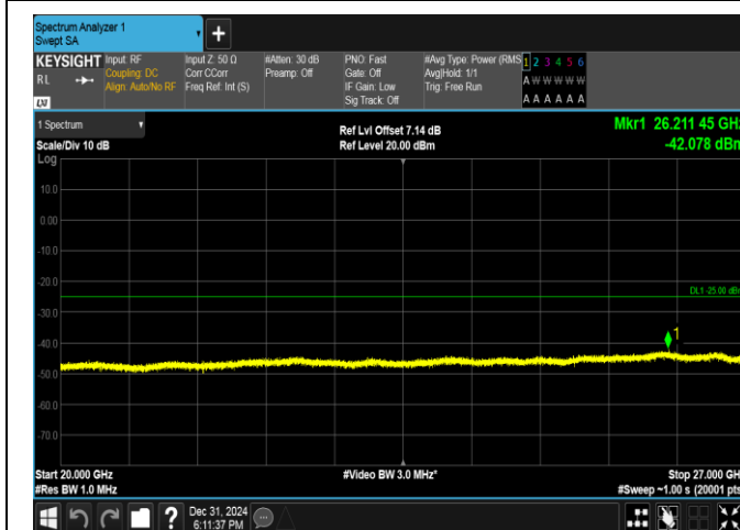
Band38-10MHz-16QAM-37800-1RB#49-20000~27000-PASS
