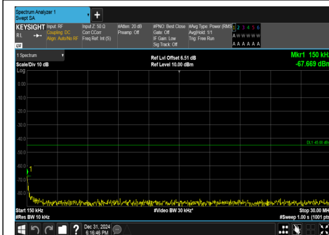
Band38-10MHz-16QAM-38000-1RB#49-0.15~30-PASS
