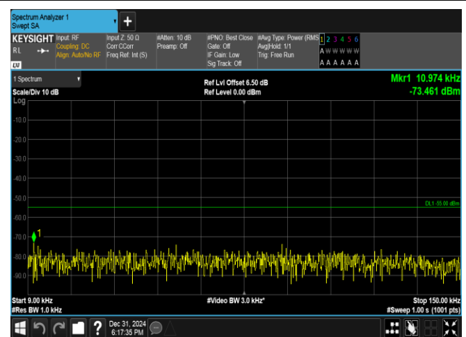
Band38-10MHz-QPSK-38000-50RB#0-0.009~0.15-PASS
