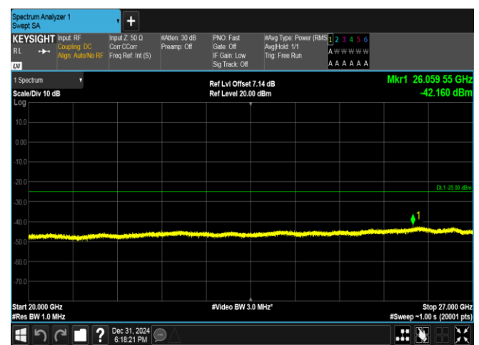
Band38-10MHz-QPSK-38000-50RB#0-20000~27000-PASS
