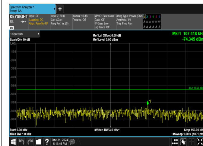
Band38-10MHz-QPSK-37800-50RB#0-0.009~0.15-PASS
