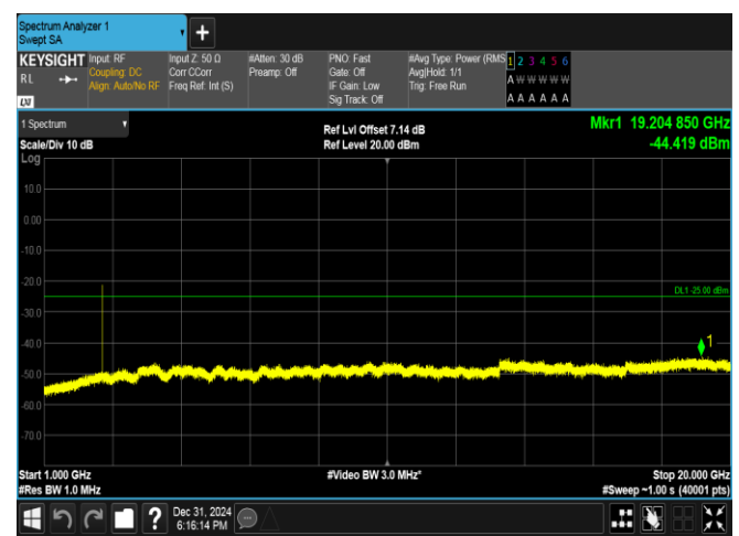
Band38-10MHz-QPSK-38000-1RB#49-1000~20000-PASS
