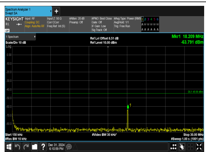
Band38-10MHz-16QAM-37800-1RB#49-0.15~30-PASS
