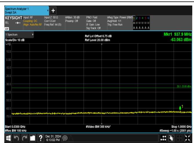
Band38-10MHz-16QAM-37800-50RB#0-30~1000-PASS
