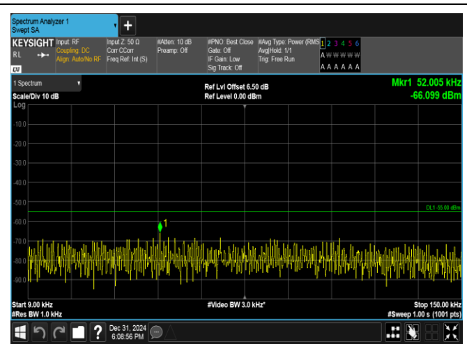
Band38-10MHz-16QAM-37800-1RB#0-0.009~0.15-PASS
