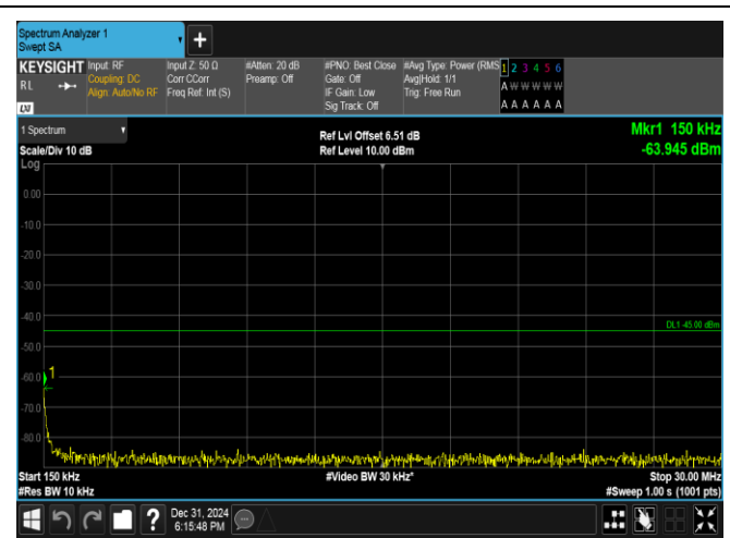
Band38-10MHz-QPSK-38000-1RB#49-0.15~30-PASS
