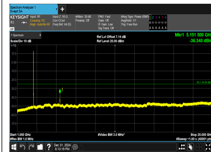
Band38-10MHz-16QAM-37800-50RB#0-1000~20000-PASS
