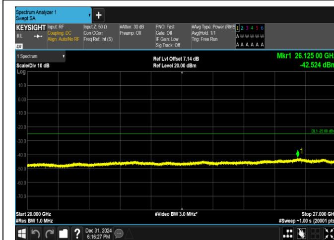
Band38-10MHz-QPSK-38000-1RB#49-20000~27000-PASS
