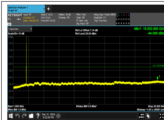
Band38-10MHz-QPSK-38200-1RB#49-1000~20000-PASS
