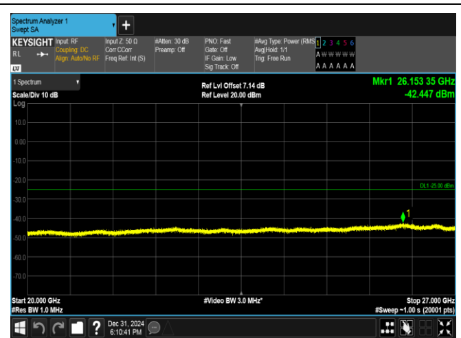
Band38-10MHz-QPSK-37800-1RB#49-20000~27000-PASS
