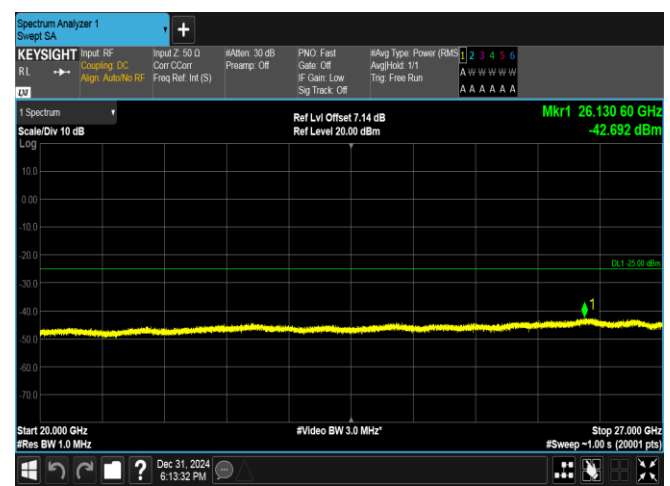
Band38-10MHz-16QAM-37800-50RB#0-20000~27000-PASS
