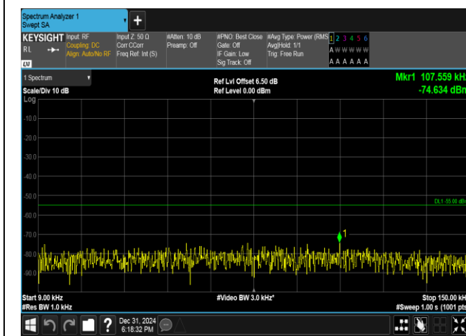
Band38-10MHz-16QAM-38000-50RB#0-0.009~0.15-PASS
