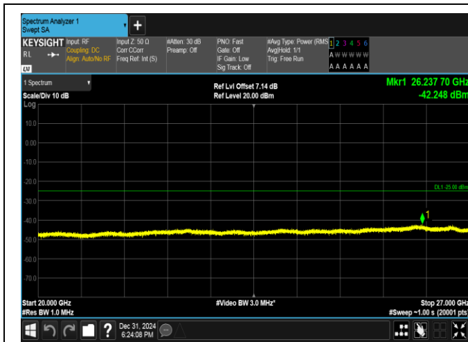
Band38-10MHz-QPSK-38200-50RB#0-20000~27000-PASS
