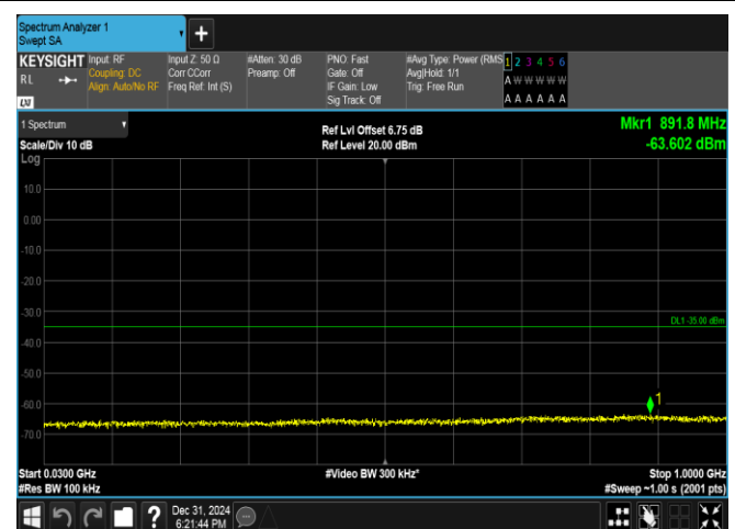
Band38-10MHz-QPSK-38200-1RB#49-30~1000-PASS
