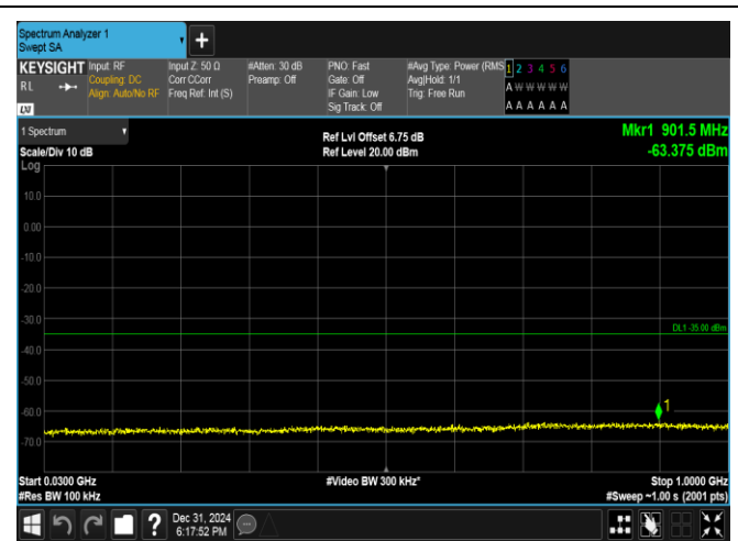
Band38-10MHz-QPSK-38000-50RB#0-30~1000-PASS
