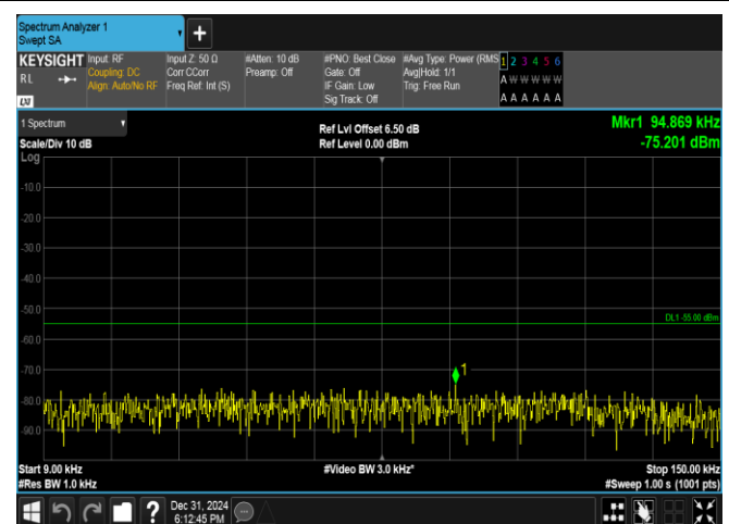
Band38-10MHz-16QAM-37800-50RB#0-0.009~0.15-PASS
