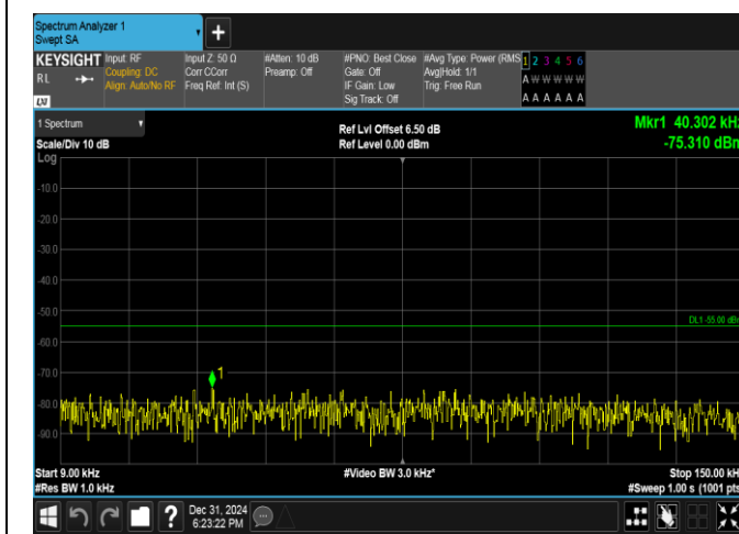
Band38-10MHz-QPSK-38200-50RB#0-0.009~0.15-PASS
