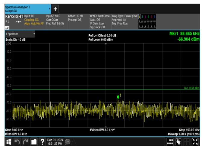
Band38-10MHz-QPSK-38200-1RB#49-0.009~0.15-PASS
