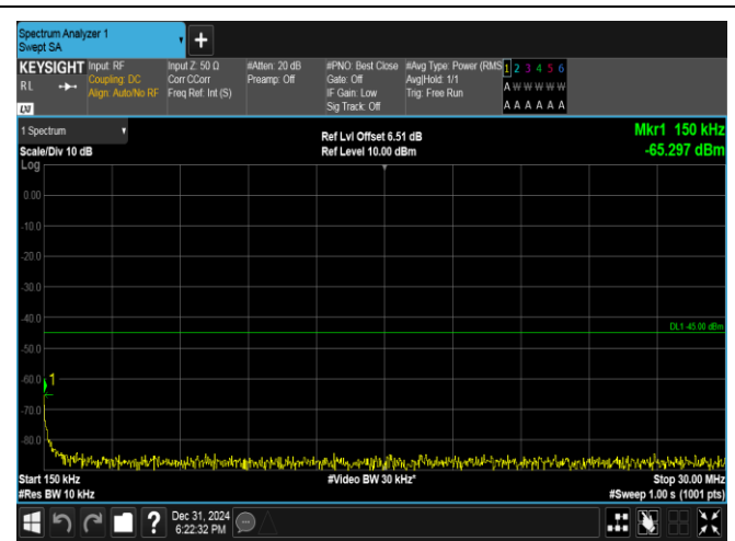
Band38-10MHz-16QAM-38200-1RB#49-0.15~30-PASS
