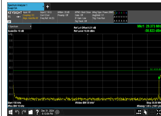
Band38-10MHz-QPSK-38000-1RB#0-0.15~30-PASS
