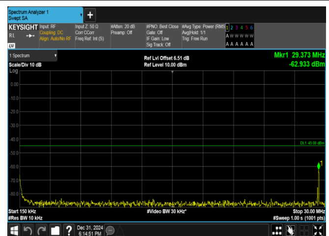
Band38-10MHz-16QAM-38000-1RB#0-0.15~30-PASS
