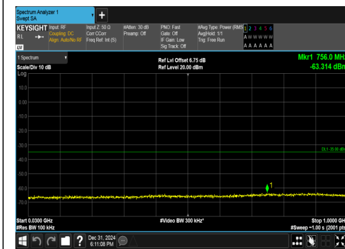
Band38-10MHz-16QAM-37800-1RB#49-30~1000-PASS
