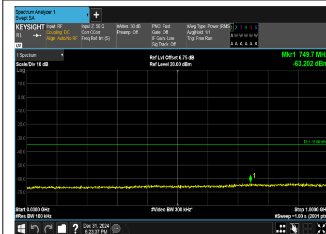
Band38-10MHz-QPSK-38200-50RB#0-30~1000-PASS
