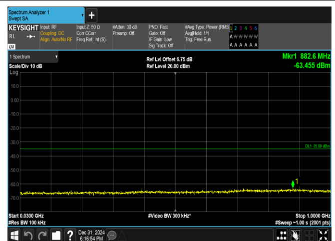
Band38-10MHz-16QAM-38000-1RB#49-30~1000-PASS
