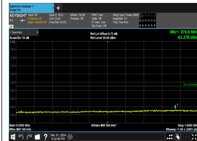
Band38-10MHz-16QAM-38200-1RB#49-30~1000-PASS
