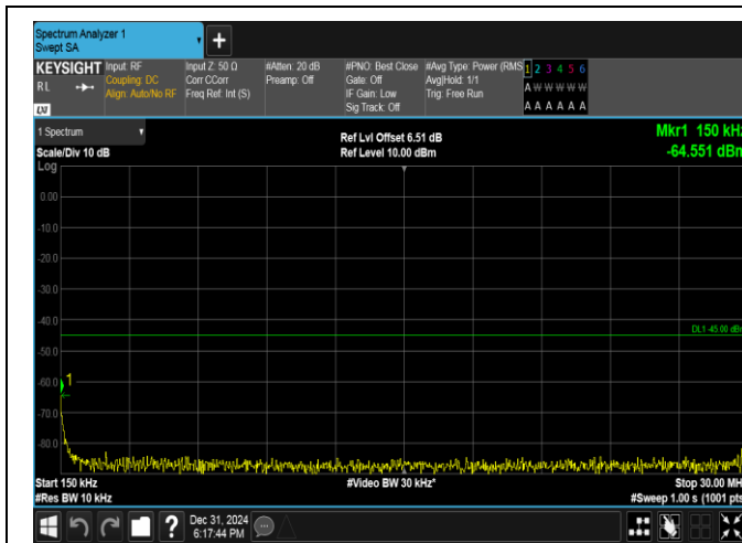
Band38-10MHz-QPSK-38000-50RB#0-0.15~30-PASS
