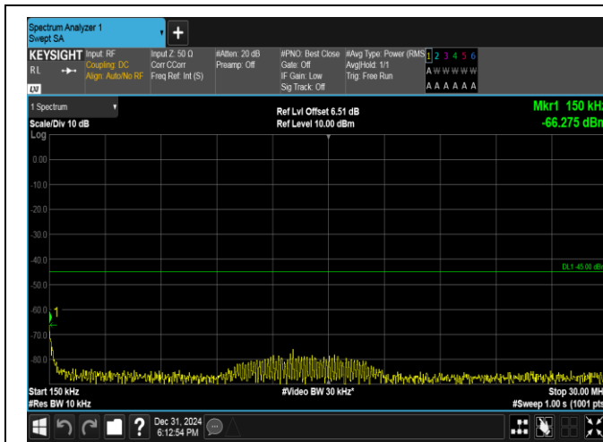
Band38-10MHz-16QAM-37800-50RB#0-0.15~30-PASS
