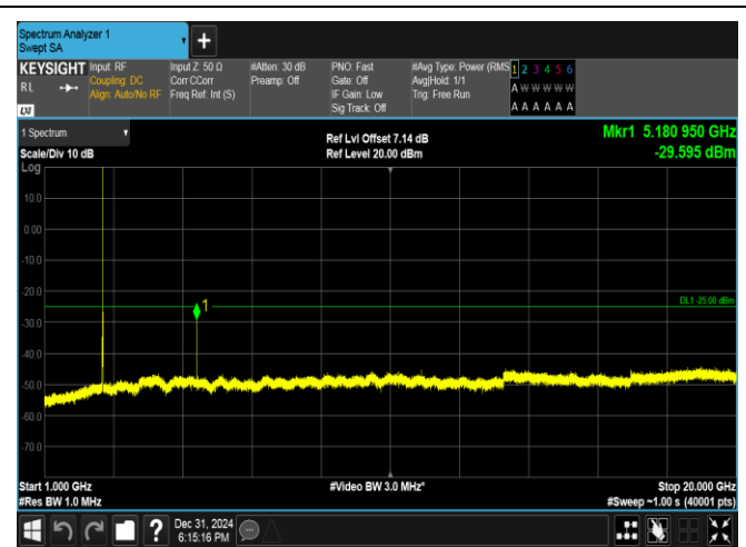
Band38-10MHz-16QAM-38000-1RB#0-1000~20000-PASS
