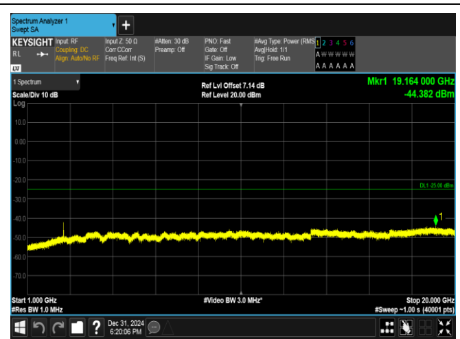
Band38-10MHz-QPSK-38200-1RB#0-1000~20000-PASS
