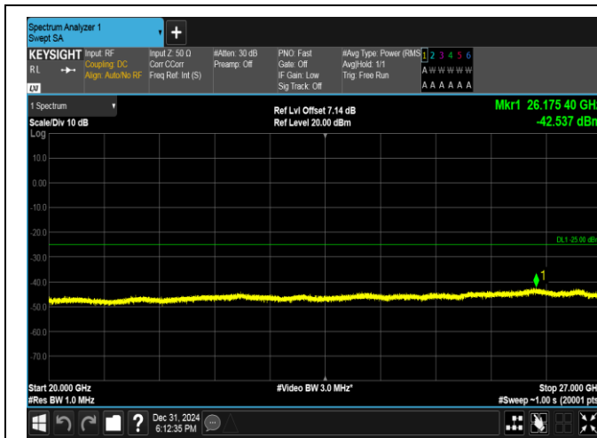
Band38-10MHz-QPSK-37800-50RB#0-20000~27000-PASS
