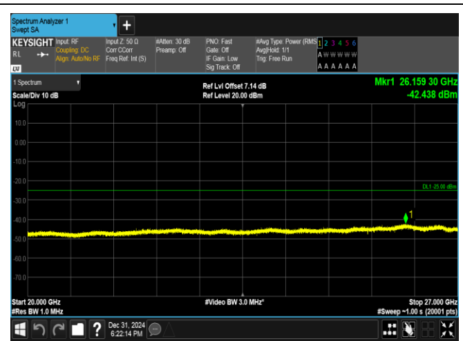
Band38-10MHz-QPSK-38200-1RB#49-20000~27000-PASS
