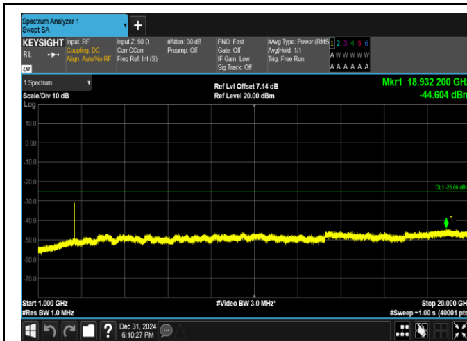
Band38-10MHz-QPSK-37800-1RB#49-1000~20000-PASS
