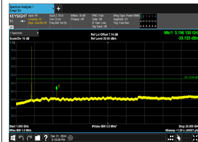
Band38-10MHz-QPSK-38000-50RB#0-1000~20000-PASS
