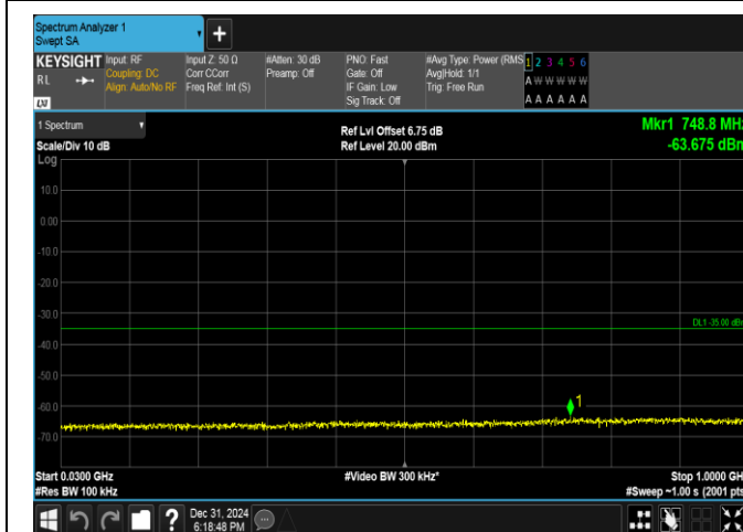
Band38-10MHz-16QAM-38000-50RB#0-30~1000-PASS
