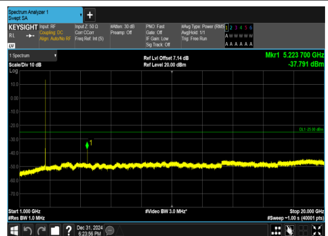
Band38-10MHz-QPSK-38200-50RB#0-1000~20000-PASS
