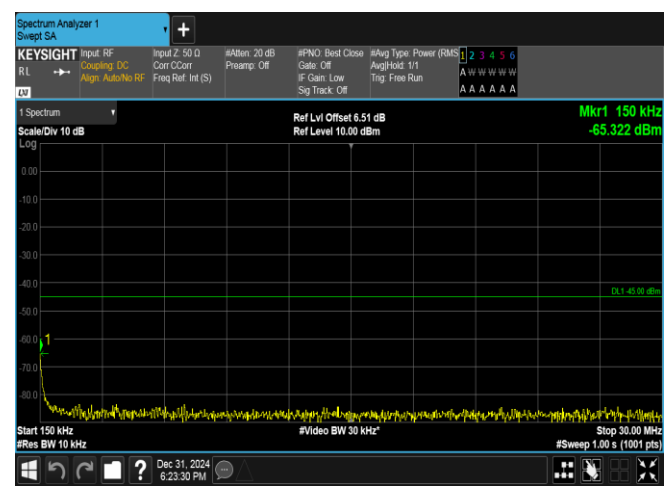
Band38-10MHz-QPSK-38200-50RB#0-0.15~30-PASS
