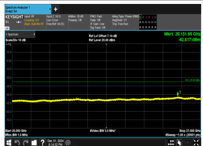
Band38-10MHz-QPSK-38000-1RB#0-20000~27000-PASS
