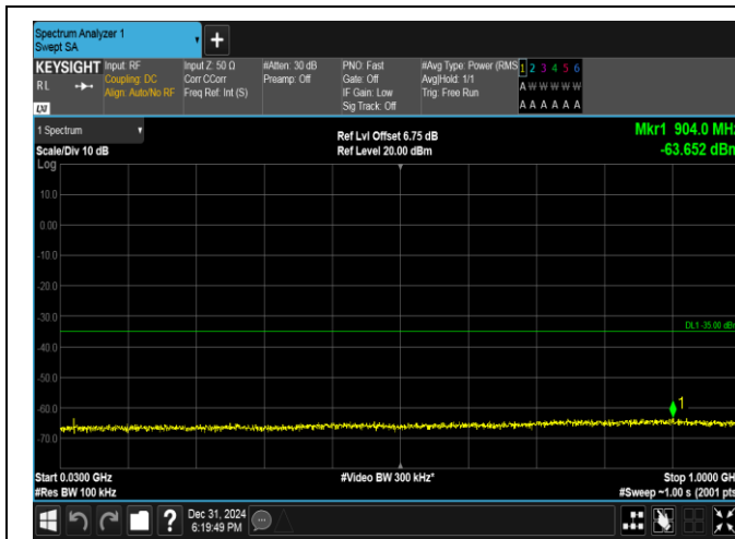
Band38-10MHz-QPSK-38200-1RB#0-30~1000-PASS
