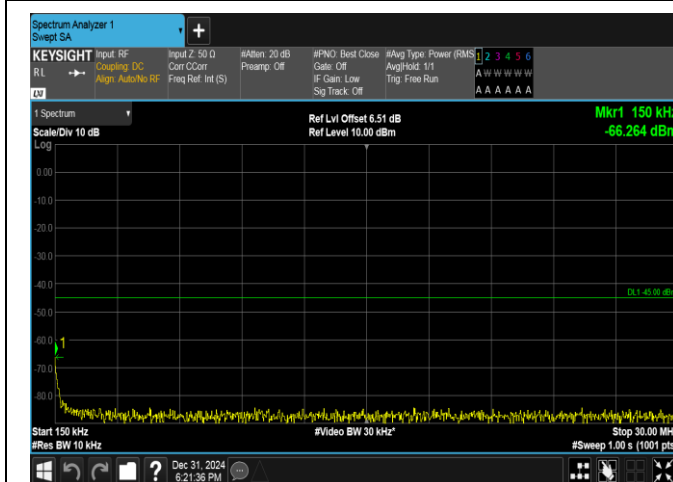
Band38-10MHz-QPSK-38200-1RB#49-0.15~30-PASS
