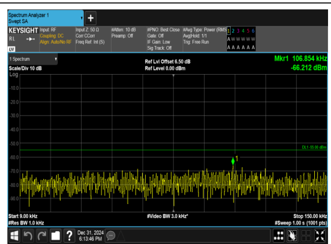
Band38-10MHz-QPSK-38000-1RB#0-0.009~0.15-PASS
