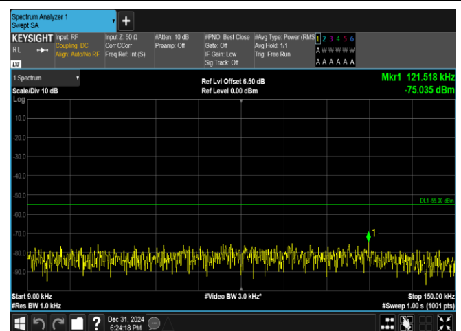
Band38-10MHz-16QAM-38200-50RB#0-0.009~0.15-PASS
