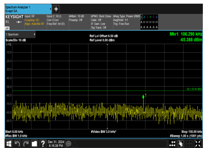
Band38-10MHz-16QAM-38000-1RB#49-0.009~0.15-PASS
