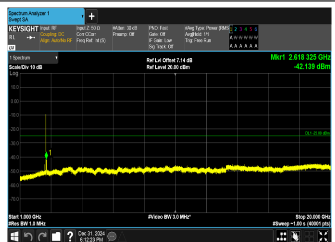
Band38-10MHz-QPSK-37800-50RB#0-1000~20000-PASS
