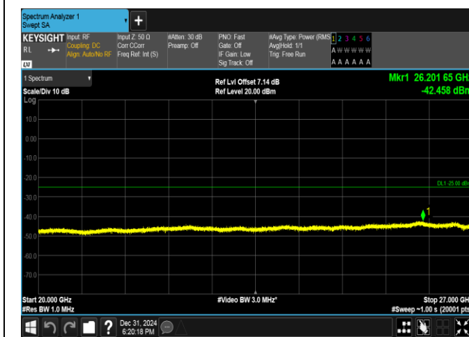
Band38-10MHz-QPSK-38200-1RB#0-20000~27000-PASS
