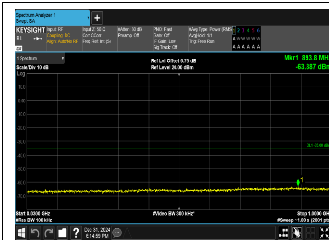
Band38-10MHz-16QAM-38000-1RB#0-30~1000-PASS
