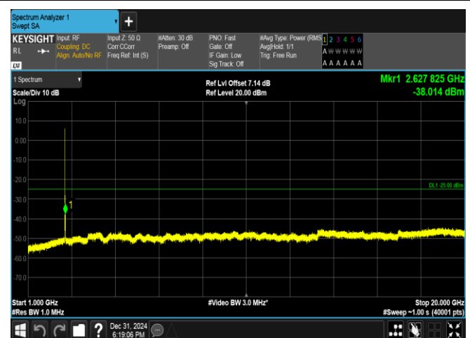
Band38-10MHz-16QAM-38000-50RB#0-1000~20000-PASS
