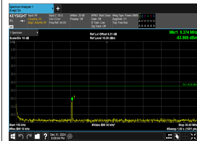
Band38-10MHz-16QAM-37800-1RB#0-0.15~30-PASS
