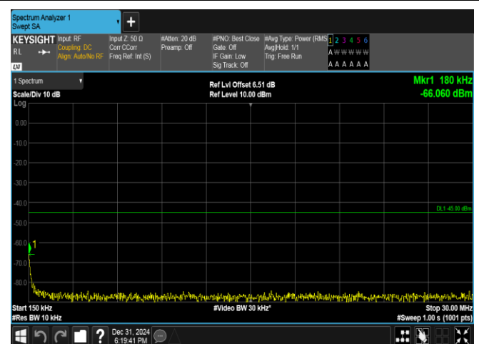
Band38-10MHz-QPSK-38200-1RB#0-0.15~30-PASS
