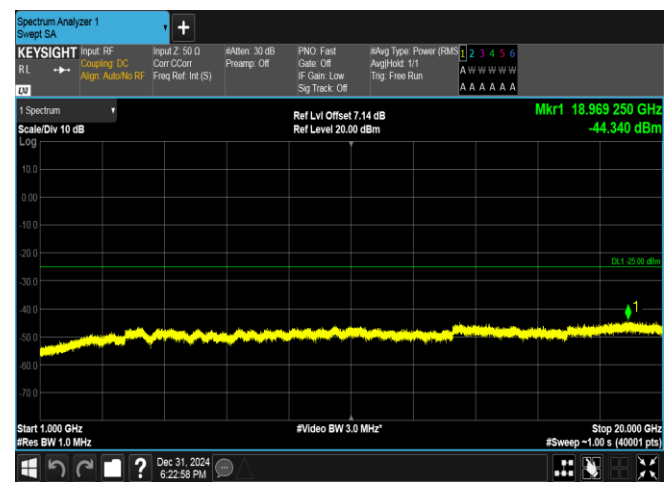
Band38-10MHz-16QAM-38200-1RB#49-1000~20000-PASS
