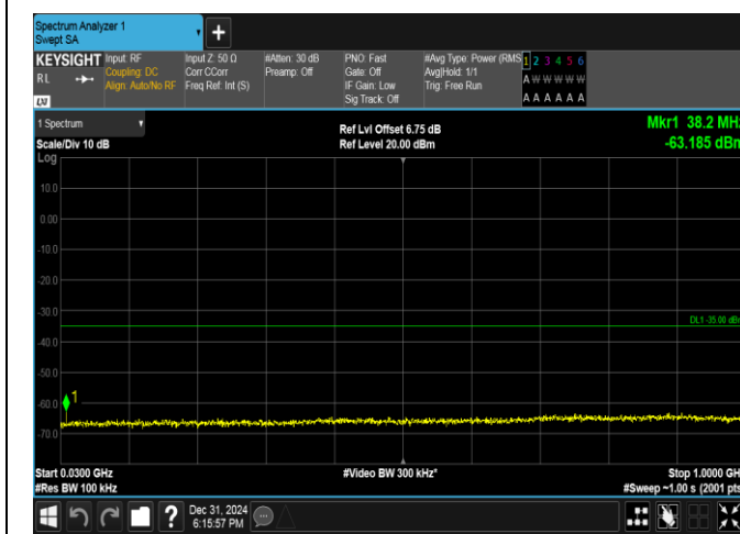
Band38-10MHz-QPSK-38000-1RB#49-30~1000-PASS
