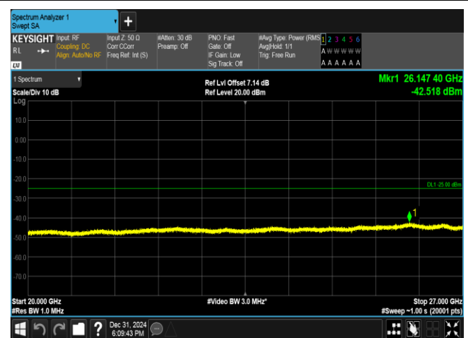
Band38-10MHz-16QAM-37800-1RB#0-20000~27000-PASS
