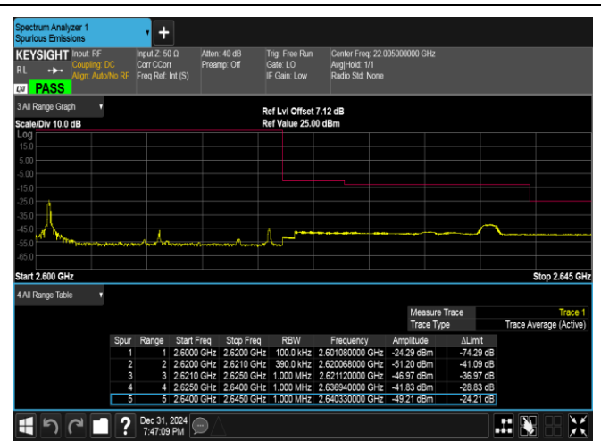
Band38-20MHz-16QAM-38150-1RB#0-PASS
