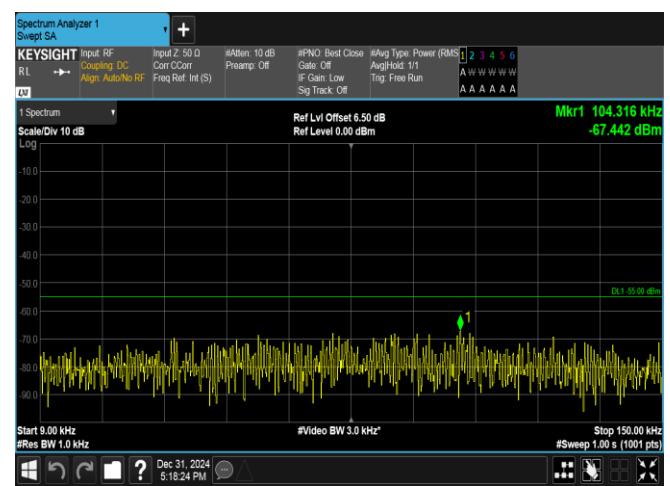
Band38-5MHz-QPSK-37775-1RB#24-0.009~0.15-PASS
