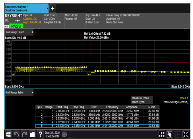
Band38-20MHz-16QAM-38150-100RB#0-PASS
