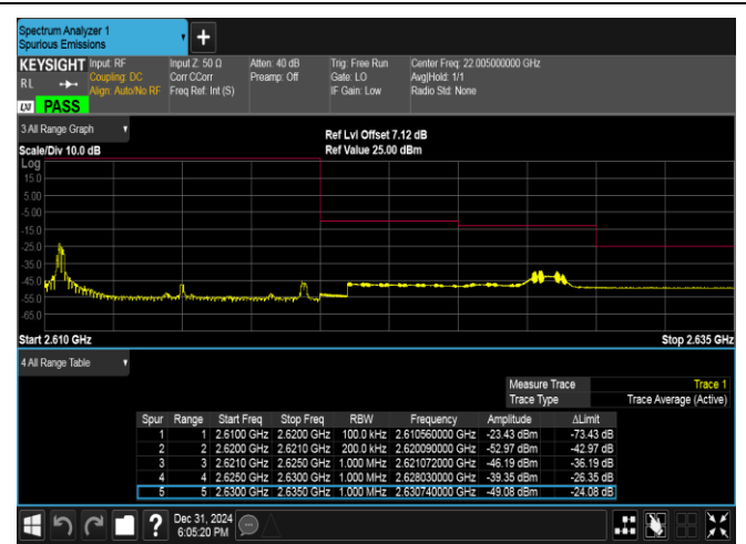
Band38-10MHz-16QAM-38200-1RB#0-PASS
