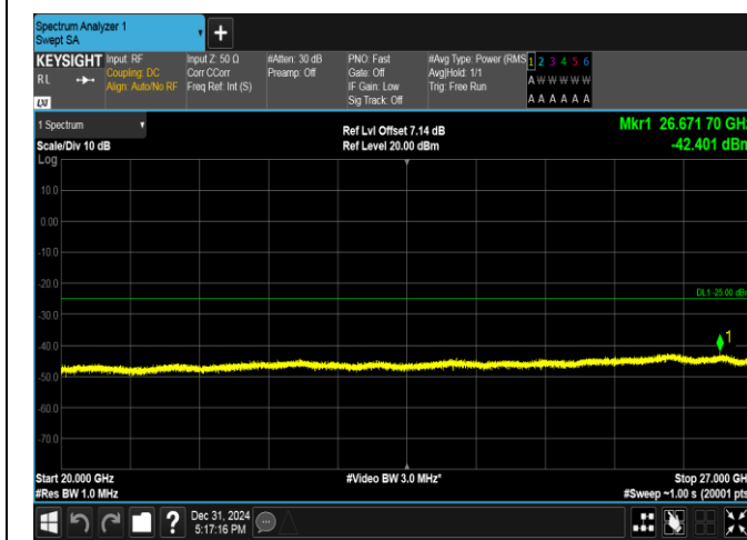
Band38-5MHz-QPSK-37775-1RB#0-20000~27000-PASS
