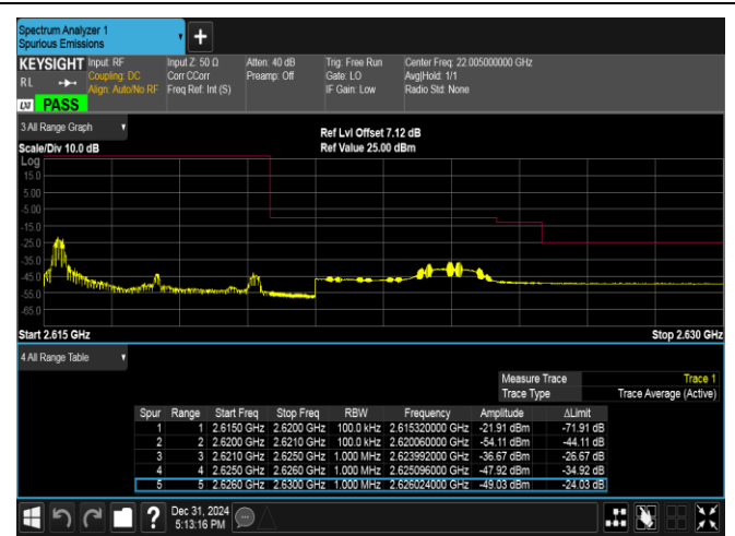
Band38-5MHz-QPSK-38225-1RB#0-PASS
