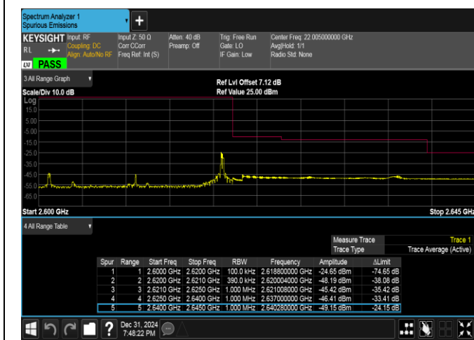
Band38-20MHz-16QAM-38150-1RB#99-PASS
