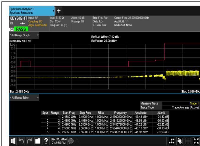
Band38-20MHz-16QAM-37850-100RB#0-PASS
