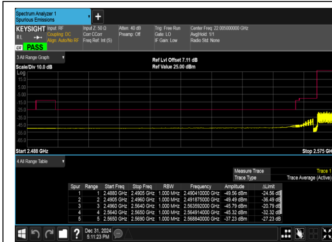
Band38-5MHz-QPSK-37775-25RB#0-PASS
