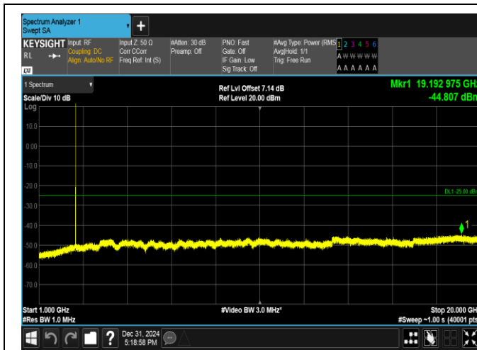
Band38-5MHz-QPSK-37775-1RB#24-1000~20000-PASS
