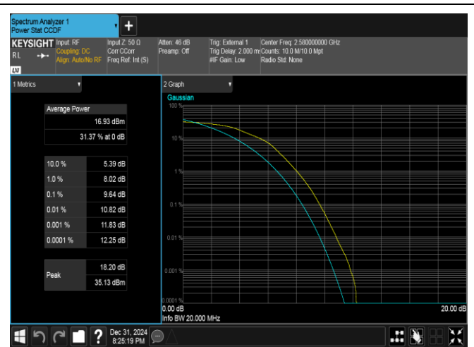
Band38-20MHz-16QAM-37850-100RB#0-PASS
