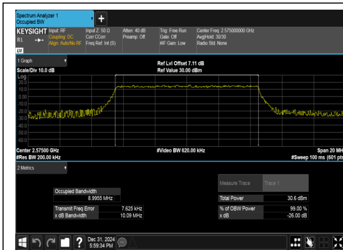
Band38-10MHz-QPSK-37800-50RB#0-PASS
