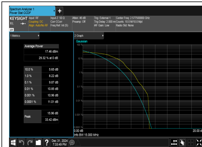
Band38-15MHz-16QAM-37825-1RB#0-PASS
