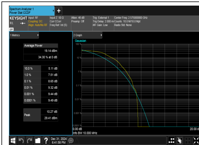
Band38-10MHz-QPSK-37800-1RB#0-PASS
