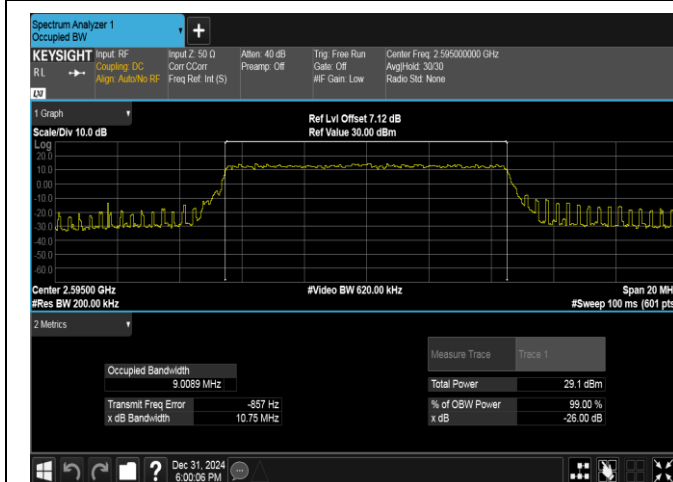
Band38-10MHz-16QAM-38000-50RB#0-PASS
