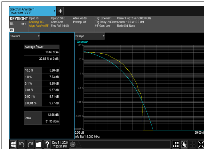
Band38-15MHz-QPSK-37825-1RB#0-PASS
