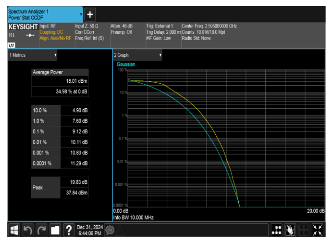
Band38-10MHz-QPSK-38000-50RB#0-PASS
