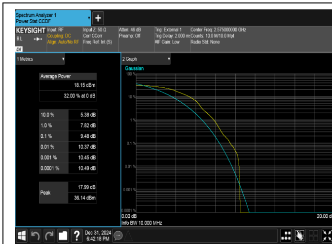
Band38-10MHz-16QAM-37800-1RB#0-PASS
