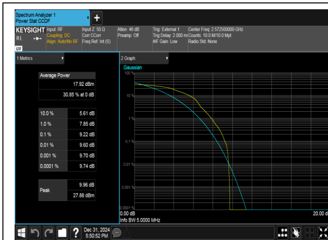
Band38-5MHz-16QAM-37775-1RB#0-PASS
