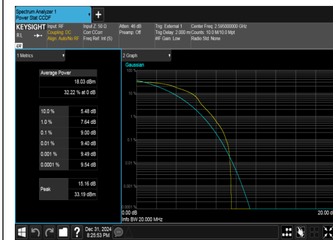
Band38-20MHz-16QAM-38000-1RB#0-PASS
