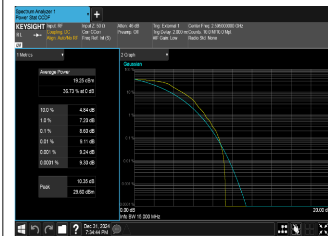
Band38-15MHz-QPSK-38000-1RB#0-PASS
