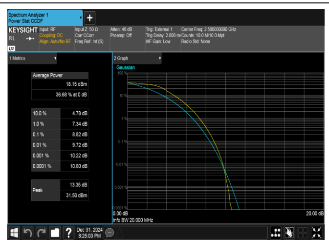
Band38-20MHz-QPSK-37850-100RB#0-PASS
