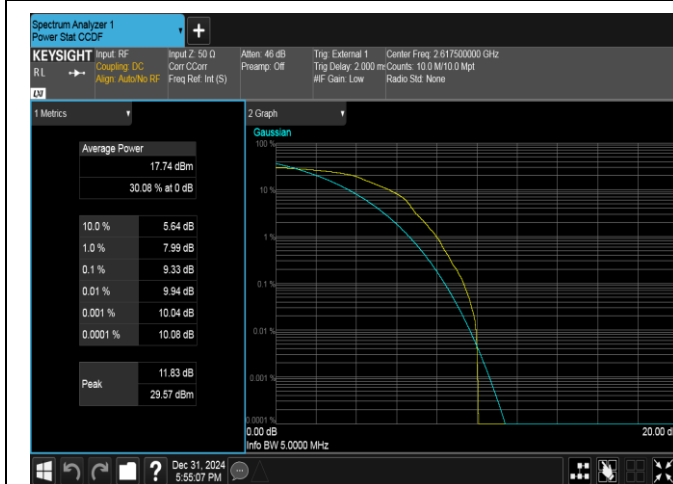
Band38-5MHz-16QAM-38225-1RB#0-PASS
