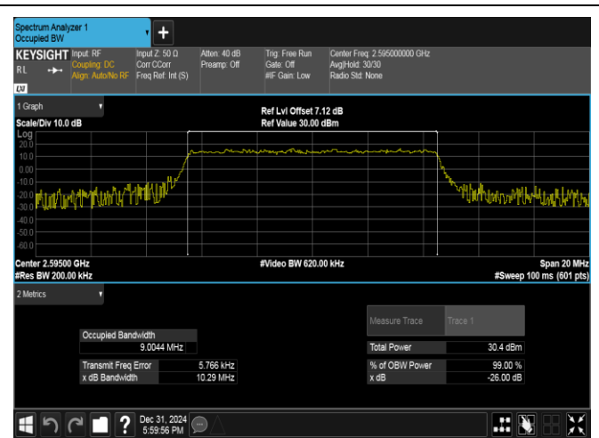
Band38-10MHz-QPSK-38000-50RB#0-PASS
