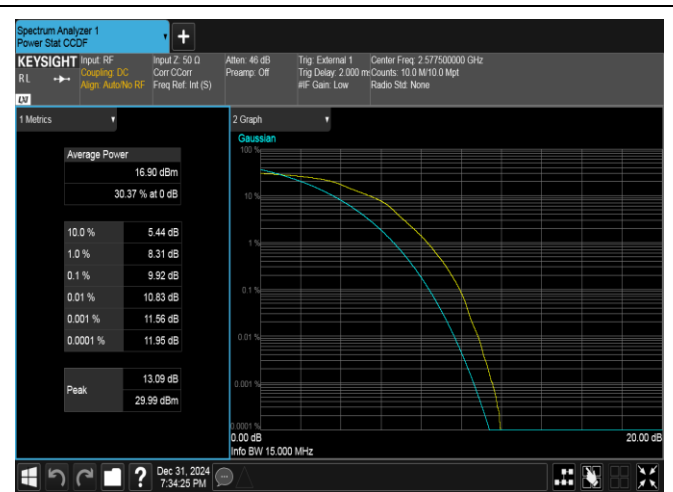
Band38-15MHz-16QAM-37825-75RB#0-PASS
