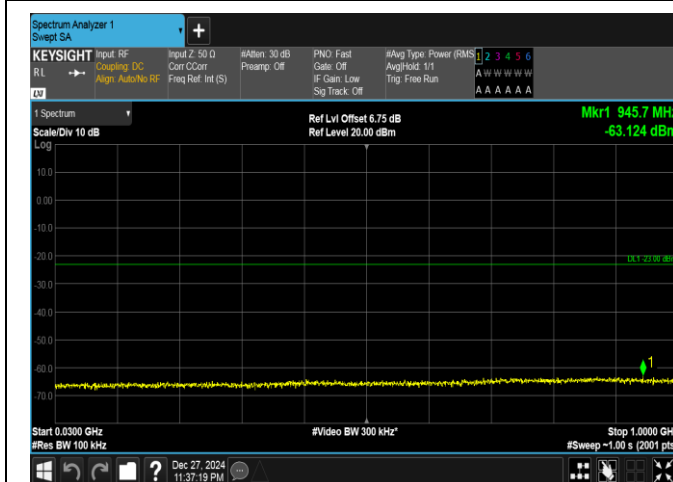
Band25-20MHz-16QAM-26590-1RB#99-30~1000-PASS
