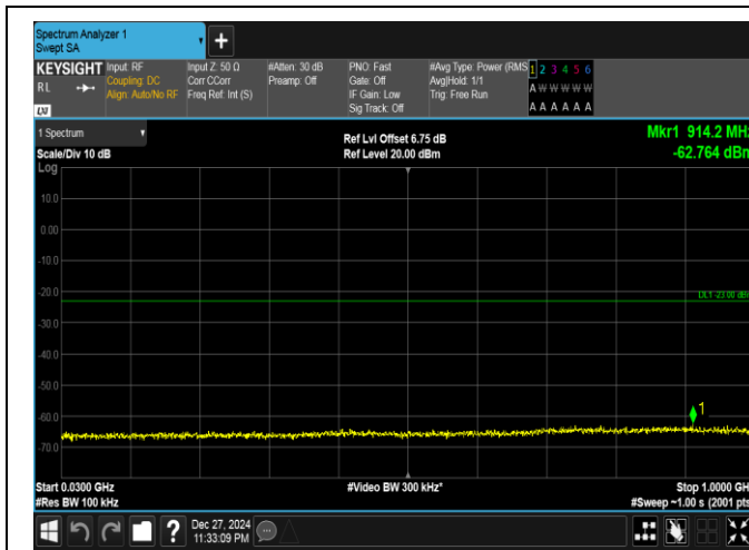
Band25-20MHz-16QAM-26365-100RB#0-30~1000-PASS
