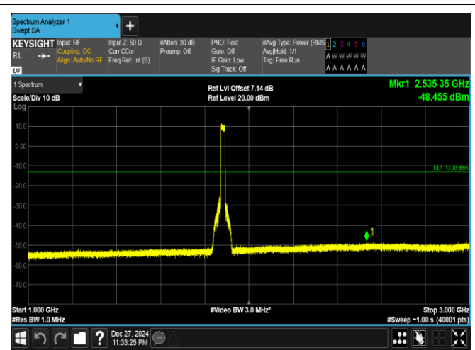
Band25-20MHz-16QAM-26365-100RB#0-1000~3000-PASS S
