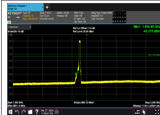
Band25-20MHz-16QAM-26590-100RB#0-1000~3000-PAS
