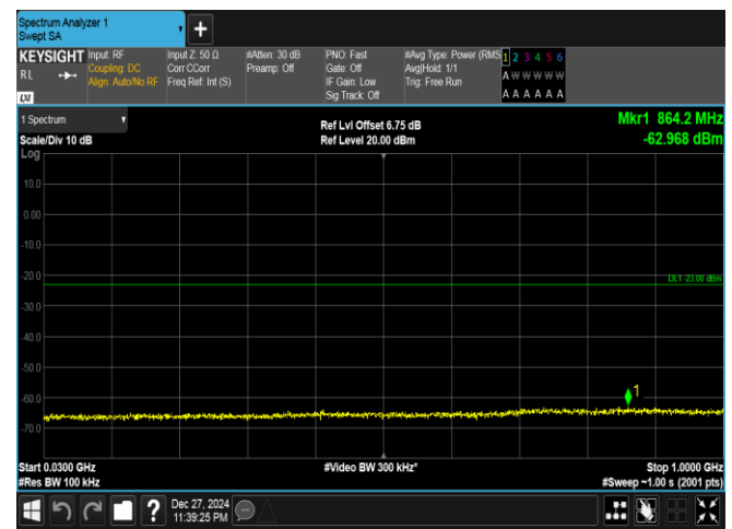
Band25-20MHz-16QAM-26590-100RB#0-30~1000-PASS
