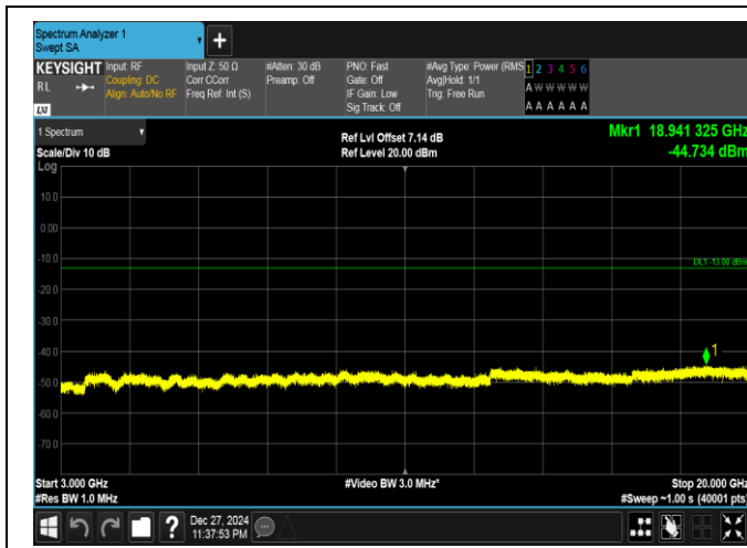
Band25-20MHz-16QAM-26590-1RB#99-3000~20000-PAS
