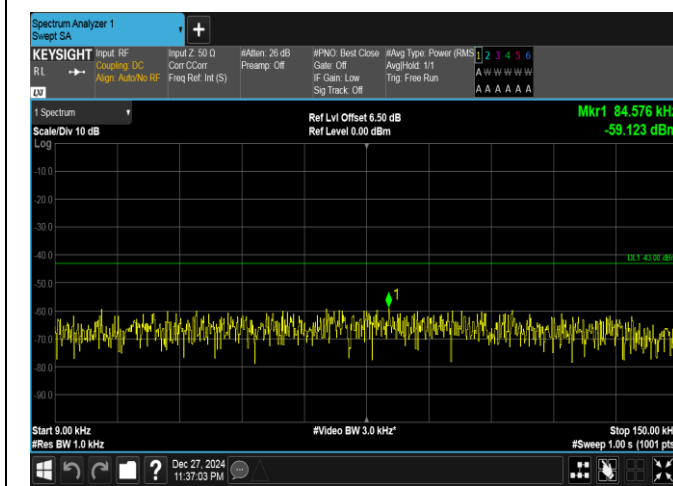
Band25-20MHz-16QAM-26590-1RB#99-0.009~0.15-PASS
