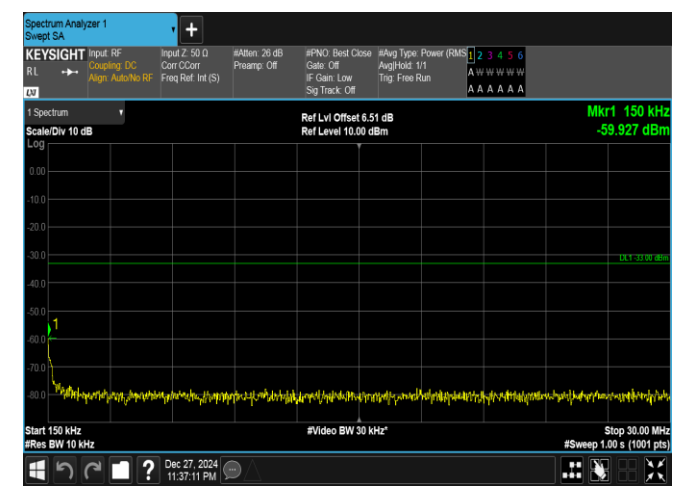
Band25-20MHz-16QAM-26590-1RB#99-0.15~30-PASS
