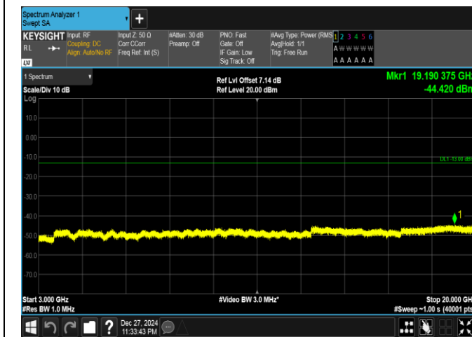
Band25-20MHz-16QAM-26365-100RB#0-3000~20000-PA SS
