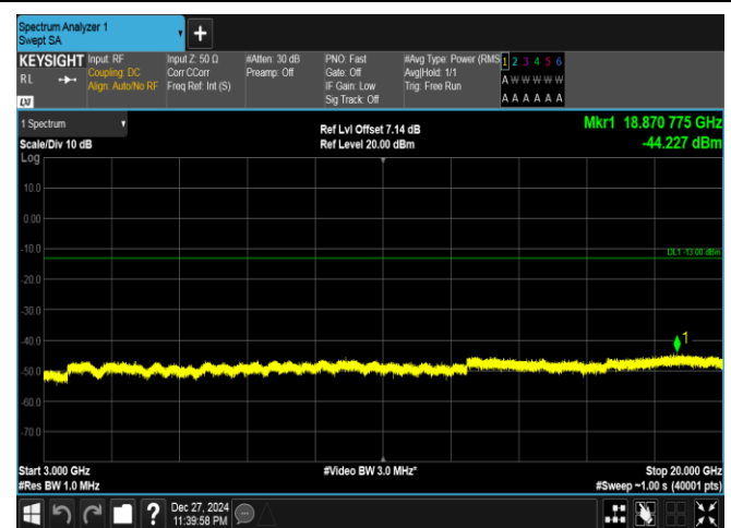
Band25-20MHz-16QAM-26590-100RB#0-3000~20000-PA
