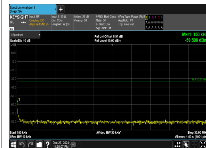
Band25-20MHz-16QAM-26590-1RB#0-0.15~30-PASS
