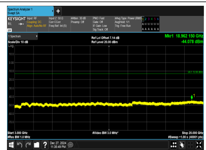
Band25-20MHz-16QAM-26590-1RB#0-3000~20000-PASS
