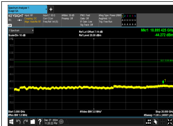
Band25-20MHz-16QAM-26140-1RB#99-3000~20000-PAS
