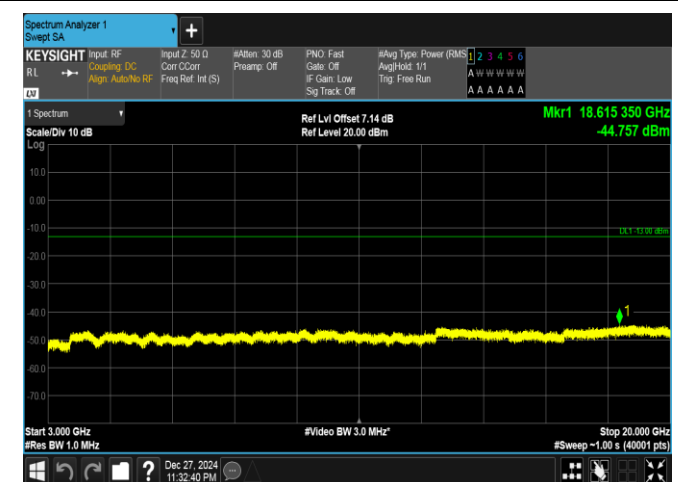
Band25-20MHz-QPSK-26365-100RB#0-3000~20000-PASS
