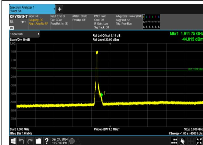
Band25-20MHz-16QAM-26140-100RB#0-1000~3000-PAS
