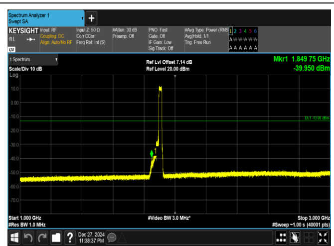
Band25-20MHz-QPSK-26590-100RB#0-1000~3000-PASS
