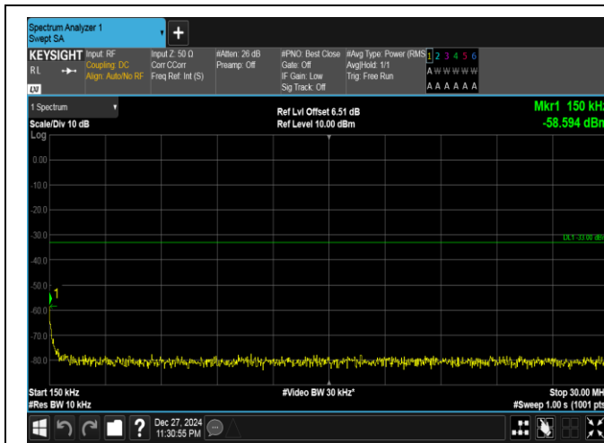
Band25-20MHz-16QAM-26365-1RB#99-0.15~30-PASS
