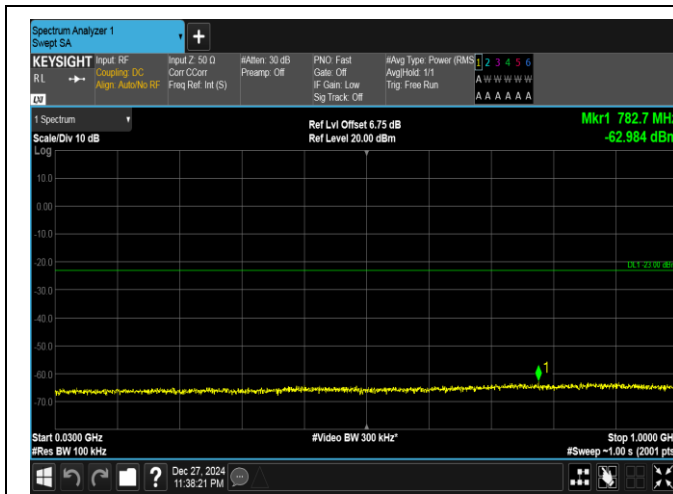
Band25-20MHz-QPSK-26590-100RB#0-30~1000-PASS
