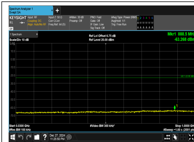
Band25-20MHz-QPSK-26140-100RB#0-30~1000-PASS
