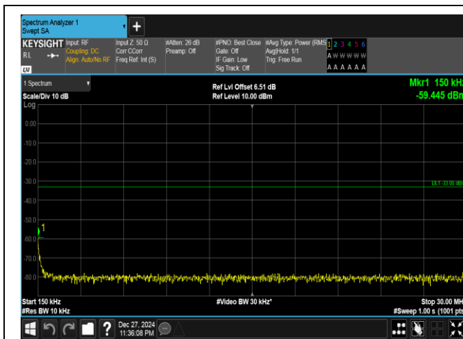
Band25-20MHz-QPSK-26590-1RB#99-0.15~30-PASS
