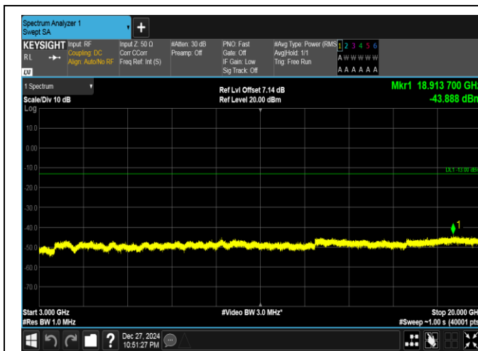
Band25-15MHz-16QAM-26615-1RB#74-3000~20000-PAS S
