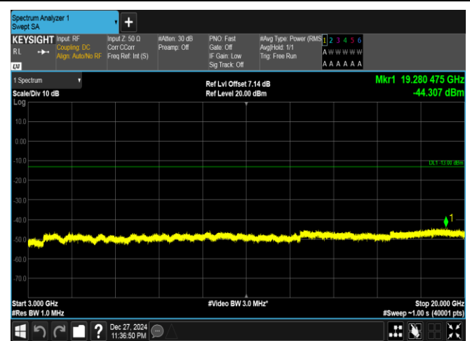
Band25-20MHz-QPSK-26590-1RB#99-3000~20000-PASS
