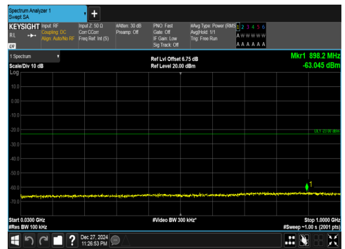
Band25-20MHz-16QAM-26140-100RB#0-30~1000-PASS
