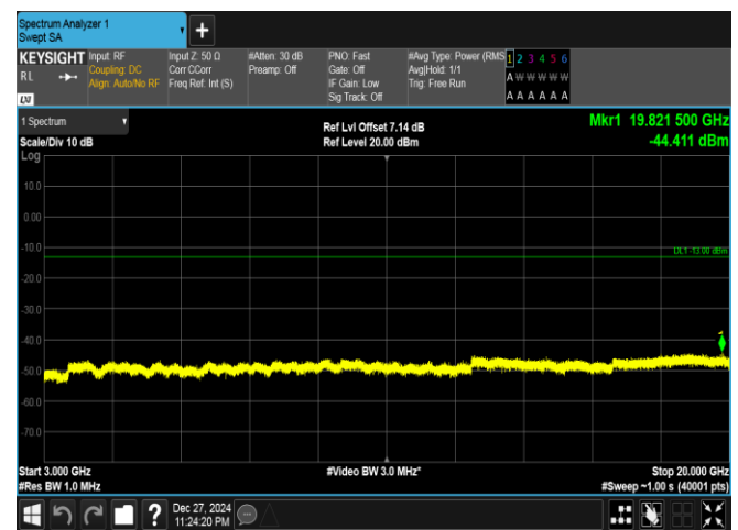
Band25-20MHz-QPSK-26140-1RB#99-3000~20000-PASS
