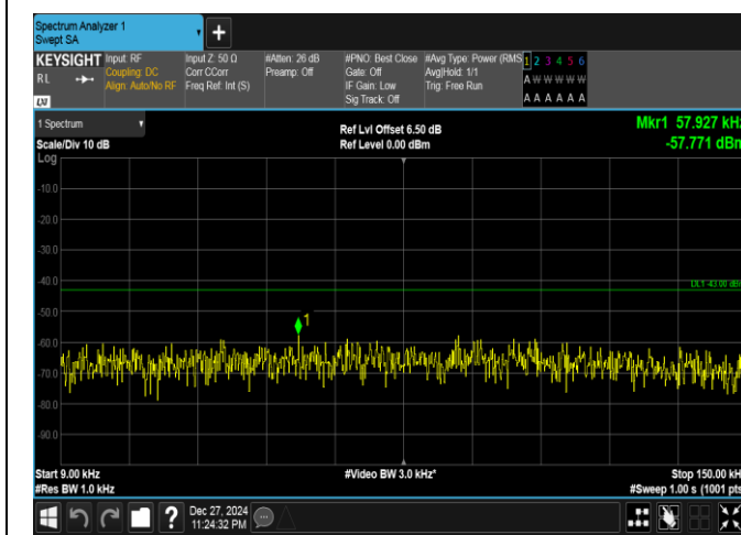
Band25-20MHz-16QAM-26140-1RB#99-0.009~0.15-PASS
