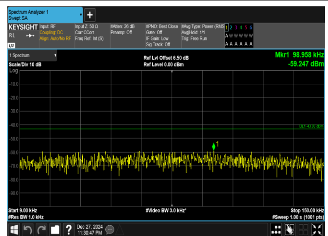
Band25-20MHz-16QAM-26365-1RB#99-0.009~0.15-PASS
