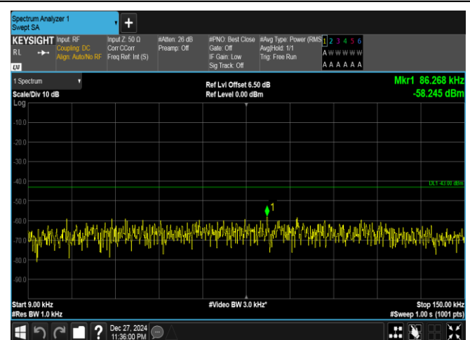
Band25-20MHz-QPSK-26590-1RB#99-0.009~0.15-PASS
