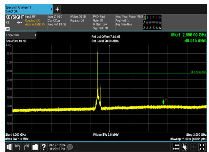
Band25-20MHz-16QAM-26365-1RB#0-1000~3000-PASS
