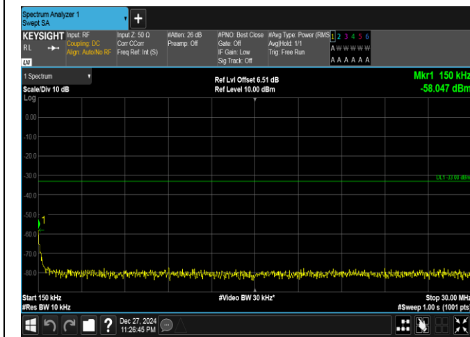
Band25-20MHz-16QAM-26140-100RB#0-0.15~30-PASS
