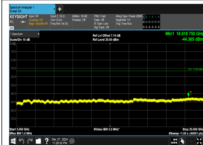
Band25-20MHz-16QAM-26365-1RB#0-3000~20000-PASS
