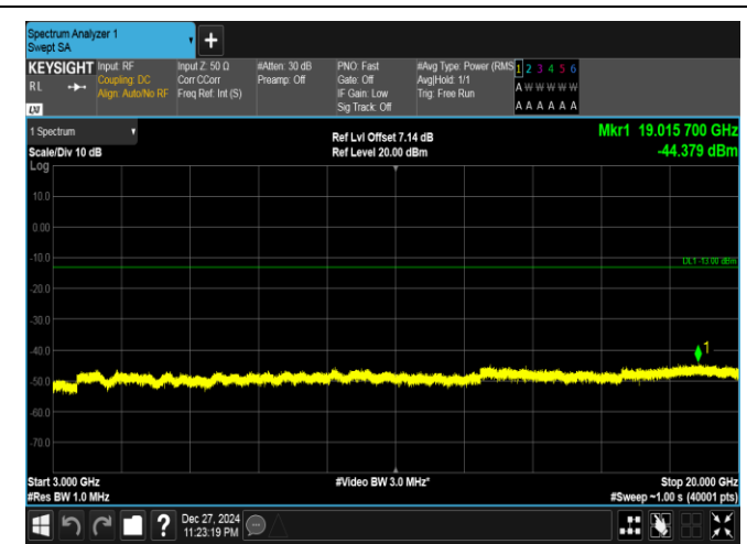
Band25-20MHz-16QAM-26140-1RB#0-3000~20000-PASS
