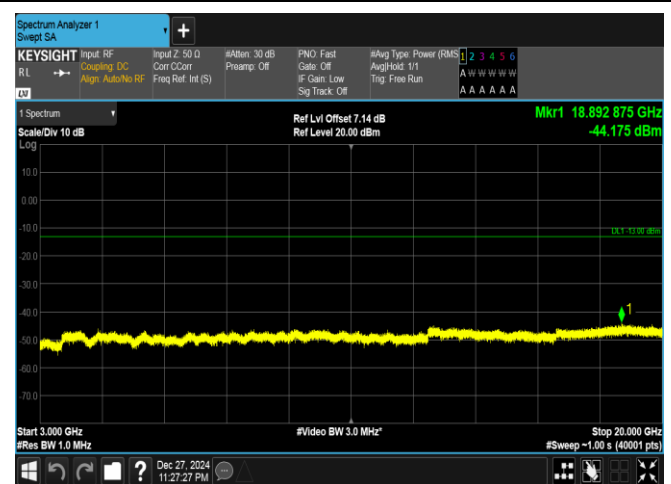
Band25-20MHz-16QAM-26140-100RB#0-3000~20000-PA
