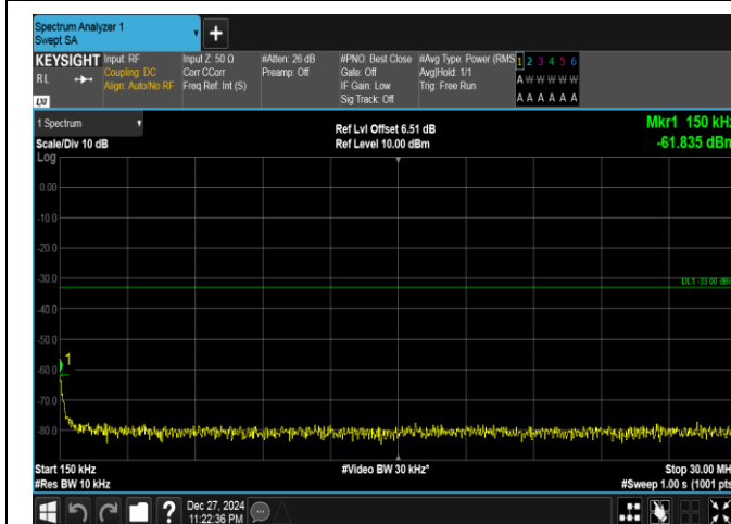
Band25-20MHz-16QAM-26140-1RB#0-0.15~30-PASS
