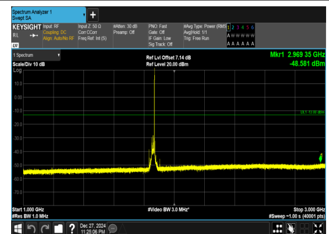
Band25-20MHz-16QAM-26140-1RB#99-1000~3000-PASS
