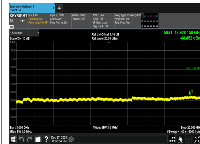
Band25-20MHz-QPSK-26590-100RB#0-3000~20000-PASS
