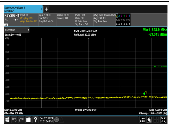
Band25-20MHz-16QAM-26365-1RB#99-30~1000-PASS
