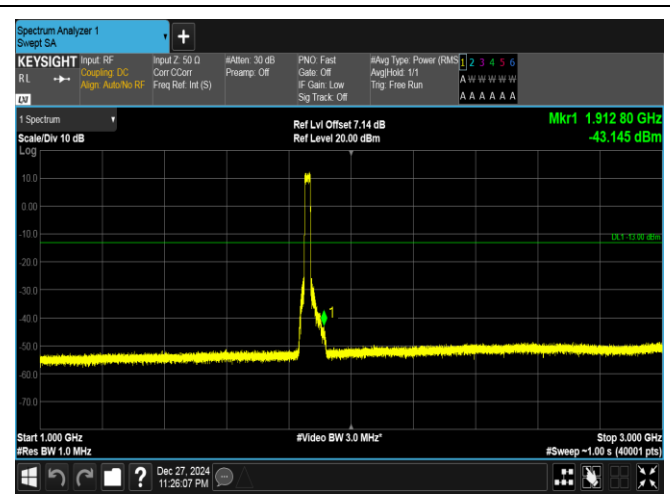
Band25-20MHz-QPSK-26140-100RB#0-1000~3000-PASS
