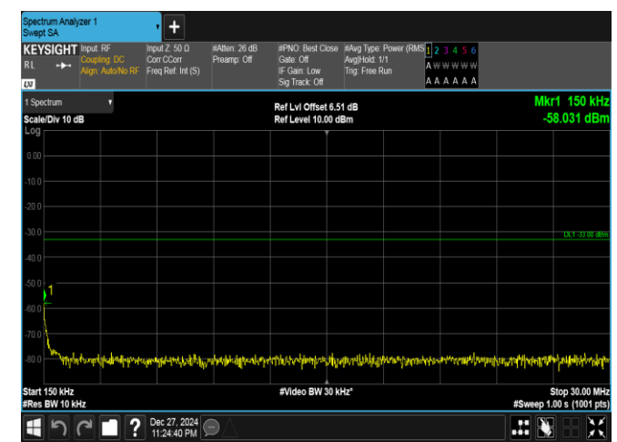
Band25-20MHz-16QAM-26140-1RB#99-0.15~30-PASS
