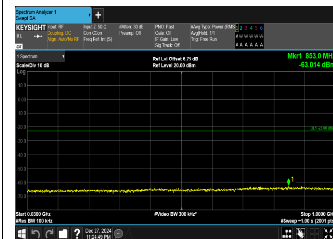
Band25-20MHz-16QAM-26140-1RB#99-30~1000-PASS
