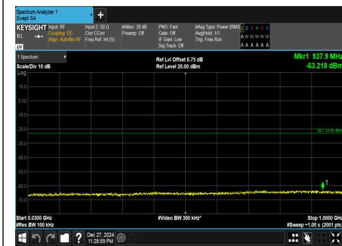
Band25-20MHz-16QAM-26365-1RB#0-30~1000-PASS
