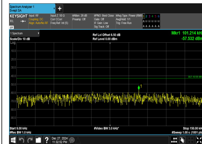
Band25-20MHz-16QAM-26365-100RB#0-0.009~0.15-PAS S
