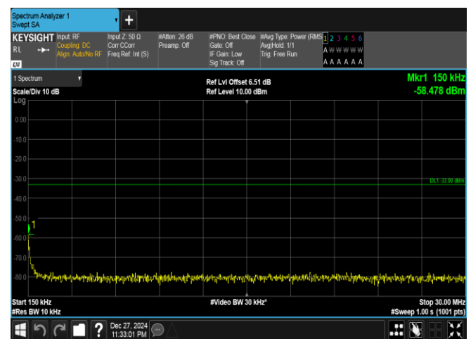
Band25-20MHz-16QAM-26365-100RB#0-0.15~30-PASS
