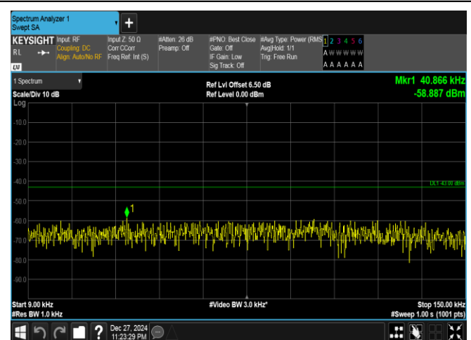
Band25-20MHz-QPSK-26140-1RB#99-0.009~0.15-PASS
