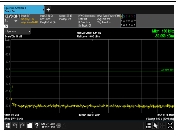
Band25-20MHz-16QAM-26365-1RB#0-0.15~30-PASS
