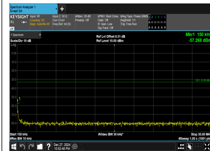
Band25-15MHz-16QAM-26615-75RB#0-0.15~30-PASS
