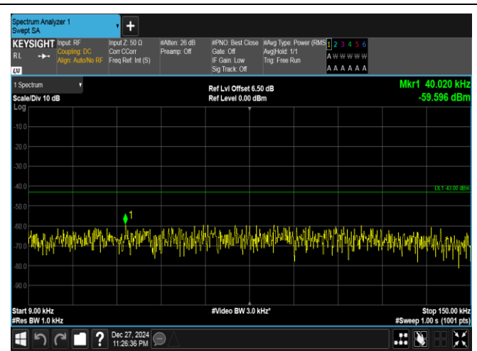
Band25-20MHz-16QAM-26140-100RB#0-0.009~0.15-PAS
