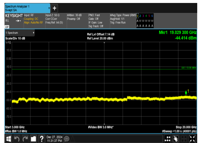
Band25-20MHz-16QAM-26365-1RB#99-3000~20000-PAS S
