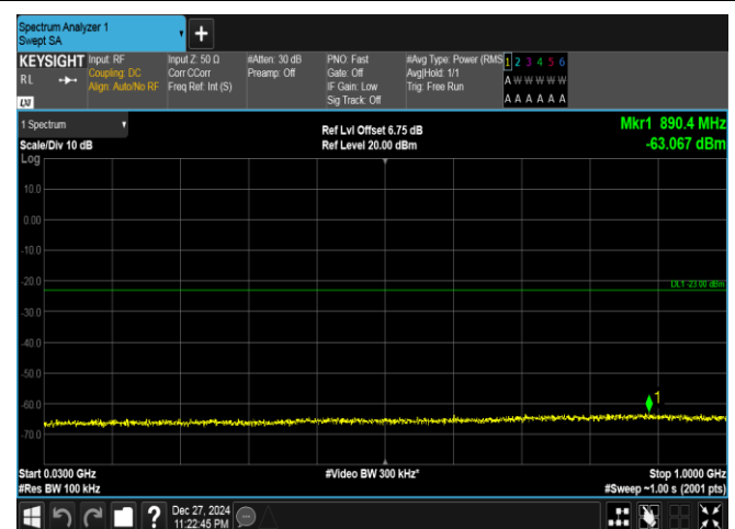
Band25-20MHz-16QAM-26140-1RB#0-30~1000-PASS
