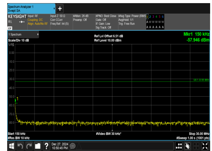
Band25-15MHz-16QAM-26615-1RB#74-0.15~30-PASS
