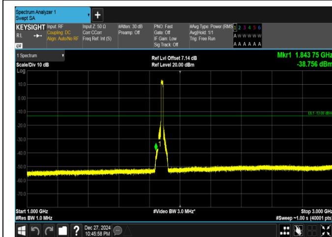
Band25-15MHz-QPSK-26365-75RB#0-1000~3000-PASS
