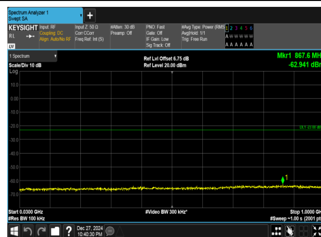
Band25-15MHz-16QAM-26115-75RB#0-30~1000-PASS
