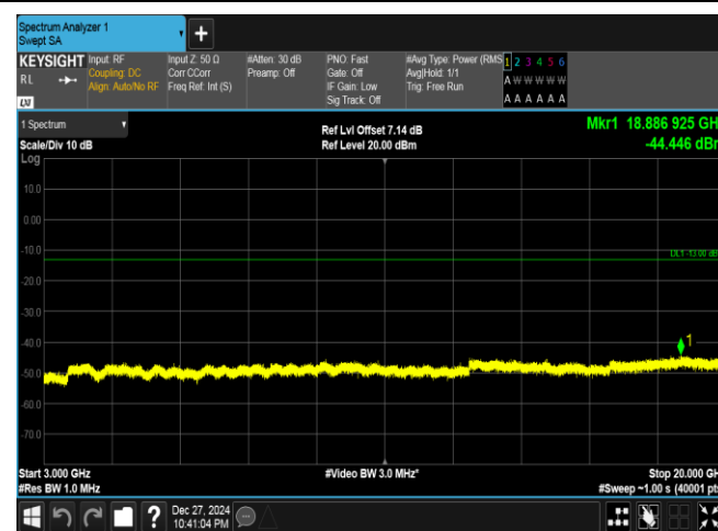
Band25-15MHz-16QAM-26115-75RB#0-3000~20000-PAS S
