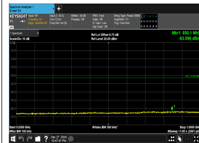
Band25-15MHz-QPSK-26615-1RB#0-30~1000-PASS
