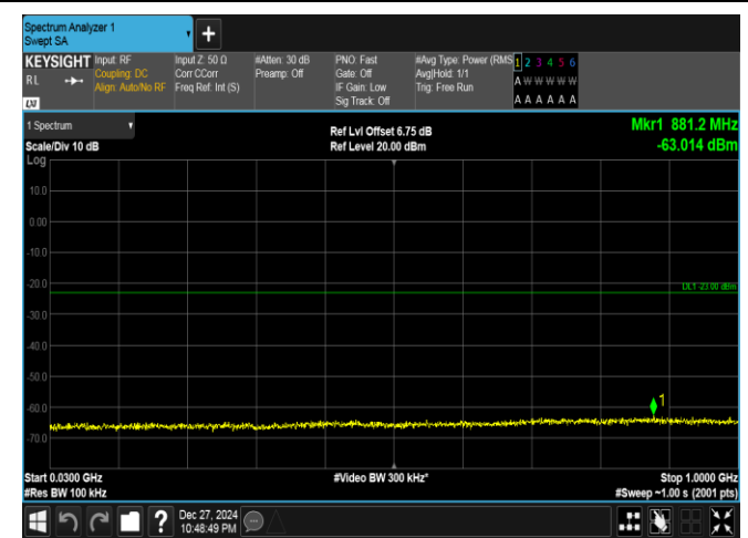
Band25-15MHz-16QAM-26615-1RB#0-30~1000-PASS
