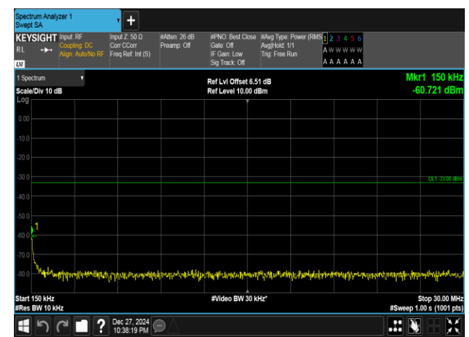
Band25-15MHz-16QAM-26115-1RB#74-0.15~30-PASS
