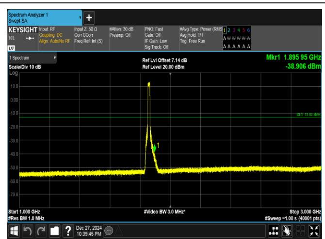
Band25-15MHz-QPSK-26115-75RB#0-1000~3000-PASS
