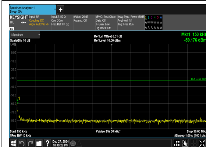
Band25-15MHz-16QAM-26115-75RB#0-0.15~30-PASS
