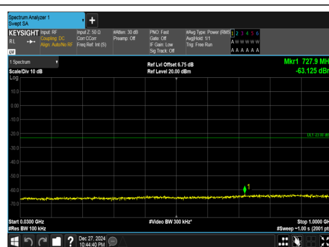
Band25-15MHz-16QAM-26365-1RB#74-30~1000-PASS
