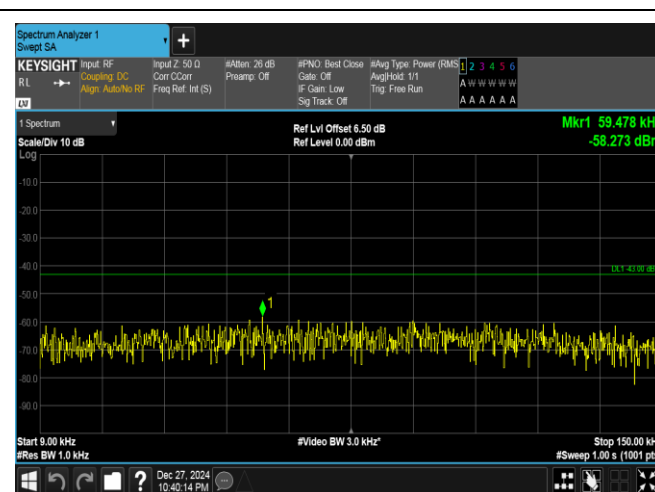
Band25-15MHz-16QAM-26115-75RB#0-0.009~0.15-PASS
