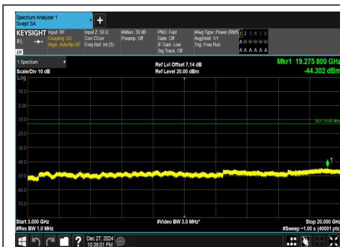
Band25-15MHz-16QAM-26115-1RB#74-3000~20000-PAS S
