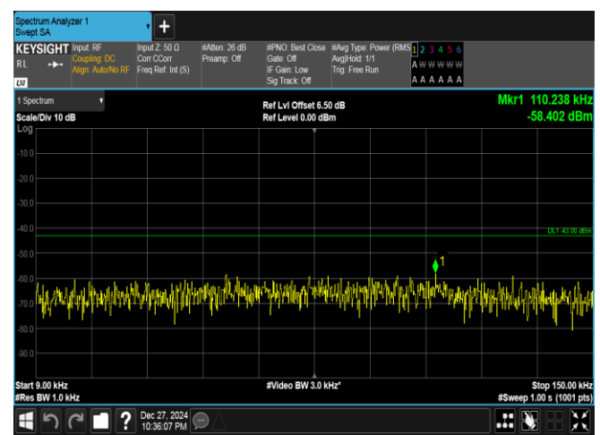
Band25-15MHz-16QAM-26115-1RB#0-0.009~0.15-PASS
