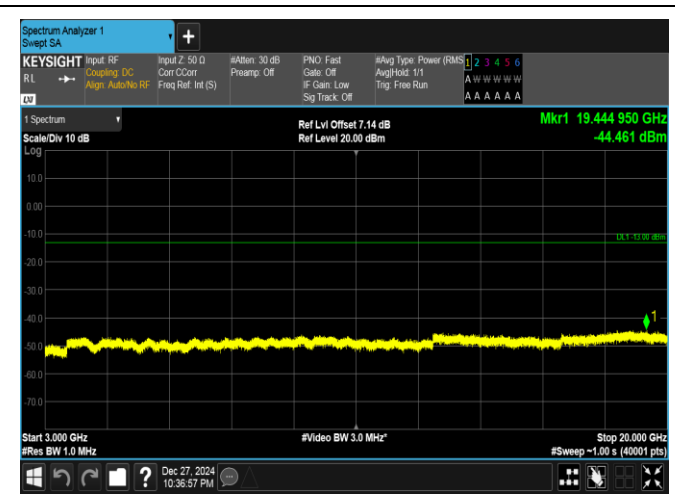
Band25-15MHz-16QAM-26115-1RB#0-3000~20000-PASS
