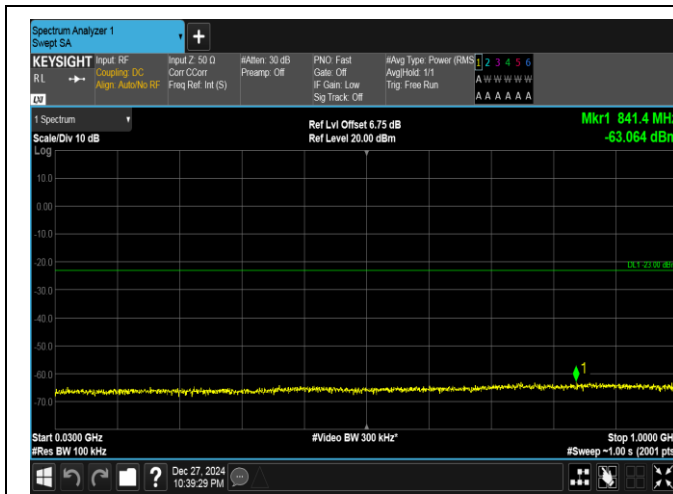
Band25-15MHz-QPSK-26115-75RB#0-30~1000-PASS
