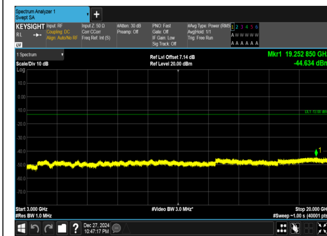
Band25-15MHz-16QAM-26365-75RB#0-3000~20000-PAS S
