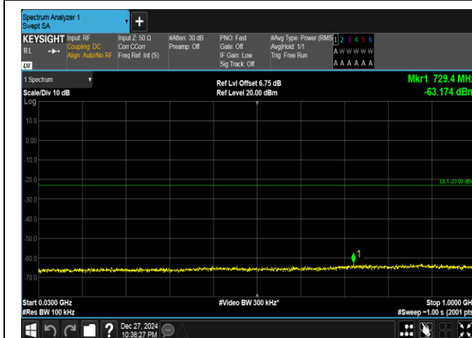
Band25-15MHz-16QAM-26115-1RB#74-30~1000-PASS
