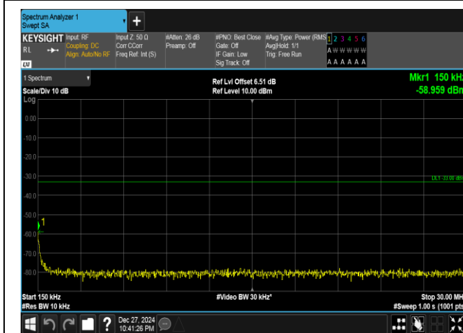
Band25-15MHz-QPSK-26365-1RB#0-0.15~30-PASS
