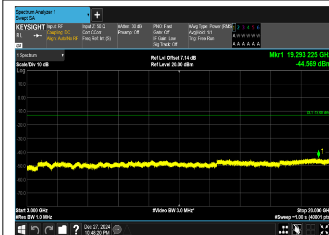
Band25-15MHz-QPSK-26615-1RB#0-3000~20000-PASS
