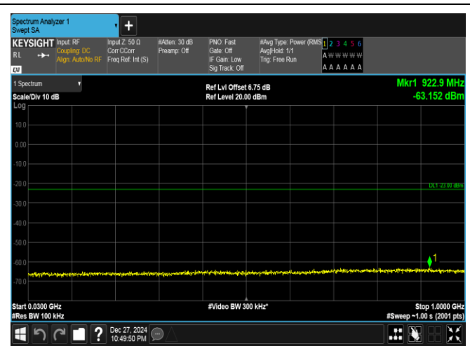
Band25-15MHz-QPSK-26615-1RB#74-30~1000-PASS
