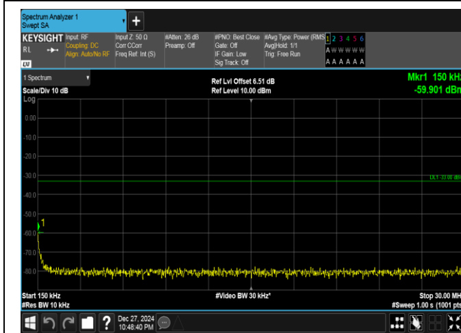
Band25-15MHz-16QAM-26615-1RB#0-0.15~30-PASS
