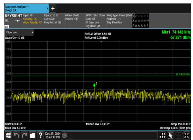
Band25-15MHz-QPSK-26365-1RB#0-0.009~0.15-PASS
