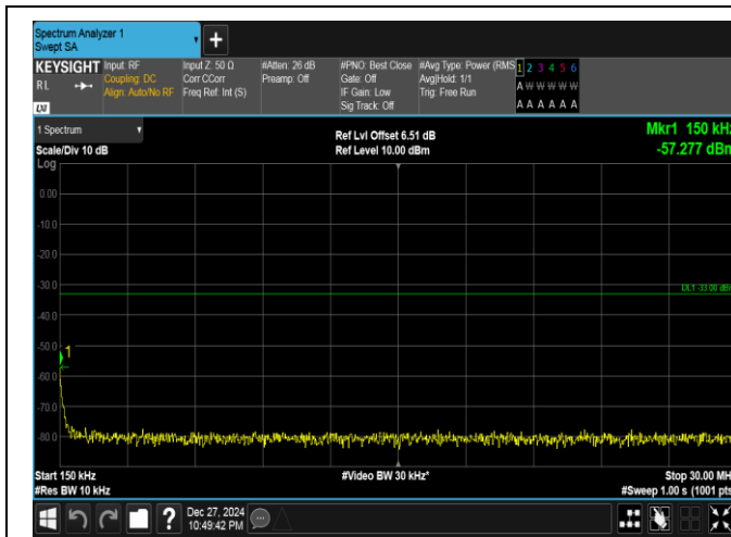
Band25-15MHz-QPSK-26615-1RB#74-0.15~30-PASS
