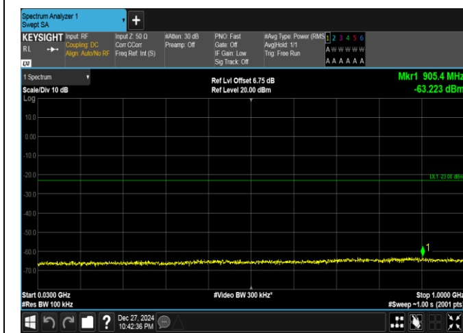
Band25-15MHz-16QAM-26365-1RB#0-30~1000-PASS
