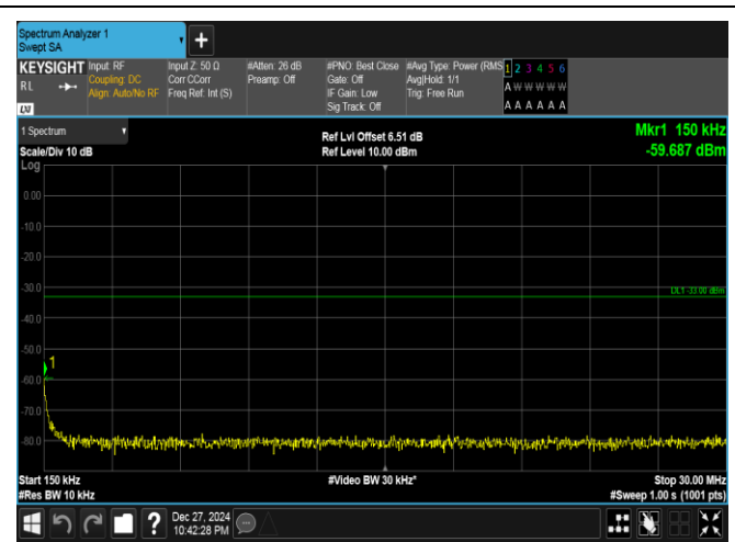
Band25-15MHz-16QAM-26365-1RB#0-0.15~30-PASS
