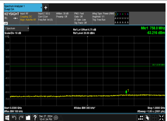
Band25-15MHz-QPSK-26365-1RB#0-30~1000-PASS
