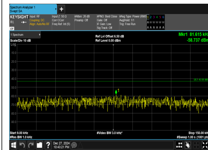
Band25-15MHz-QPSK-26365-1RB#74-0.009~0.15-PASS
