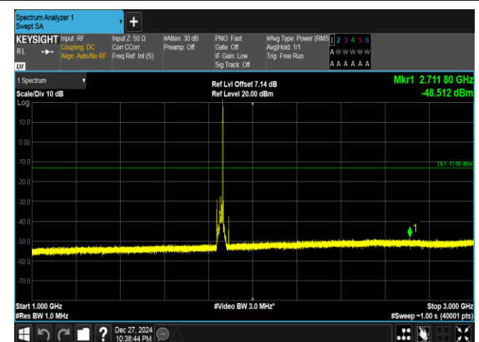
Band25-15MHz-16QAM-26115-1RB#74-1000~3000-PASS
