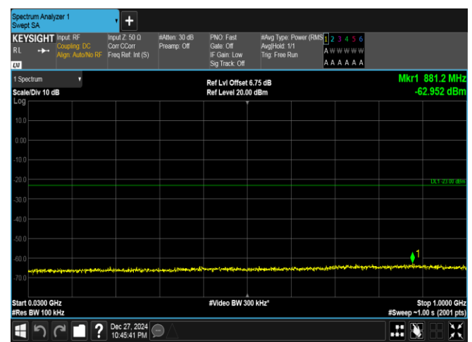
Band25-15MHz-QPSK-26365-75RB#0-30~1000-PASS
