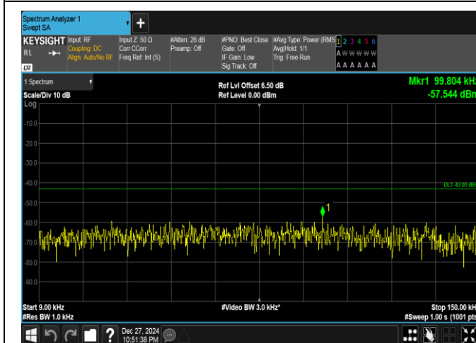
Band25-15MHz-QPSK-26615-75RB#0-0.009~0.15-PASS
