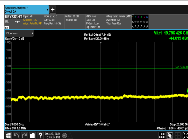
Band25-15MHz-16QAM-26365-1RB#74-3000~20000-PASS S
