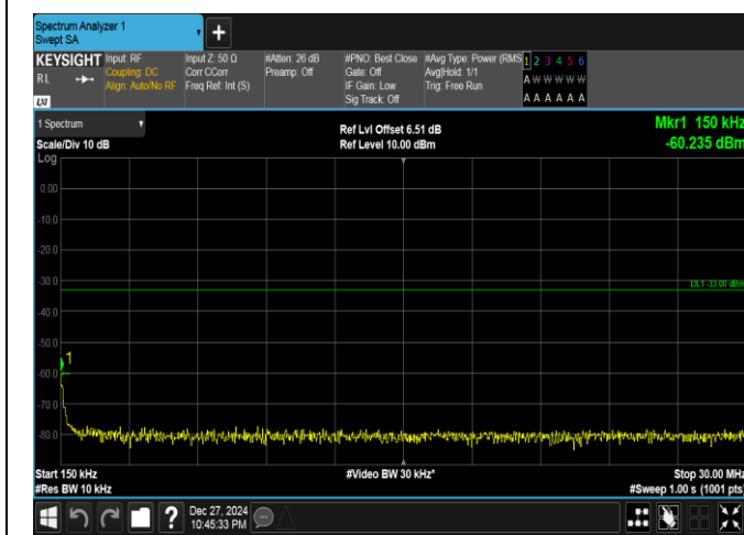
Band25-15MHz-QPSK-26365-75RB#0-0.15~30-PASS
