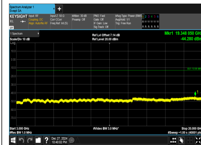
Band25-15MHz-QPSK-26115-75RB#0-3000~20000-PASS
