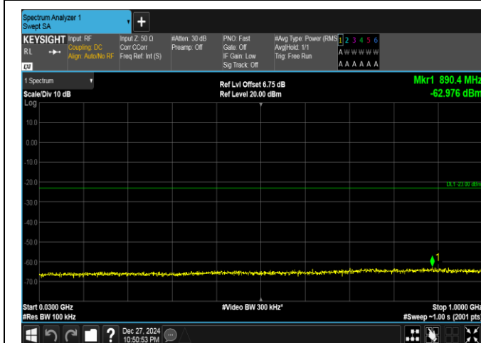
Band25-15MHz-16QAM-26615-1RB#74-30~1000-PASS
