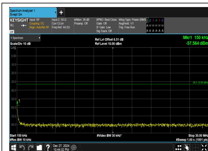
Band25-15MHz-16QAM-26365-1RB#74-0.15~30-PASS
