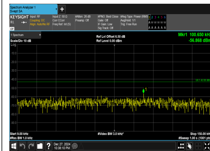
Band25-15MHz-16QAM-26115-1RB#74-0.009~0.15-PASS
