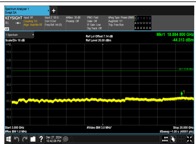
Band25-15MHz-QPSK-26365-1RB#0-3000~20000-PASS
