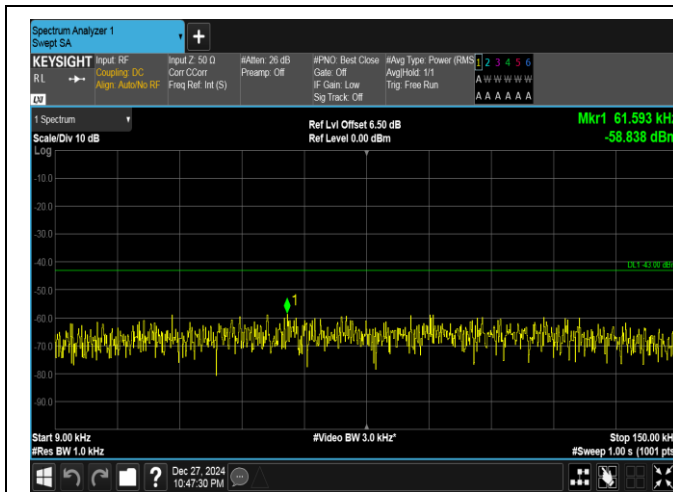
Band25-15MHz-QPSK-26615-1RB#0-0.009~0.15-PASS
