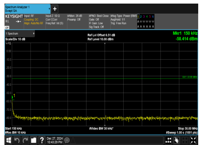
Band25-15MHz-QPSK-26365-1RB#74-0.15~30-PASS
