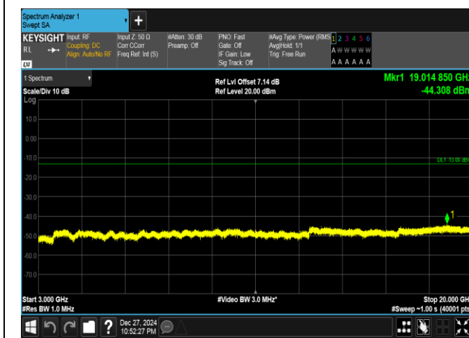
Band25-15MHz-QPSK-26615-75RB#0-3000~20000-PASS
