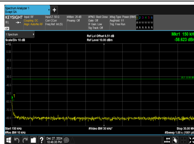
Band25-15MHz-16QAM-26365-75RB#0-0.15~30-PASS
