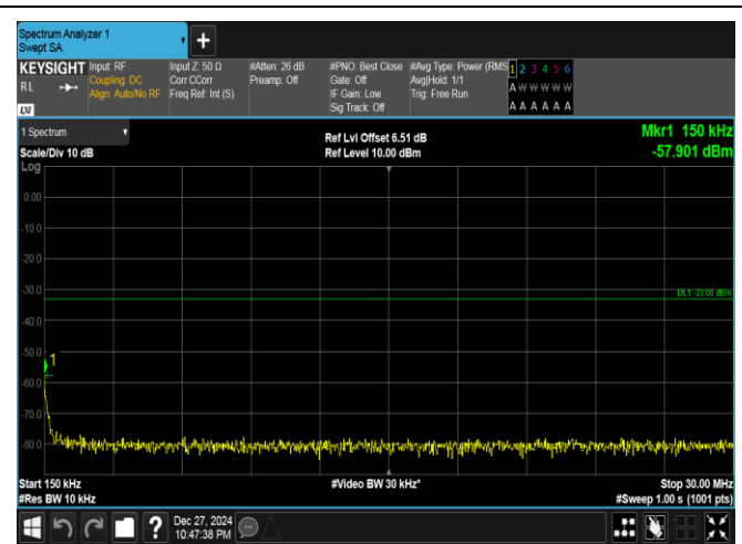
Band25-15MHz-QPSK-26615-1RB#0-0.15~30-PASS
