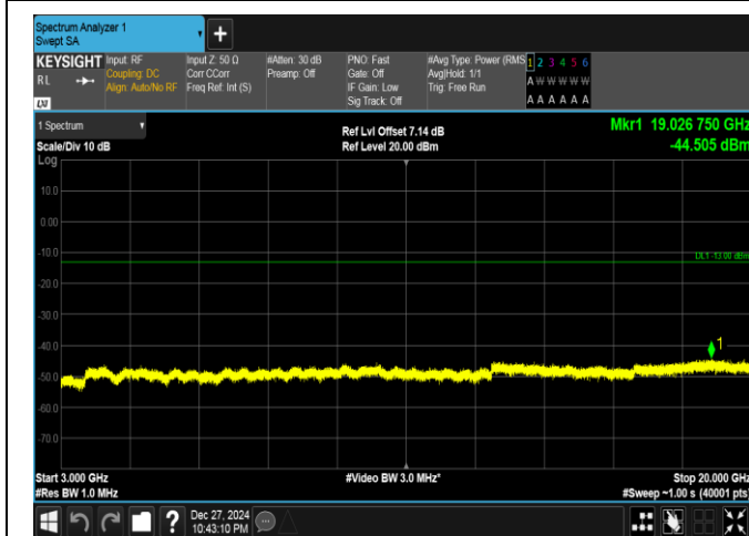
Band25-15MHz-16QAM-26365-1RB#0-3000~20000-PASS
