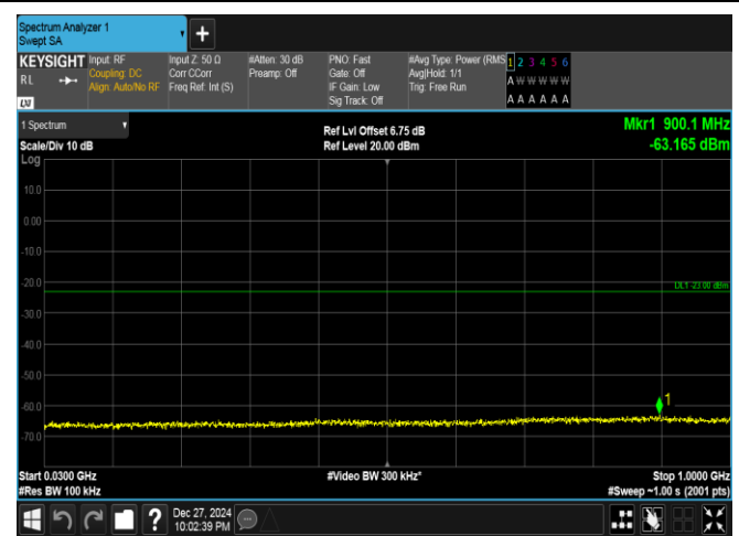
Band25-10MHz-16QAM-26640-1RB#0-30~1000-PASS
