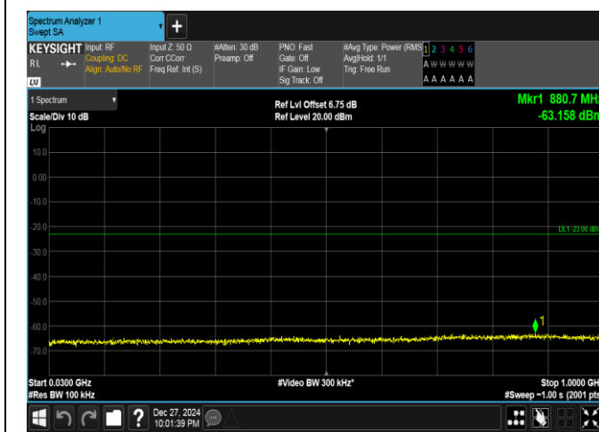
Band25-10MHz-QPSK-26640-1RB#0-30~1000-PASS
