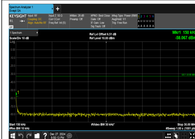
Band25-10MHz-16QAM-26090-1RB#0-0.15~30-PASS
