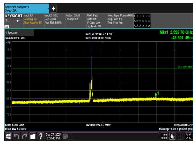
Band25-10MHz-16QAM-26365-1RB#0-1000~3000-PASS
