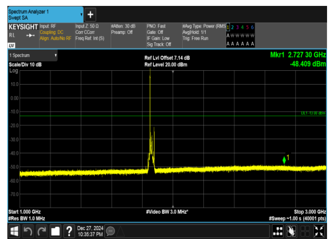
Band25-15MHz-QPSK-26115-1RB#0-1000~3000-PASS
