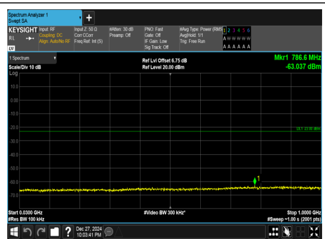
Band25-10MHz-QPSK-26640-1RB#49-30~1000-PASS
