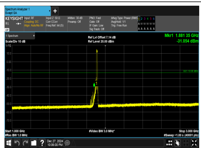
Band25-10MHz-QPSK-26640-50RB#0-1000~3000-PASS
