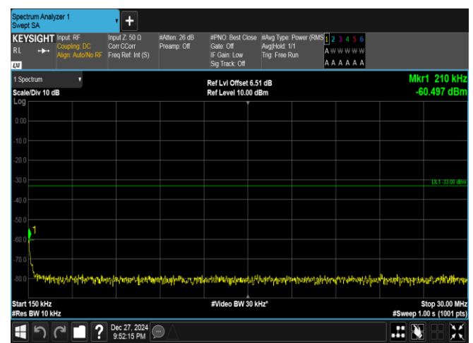
Band25-10MHz-16QAM-26090-1RB#49-0.15~30-PASS
