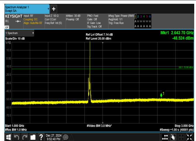
Band25-10MHz-16QAM-26090-1RB#49-1000~3000-PASS
