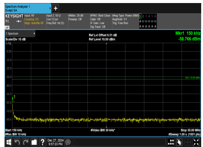
Band25-10MHz-QPSK-26365-1RB#49-0.15~30-PASS
