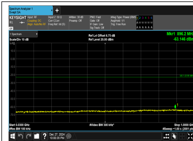
Band25-10MHz-16QAM-26365-50RB#0-30~1000-PASS
