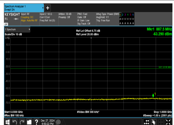
Band25-10MHz-16QAM-26090-1RB#0-30~1000-PASS
