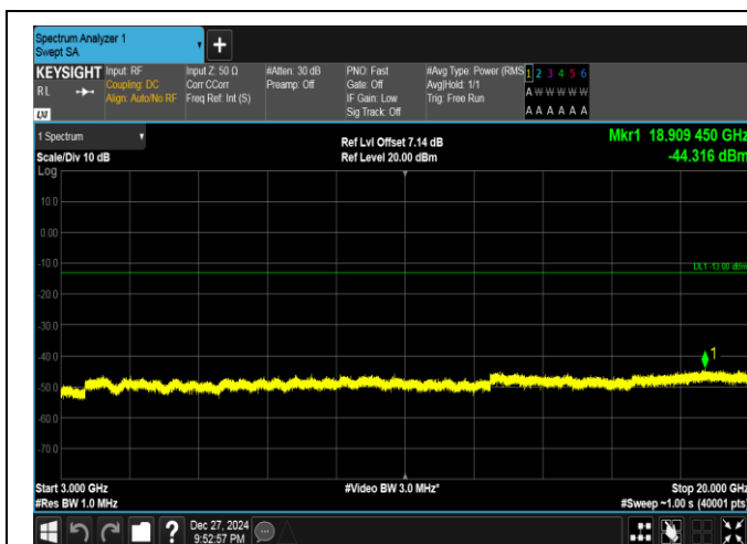
Band25-10MHz-16QAM-26090-1RB#49-3000~20000-PAS
