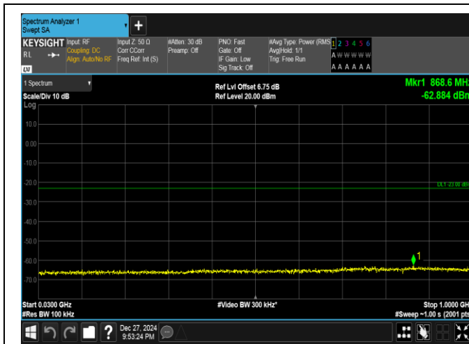
Band25-10MHz-QPSK-26090-50RB#0-30~1000-PASS
