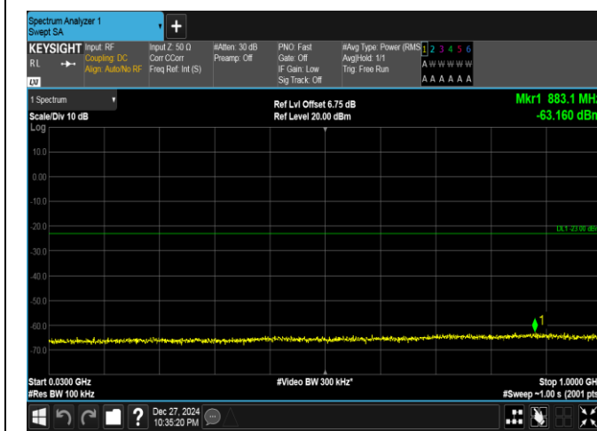
Band25-15MHz-QPSK-26115-1RB#0-30~1000-PASS
