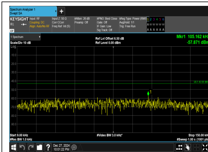
Band25-10MHz-QPSK-26640-1RB#0-0.009~0.15-PASS
