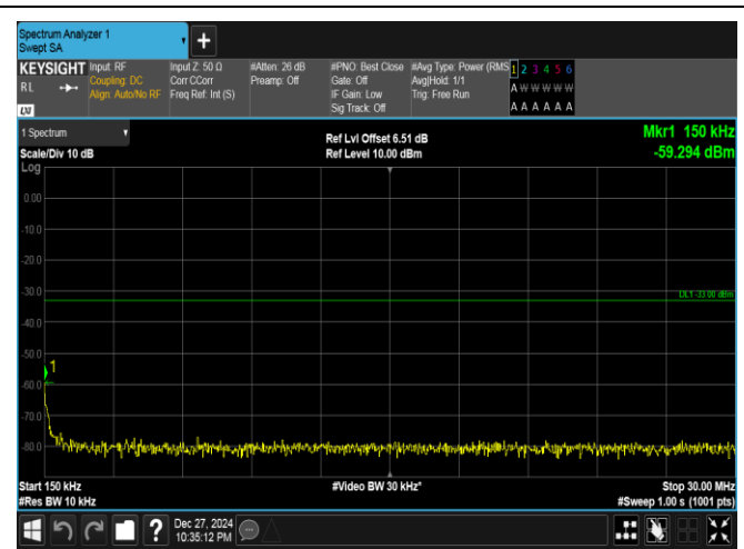
Band25-15MHz-QPSK-26115-1RB#0-0.15~30-PASS
