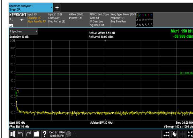
Band25-10MHz-16QAM-26640-50RB#0-0.15~30-PASS
