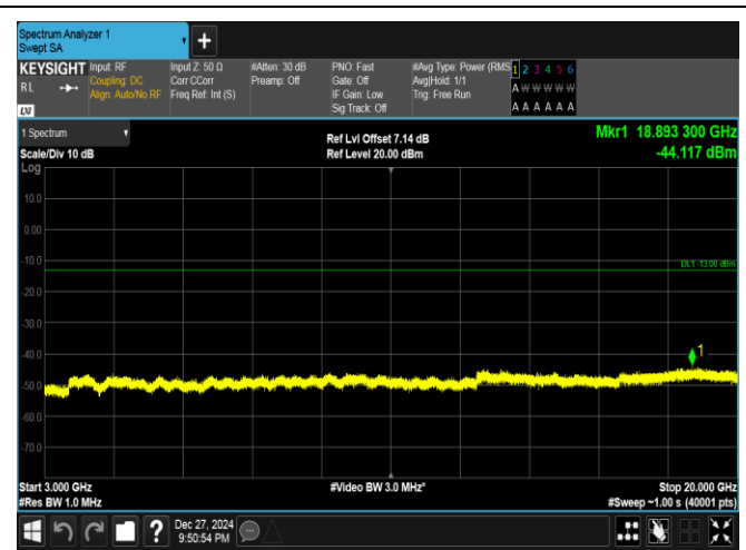
Band25-10MHz-16QAM-26090-1RB#0-3000~20000-PASS
