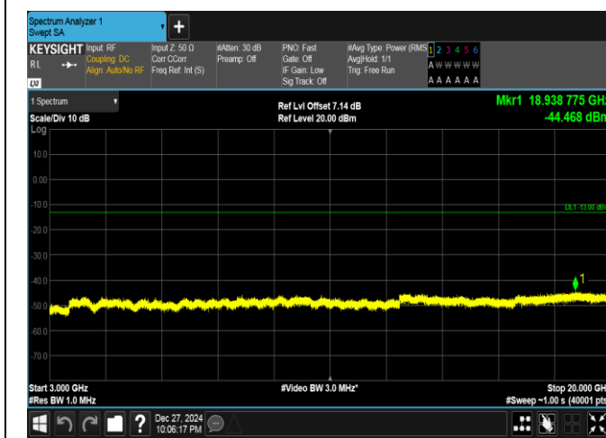
Band25-10MHz-QPSK-26640-50RB#0-3000~20000-PASS
