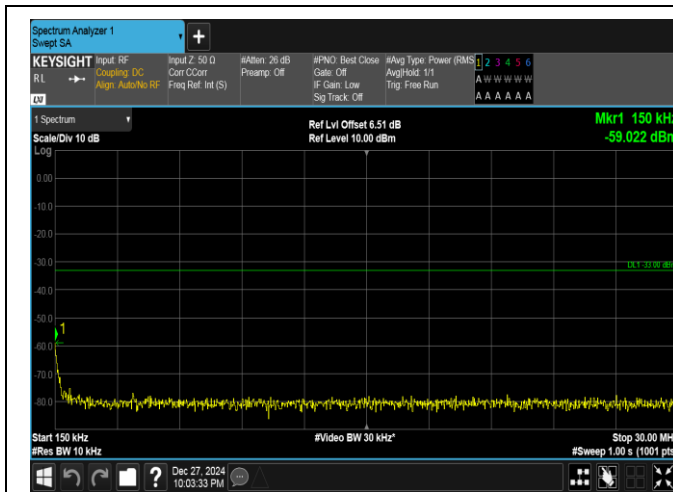
Band25-10MHz-QPSK-26640-1RB#49-0.15~30-PASS
