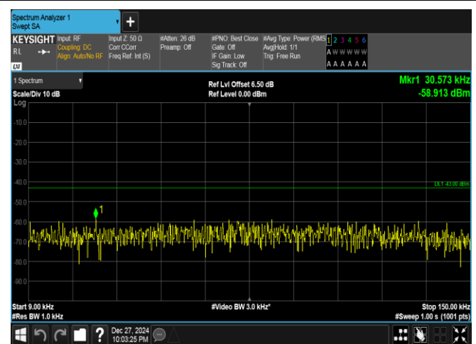
Band25-10MHz-QPSK-26640-1RB#49-0.009~0.15-PASS
