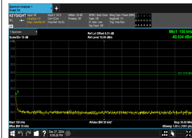
Band25-10MHz-QPSK-26365-50RB#0-0.15~30-PASS
