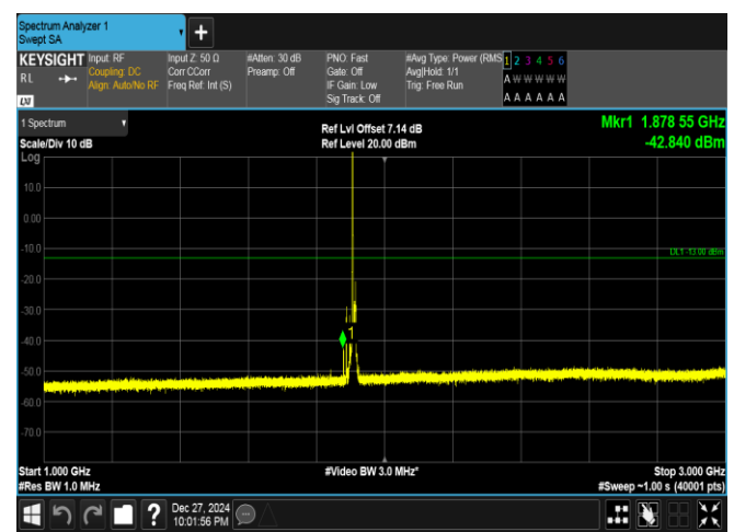
Band25-10MHz-QPSK-26640-1RB#0-1000~3000-PASS
