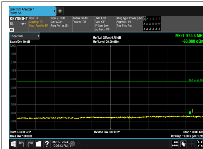
Band25-10MHz-QPSK-26640-50RB#0-30~1000-PASS
