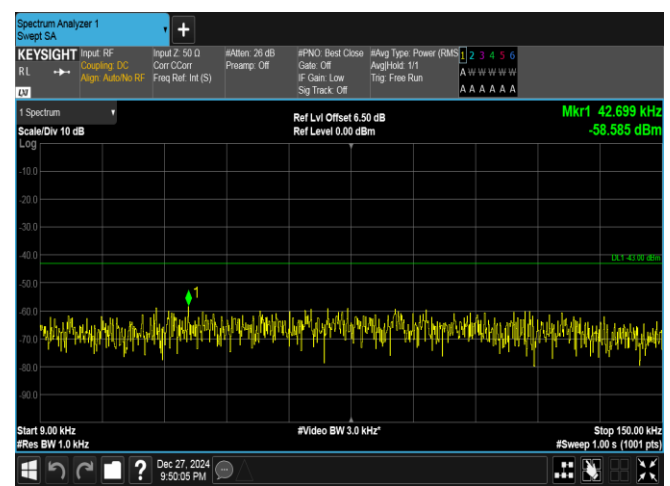
Band25-10MHz-16QAM-26090-1RB#0-0.009~0.15-PASS
