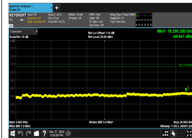
Band25-10MHz-QPSK-26090-50RB#0-3000~20000-PASS
