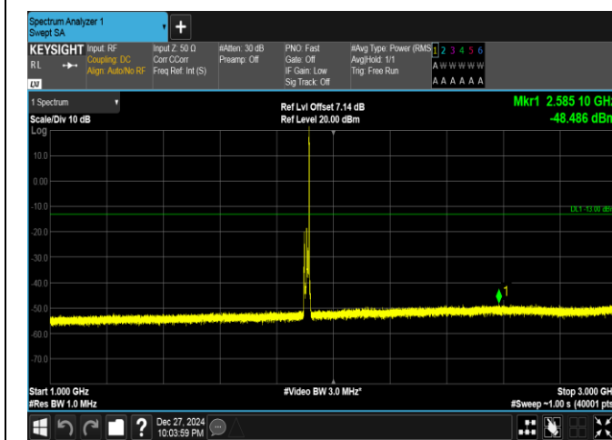
Band25-10MHz-QPSK-26640-1RB#49-1000~3000-PASS
