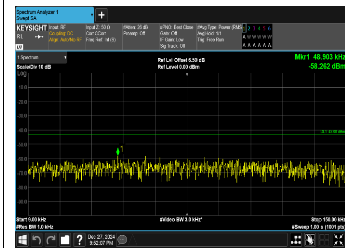
Band25-10MHz-16QAM-26090-1RB#49-0.009~0.15-PASS
