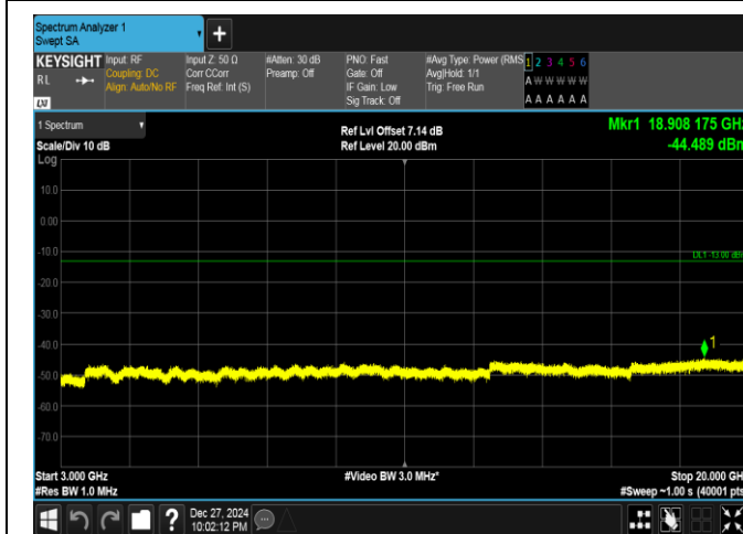
Band25-10MHz-QPSK-26640-1RB#0-3000~20000-PASS
