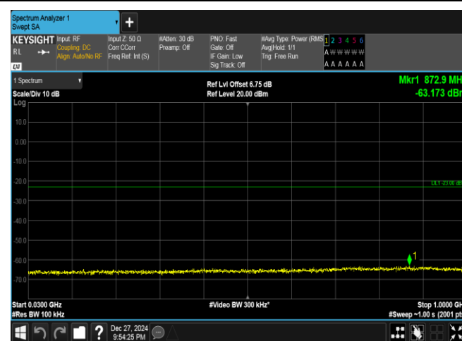
Band25-10MHz-16QAM-26090-50RB#0-30~1000-PASS
