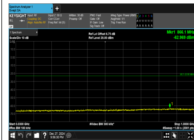
Band25-10MHz-16QAM-26365-1RB#0-30~1000-PASS
