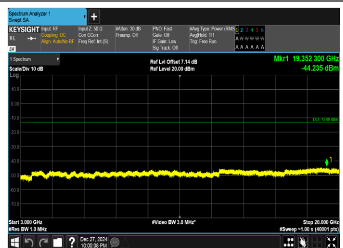
Band25-10MHz-QPSK-26365-50RB#0-3000~20000-PASS
