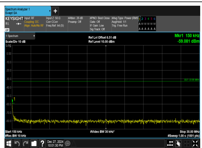
Band25-10MHz-QPSK-26640-1RB#0-0.15~30-PASS
