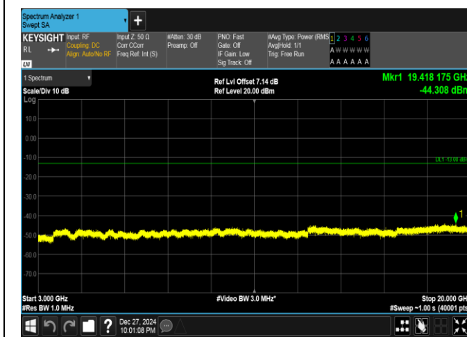
Band25-10MHz-16QAM-26365-50RB#0-3000~20000-PAS S
