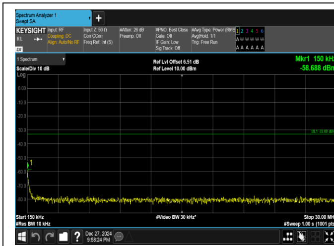
Band25-10MHz-16QAM-26365-1RB#49-0.15~30-PASS
