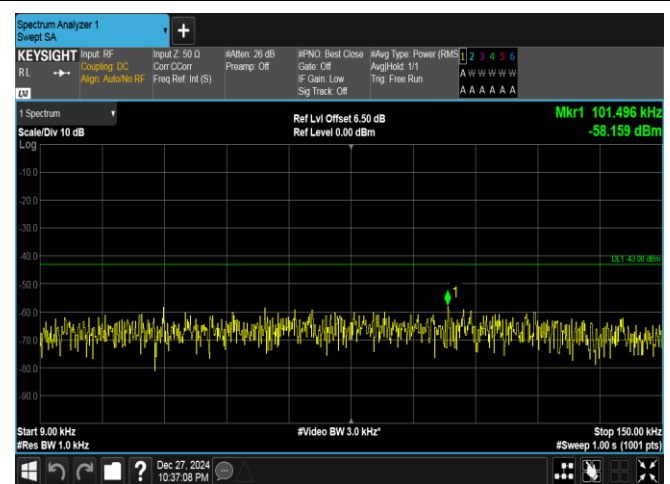
Band25-15MHz-QPSK-26115-1RB#74-0.009~0.15-PASS
