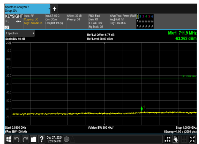
Band25-10MHz-QPSK-26365-50RB#0-30~1000-PASS
