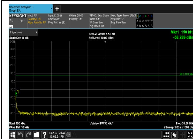
Band25-10MHz-16QAM-26640-1RB#0-0.15~30-PASS
