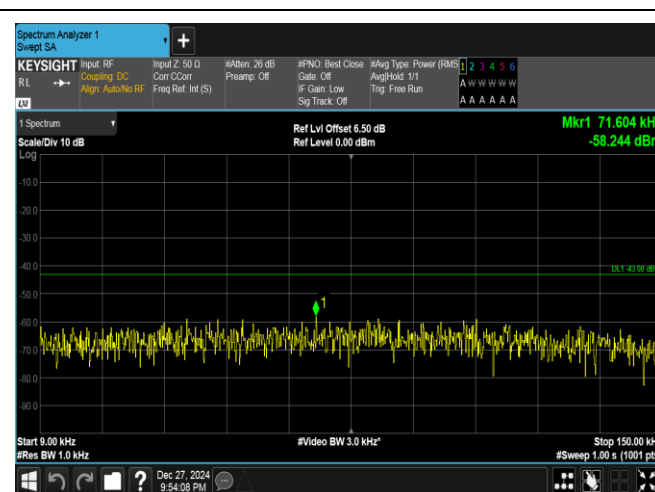
Band25-10MHz-16QAM-26090-50RB#0-0.009~0.15-PASS
