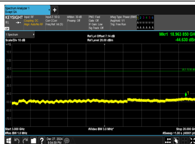
Band25-10MHz-16QAM-26090-50RB#0-3000~20000-PAS
