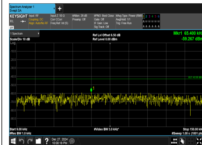
Band25-10MHz-16QAM-26365-50RB#0-0.009~0.15-PASS
