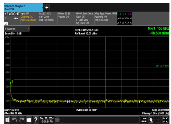
Band25-10MHz-16QAM-26640-1RB#49-0.15~30-PASS
