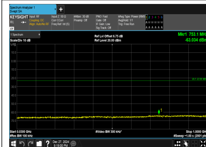
Band25-5MHz-16QAM-26665-1RB#24-30~1000-PASS
