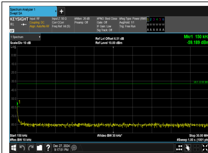
Band25-5MHz-QPSK-26665-1RB#24-0.15~30-PASS
