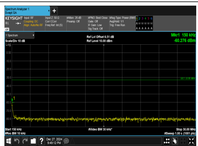
Band25-10MHz-QPSK-26090-1RB#0-0.15~30-PASS
