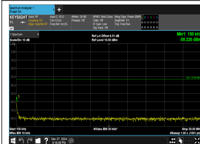
Band25-5MHz-16QAM-26665-1RB#0-0.15~30-PASS
