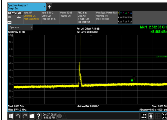
Band25-10MHz-QPSK-26090-1RB#49-1000~3000-PASS
