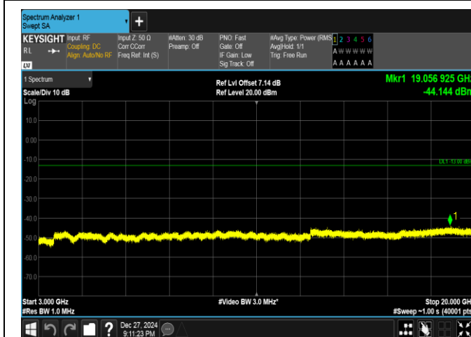
Band25-5MHz-16QAM-26365-1RB#0-3000~20000-PASS
