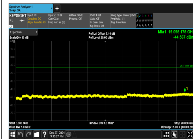
Band25-5MHz-16QAM-26365-25RB#0-3000~20000-PASS
