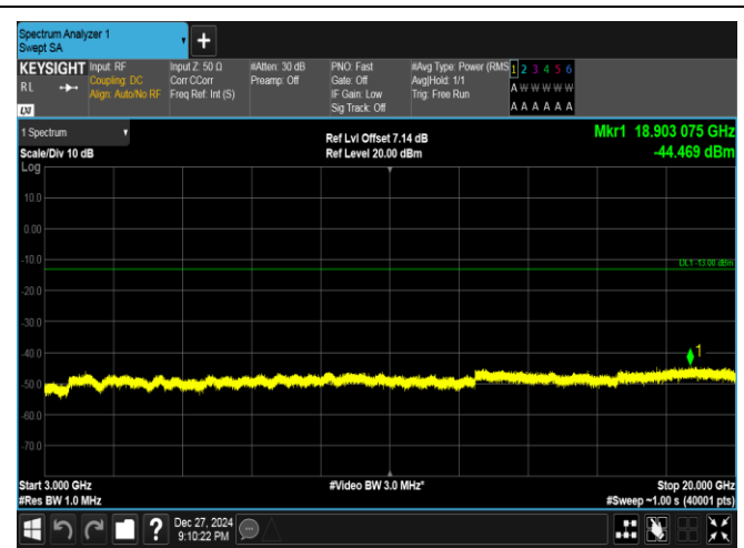
Band25-5MHz-QPSK-26365-1RB#0-3000~20000-PASS
