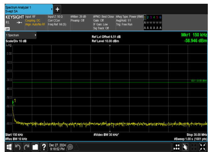
Band25-5MHz-16QAM-26665-1RB#24-0.15~30-PASS
