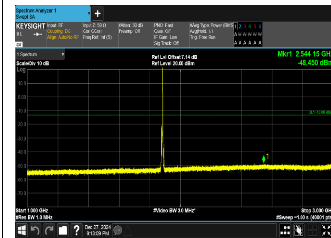
Band25-5MHz-16QAM-26365-1RB#24-1000~3000-PASS
