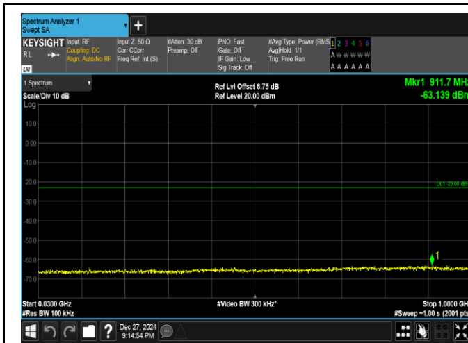
Band25-5MHz-16QAM-26365-25RB#0-30~1000-PASS
