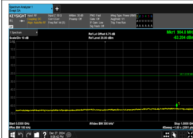
Band25-5MHz-16QAM-26065-1RB#24-30~1000-PASS
