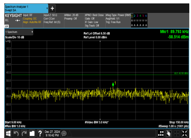
Band25-5MHz-16QAM-26665-1RB#0-0.009~0.15-PASS
