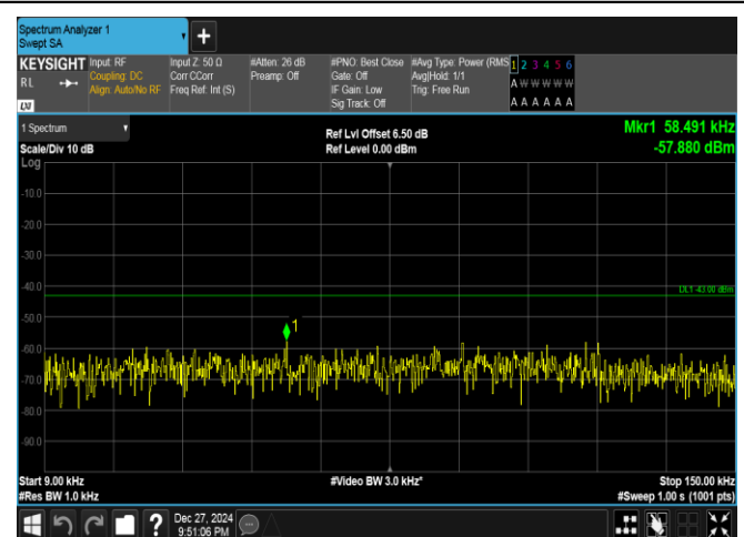
Band25-10MHz-QPSK-26090-1RB#49-0.009~0.15-PASS
