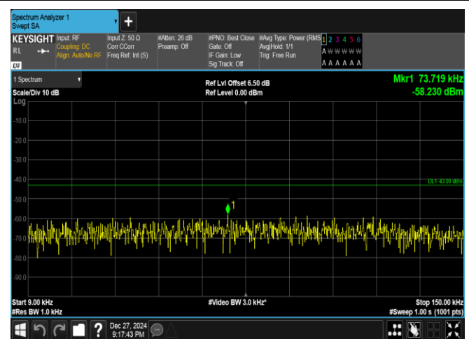
Band25-5MHz-QPSK-26665-1RB#24-0.009~0.15-PASS
