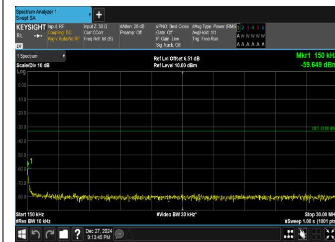
Band25-5MHz-QPSK-26365-25RB#0-0.15~30-PASS
