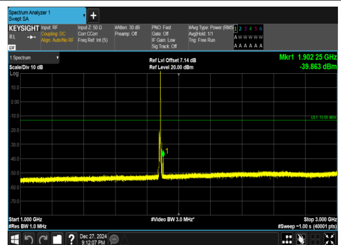
Band25-5MHz-QPSK-26365-1RB#24-1000~3000-PASS
