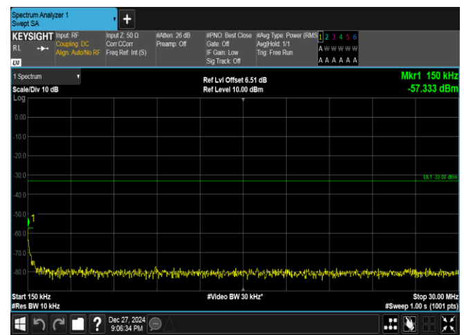
Band25-5MHz-16QAM-26065-1RB#24-0.15~30-PASS
