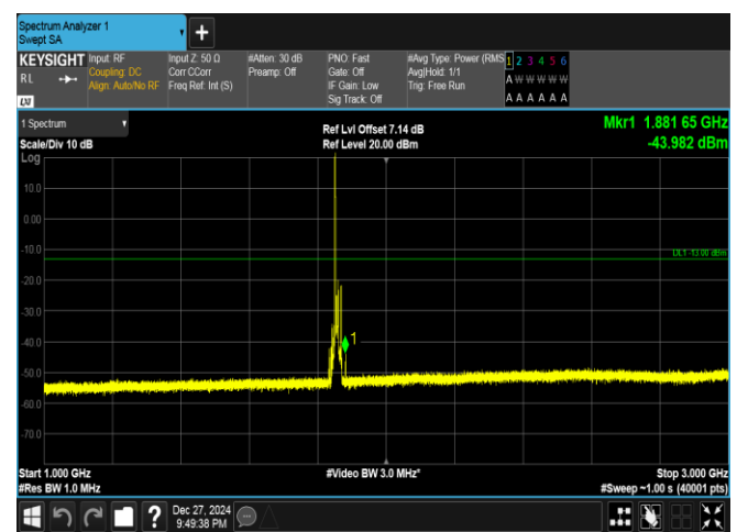
Band25-10MHz-QPSK-26090-1RB#0-1000~3000-PASS
