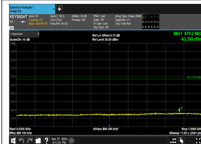
Band25-5MHz-QPSK-26365-1RB#24-30~1000-PASS
