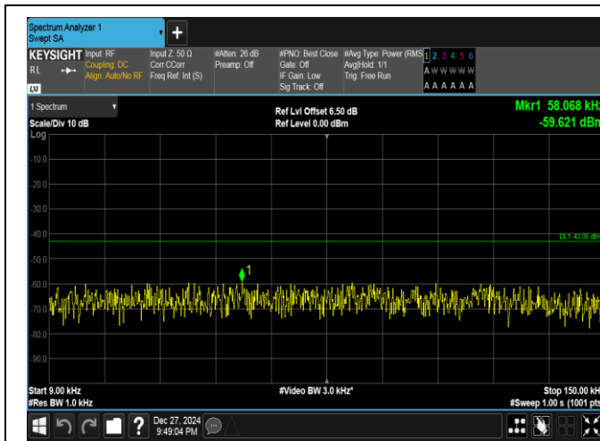
Band25-10MHz-QPSK-26090-1RB#0-0.009~0.15-PASS
