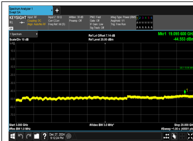
Band25-5MHz-QPSK-26365-1RB#24-3000~20000-PASS
