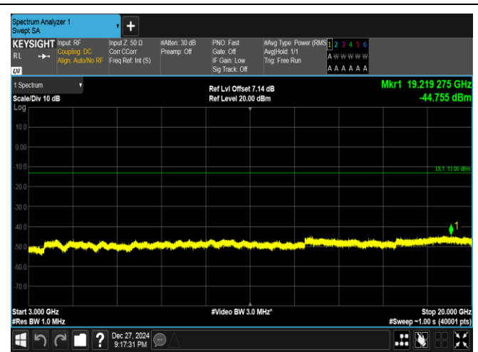
Band25-5MHz-16QAM-26665-1RB#0-3000~20000-PASS
