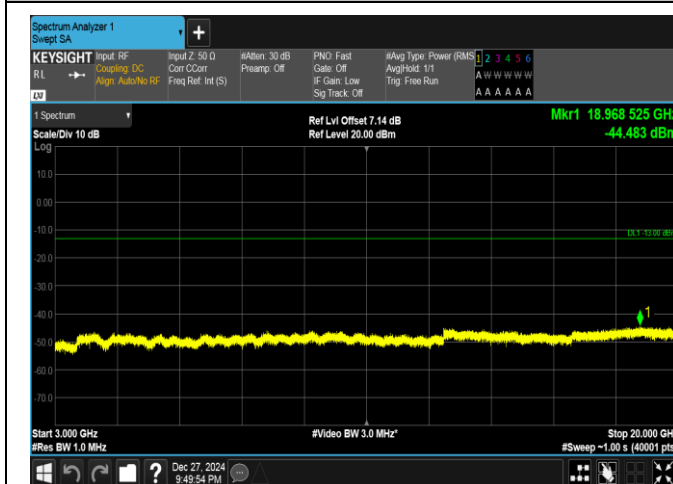
Band25-10MHz-QPSK-26090-1RB#0-3000~20000-PASS
