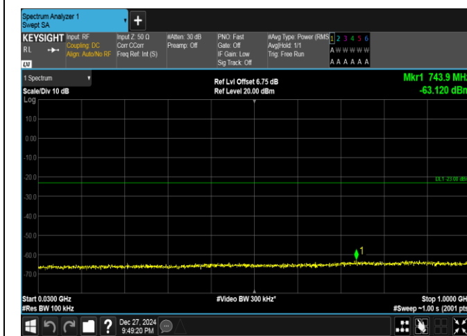
Band25-10MHz-QPSK-26090-1RB#0-30~1000-PASS
