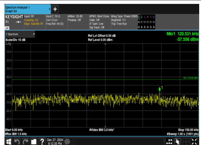
Band25-5MHz-16QAM-26365-1RB#24-0.009~0.15-PASS
