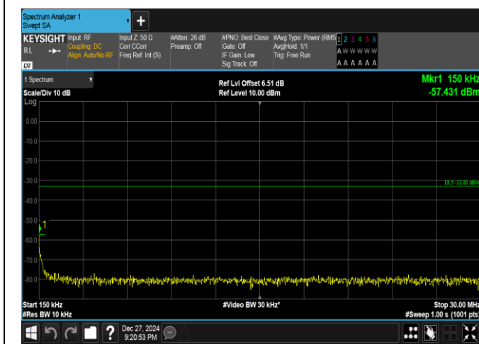
Band25-5MHz-16QAM-26665-25RB#0-0.15~30-PASS
