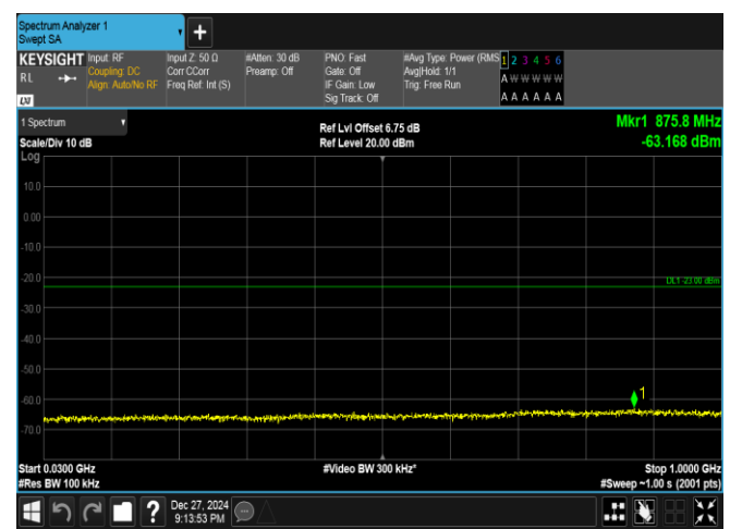
Band25-5MHz-QPSK-26365-25RB#0-30~1000-PASS
