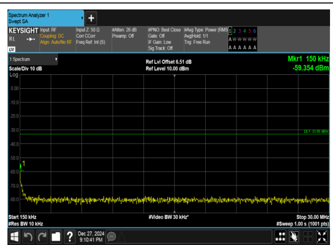
Band25-5MHz-16QAM-26365-1RB#0-0.15~30-PASS
