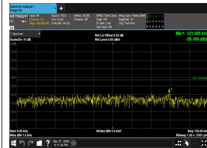
Band25-5MHz-QPSK-26365-1RB#24-0.009~0.15-PASS
