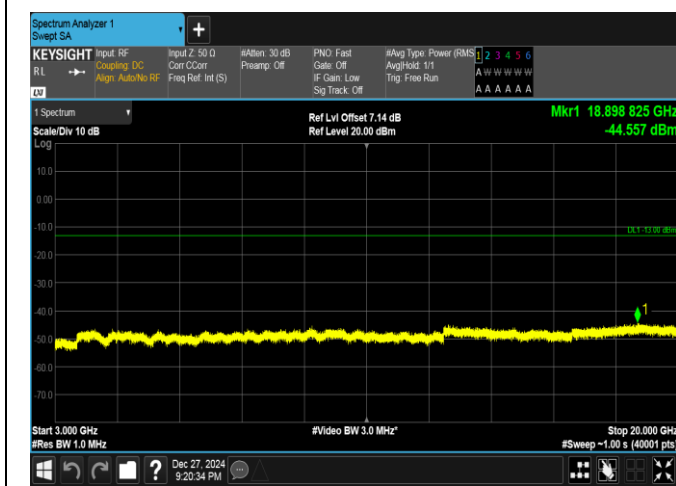
Band25-5MHz-QPSK-26665-25RB#0-3000~20000-PASS
