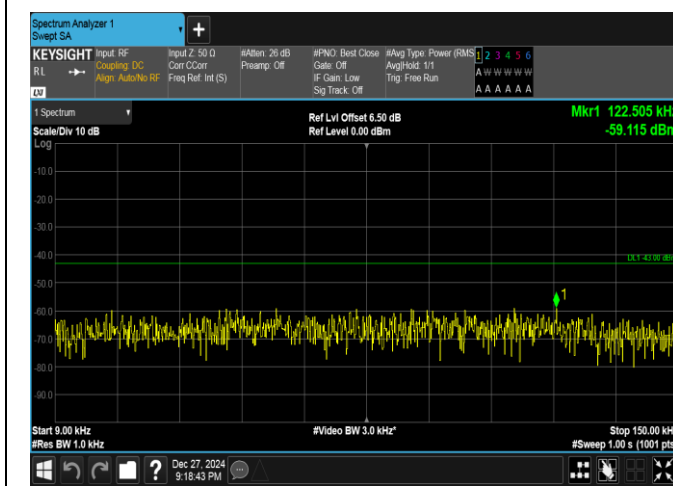
Band25-5MHz-16QAM-26665-1RB#24-0.009~0.15-PASS
