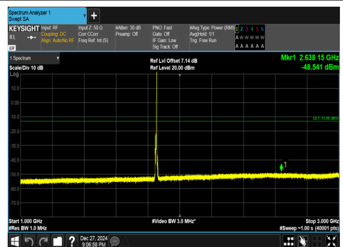
Band25-5MHz-16QAM-26065-1RB#24-1000~3000-PASS
