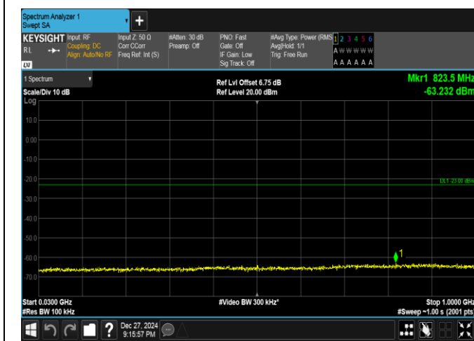
Band25-5MHz-QPSK-26665-1RB#0-30~1000-PASS
