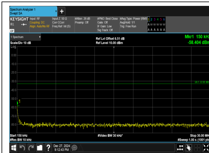
Band25-5MHz-16QAM-26365-1RB#24-0.15~30-PASS
