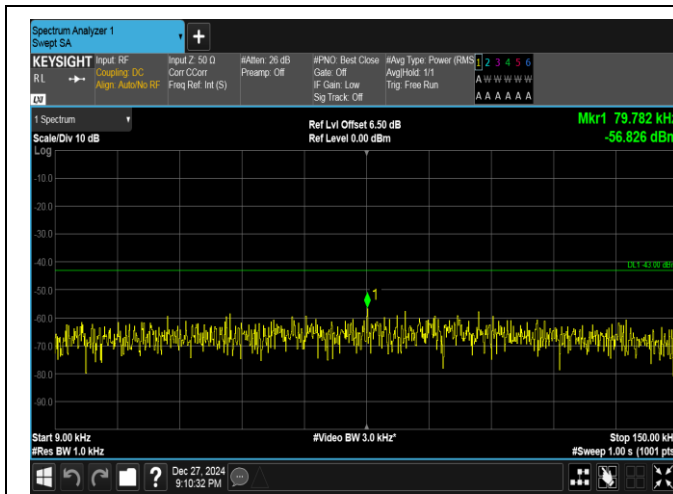
Band25-5MHz-16QAM-26365-1RB#0-0.009~0.15-PASS
