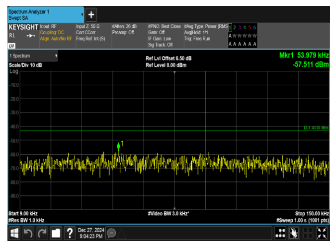
Band25-5MHz-16QAM-26065-1RB#0-0.009~0.15-PASS
