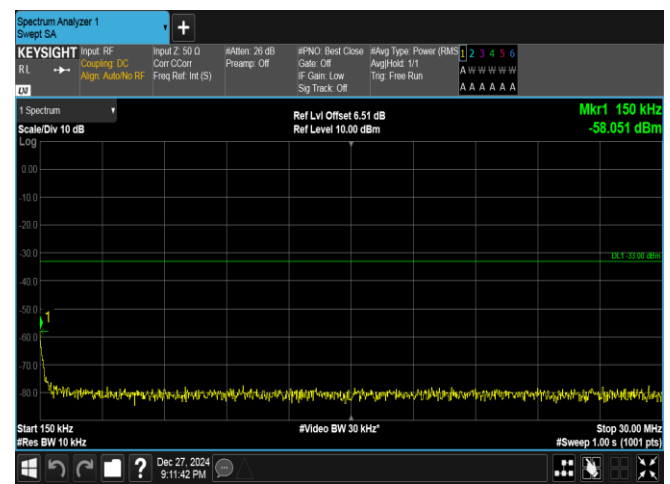
Band25-5MHz-QPSK-26365-1RB#24-0.15~30-PASS
