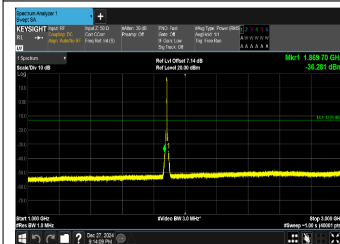
Band25-5MHz-QPSK-26365-25RB#0-1000~3000-PASS
