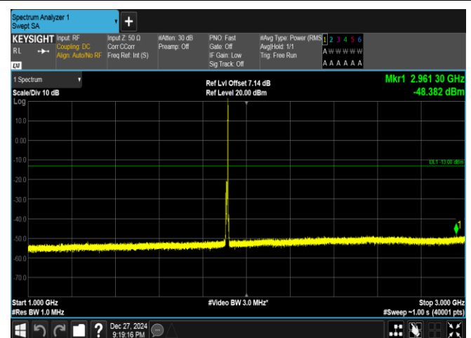
Band25-5MHz-16QAM-26665-1RB#24-1000~3000-PASS
