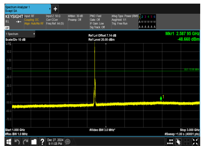
Band25-5MHz-16QAM-26365-1RB#0-1000~3000-PASS
