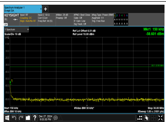
Band25-5MHz-QPSK-26065-1RB#0-0.15~30-PASS
