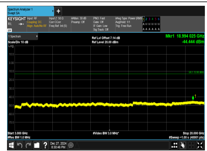
Band25-3MHz-16QAM-26675-1RB#0-3000~20000-PASS
