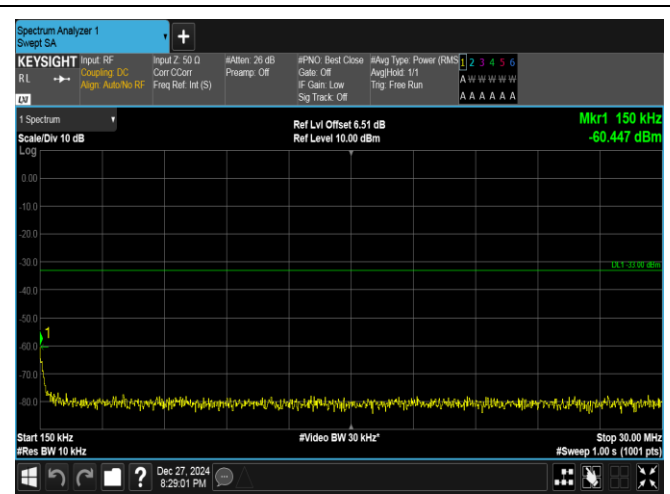
Band25-3MHz-QPSK-26675-1RB#0-0.15~30-PASS
