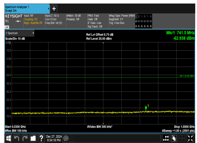
Band25-3MHz-16QAM-26675-15RB#0-30~1000-PASS
