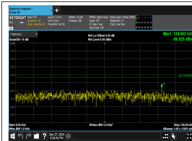
Band25-3MHz-QPSK-26675-1RB#0-0.009~0.15-PASS
