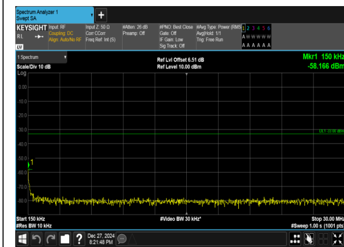
Band25-3MHz-16QAM-26055-15RB#0-0.15~30-PASS
