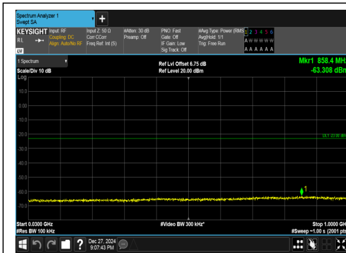
Band25-5MHz-QPSK-26065-25RB#0-30~1000-PASS
