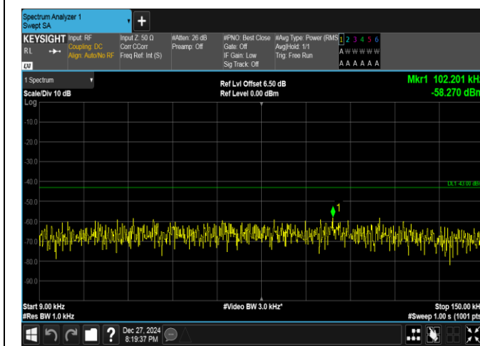
Band25-3MHz-16QAM-26055-1RB#14-0.009~0.15-PASS
