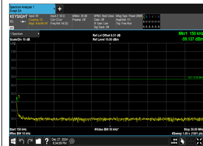
Band25-3MHz-16QAM-26675-15RB#0-0.15~30-PASS
