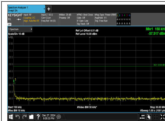
Band25-5MHz-QPSK-26065-1RB#24-0.15~30-PASS
