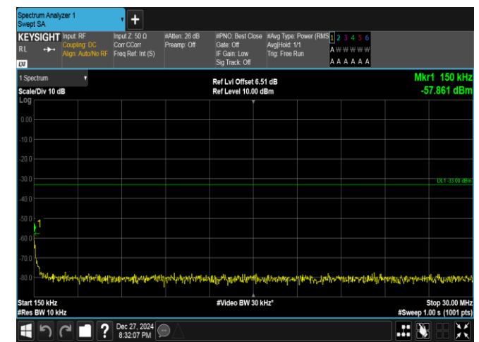
Band25-3MHz-16QAM-26675-1RB#14-0.15~30-PASS
