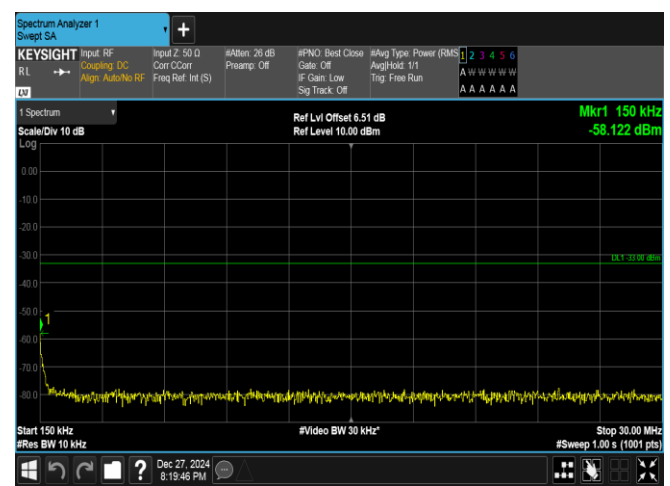
Band25-3MHz-16QAM-26055-1RB#14-0.15~30-PASS
