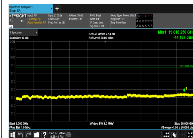
Band25-3MHz-QPSK-26675-1RB#0-3000~20000-PASS
