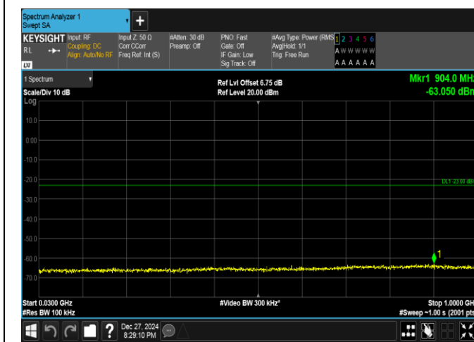
Band25-3MHz-QPSK-26675-1RB#0-30~1000-PASS
