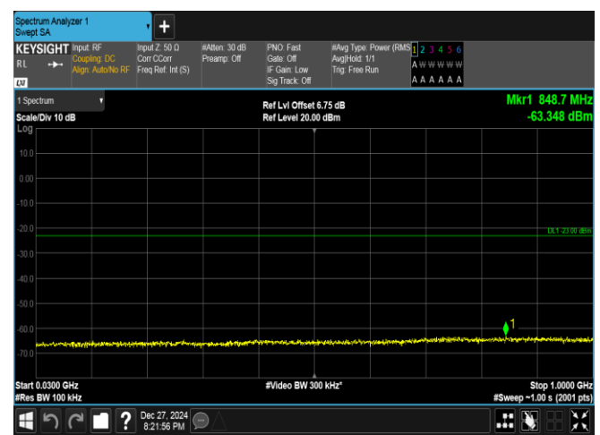
Band25-3MHz-16QAM-26055-15RB#0-30~1000-PASS
