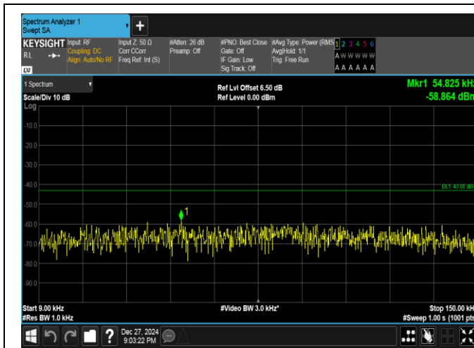
Band25-5MHz-QPSK-26065-1RB#0-0.009~0.15-PASS
