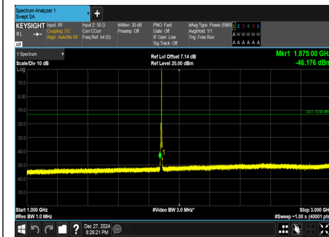
Band25-3MHz-16QAM-26365-1RB#14-1000~3000-PASS
