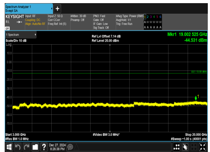
Band25-3MHz-16QAM-26365-1RB#14-3000~20000-PASS
