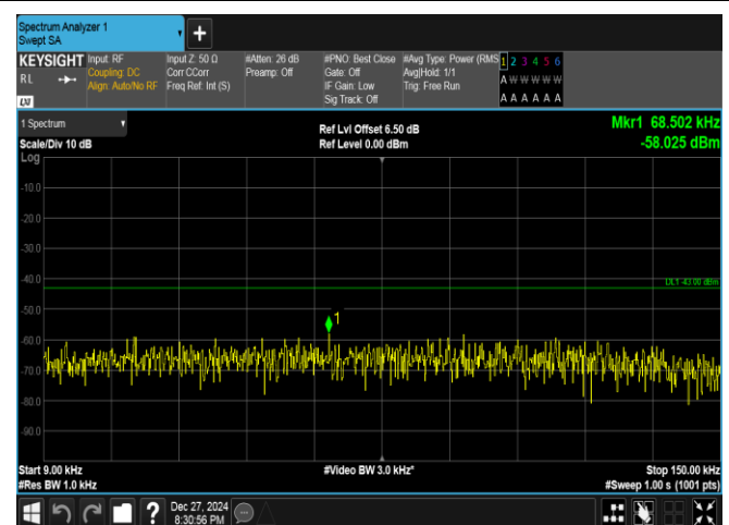
Band25-3MHz-QPSK-26675-1RB#14-0.009~0.15-PASS
