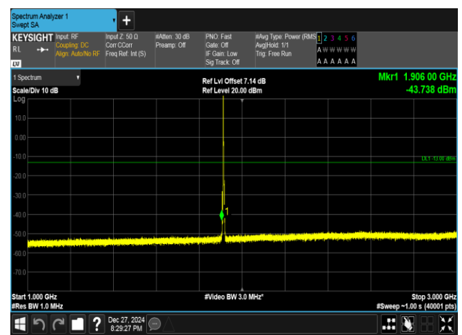
Band25-3MHz-QPSK-26675-1RB#0-1000~3000-PASS
