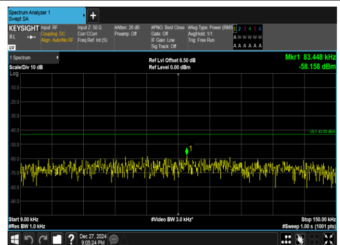
Band25-5MHz-QPSK-26065-1RB#24-0.009~0.15-PASS
