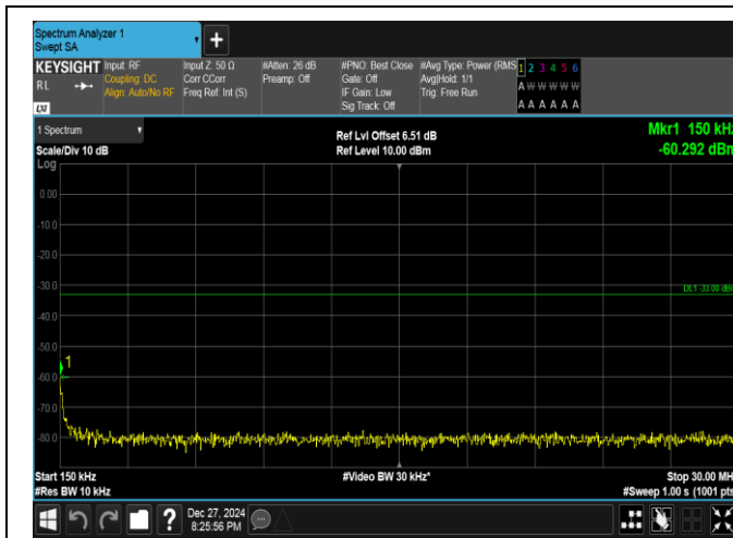
Band25-3MHz-16QAM-26365-1RB#14-0.15~30-PASS
