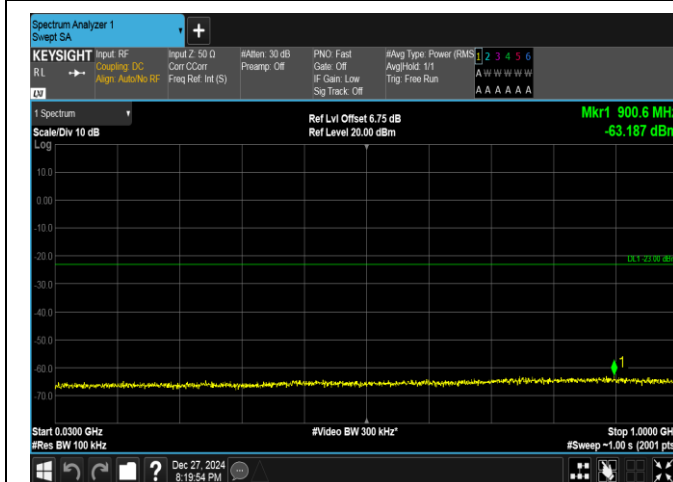
Band25-3MHz-16QAM-26055-1RB#14-30~1000-PASS
