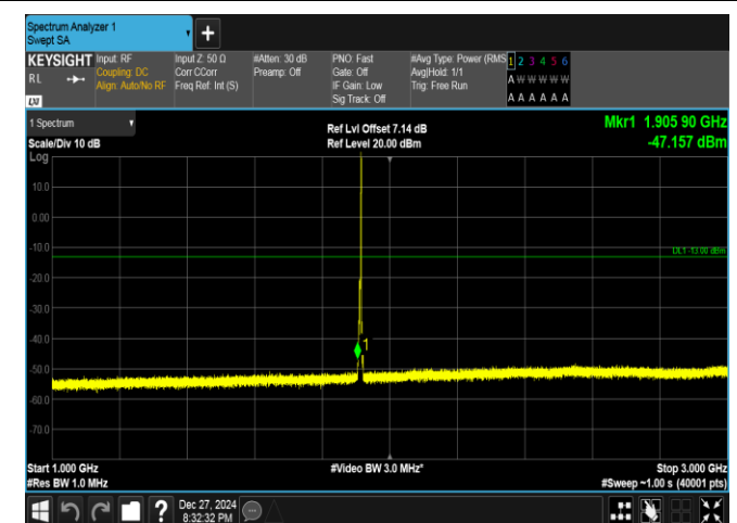
Band25-3MHz-16QAM-26675-1RB#14-1000~3000-PASS
